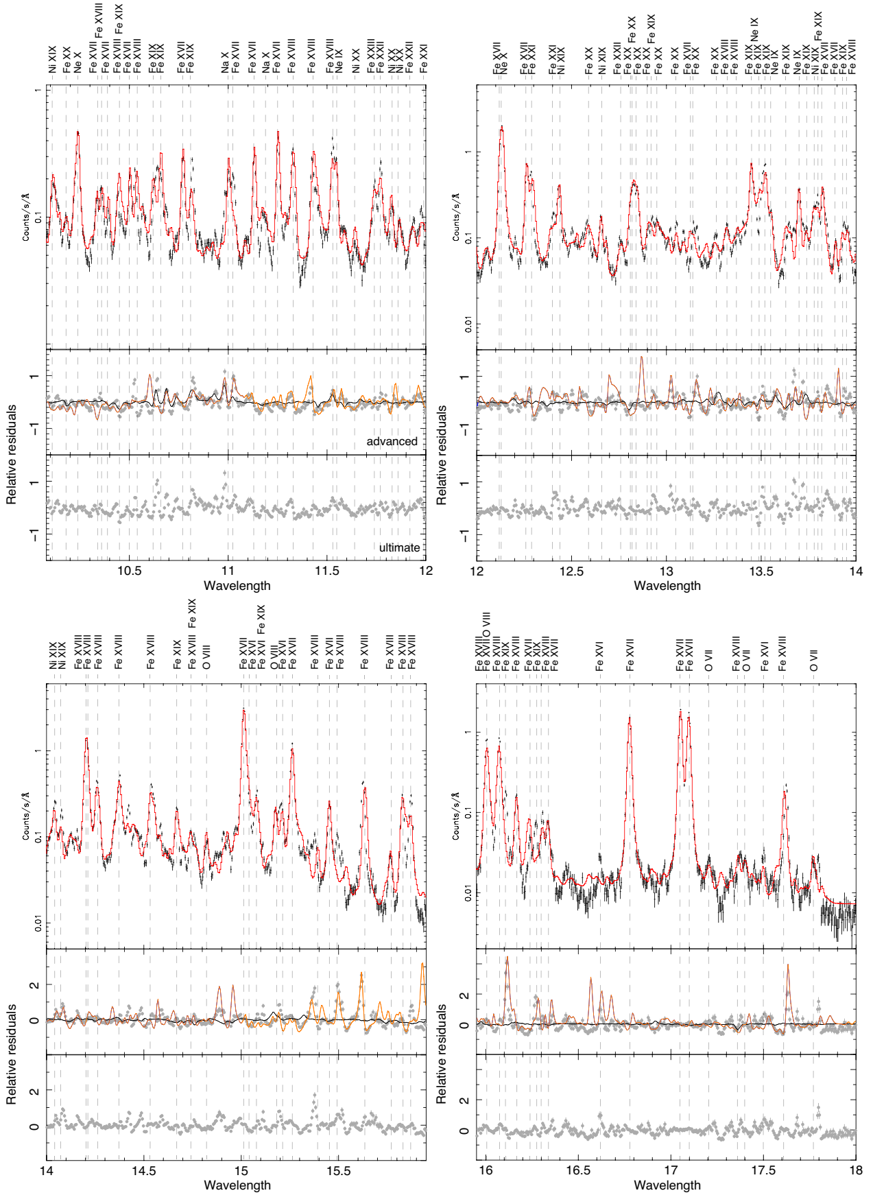
Fig. B.2. Same as Fig. B.1, but in 10.08 - 18 \text{ \AA} .
