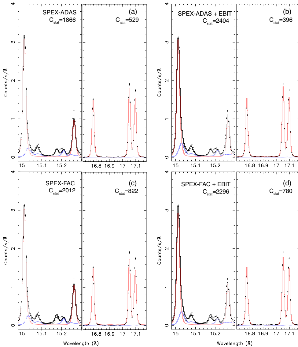
Fig. 13. Advanced fits shown in the wavelength ranges of 14.98 – 15.3 Å and 16.7 – 17.18 Å. The fits with SPEX-ADAS and SPEX-FAC calculations are plotted in panels (a) and (c), and those with EBIT-calibrated rates are shown in panels (b) and (d). Total model, Fe XVII transitions, and Fe XVI transitions are shown in black, red, and blue. Local C-stat values are given at the top. The total model is omitted in the 17 Å plot, as it would overlap with the Fe XVII lines.
