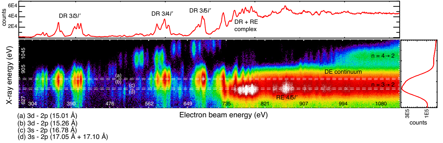
Fig. 1. EBIT X-ray data as a function of the electron beam energy (abscissa) and the photon energy (ordinate), corrected for the carbon foil transmission and the varying beam current. Color shows the number of counts. Photon energies of the main 3d - 2p and 3s - 2p transitions of Ne-like Fe are marked with the dashed lines. The upper and right panels show the count profiles projected along the beam energy and the photon energy, respectively.
