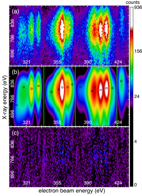
Fig. 2. (a) EBIT data of the dielectronic recombination from 3l3l' states (where two electrons are excited to n = 3 ). (b) Best-fit model, the central position of each peak is marked by a black box. The boundaries of the regions of interest are shown by green lines. (c) Background noise and residual of the fit.
