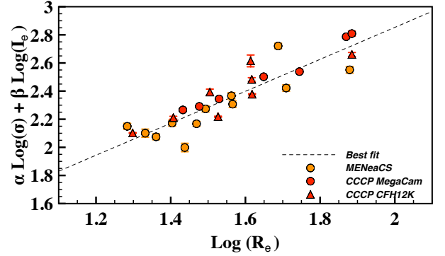
Figure 1. We use our spectral and imaging measurements to plot the fundamental plane for our BCGs, using \alpha = 1.24 and \beta = -0.80 from Bildfell et al. (2008) and Bildfell (2013). The MENeACS BCGs are indicated with orange symbols, and the CCCP BCGs in red (MegaCam imaging in circles and CFH12K imaging in triangles). We measure an intrinsic scatter of 0.095.
