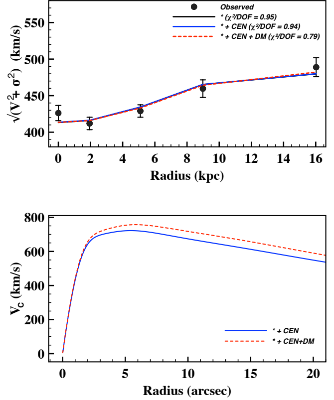
Figure 4. Top: The averaged second moment of velocity ( \sqrt{V^2 + \sigma^2} ) profile for Abell 2261 with three combinations of mass models shown. Bottom: Circular velocity curves for the total mass (red dashed), and for the central plus stellar mass only (blue solid).
