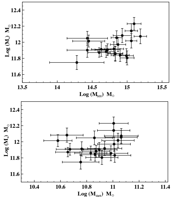
Figure 7. We show the enclosed stellar mass ( M_{\text{stellar}} ) for a sphere with a radius of 15 kpc, against the halo mass at M_{500} from weak lensing (Herbonnet et al. 2019), as well as against the enclosed dark matter mass ( M_{\text{dark}} ) for a sphere with a radius of 15 kpc.
