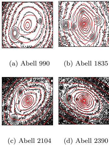
Figure B2. MGE: Cases where the features in the r -band images were particularly problematic, and could not be completely removed. These are not used in the dynamical modelling.
