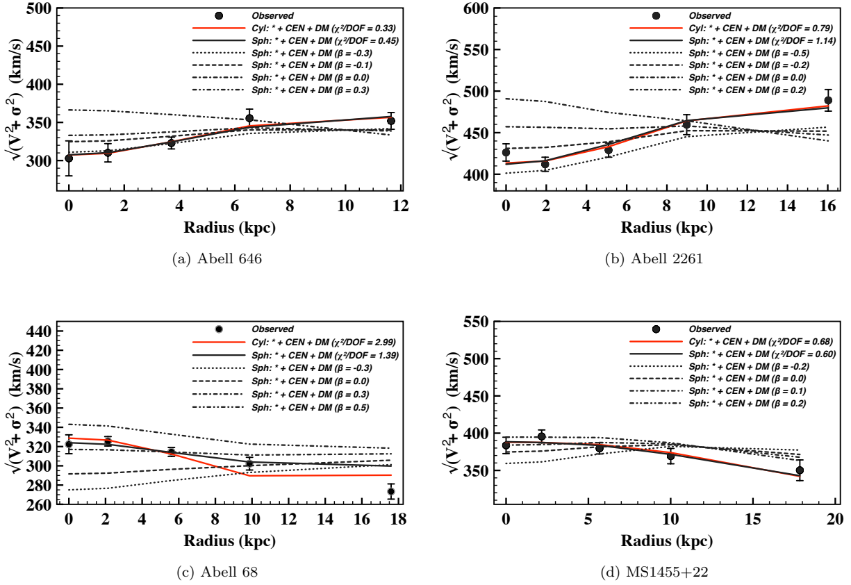
Figure 9. In each case, the solid red line shows the best-fitting cylindrically-aligned JAM model, and the black solid line shows the best-fitting spherically-aligned JAM sph model. In each case we also show JAM sph models progressively changing \beta from tangential anisotropy to radial anisotropy (where \Upsilon_{\star\text{DYN}} was kept constant at the best-fitting \Upsilon_{\star\text{DYN}} derived from the JAM cylindrically-aligned models) to show the change in the predicted \nu_{\text{rms}} slope as a function of \beta .
