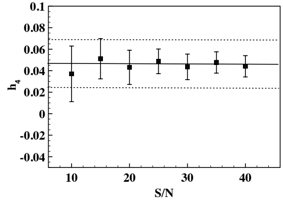
Figure 2. We use the spectrum of the BCG in Abell 68 as an example, and create mock spectra of different S/N , and repeat measurements of h_4 50 times using Monte Carlo simulations. We plot the average measurements for the spectra with different S/N , where the solid and dotted lines indicate our actual h_4 measurement and error bars, respectively. We conclude that we are not biased in our h_4 measurements as a result of poor S/N .
