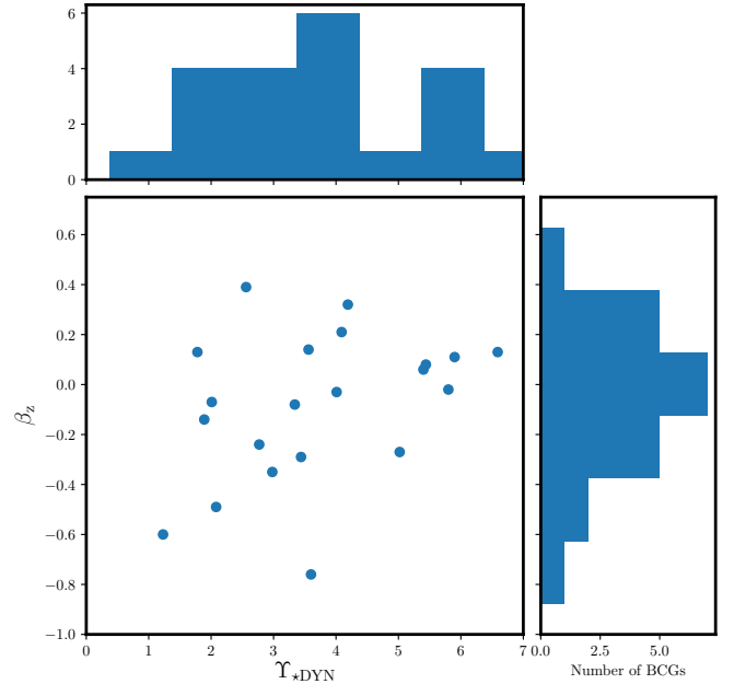
Figure 6. We show the distributions of the best-fitting free parameters ( \Upsilon_{\star\text{DYN}} , \beta_z ) for the mass model with all three components ( \star + \text{CEN} + \text{DM} ). The dynamical modelling results of the BCGs in Abell 2055 and 963 are excluded. The typical error on \beta_z is 0.02, and the typical error on \Upsilon_{\star\text{DYN}} is < 0.2 (see Table 3). We find a wide range of best-fitting values for both parameters.
