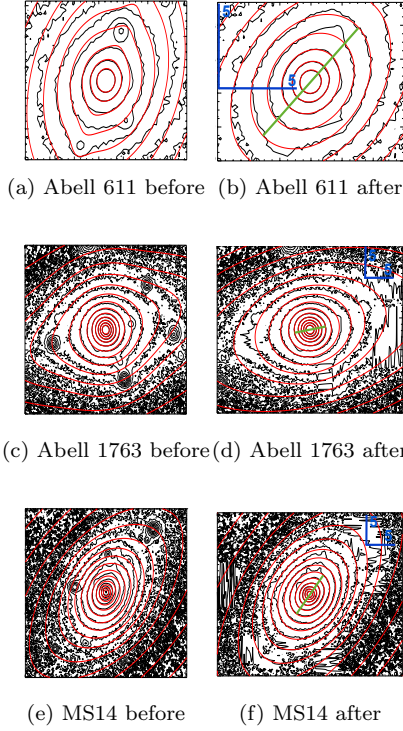
Figure B1. MGE: before and after examples where the r -band images were masked to improve the MGE model fitting.
