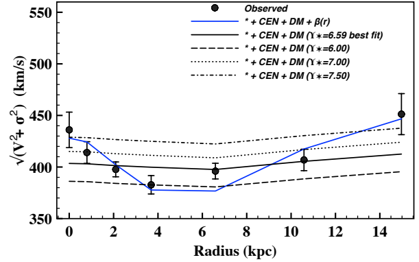
Figure 10. We show the model fit for all three mass components ( \star + \text{CEN} + \text{DM} ) for Abell 2029, where the best-fitting value for a constant \Upsilon_{\star\text{DYN}} (solid line), and lines for other constant values for \Upsilon_{\star\text{DYN}} , are shown in black. We also show a fit for a variable \beta_z(r) from radial to tangential anisotropy (in blue). A similar fit could be achieved by first decreasing and then increasing \Upsilon_{\star\text{DYN}}(r) .
