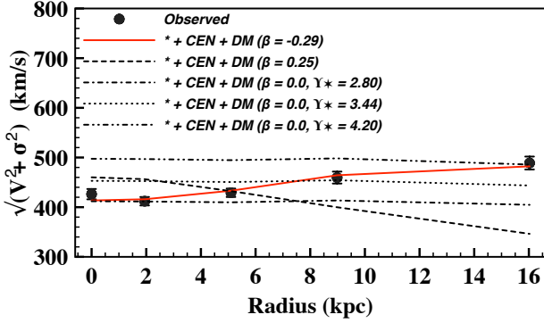
Figure 11. Fits to the observed kinematics, illustrated for the BCG in Abell 2261 for \beta_z negative, positive or zero.
