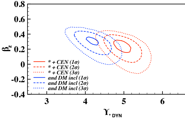
Figure 5. We show the free parameters \beta_z and \Upsilon_{\star\text{DYN}} , with the 1\sigma (68 per cent), 2\sigma (95.4 per cent), 3\sigma (99.73 per cent) confidence contours indicated, for the fit with just the stellar and central mass components i.e. assuming dark matter does not contribute to the total mass (red), and the stellar, central and dark matter components (blue) for the BCG in Abell 68 as an example. Adding the M_{\text{DM}} mass component decreases \Upsilon_{\star\text{DYN}} on average by 8.3 \pm 2.9 per cent over our kinematic range, and increases \beta_z by on average 0.04. This figure also illustrates that we can actually constrain \beta_z and \Upsilon_{\star\text{DYN}} quite well separately, and that even without using h_4 we can get reasonably good constraints on the \Upsilon_{\star\text{DYN}} .
