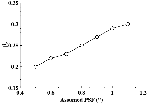
Figure D1. Illustrating the sensitivity of our dynamical modelling is to variations in the PSF, using the BCG in Abell 68 (with a measured PSF of 0.8'' ) as an example. Here, we use just a stellar mass component, and illustrate the increase in \beta_z with an increase in the PSF. As the PSF increases from 0.5'' to 1.1'' , \Upsilon_{\star\text{DYN}} also decreases from 5.10 to 4.84. The uncertainties of the measured PSFs are small ( <0.05'' ).
