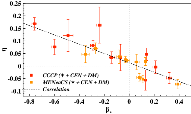
Figure 8. The correlation between best-fitting velocity anisotropy \beta_z and velocity dispersion slope ( \eta , as measured in Loubser et al. (2018)). We find a strong correlation between the two parameters, given by \eta = (-0.185 \pm 0.028)\beta_z + (0.013 \pm 0.008) , with an intrinsic scatter of 0.026, and correlation coefficient 0.929.
