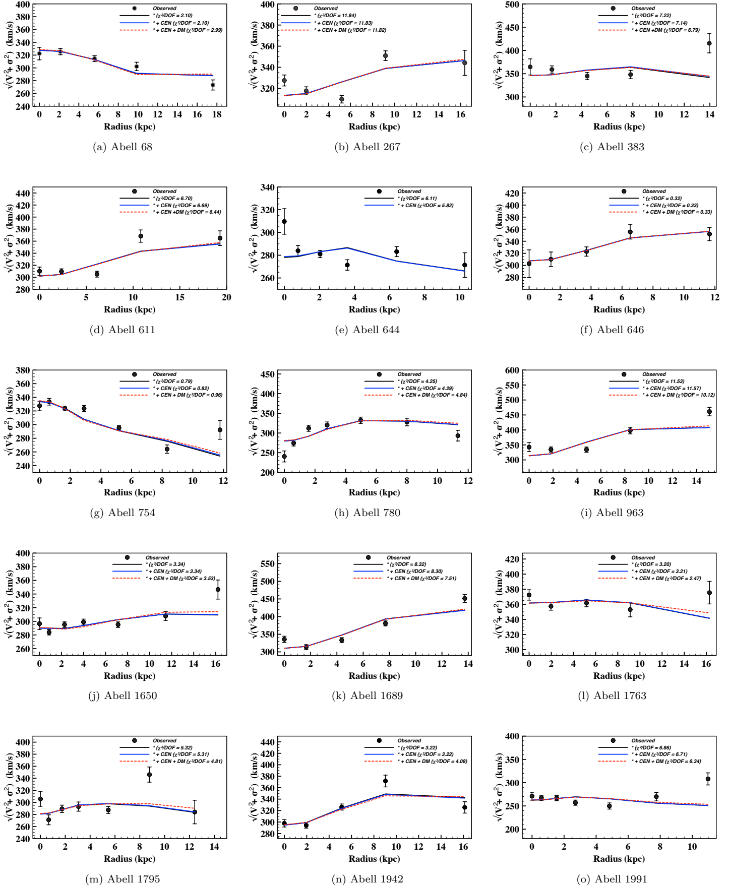
Figure H1. The averaged second moment of velocity ( \sqrt{V^2 + \sigma^2} ) profile.
