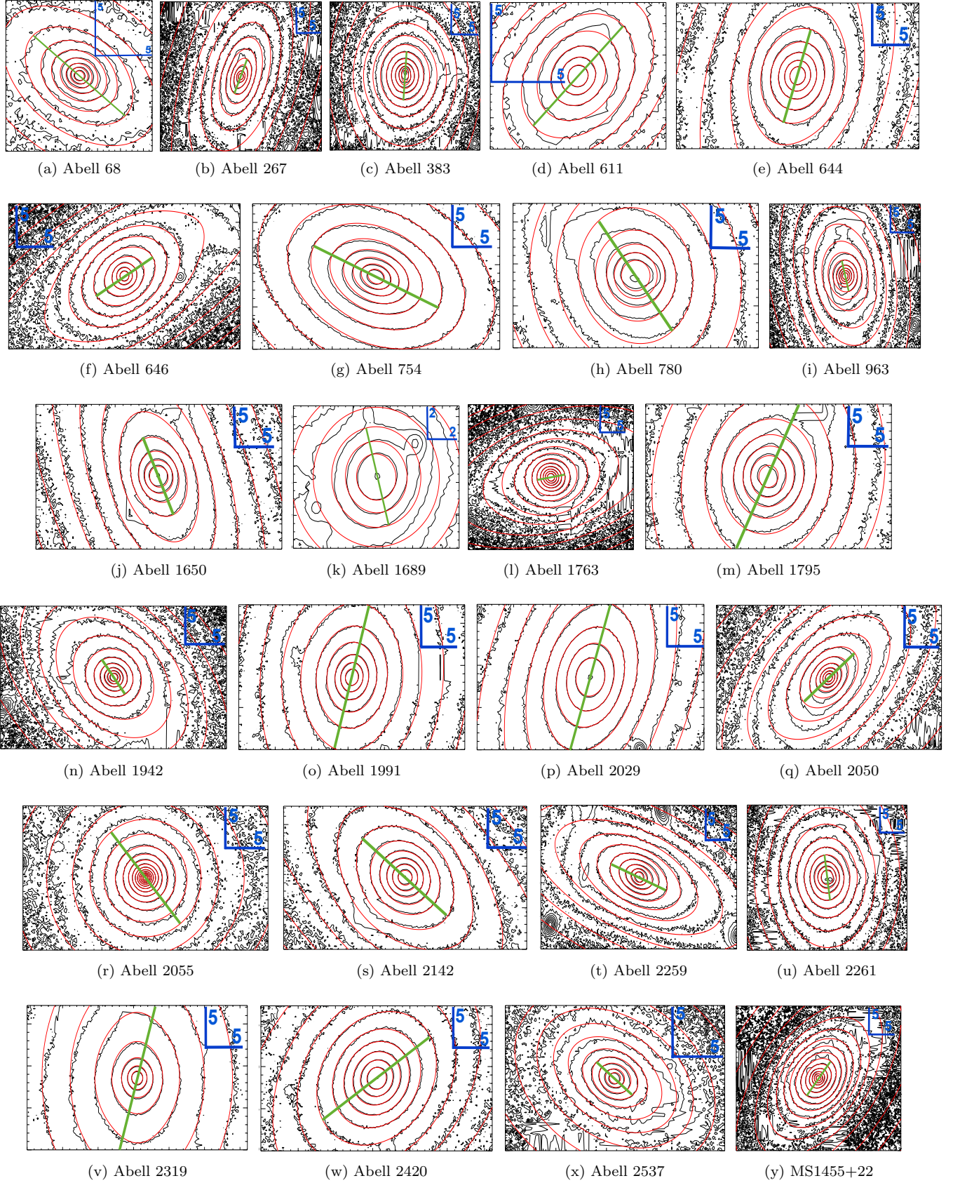
Figure B4. MGE fits to the r -band images. The green line indicates the position of the slit, and the blue lines the scale in arcsec.
