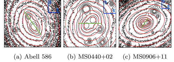
Figure B3. MGE: the BCGs with double nuclei. These are not used for the dynamical modelling.
