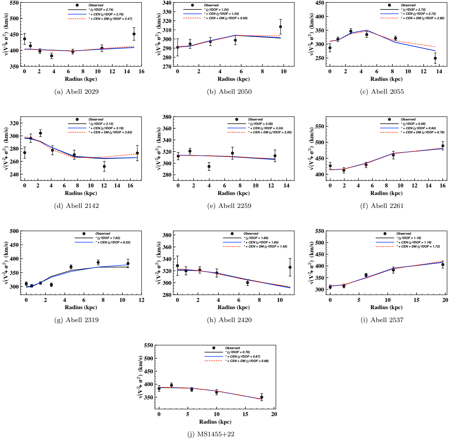
Figure H2. The averaged second moment of velocity ( \sqrt{V^2 + \sigma^2} ) profile.
