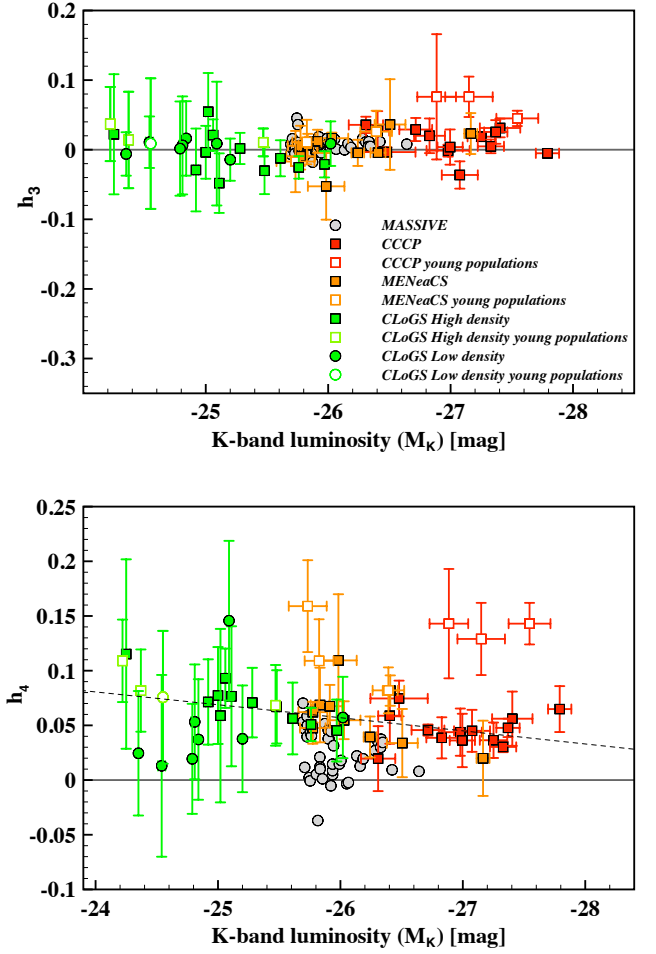
Figure 3. Top: the central h_3 measurements vs K -band luminosity. Here we also plot the averaged \langle h_3 \rangle within the effective radius for MASSIVE (Veale et al. 2017) for comparison (grey). Bottom: the central h_4 measurements vs K -band luminosity. We also plot the central h_4 for MASSIVE for comparison. The BCGs with young stellar components are plotted with open symbols, and likely suffer from template mismatch. The CLoGS BGGs with young components are results from preliminary analysis in preparation.
