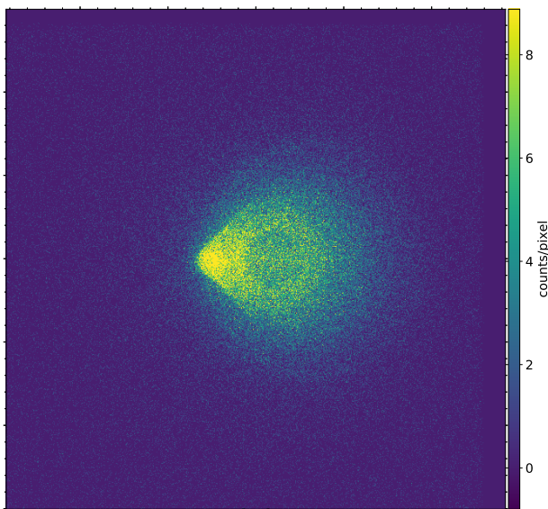
3:1 Mass - Noisy Mock Cluster Merger - Simulated Chandra - 65 deg
