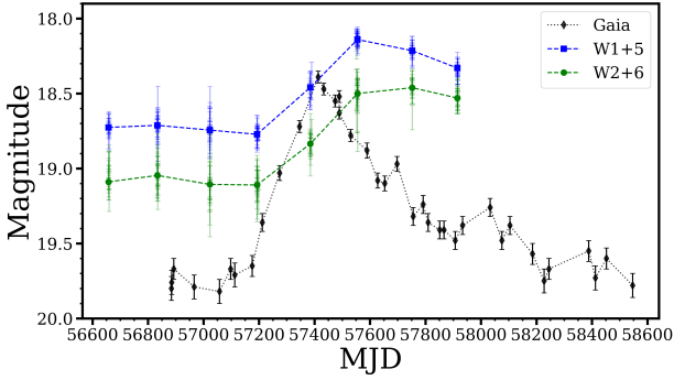
Figure 8. Lightcurve from the NEO-WISE mission, compared with the Gaia lightcurve. Plotted are the magnitudes in the two filters W1 (blue) and W2 (green), shifted along the y-axis to allow to compare with the Gaia data. Solid blue squares (W1) and green circles (W2) are the mean values of the exposures taken for each epoch. The NEO-WISE lightcurve reaches its peak with a delay of \sim 140 days with respect to the Gaia lightcurve.
