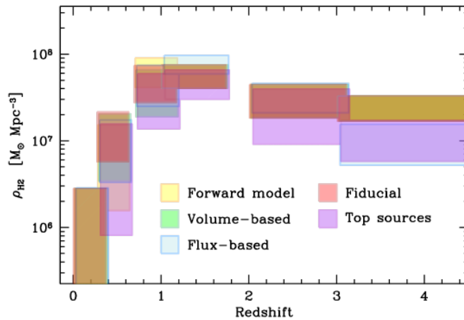
Figure 11. The evolution of the molecular gas cosmic density in galaxies as a function of redshift, shown under different treatments of the line candidates without a counterpart. Red boxes: our bona-fide constraints, as shown in Fig. 9. Green boxes: the probability distribution of line identification scales with the sampled volume in each transition, for both ASPECS bands. Yellow boxes: the probability distribution of line identification scales as the volume for 3 mm transitions, and as the predicted number of detections assuming the corresponding CO LFs from 3 mm at similar redshifts, and the large velocity gradient modeling of the CO spectral energy distribution from Boogaard et al. (2020). Blue boxes: the probability distribution scales as the observed flux distributions shown in Fig. 5. Purple boxes: Constraints on \rho_{\text{H}_2} based exclusively on the sources detected in the 1.2 mm dust continuum.
