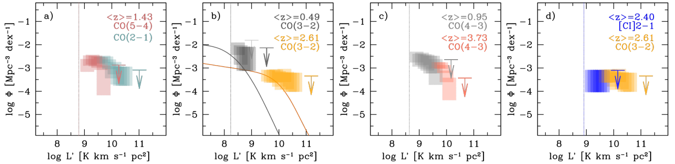
Figure 8. Comparison between CO and [C\text{I}]_{2-1} luminosity functions. a) The CO(2-1) (grey blue) and CO(5-4) (dark red) luminosity functions in the common redshift range around \langle z \rangle = 1.43 . The CO(2-1) luminosity function appears in systematic excess with respect to the CO(5-4), hinting at generally sub-thermalized conditions ( r_{52} < 0.3 , see text for details). b) The CO(3-2) luminosity functions observed at 3 mm and 1.2 mm at \langle z \rangle = 2.61 and \langle z \rangle = 0.49 , respectively. For comparison, the empirical predictions of the CO(3-2) luminosity functions based on Herschel IR luminosity functions by Vallini et al. (2016) are shown in grey ( z \sim 0 ) and orange ( z \sim 2 ) lines. The CO(3-2) LF appears to evolve from z \sim 2.6 to the present age. ASPECS data point to an evolution in the CO(3-2) luminosity function consistent with the empirical predictions, although the difference in the sampled luminosity ranges in the two redshift bins limits the robustness of this finding. c) Similar to the previous panel, but for the CO(4-3) luminosity functions observed at z \sim 0.95 at 1.2 mm and at z \sim 3.7 at 3 mm. d) Comparison between the [C\text{I}]_{2-1} and CO(3-2) luminosity functions at z \sim 2.5 . We find an offset of \gtrsim 0.5 dex between the two luminosity functions, broadly in agreement with similar ratios between the two line luminosities reported in the literature from studies of individual sources (see Sec. 4.2).
