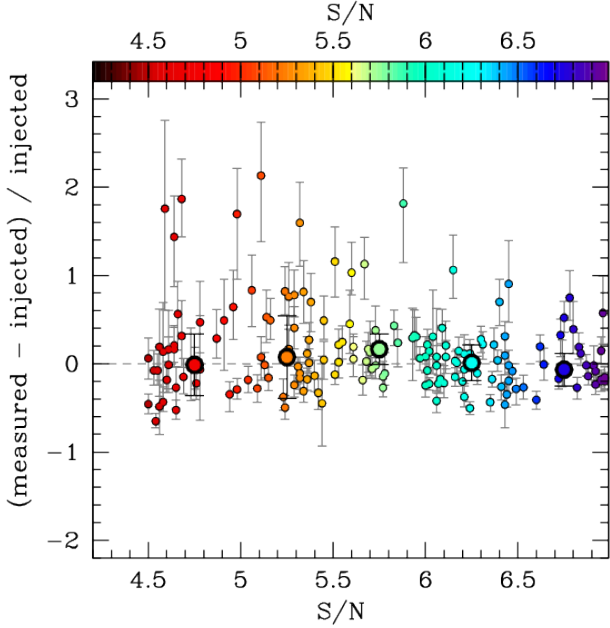
Figure 3. The impact of flux boosting on our analysis, estimated by comparing the injected and measured fluxes of mock lines. Small symbols show a random subset of individual mock lines, larger symbols are median values in bins of \Delta S/N=0.5 . Flux boosting affects the flux measurement of \approx 10\% of lines at S/N < 5 , and is completely negligible at S/N > 6 .
