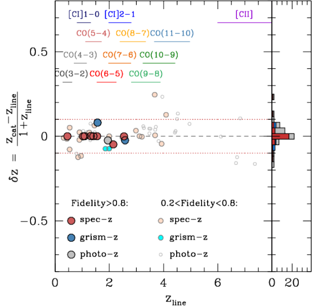
Figure 4. Redshift match from the line search in the ASPECS LP 1.2 mm mosaic, z_{\text{line}} , and the ancillary catalog values, z_{\text{cat}} , based on the 3D-HST catalog (Skelton et al. 2014), augmented with the most up to date spectroscopic information (see Sec. 2.2 for details). We consider good matches cases where |\delta z| < 0.1 ( < 0.01 for sources with spectroscopic redshifts). All of the high fidelity lines have a matching redshift in the catalog. The redshift ranges mapped by the various transitions considered in this work are marked as horizontal bars.
