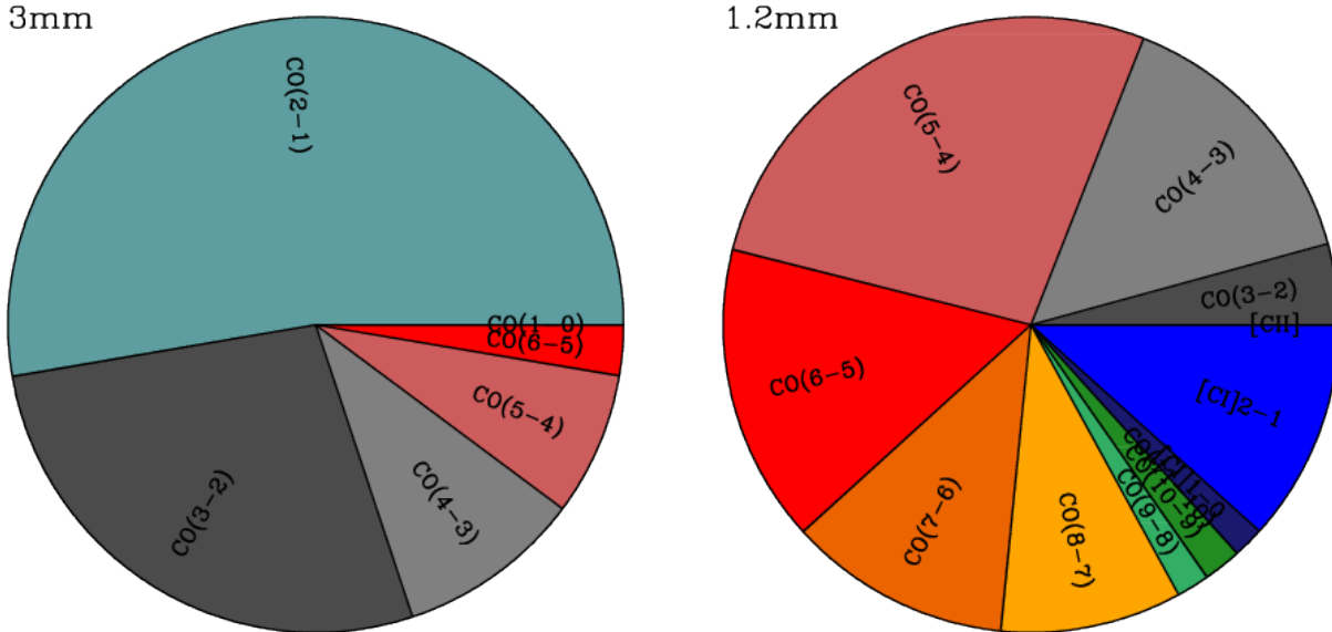
Figure 5. Pie charts of the fidelity-corrected flux distribution of the lines detected in the ASPECS LP 3 mm ( left ) and 1.2 mm ( right ) cubes. The 3 mm cube is dominated by low- J CO transitions observed at z=1-3 . At 1.2 mm, about 62% of the total line emission arises from CO transitions with intermediate J=3-6 . Higher- J transitions account for 25% of the total line flux in the 1.2 mm band. The two [C I] lines account for \sim 12\% of the total line emission, while [C II] contributes <1\% .
