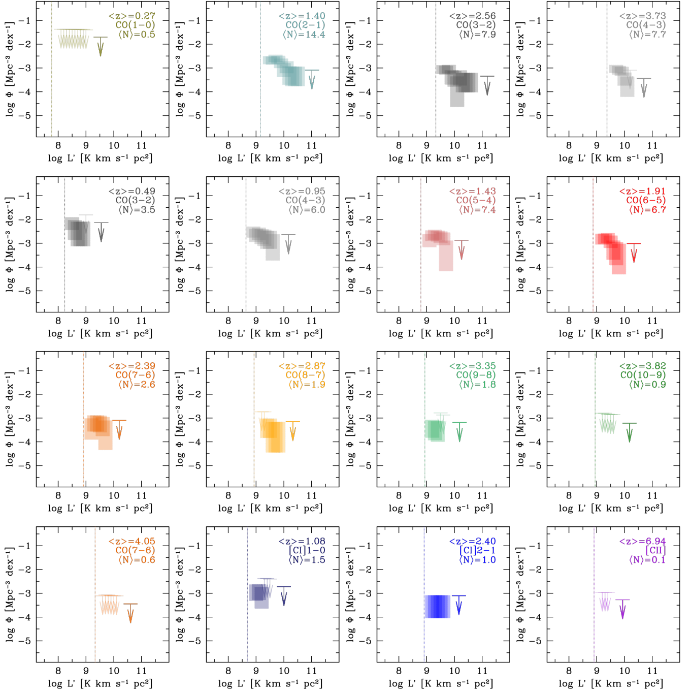
Figure 7. Constraints on the CO, [C I], and [C II] luminosity functions from ASPECS. The vertical extent of the boxes shows the average \pm 1\text{-}\sigma range in each 0.5 dex bin. For each transition, we report the volume-averaged redshift, and the average number of line candidates used in the various LF realizations. Bins with an average of > 1 line candidate entry per realization are shown as boxes, while arrows mark the corresponding 3- \sigma limits for all of the other bins. The vertical bars show the formal 5- \sigma line luminosity limit (see Table 1).
