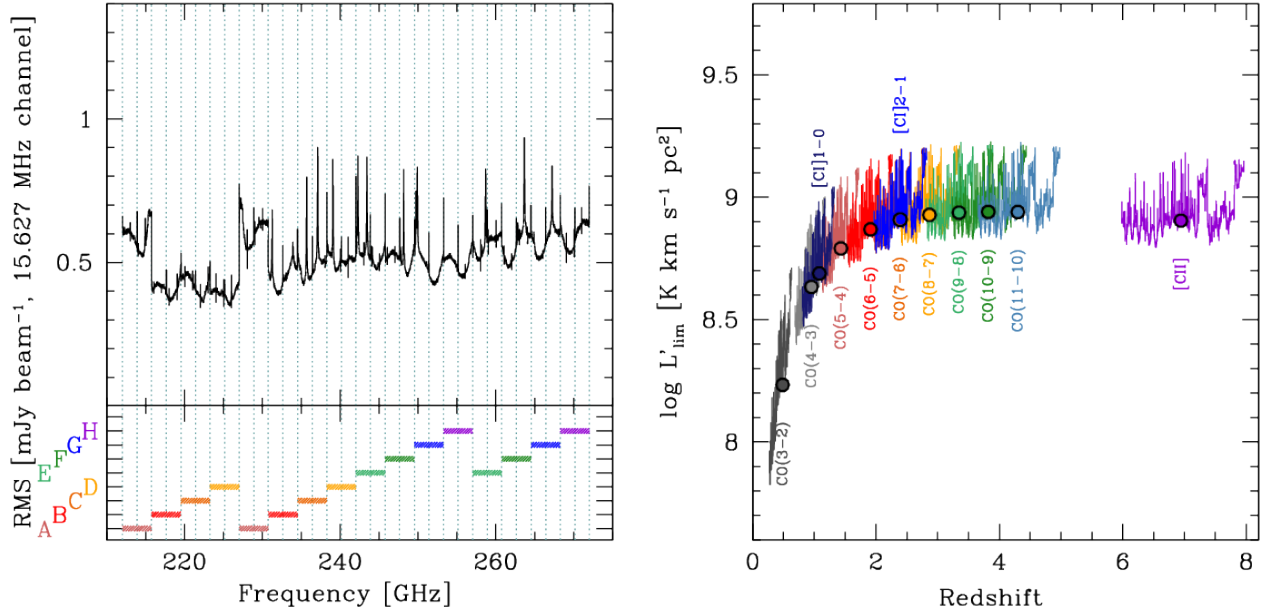
Figure 1. Sensitivity limits of the ASPECS 1.2mm cube. Left: Channel rms as a function of frequency. For a 15.6 MHz channel, the typical rms is \sim 0.5 \text{ mJy beam}^{-1} throughout the entire band. The frequency settings used in the observations (labeled A–H) and the edges of each spectral window are also marked. Right: Line luminosity limits (in units of \text{K km s}^{-1} \text{ pc}^2 ) as a function of redshift. Here we assume a 5\text{-}\sigma limit for a line width of 200 \text{ km s}^{-1} . The dots highlight the fiducial limit, obtained as the median sensitivity throughout the band.
