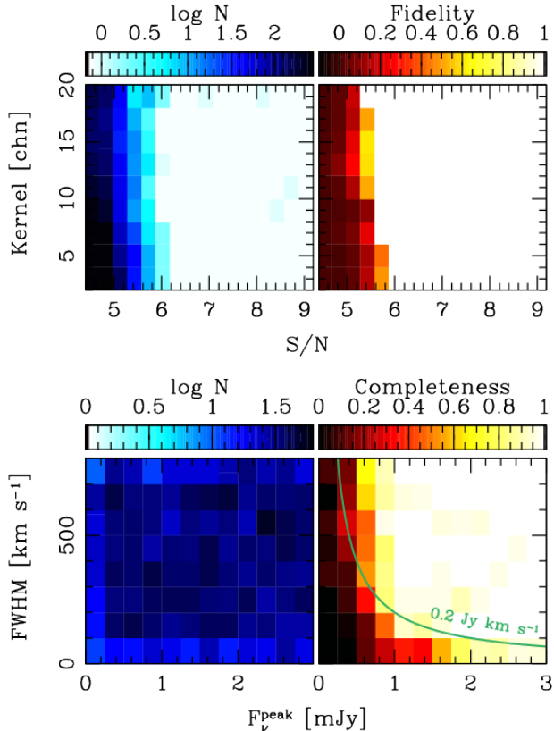
Figure 2. Top-left: Number of observed (positive) line candidates from the line search as a function of S/N and kernel width that maximized the S/N of the line candidate in the line search. Top-right: Best-fits of the fidelity dependence on S/N and kernel width. The fidelity of line candidate is close to unity at S/N > 5.8 , and drops rapidly to zero at S/N < 5 . The fidelity at a given S/N increases with increasing line widths, as expected because of the fewer independent noise realizations in the cubes. Bottom-left: Number of simulated lines injected in the cube for completeness assessments, as a function of line peak flux, F_{\nu}^{\text{peak}} , and width (parametrized as FWHM). Only lines located within the footprint at >50\% response in the cube. Bottom-right: Completeness of the line search. The completeness is \gtrsim 90\% for virtually any line with integrated flux larger than 0.2 \text{ Jy km s}^{-1} (indicated by a green solid line) and peak fluxes of >1 \text{ mJy} .
