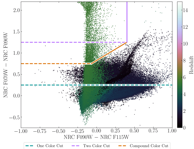
Figure 8. NIRCcam color-color plot with the three selection criteria that we employ and compare in this paper. In lavender, we show the two-color selection method used in Section 3.1. In teal and orange, we show the One Color and Compound Color Cut selection methods, respectively.
