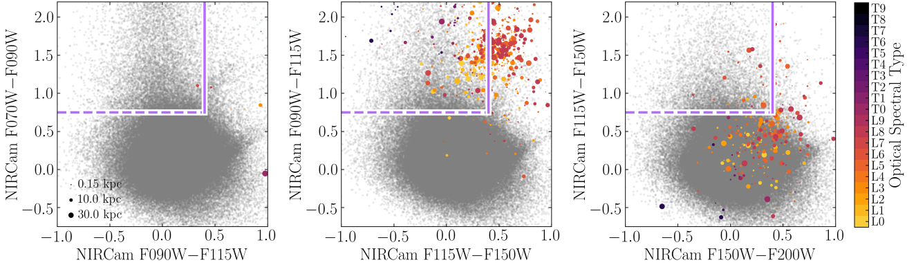
Figure 17. NIRCcam color-color plots with the mock galaxies from Figure 3 plotted with grey points, overlapped with a selection of brown dwarfs, at different simulated distances and with at the DEEP HST +NIRCcam survey depth. The points are colored by their optical spectral type, as shown on the color bar, and the sizes of the points indicate the distance from Earth, as shown in the bottom-left corner of the leftmost figure.
