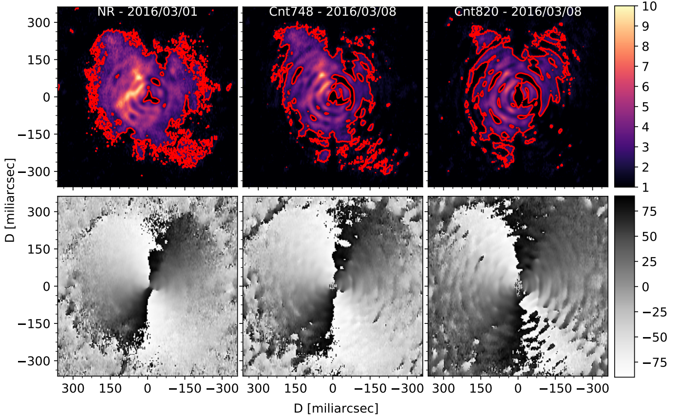
Fig. 6. Polarised light in the close environment of SW Vir in filters NR, cnt748, and cnt820. Upper panels: Colour maps showing the percentage polarisation degree observed towards SW Vir in filters NR, cnt748, and cnt820 (from left to right). The red contours show the 2% level of the polarisation degree below which instrumental polarisation can dominate. Bottom panels: Grey-scale maps showing the polarisation angle in degrees with respect to the north direction measured in filters NR, cnt748, and cnt820 (from left to right).
