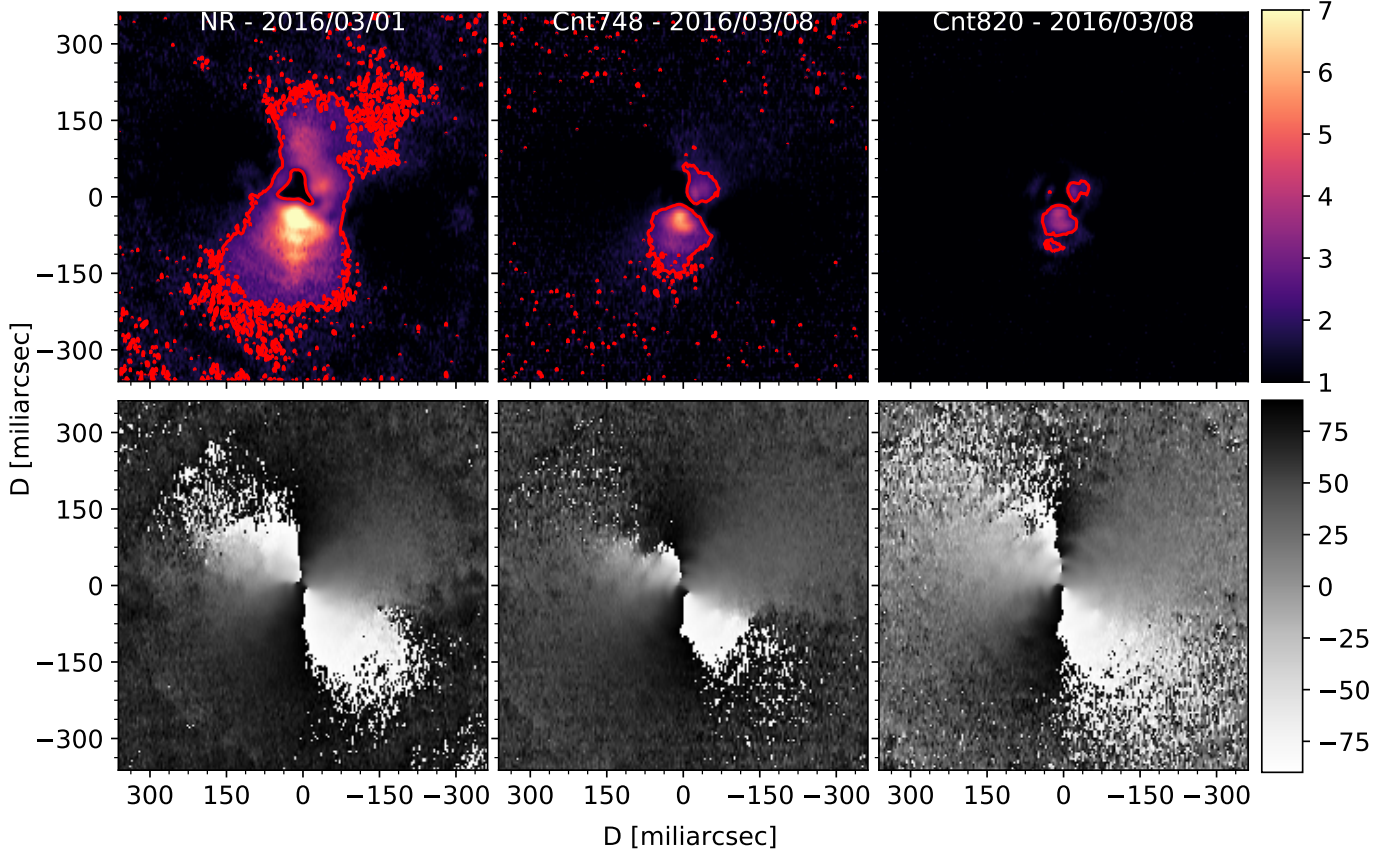
Fig. 4. Polarised light in the close environment of R Crt in filters NR, cnt748, and cnt820. Upper panels: Colour maps showing the percentage polarisation degree observed towards R Crt in filters NR, cnt748, and cnt820 (from left to right). The red contours show the 2% level of the polarisation degree below which instrumental polarisation can dominate. Bottom panels: Grey-scale maps showing the polarisation angle in degrees with respect to the north direction measured in filters NR, cnt748, and cnt820 (from left to right).
