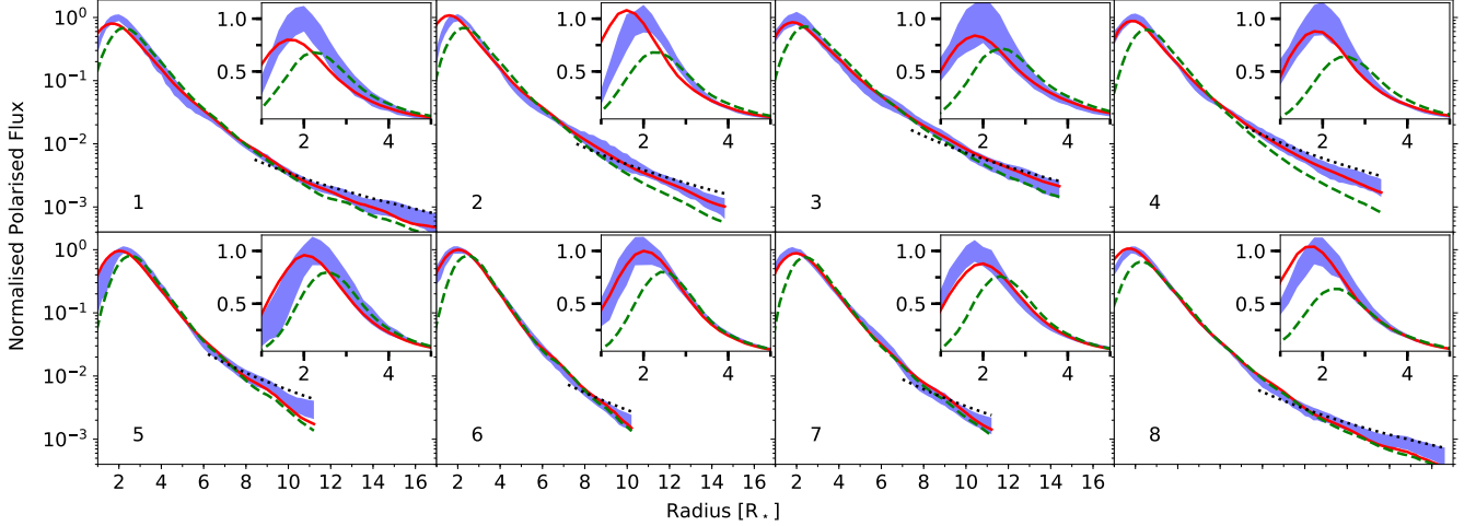
Fig. 9. Models to fit the polarised light observed towards W Hya for each of the eight octants of the image in filter cnt820. The observations with the 1\sigma error bars are shown by the shaded blue region, the full red lines show the best-fit models for each octant, the dashed green line shows the best model with a 3.45 au star, and the dotted black lines show the best-fit models with a radial power-law index n = 2 . The stellar radius assumed in this plot, R_* , is the near-infrared stellar radius measured by Woodruff et al. (2009) of 18 mas.
