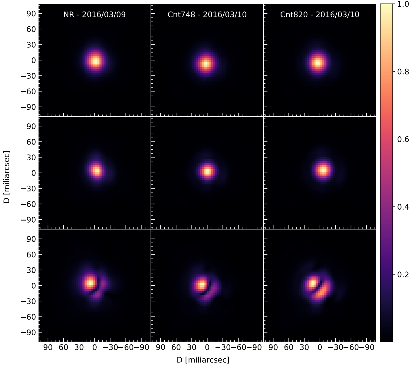
Fig. 5. ZIMPOL observations of SW Vir in filters NR, cnt748, and cnt820. Top panels: Total intensity observed towards SW Vir normalised to the peak intensity image. Middle panels: Images of the PSF-reference star \rho Vir normalised to the peak intensity in the image. Bottom panels: Polarised intensity observed towards SW Vir normalised to the peak polarised intensity in the image.
