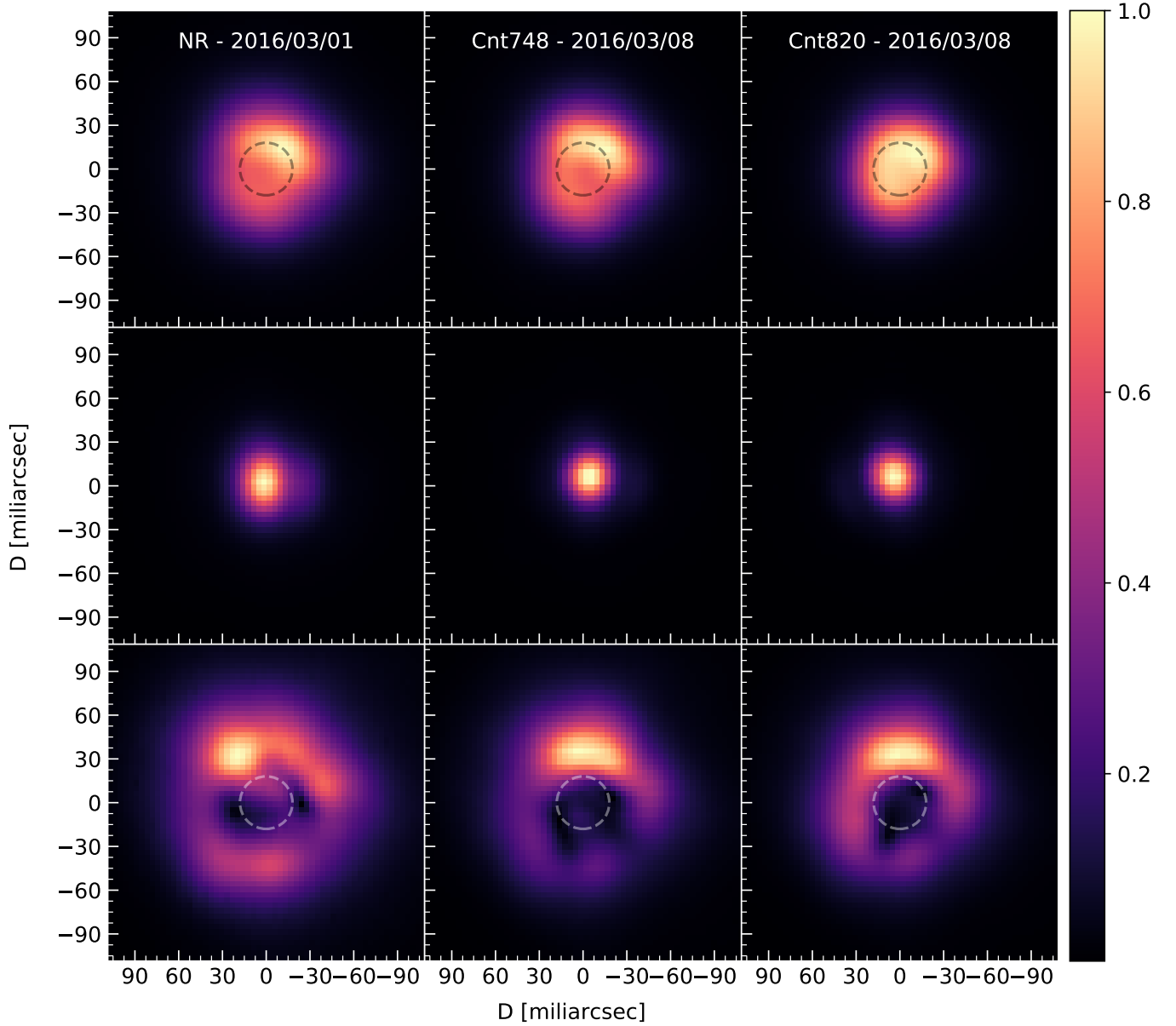
Fig. 1. ZIMPOL observations of W Hya in filters NR, cnt748, and cnt820. Top panels: Total intensity of W Hya normalised to the peak total intensity value in the image. Middle panels: Images of the PSF-reference star HD 123906 normalised to the peak polarised intensity. Bottom panels: Images of the polarised intensity of W Hya normalised to the peak polarised intensity value in the image. The dashed circles indicate the radius of 18 mas measured by Woodruff et al. (2009) in the near-infrared.
