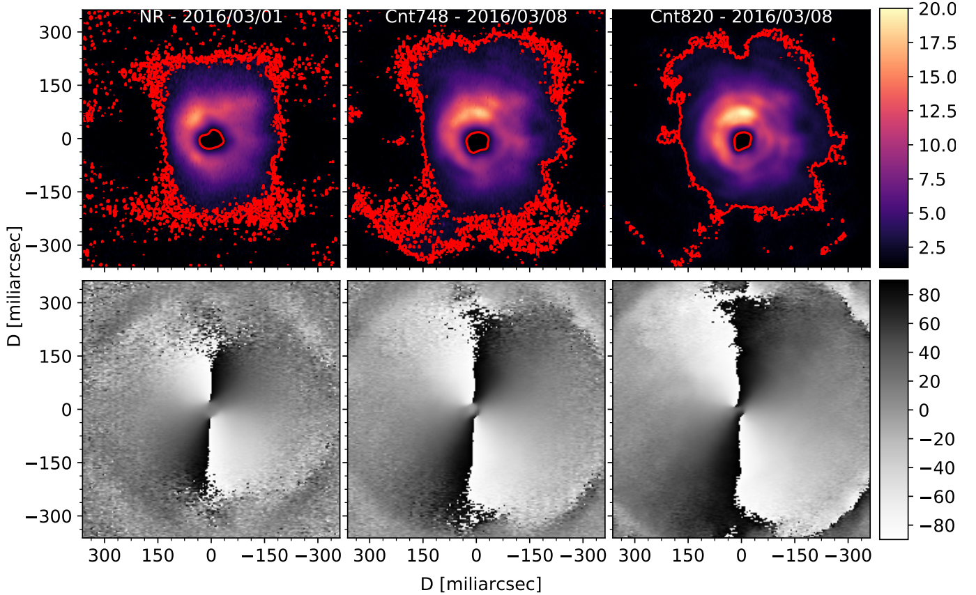
Fig. 2. Polarised light in the close environment of W Hya in filters NR, cnt748, and cnt820. Upper panels: Colour maps showing the percentage polarisation degree observed toward W Hya in filters NR, cnt748, and cnt820 (from left to right). The red contours show the 2% level of the polarisation degree below which instrumental polarisation can dominate. Bottom panels: Grey-scale maps showing the polarisation angle in degrees with respect to the north direction measured in filters NR, cnt748, and cnt820 (from left to right).
