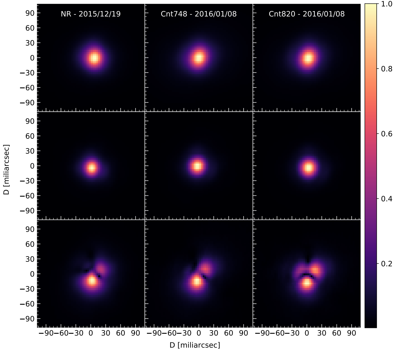
Fig. 3. ZIMPOL observations of R Crt in filters NR, cnt748, and cnt820. Top panels: Total intensity observed towards R Crt normalised to the peak intensity. Middle panels: Images of the PSF-reference star HD 96364 normalised to the peak intensity. Bottom panels: Polarised intensity observed towards R Crt normalised to the peak polarised intensity. The dark stripes seen in the centre appear in the regions where the total intensity peaks and do not correspond to physical features.
