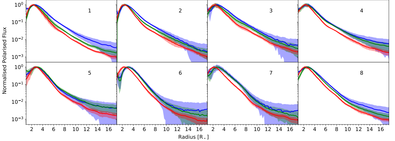
Fig. 7. Normalised radial profiles of the polarised intensity observed towards W Hya for the eight octants of the images using filters NR (blue), cnt748 (green), and cnt820 (red). The stellar radius assumed in this plot, R_* , is the near-infrared stellar radius measured by Woodruff et al. (2009) of 18 mas.
