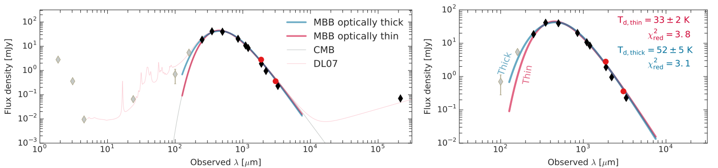
Fig. 2. Mid-IR to millimeter SED of GN20 in observed wavelength. Left: we complement our new continuum measurements at 1.86 and 3.05 \text{ mm} (red points) with existing photometry observations at observed and \lambda \leq 160 \text{ }\mu\text{m} and \lambda > 160 \text{ }\mu\text{m} (black and grey points, respectively), where the latter is omitted from the MBB modeling. Blue and red lines show the best-fit single-temperature MBB prescription assuming an optically thick ( \lambda_0 = 170 \pm 23 \text{ }\mu\text{m} ) and thin dust emission, respectively. We also present the best-fit MBB model when accounting for the effect of the CMB (grey curve). The solid pink line shows the best-fit using the DL07 dust models, containing a diffuse ISM component and dust in PDR regions. The best-fit MBB parameters are listed in Table 1. Right: A zoom-in of the rest-frame FIR part of the SED of GN20 when including the optically thick and thin MBB prescriptions. We note that the optically thick MBB model is a better match to the photometry observations at \lambda \leq 160 \text{ }\mu\text{m} .
