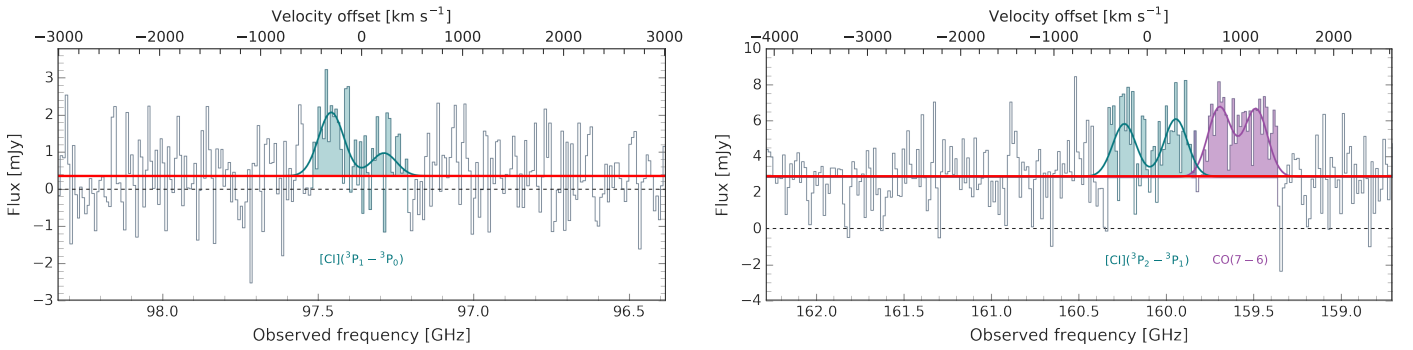
Fig. 1. Extracted spectra of the [\text{C I}](^3P_1 - ^3P_0) line (left) and the [\text{C I}](^3P_2 - ^3P_1) and \text{CO}(7-6) lines (right). Both spectra are binned in steps of 26 \text{ km s}^{-1} . The colored areas indicate that the velocity ranges corresponding to detected line emission as labeled, which were used to obtain the velocity-integrated fluxes. Blue and purple solid lines show the best-fit double Gaussians, whereas the red line in each panel shows the continuum level. The velocity offset in both panels is relative to the expected frequency of the [\text{C I}] lines at z = 4.0553 .
