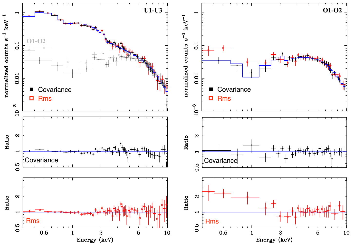
Fig. 4. Rms and covariance spectra of U1-U3 (left panels) and O1-O2 (right panels). The blue curve is the best-fit model to the covariance spectrum. Rms and covariance spectra of O1-O2 are also overplotted on those of observations U1-U3 (left panel, grey squares) for an easier comparison. The bottom panels show the ratio of rms and covariance spectra to the best-fit model of the covariance spectrum.
