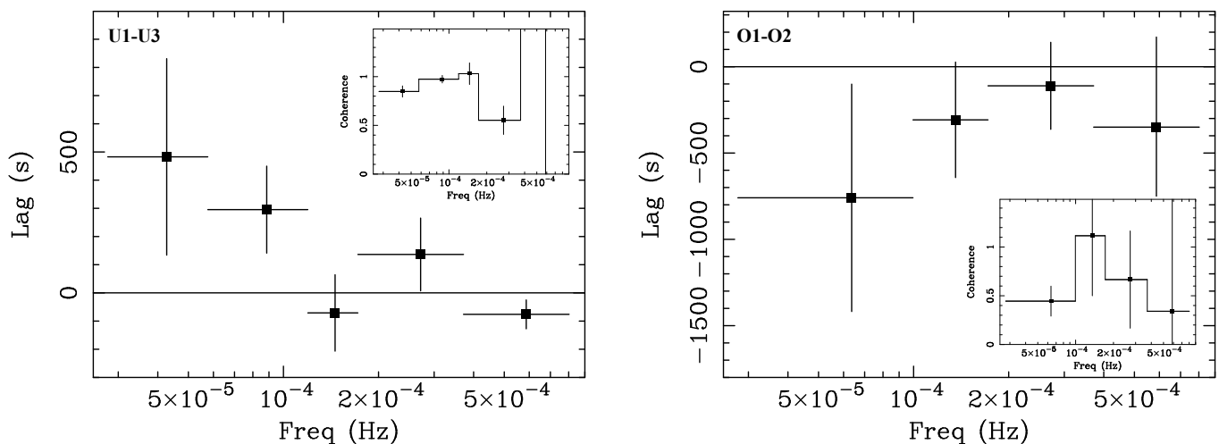
Fig. 7. The lag-frequency spectrum of observations U1-U3 (unobscured, left panel) and of O1-O2 (obscured, right panel) between the 0.5 – 2 keV and 4 – 10 keV energy bands. The insets show the intrinsic coherence as a function of frequency between the two energy bands.
