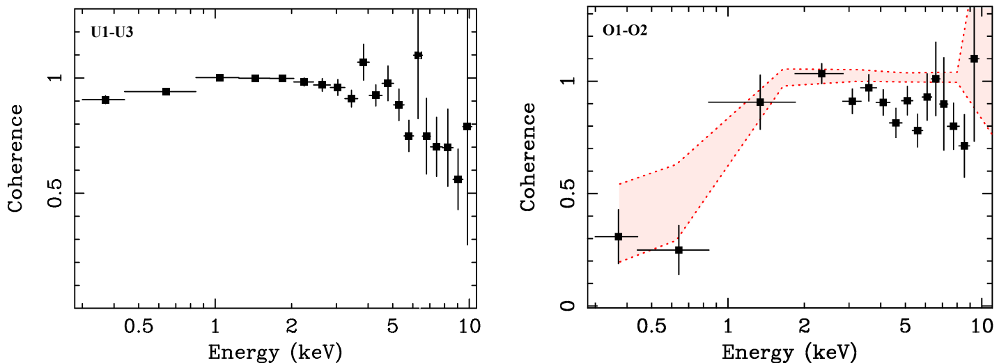
Fig. 5. Coherence as a function of energy (U1-U3 left panel; O1-O2 right panel), over the frequency range 2.78 \times 10^{-5} - 3.3 \times 10^{-4} Hz, and with the 0.3 – 10 keV band as the reference band. The red-shaded area in the right panel marks the 90% confidence level contours obtained from Cloudy simulations of an obscuring gas located at a distance of 10 light days, of electron density n_e = 2.6 \times 10^9 \text{ cm}^{-3} and \log N_{\text{H}} = 23.1 , responding to the observed variations of the ionising continuum on timescales \tau_{\text{rec}} < 1500 s. The ionisation parameter of the simulated obscuring gas varies within the range \log \xi = 1.53 - 1.82 as a consequence of short timescale variations of the ionising continuum.
