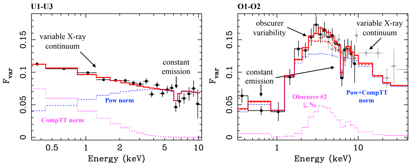
Fig. 3. F_{\text{var}} spectra of observations U1-U3 (left panel) and O1-O2 (right panel). Black squares and grey dots refer, respectively, to XMM-Newton and NuSTAR data. The blue and magenta dashed curves show F_{\text{var}} models obtained by letting different parameters (as indicated in the labels) of the continuum or of obscurer #2 vary, while the red solid curves are obtained by letting all those parameters vary simultaneously. The red dashed curve in the right panel shows the simple model obtained assuming only variations of the primary continuum and correlated variations of the ionisation parameter of obscurer #2. The main spectral features contributing to the shape of the F_{\text{var}} spectra at different energies are schematically indicated by arrows in the plots.
