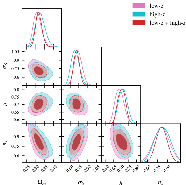
Fig. A.1. Constraints on flat \Lambda CDM derived from BOSS DR12 correlation function wedges using only the low-redshift bin (pink), only the high-redshift bin (cyan), and the joint constraints used in the main analysis (red).
