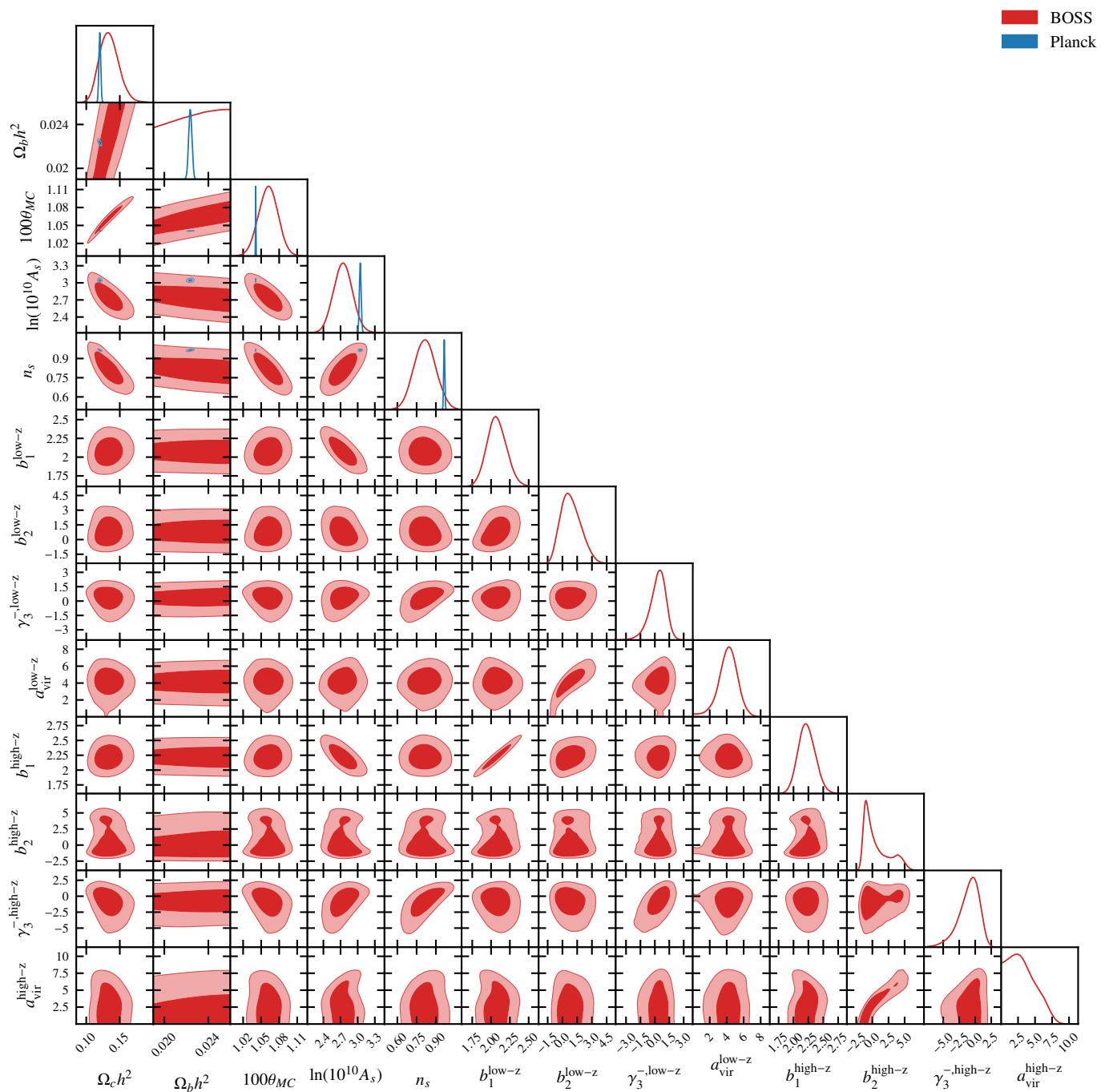
Fig. C.1. Posterior distributions for all sampled parameters in our main analysis. The posteriors derived from the BOSS clustering wedges are shown in red, while those from Planck 2018 are shown in blue.
