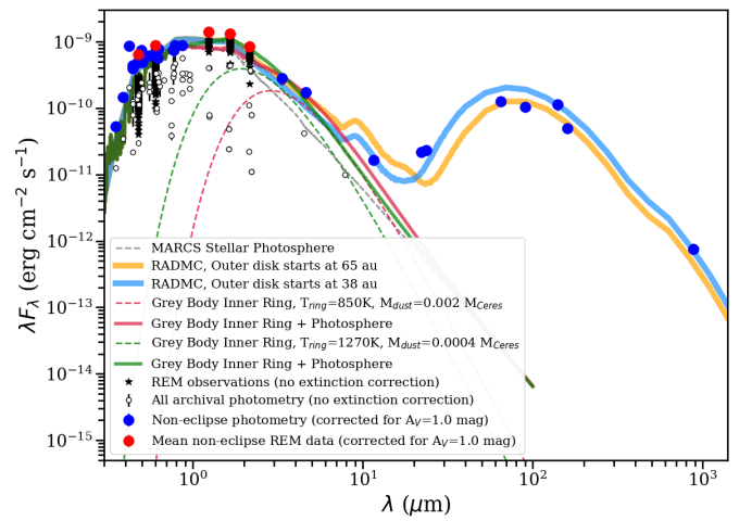
Fig. 15. SED with archival data for RX J1604.3-2130A and simple disk models. The open dots show all the available data obtained from VizieR and not corrected for extinction. The REM data are shown for the filters with negligible color terms. The blue dots show the selected brightest magnitudes for each band, dereddened by the nominal A_V=1.0 mag (Preibisch & Zinnecker 1999). Three very simple models are shown for comparison for the purpose of estimating the mass that could be associated to inner disk emission (see text for details): Two constructed using RADMC radiative transfer code, and two assume a grey body model for material located in a ring with temperature 850 K and dust mass 0.003 M_{Ceres} , and temperature 1270 K, dust mass 4e-4 M_{Ceres} , respectively.
