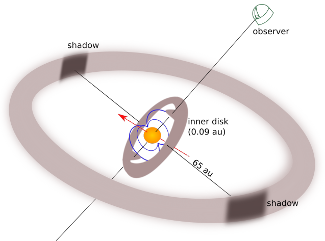
Fig. 10. Not-to-scale sketch showing the inferred structure of the system. The star and its magnetosphere are displayed in the center, the red arrow indicates the rotation axis of the star, magnetosphere, and corotating inner disk. The inner disk is deformed in the regions where the magnetosphere is joining in, which causes warps that cross our line-of-sight when the disk rotates. The outer and inner disk are highly inclined with respect to each other, so that there are always shadows along the line where the plane of the inner disk and the plane of the outer disk cross. Note that the inner disk is expected to be more wobbly and irregular than shown here.
