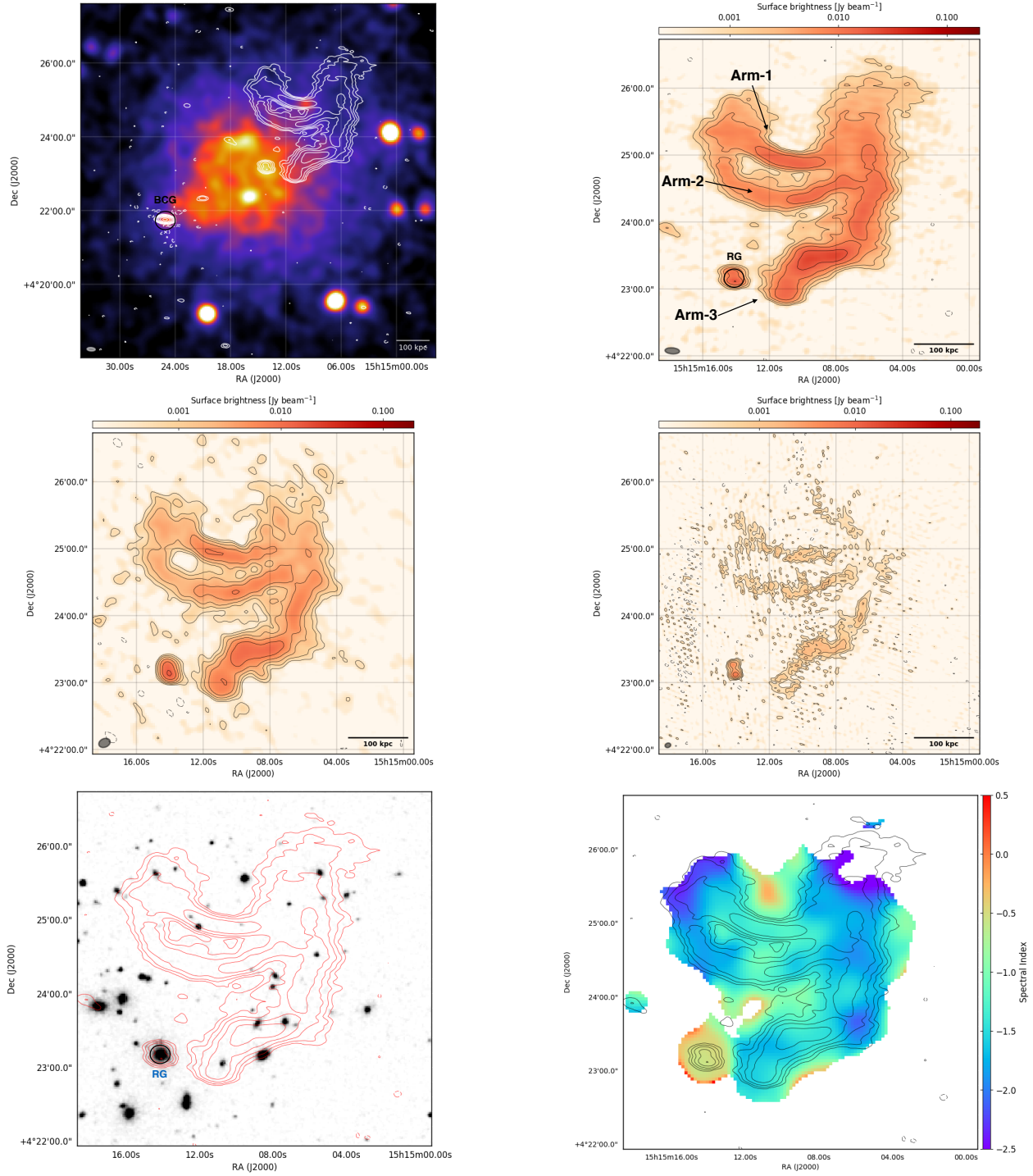
Fig. 3. Top left panel: Shows the full-resolution LOFAR image contours (white; as shown in the top right panel) of Abell 2048, overlaid on an exposure-corrected, background-subtracted XMM-Newton image in the 0.5-2.0 keV energy band with a total integration time of 68 ks. Top right panel: The 150 MHz LOFAR image ( 13'' \times 6'' ) of the source Abell 2048; where the black contours and dashed lines show the (1,2,4,\dots) \times 5 \times \sigma_{\text{LOFAR}150} and -3 \times \sigma_{\text{LOFAR}150} levels respectively, where \sigma_{\text{LOFAR}150} = 266 \mu\text{Jy/beam} . Middle left panel: The 325 MHz GMRT image ( 11'' \times 8'' ) of Abell 2048; where the black contours and dashed lines show the (1,2,4,\dots) \times 5 \times \sigma_{\text{GMRT}325} and -3 \times \sigma_{\text{GMRT}325} levels respectively, where \sigma_{\text{GMRT}325} = 125 \mu\text{Jy/beam} . Middle right panel: The 610 MHz GMRT image ( 8'' \times 5'' ) of Abell 2048 where the black contours and dashed lines show the (1,2,4,\dots) \times 5 \times \sigma_{\text{GMRT}610} and -3 \times \sigma_{\text{GMRT}610} levels respectively, where \sigma_{\text{GMRT}610} = 117 \mu\text{Jy/beam} . Bottom left panel: The LOFAR 150 MHz contours as shown in the left panel in red overlaid on an DSS2 r-band image of Abell 2048. A possible optical counterpart is marked as RG. Bottom right panel: The LOFAR 150 MHz contours as shown in the top right panel overplotted on the high resolution ( 20'' \times 20'' ) spectral index map of Abell 2048.
