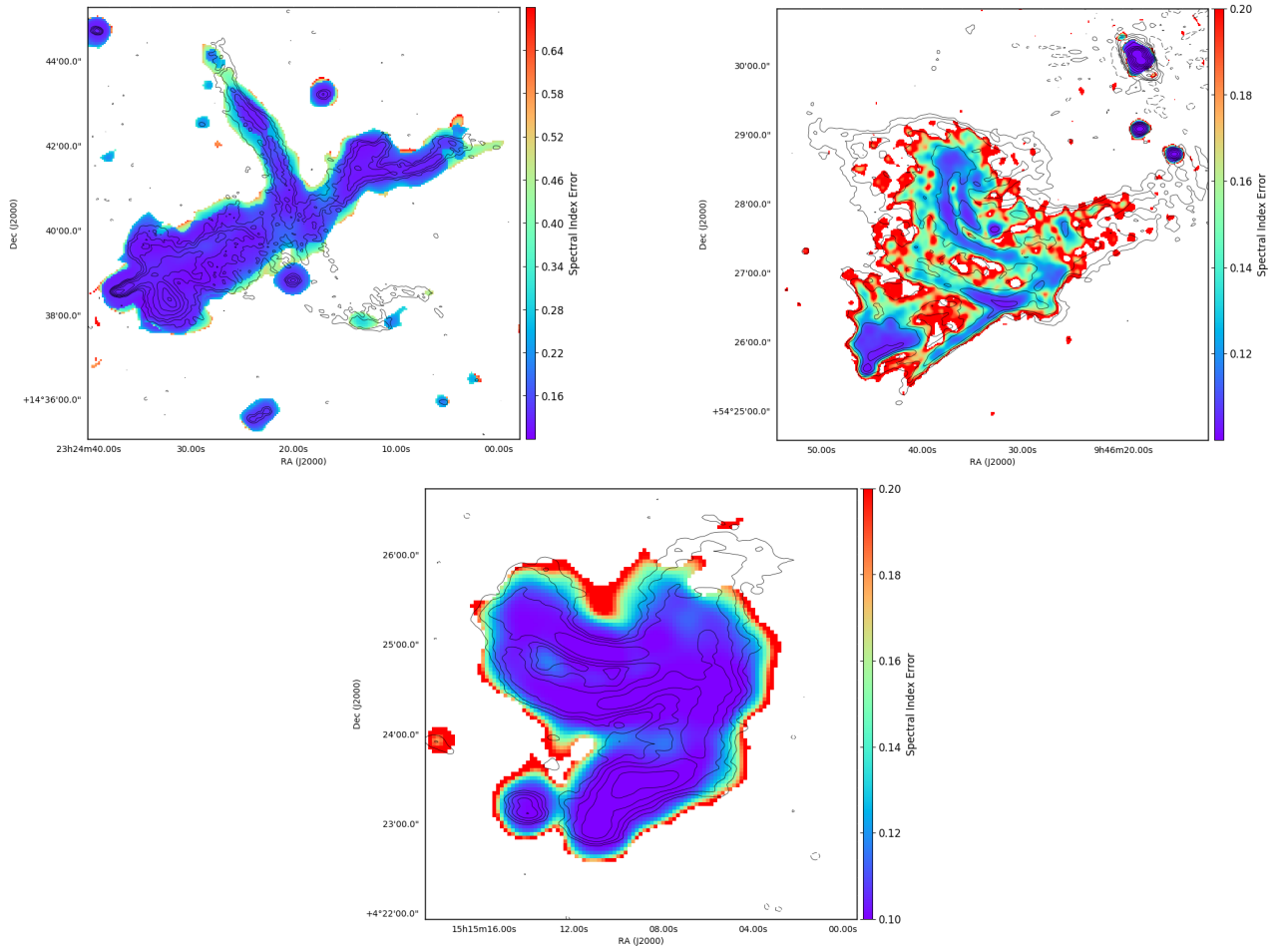
Fig. A.1. Spectral index error maps of Abell 2593, SDSS-C4-DR3-3088 and Abell 2048, respectively. The overplotted contours are same as in the LOFAR 150 MHz images for each sources.
