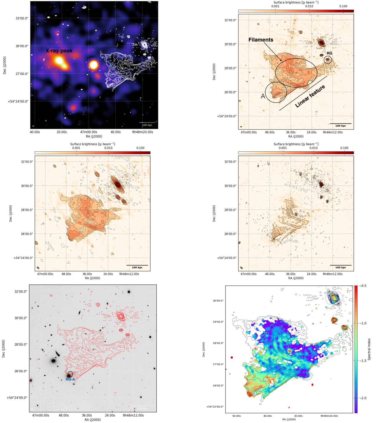
Fig. 2. Top left panel: Full-resolution LOFAR image contours (white; as shown in the right panel ) of SDSS-C4-DR3-3088, overlaid on an exposure-corrected Chandra image in the 0.5-2.0 keV energy band with a total integration time of 17ks. Top right panel: The 150 MHz LOFAR image of SDSS-C4-DR3-3088 ( 6'' \times 6'' ) where the black contours and dashed lines show the (1,2,4,\dots) \times 5 \times \sigma_{\text{LOFAR}150} and -3 \times \sigma_{\text{LOFAR}150} levels respectively, where \sigma_{\text{LOFAR}150} = 80 \mu\text{Jy/beam} . Middle left panel: The 325 MHz GMRT image ( 13'' \times 7'' ) where the black contours and dashed lines show the (1,2,4,\dots) \times 5 \times \sigma_{\text{GMRT}325} and -3 \times \sigma_{\text{GMRT}325} levels respectively, where \sigma_{\text{GMRT}325} = 43 \mu\text{Jy/beam} . Middle right panel: The 610 MHz GMRT image ( 6'' \times 4'' ) where the black contours and dashed lines show the (1,2,4,\dots) \times 5 \times \sigma_{\text{GMRT}610} and -3 \times \sigma_{\text{GMRT}610} levels respectively, where \sigma_{\text{GMRT}610} = 40 \mu\text{Jy/beam} . Bottom left panel: The LOFAR 150 MHz contours as shown in left panel in red overlaid on an SDSS r-band image of SDSS-C4-DR3-3088. Possible optical counterpart is marked as RG-A. Bottom right panel: The LOFAR 150 MHz contours as shown in the top right panel overplotted on the high resolution ( 7'' \times 7'' ) spectral index map of SDSS-C4-DR3-3088.
