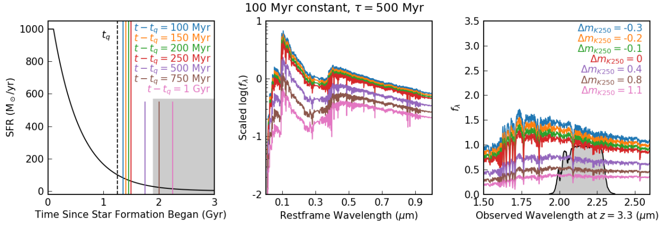
Figure E.2. The same as Figure 11 but with a SFH of 100 Myr constant followed by an exponential decline of \tau = 500 Myr. The grayed out region on the left panel indicates an age greater than that of the universe at z = 3.3 . Assuming star-formation began \sim 400 Myr after the Big Bang ( z \sim 11 ), this extreme example would have dropped below 10% of its maximum SFR at z \sim 5 .
