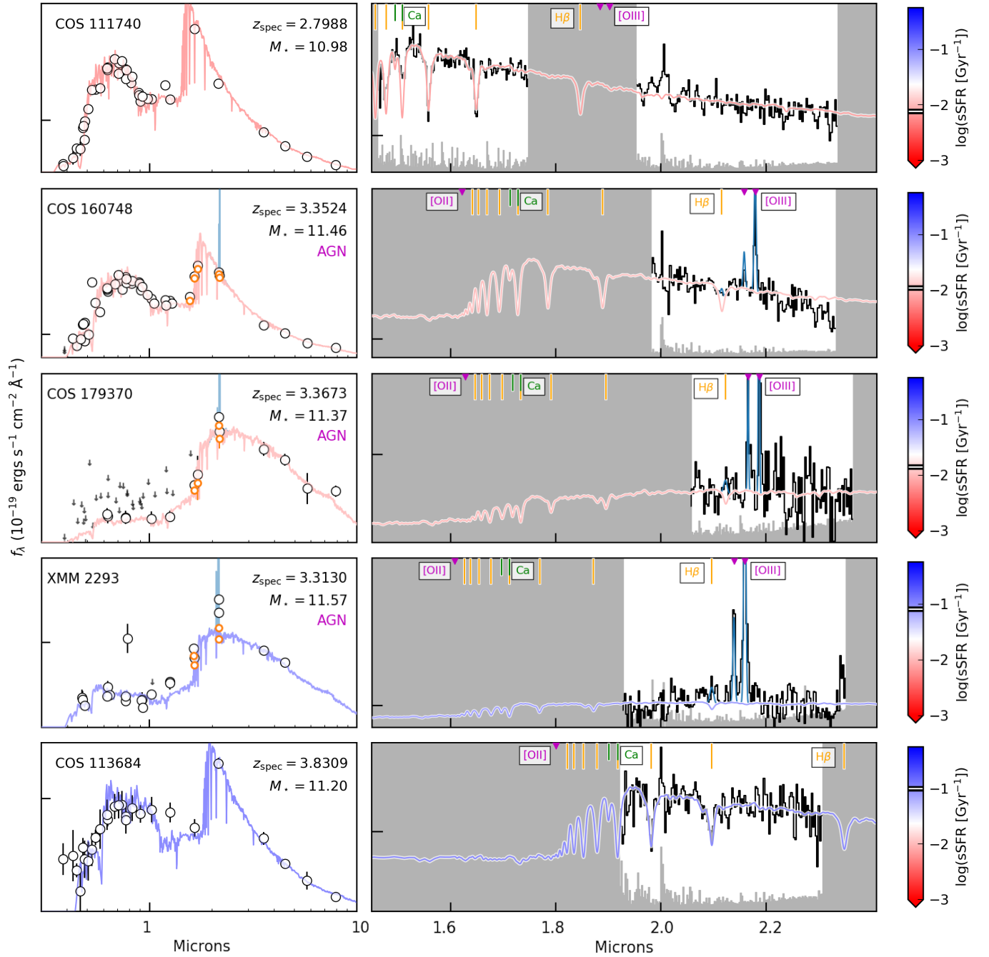
Figure 3. Same as Figure 2. For UMGs with strongly detected emission features, the best-fit model to the observed emission-lines is overlaid in teal. Orange points indicate the photometry corrected for the flux of emission lines (see Section 4.3), while photometric points with \text{SNR} < 3 are shown as downward facing arrows.
