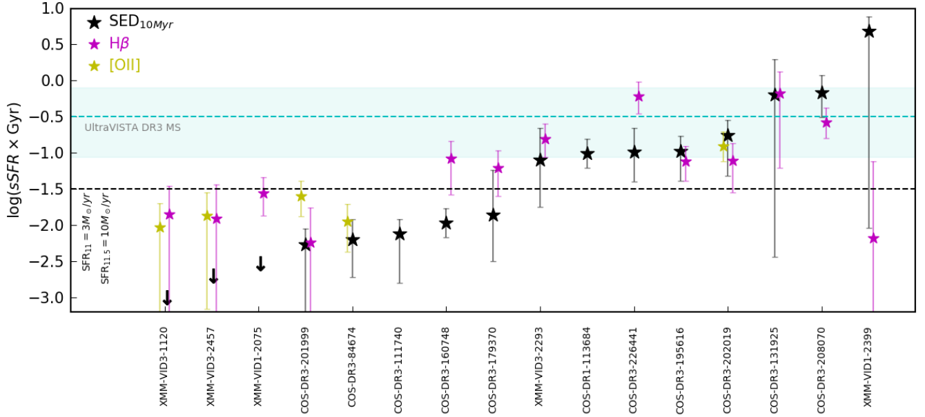
Figure 7. Comparison of sSFR for the UMGs using various star formation indicators. Black stars show the SFH from the best-fit template averaged over 10 Myr, gold stars use SFR from the [OII] line, and magenta stars use SFR from the H \beta line. Note that the H \beta value assumes all line flux is from star formation, which is not accurate for AGN hosts, and may therefore be an upper limit. The sSFR from the massive bin of the DR3 catalog plotted in Figure 6 is shown in cyan. A sSFR one dex below this value, corresponding to SFR = 3 M _{\odot} /yr for a log( M_{*}/M_{\odot} ) = 11 UMG, and SFR = 10 M _{\odot} /yr for a log( M_{*}/M_{\odot} ) = 11.5 UMG, is shown as a black dashed line.
