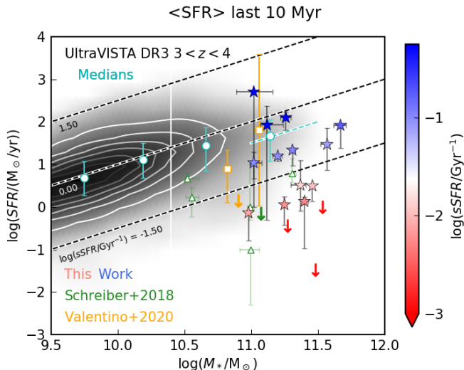
Figure 6. The SFR-stellar mass plane. UMGs are shown as stars with the same color scheme as in previous figures. The population of galaxies at 3 < z < 4 in the UltraVISTA DR3 catalog are shown in black, with the stellar mass completeness limit of the catalog as a white vertical line and medians in bins of 0.5 dex in stellar mass also shown in cyan. The highest mass bin average corresponds to \log(sSFR/Gyr^{-1}) \sim -0.5 , which is represented by a dashed cyan line spanning the width of the bin. Massive z > 3 galaxies from Schreiber et al. (2018a) and Valentino et al. (2020) are shown in green and orange, respectively.
