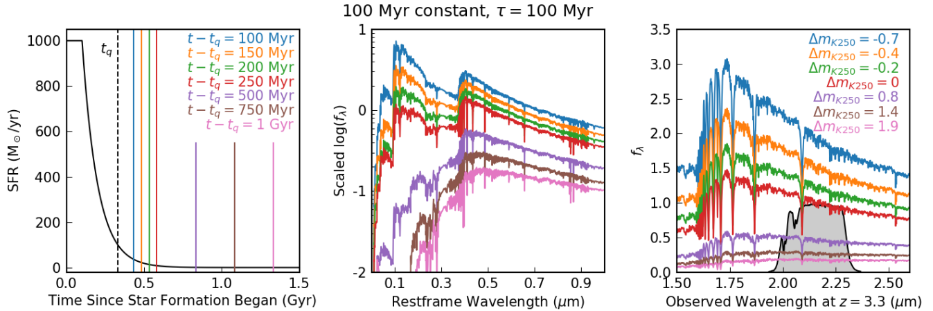
Figure 11. The evolution of K_s -band magnitude for an object with a 100 Myr of constant star formation followed by an exponential decline parameterised by \tau = 100 Myr. Left: The SFH (black) used to construct the SEDs at various times (solid, colored lines). The vertical dashed line represents the nominal quenching time, t_q , taken to be when the SFR drops below 10% that of the main starburst period. Center: The resultant SEDs at each timestep, corresponding to 100, 150, 200, 250, 500, 750, and 1000 Myr after the quenching time, and scaled relative to the t - t_q = 250 Myr SED (red). Right: The SEDs redshifted to z = 3.3 . The gray curve corresponds to the K_s -band response function, and magnitude differences are given relative to the t - t_q = 250 Myr SED (red).
