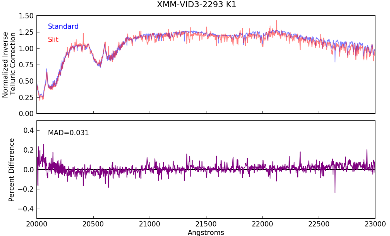
Figure D.1. Top: Comparison of the telluric correction derived using stars on science slits (red) to the telluric corrections derived using a standard star (blue) observed directly after the mask. Bottom: The percent difference between the two corrections as a function of wavelength. The median absolute deviation is given as well.
