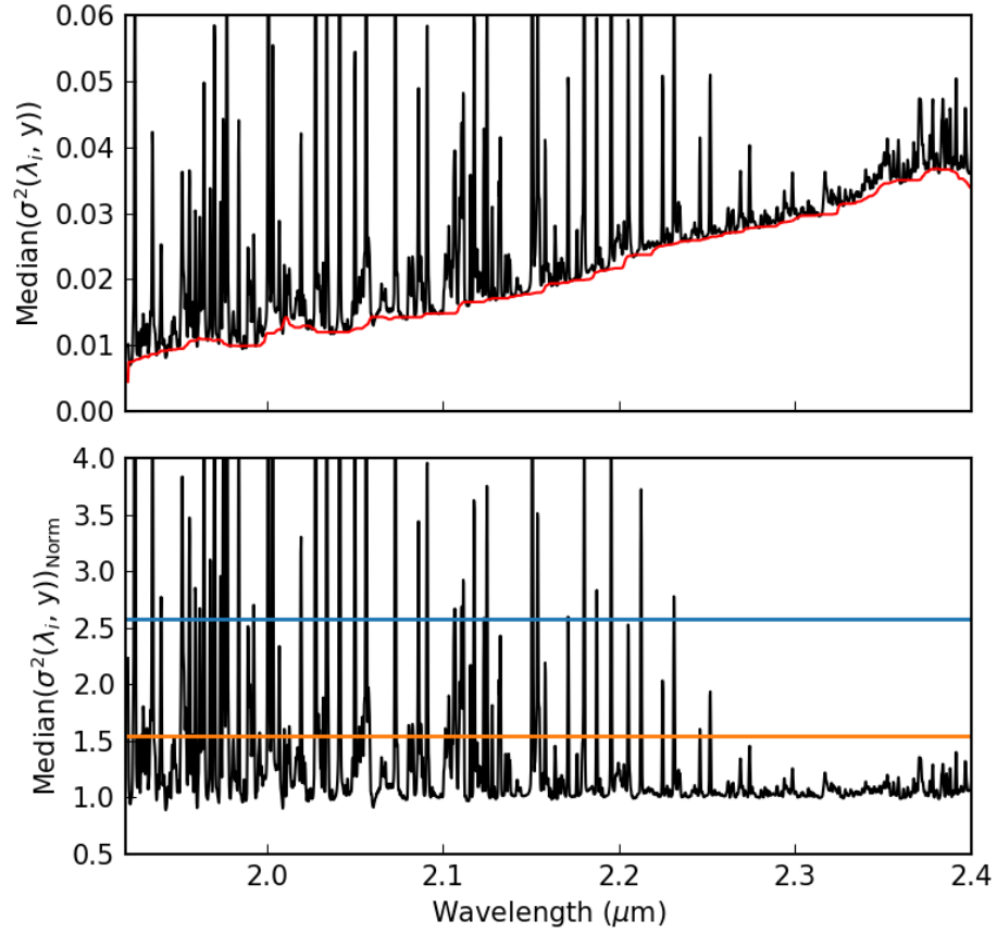
Figure C.2. Top: The median variance per pixel across wavelengths for a sample K -band mask (black). The value over which we normalize is shown in red. Bottom: The normalized variance per wavelength (black) as well as the thresholds for weak (orange) and strong (blue) sky line contamination.
