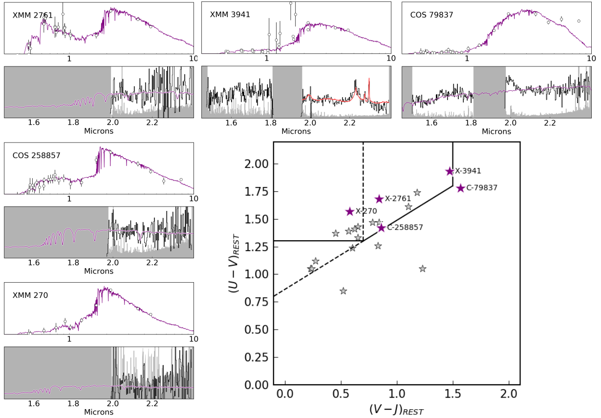
Figure B.1. Central panel: The restframe UVJ -diagram showing the location of the five unconfirmed objects (purple) relative to the 16 confirmed UMGs (gray). Surrounding panels: The photometry (top) and spectroscopy (bottom) for each object, shown with the best-fit template in purple. For XMM-VID3-3941, the SDSS composite quasar template (Vanden Berk et al. 2001) redshifted to z = 3.59 is shown in red.
