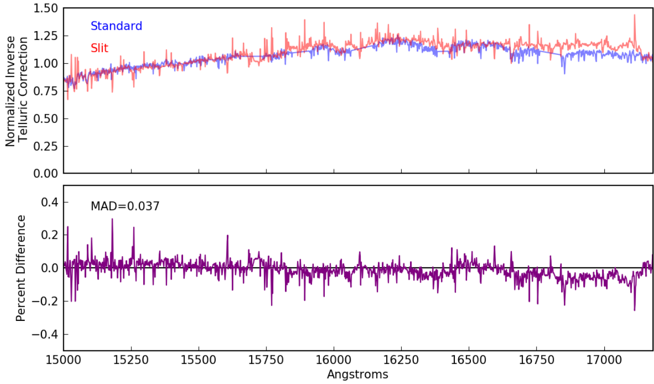
Figure D.2. Same as Figure D.1 but for a mask which had two hours between observations of the mask and the standard star.
