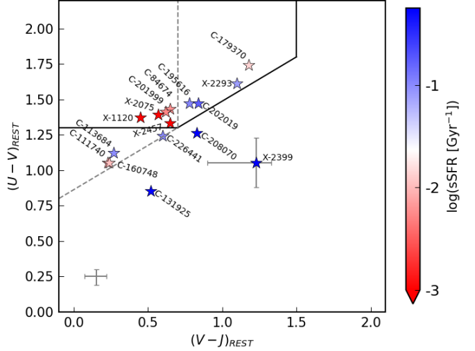
Figure 5. The restframe UVJ diagram for all confirmed UMGs, colored by sSFR averaged over the last 10 Myr based on the best-fit SFH. The median error bar is shown in the lower left, and the only UMG with an error bar twice this size has the error plotted on the point.
