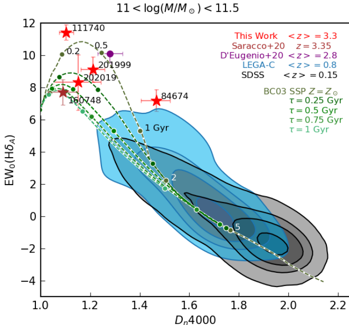
Figure 8. The EW_0(H\delta)-D_n(4000) plane, used to constrain age. Lower redshift samples from SDSS and LEGA-C, presented in (Wu et al. 2018), are shown in black and blue, respectively. A stack of 9 galaxies from D’Eugenio et al. (2020) is shown in purple. The UMGs with spectroscopic coverage of both features are shown in red, while COS-160748, presented in Saracco et al. (2020, submitted), is shown in brown. Stellar evolution tracks for a simple stellar population (SSP) and exponentially-declining SFH with varying \tau are shown in shades of green. Ages of 0.2, 0.5, 1, 2, and 5 Gyr are marked with a circle for each track.
