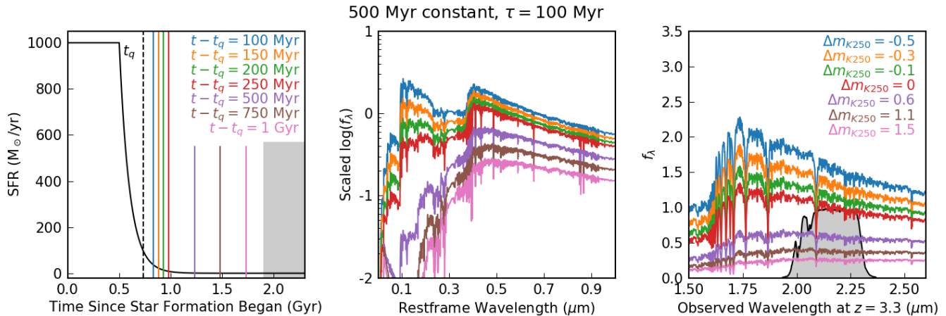
Figure E.1. The same as Figure 11 but with a SFH of 500 Myr constant followed by an exponential decline of \tau = 100 Myr. The grayed out region on the left panel indicates an age greater than that of the universe at z = 3.3 .
