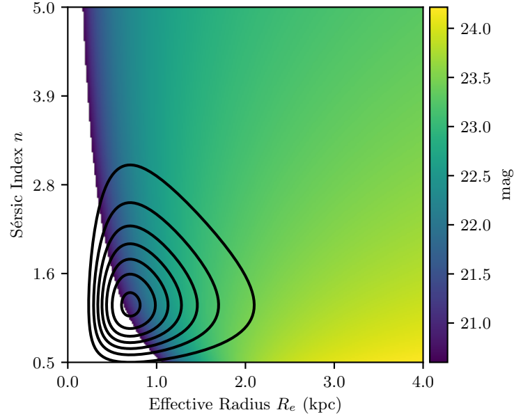
Figure 13. The J-band magnitude of the host galaxy of NDWFS-J1425+3254, as an example, assuming a Sérsic profile with Sérsic index n and effective radius R_e that is constrained to have the measured flux (a 2\sigma noise limit) in the annulus 0''.42\text{--}0''.60 . We show a range of Sérsic profiles, with n \in (0.5, 5) and R_e \in (0, 4) kpc. The white regions show galaxies with magnitudes brighter than the quasar itself (here m_J < 20.6 ), which we exclude. The black contours show the 2D probability distribution functions for n and R_e , guided by the observations of z \simeq 6 bright ( 1\text{--}10L_{z=3}^* ), massive galaxies by Shibuya et al. (2015), assuming the parameters are independent. Using a Monte Carlo technique to sample magnitudes from this distribution gives a magnitude probability distribution function, from which we choose the most likely value as the corresponding magnitude limit, in this case m_J > 22.8 mag.
