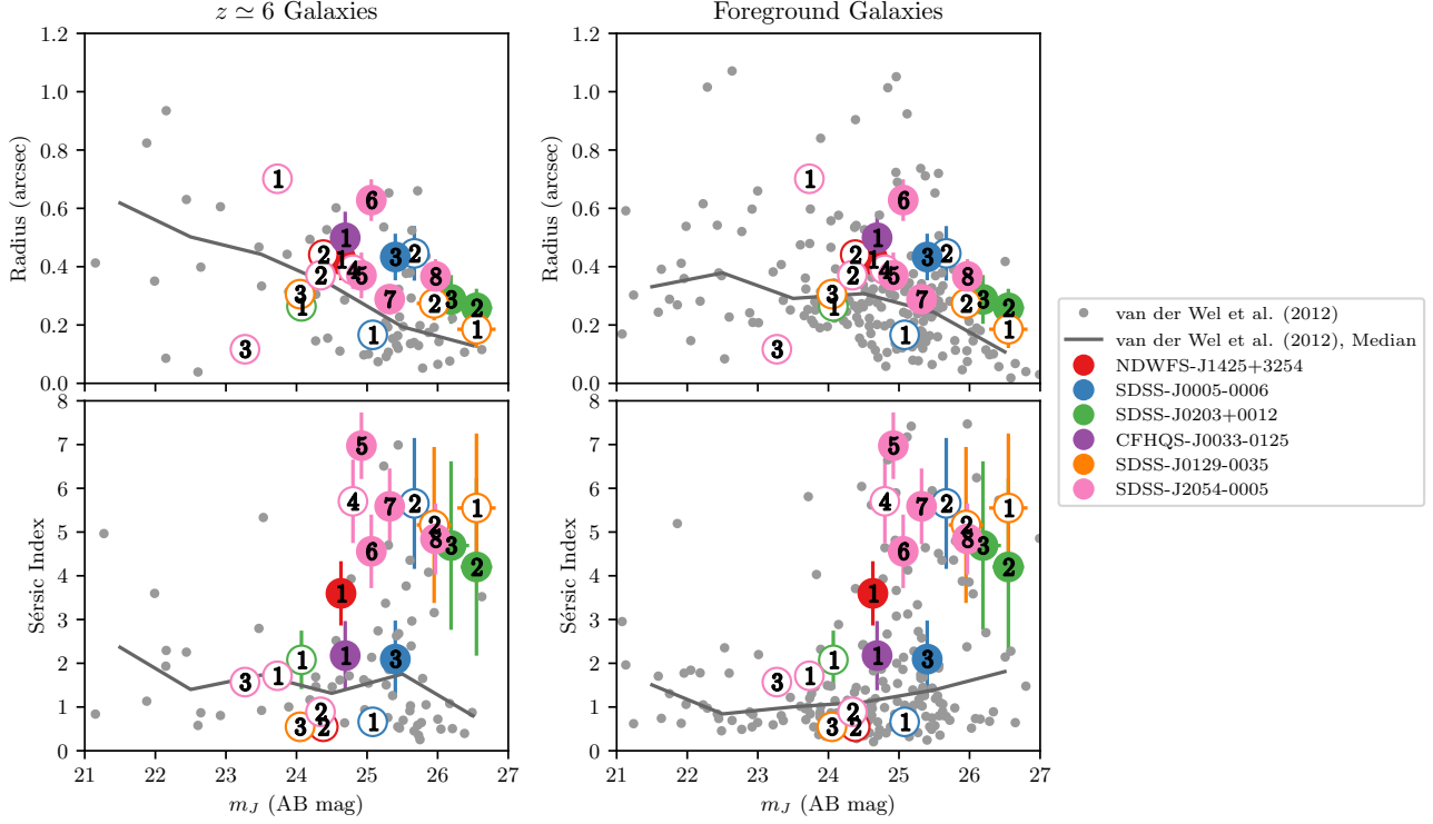
Figure 8. The morphological properties measured for each of the galaxies within 3'' of our 6 quasars. Top row: effective radius R_e vs. J-band magnitude. Bottom row: Sérsic index n vs. J-band magnitude. Filled colored circles show those with colors and magnitudes consistent with z \simeq 6 galaxies, while open colored circles show candidates which are likely to be foreground interlopers given their colors and magnitudes. The numerical labels correspond to labels in the individual quasar images (Figures 2-4), and Table 3, for ease of comparison. Also shown are measurements of galaxy sizes in the CANDELS GOODS-South survey from van der Wel et al. (2012), for comparison. Left panel: van der Wel et al. (2012) galaxies with best estimate redshift z > 5.5 , and a 95 per cent confidence that z > 5 . Right panel: Galaxies within 3'' of these z > 5.5 galaxies, at any redshift. Grey dots show individual galaxies, and the grey line shows the median in bins of 1 magnitude.
