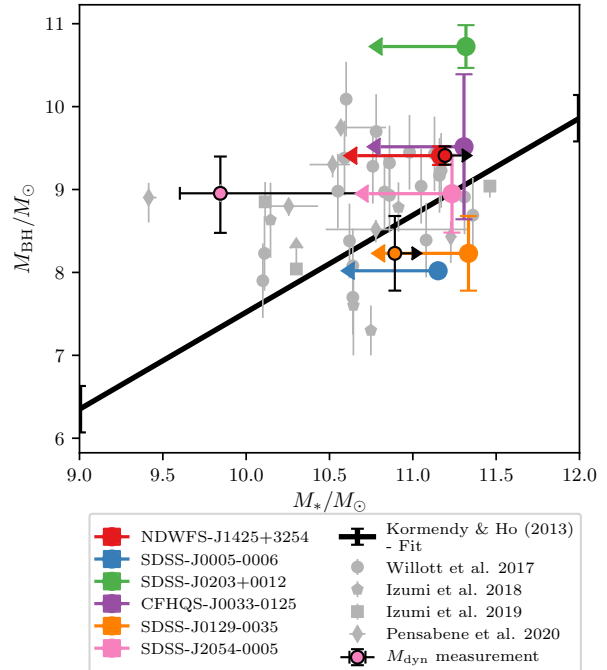
Figure 6. The black hole–stellar mass relation for our z \simeq 6 quasar host galaxies, alongside other z \simeq 6 quasars from the literature (Willott et al. 2017; Izumi et al. 2018, 2019; Pensabene et al. 2020). Existing dynamical mass measurements/limits are shown with black errorbars, for NDWFS J1425+3254 (red; Wang et al. 2010), SDSS J2054-0005 (pink; Pensabene et al. 2020) and SDSS J0129-0035 (orange; Pensabene et al. 2020). Also shown is the z=0 relation of Kormendy & Ho (2013), for comparison.
