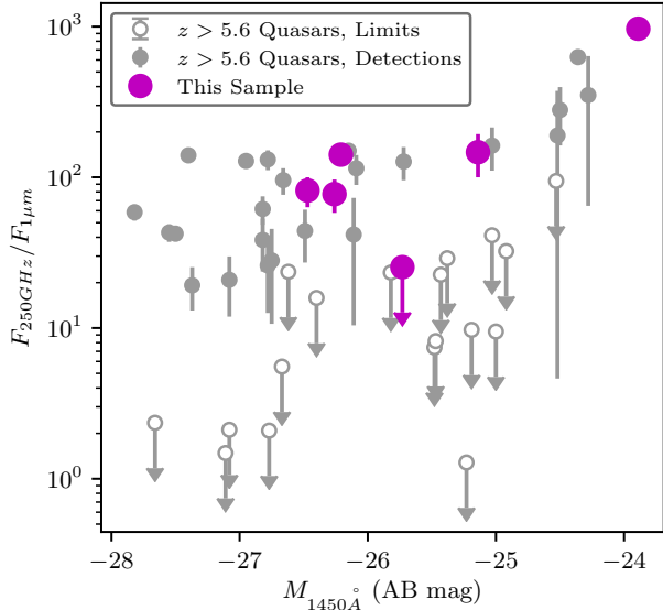
Figure 1. Selection of ultraviolet-faint, far infrared-luminous quasars based on absolute magnitude (rest-frame 1450Å) and observed sub-mm to near-infrared flux ratio. Our sample of six quasars is denoted by magenta circles, with detections for the five IR-luminous quasars, and an upper limit for the additional quasar SDSS J0005-0006. Other z > 5.6 quasars with sub-mm observations are plotted in gray (Fan et al. 2000, 2001, 2003, 2004, 2006b; Petric et al. 2003; Bertoldi et al. 2003; Mahabal et al. 2005; Cool et al. 2006; McGreer et al. 2006; Goto 2006; Venemans et al. 2007, 2013; Wang et al. 2007, 2008, 2011, 2013; Kurk et al. 2007, 2009; Willott et al. 2007, 2010a,b; Jiang et al. 2007b, 2008, 2009; Mortlock et al. 2009, 2011; Zeimann et al. 2011; De Rosa et al. 2011, 2014; Omont et al. 2013; Bañados et al. 2014; Wu et al. 2015).
