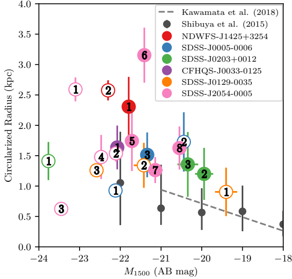
Figure 9. The circularized effective radius R_e \sqrt{b/a} vs. 1500 \text{ \AA} absolute magnitude measured for each of the galaxies within 3'' of our 6 quasars, assuming they are at the same redshift as the quasar. Filled colored circles show those with colors and magnitudes consistent with z \sim 6 galaxies, while open colored circles show candidates which are likely to be foreground interlopers given their colors and magnitudes. The numerical labels correspond to labels in the individual quasar images (Figures 2-4), and Table 3, for ease of comparison. The size–luminosity relations from the high-redshift observations of Shibuya et al. (2015) and Kawamata et al. (2018) are also shown, for comparison.
