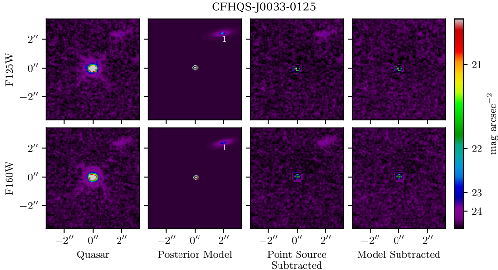
Figure 2. Posterior-weighted model images for CFHQS J0033–0125. All images show a \approx 6''.5 \times 6''.5 FOV around the quasar, in order to see any companion galaxies, and are displayed with the same arcsinh color stretch and 0''.060 pixel scale. Top row: F125W filter. Bottom row: F160W filter. First column: drizzled, undistorted WFC3 images. Second column: posterior-weighted models from the MCMC fitting process, before convolution with the PSF. Third column: residual after subtracting only the point source model from the original image. Fourth column: residual after subtracting the point source model and all modeled companions from the original image. Any galaxies surrounding the quasar are indicated with a white number, for ease of comparison with Figs. 7 and 9 and Table 3.
