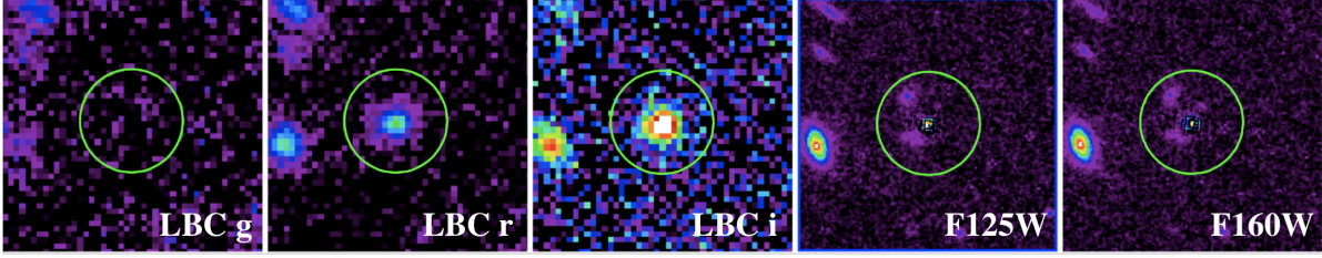
Figure 11. Thumbnail images of NDWFS-J1425+3254. From left to right: LBT/LBC g -, r -, and i -bands, and HST WFC3 IR J- and H-bands. The companion galaxies are visible within the green circle of radius 2''0 in the point source-subtracted WFC3 IR images. Lyman- \alpha emission from the quasar at \simeq 8330\text{\AA} is captured by the i -band image, while Lyman-Werner flux from the quasar is bright enough to be seen in the r -band, even in these LBT observations (see the discovery spectrum of Cool et al. 2006). Due to the seeing of the ground-based images, estimated as \simeq 0''.8 - 1''.0 FWHM, point source subtraction on the r -band LBC image produces an inconclusive upper limit for the combined companion galaxy flux.
