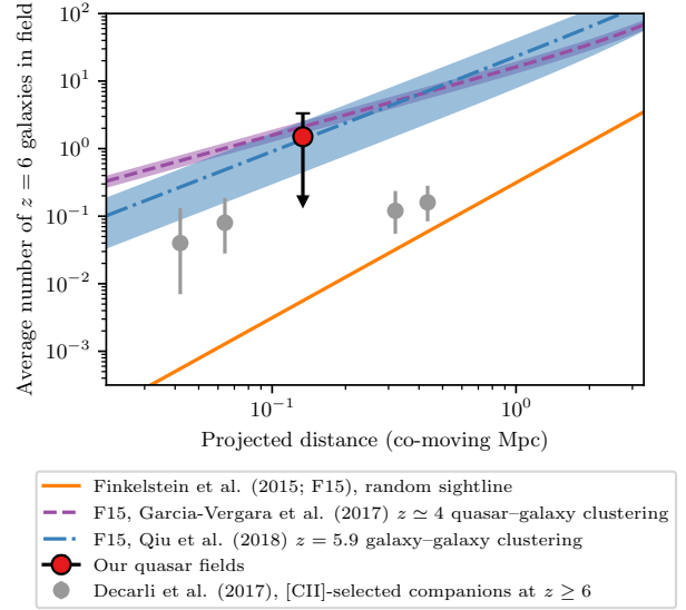
Figure 10. The average number of potential z \simeq 6 companion galaxies found within 3''.2 ( 0.13 \text{ cMpc} ) of our six quasars, compared with expectations for counts of z = 6 galaxies in random fields from the Finkelstein et al. (2015) luminosity function, as a function of projected distance from the quasar. We consider a cylindrical volume centred on the quasar with depth \Delta z = 1 . Errors on our observation show the range of 1–20 true z \simeq 6 companions, around our best estimate of 9, where 20 is the total number of objects found within 3''.2 of our six quasars; the lower error is marked with an arrow to account for the (unlikely) limiting case that none of the neighboring galaxies are true z \simeq 6 companions. Also shown are the observations of z \geq 6 quasar companions of Decarli et al. (2017), for comparison. We also plot the Finkelstein et al. (2015) luminosity function predictions modified to account for the effect of large-scale clustering. We take two models for the excess in the galaxy number density \xi(r) = (r_0/r)^\gamma , with r_0 = 8.83^{+1.39}_{-1.51} h^{-1} \text{ cMpc} and \gamma = 2.0 from the quasar–Lyman break galaxy clustering of z = 4 galaxies measured by García-Vergara et al. (2017), and r_0 = 5.3^{+2.3}_{-2.8} h^{-1} \text{ cMpc} and \gamma = 1.6 from the galaxy–galaxy clustering measurements of z = 5.9 M_{UV} < -19.99 galaxies (Qiu et al. 2018).
