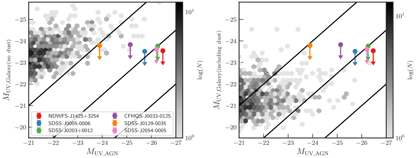
Figure 12. The relation between quasar and host galaxy UV-luminosity for our sample (colored upper limits; see legend) and for the simulated z=7 quasars from the BlueTides simulation (grey density plots). The left panel shows the BlueTides host galaxies' intrinsic UV-luminosities, while the right panel shows them after dust attenuation, which is calculated using the density of gas in the simulation (see Ni et al. 2019; Marshall et al. 2019). Diagonal black lines show where the ratio of quasar to host brightness is 1:1, 10:1 and 100:1.
