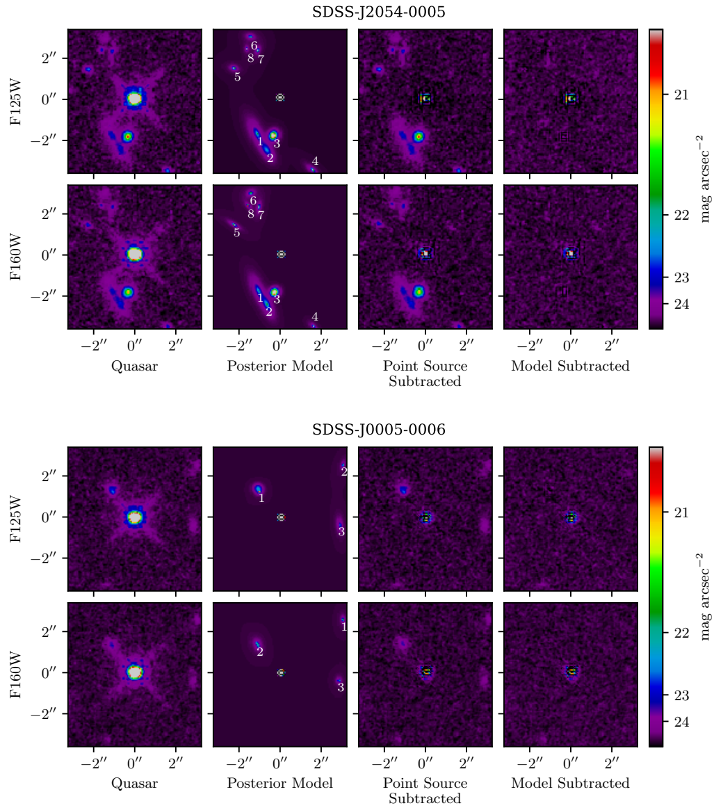
Figure 4. Posterior-weighted model images for SDSS J2054-0005 and SDSS J0005-0006. See Figure 2 for details.
