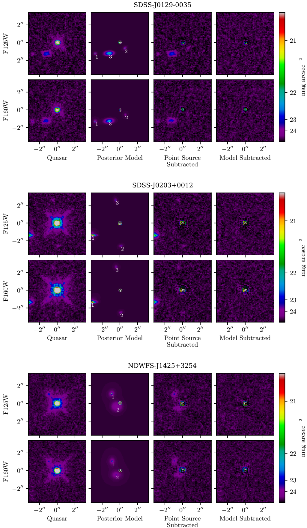
Figure 3. Posterior-weighted model images for SDSS J0129–0035, SDSS J0203+0012 and NDWFS J1425+3254. See Figure 2 for details.
