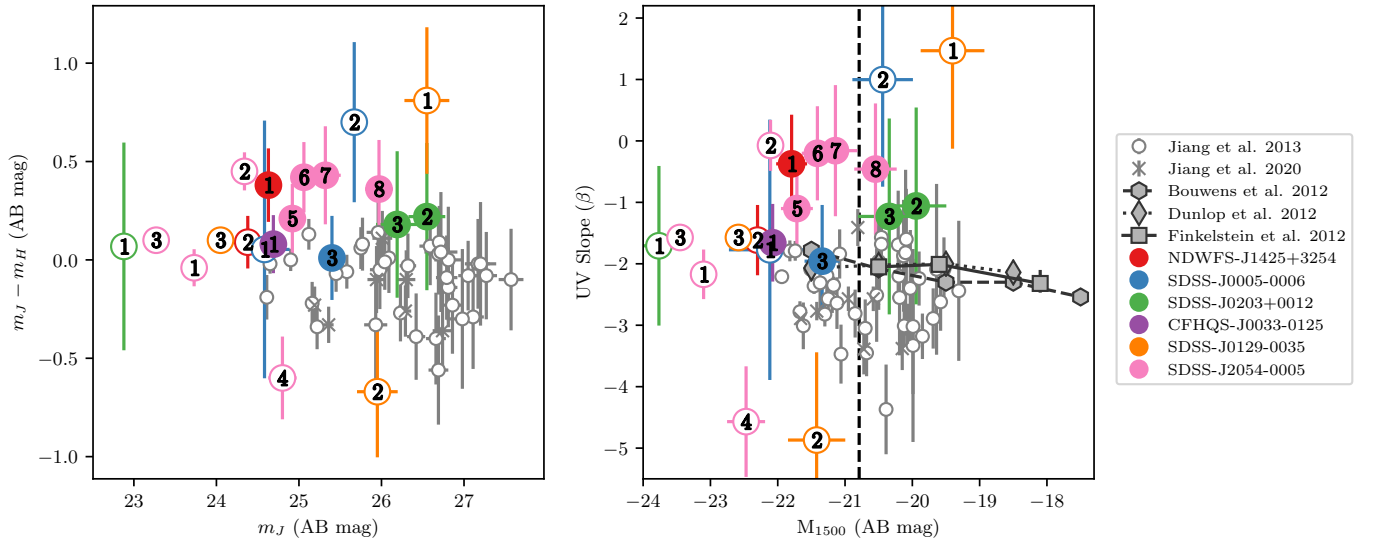
Figure 7. Left: J-H color vs. J-band magnitude and Right: Rest-frame UV slope \beta vs. 1500 Å absolute magnitude, measured for each of the galaxies within \simeq 3'' of our six quasars, assuming they are at the same redshift as the quasar. Filled colored circles show those with colors and magnitudes consistent with z \sim 6 galaxies, while open colored circles show candidates which are likely to be foreground interlopers given their colors and magnitudes. The numerical labels correspond to labels in the individual quasar images (Figures 2-4), and Table 3, for ease of comparison. Grey symbols represent spectroscopically-confirmed z \simeq 6 galaxies from Jiang et al. (2013, 2020) and the average relations for dropout-selected LBGs from Bouwens et al. (2012), Dunlop et al. (2012), and Finkelstein et al. (2012) (see legend). The dashed black line shows the value of M^* (Finkelstein 2016).
