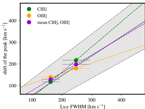
Fig. 5. Correlations between the shift of the Ly \alpha peak and the Ly \alpha FWHM obtained from the Ly \alpha FWHM subsamples of our LAEs. These correlations have been obtained considering the rest-wavelengths of C III] (green line) and O III] (orange line) as reference wavelengths and their mean shift (purple line). In gray, Eq. 2 of V18, obtained from object-by-object measurements, and the associated scatter (gray shaded area).
