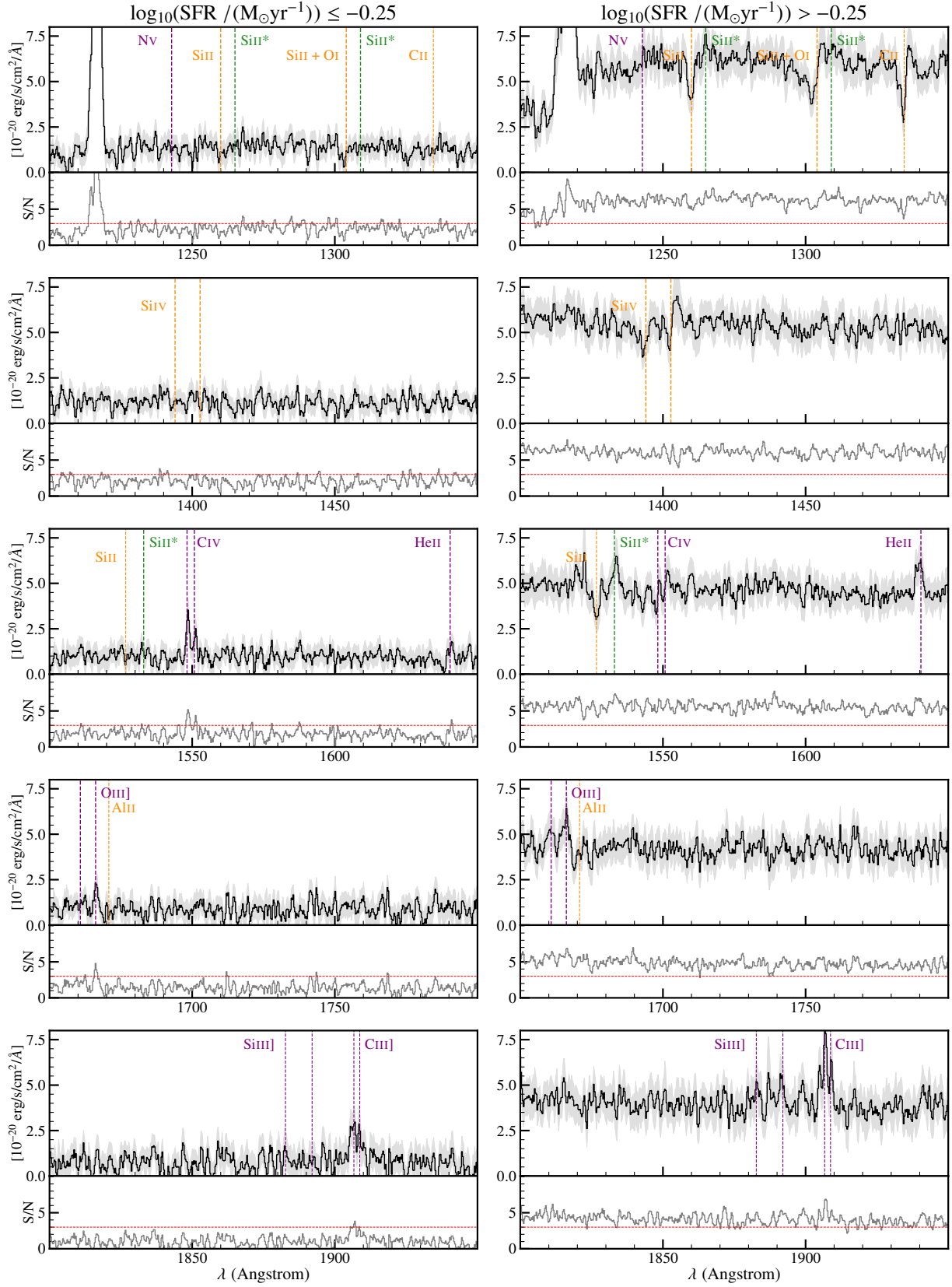
Fig. A.8. Mean spectra of LAEs with \log_{10}(\text{SFR} / (\text{M}_{\odot} \text{yr}^{-1})) \leq -0.25 and > -0.25 (left and right, respectively). The median values of \log_{10}(\text{SFR} / (\text{M}_{\odot} \text{yr}^{-1})) for the two subsamples are -0.57 and 0.16 , respectively. Lines and symbols as in Fig. 4.
