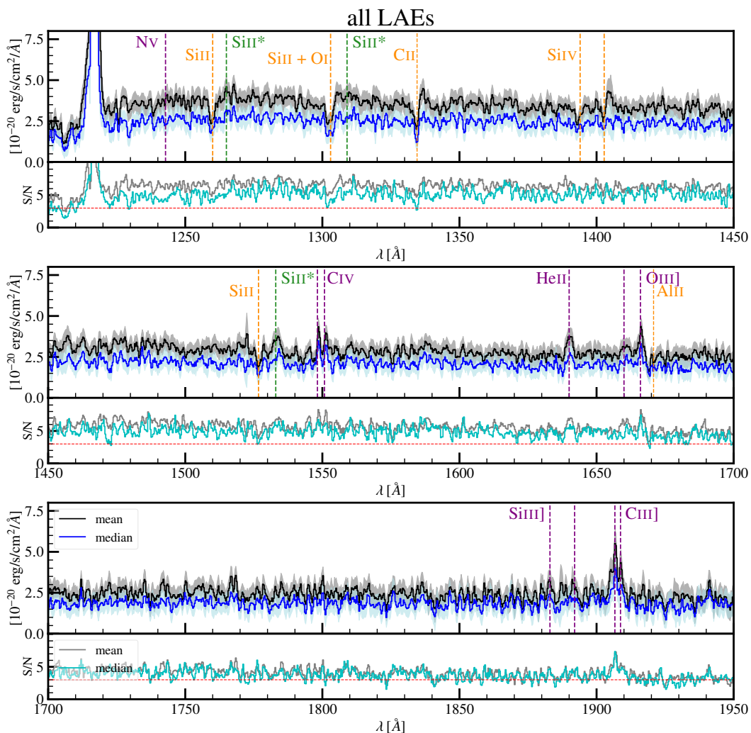
Fig. 3. Mean and median spectra of all the 220 LAEs described in Sect. 2.1 shown in black and blue with the error displayed with the gray and light-blue shaded areas, respectively. The vertical lines indicate the rest-frame wavelengths of some of the main spectral features: nebular emission lines (purple), ISM absorption (orange) and fine-structure transitions (green). The bottom panels show the S/N per pixel (gray and cyan curves for mean and median spectra, respectively) with the dotted red horizontal line indicating S/N = 3 .
