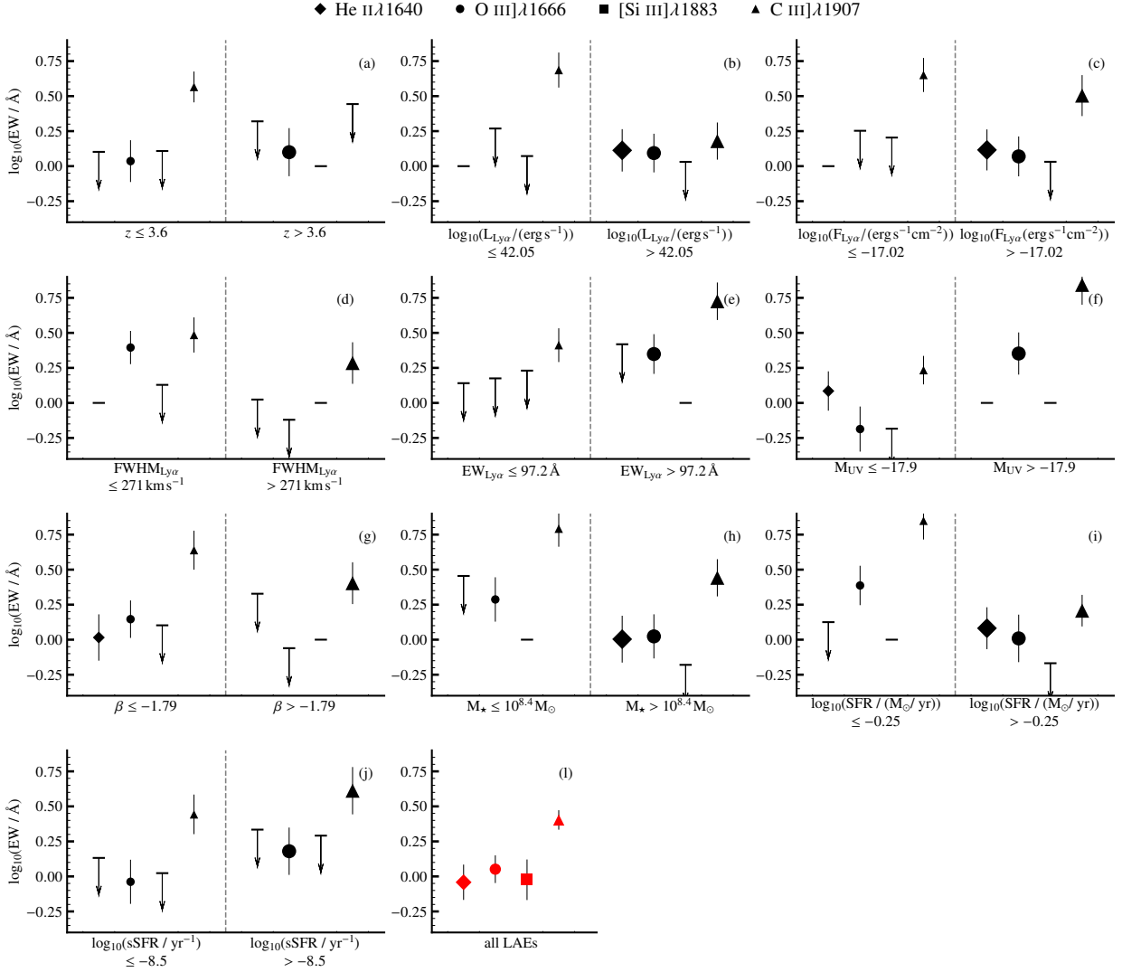
Fig. 6. EWs of He II, O III]1666, [Si III]1883 and [C III]1907 for the different subsamples of MUSE HUDF LAEs (x-axis). The symbols refer to different emission lines, as labeled in the legend. Smaller and larger symbol sizes indicate the subsample of LAEs whose property is lower and higher than the median value, respectively. Empty symbols with downward arrows indicate upper limits, while non-detections are shown with the black dash. Red symbols show the EWs for all the 220 LAEs in the sample.
