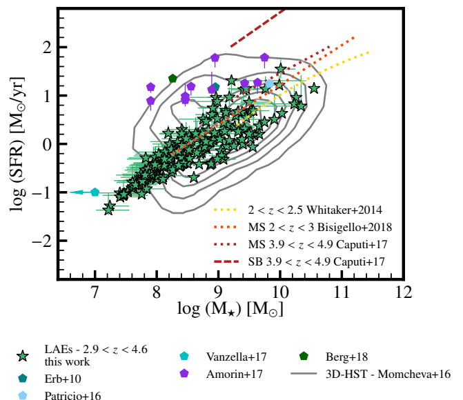
Fig. 2. Distribution of the LAEs sample (green stars) in the stellar mass - SFR plane. For comparison, values for 2.4 < z < 5.5 galaxies in the 3D-HST survey public catalog by Momcheva et al. (2016) and data for z \gtrsim 2 star-forming galaxies from Erb et al. (2010), Patricio et al. (2016), Amorin et al. (2017), Vanzella et al. (2017) and Berg et al. (2018) (see also Sect. 5.2) are shown color-coded as labeled in the legend. The curves of the star-formation sequence from Whitaker et al. (2014) at 2 < z < 2.5 , main sequence (MS) at 2 < z < 3 from Bisigello et al. (2018) and at 3.9 < z < 4.9 from Caputi et al. (2017) and the starburst (SB) sequence at 3.9 < z < 4.9 from Caputi et al. (2017) are shown for reference.
