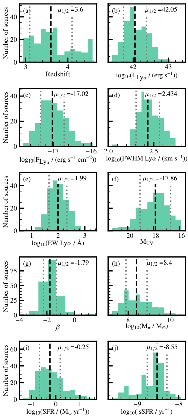
Fig. 1. Distributions of observed and physical properties of the LAEs sample described in Sect. 2.1. From panel a) to j): redshift, L_{\text{Ly}\alpha} luminosity, L_{\text{Ly}\alpha} flux, L_{\text{Ly}\alpha} FWHM, rest-frame L_{\text{Ly}\alpha} EW, absolute UV magnitude, UV spectral slope, stellar mass, SFR and sSFR. The Ly \alpha emission shown here has not been corrected by attenuation from dust. The vertical dashed black line indicate the median value, \mu_{1/2} (reported on the top right), of the distributions used to select the subsamples of Sect. 3.2. The vertical dotted gray lines indicate the median absolute deviation.
