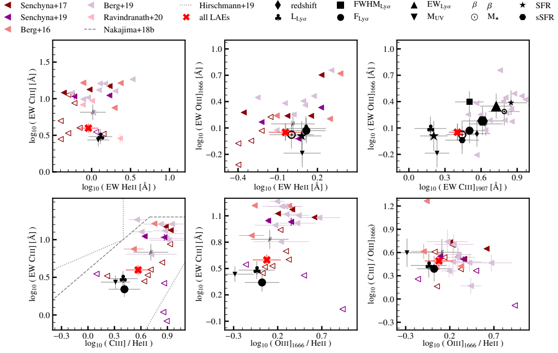
Fig. 8. UV emission line properties of the MUSE HUDF LAE subsamples and local galaxies from the literature described in Sects. 4.1 and 5.2. The diagrams show different combinations of EWs and ratios of the He II, O III] \lambda 1666, C III] and [C III] \lambda 1907 emission lines. Different black symbols refer to S/N > 2.5 line detections for different LAE subsamples and the red cross to the total LAE sample. Smaller and larger symbols indicate the subsample of LAEs whose property is lower or higher than the median value, respectively. Different colors refer to different samples from the literature, as labelled in the legend. Open and filled symbols indicate upper limits and detections, respectively. The left triangles refer to local galaxies. The gray dashed lines are the separation criteria between AGN and star-forming galaxies from Nakajima et al. (2018a), while the gray dotted lines the selection criteria for AGN, composite and star-forming galaxies from Hirschmann et al. (2019).
