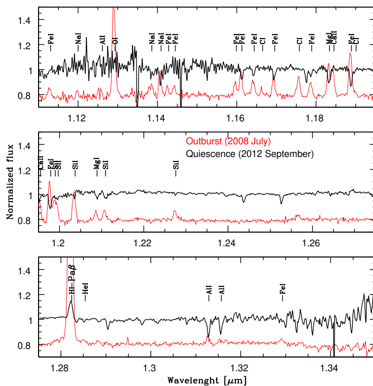
Fig. 2. Normalized SINFONI J-band spectrum of EX Lup in quiescence compared to the outburst. The position of the emission lines seen in the J-band spectrum taken during the outburst are marked (Kóspál et al. 2011). Many lines are seen in absorption rather than in emission, with the exception of the \text{Pa}\beta lines, which is still seen in emission. The outburst spectrum is shifted in intensity.
