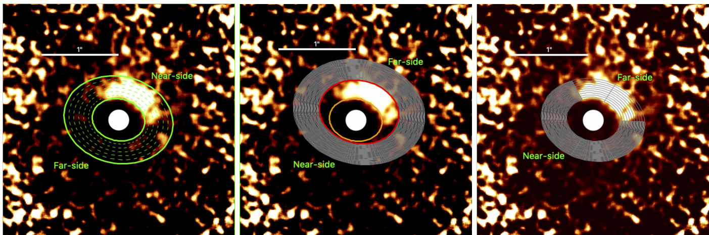
Fig. 8. Q_\phi-r^2 scaled image. Near and far-side of the disk are marked, North is up, East is left. Left panel: the ellipses show the de-projected scattering surface. Near and far-side of the disk are defined according to the brightness asymmetries: brighter side closer to the observer. Middle panel: the brighter side of the disk is coming from the illuminated wall of the outer disk. The orange and red ellipses mark the walls of the disk, the grey-shaded area marks the optically thick disk. Right panel: shadowed disk. The heavy-shaded grey area shows the portion of the disk that is shadowed due to the multiple inner rings misalignment. The light-shaded grey area marks the portion of the disk that is not shadowed, and is emitting in scattered light.
