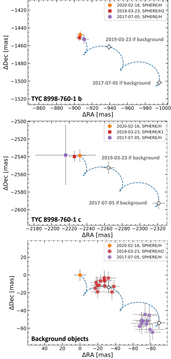
Figure 2. Multiepoch proper motion assessments of TYC 8998-760-1 b, c, and confirmed background objects. The colored markers represent the extracted relative astrometry of objects in the SPHERE field of view. The blue, dashed line represents the trajectory of a static background object and the white circles indicate the expected position of such an object, evaluated at the epochs indicated in the top and middle panels. Whereas the origin of the coordinate system is located at the position of the star for the comoving companions (top and middle panel), we present the relative offsets to reference epoch 2020 February 26 for confirmed background objects (bottom panel). The field of view sizes of the plots and the relative positions of the background trajectories are identical for all three panels, so that individual measurements of companions and background objects can be compared amongst each other.
