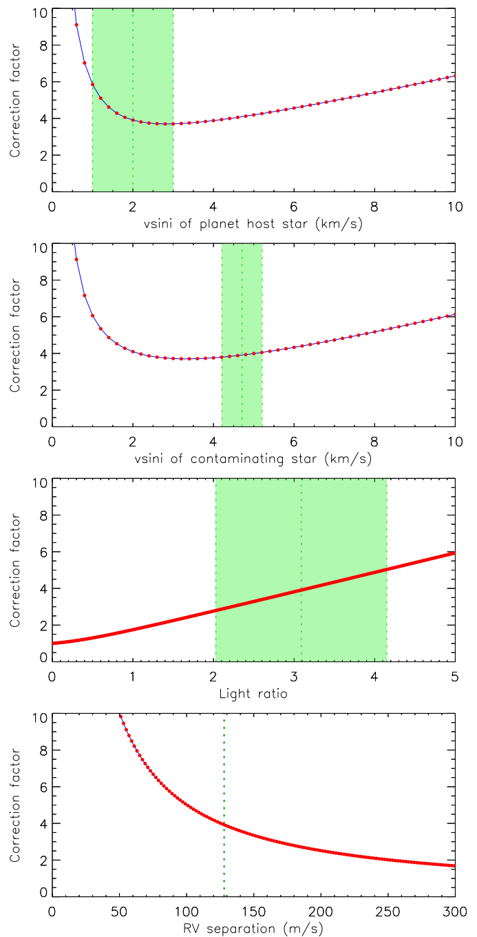
Fig. 3. Plots showing the behaviour of the correction factor for WASP-20 in the case that the planet host star is the fainter star. Other comments are as for Fig. 2.
