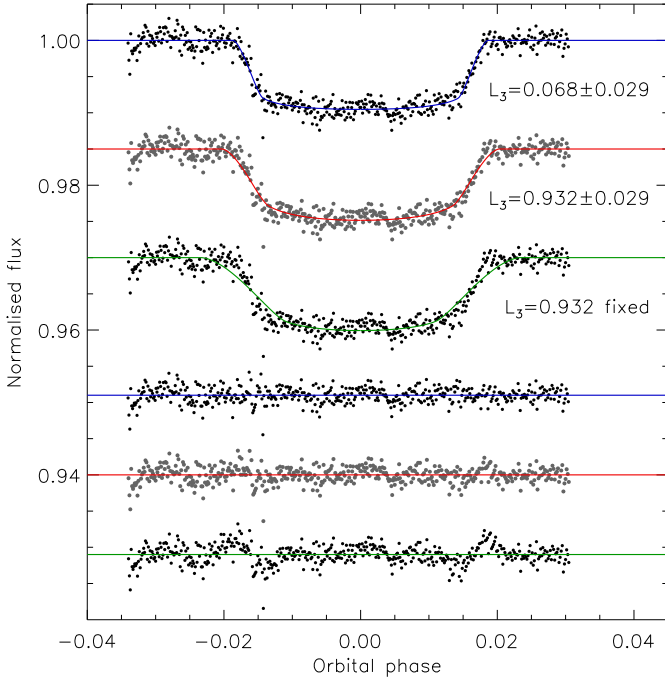
Fig. 4. Fit to the Euler telescope light curve of WASP-70. The observational data are shown as black and grey points. The JKTEBOP fits are shown for three scenarios: planet transiting brighter star; planet transiting fainter star; and planet transiting fainter star with the third light value forced to match that found from our direct image. The residuals of the fits are shown at the base of the figure with arbitrary offsets from zero.
