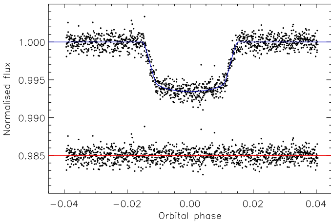
Fig. 7. Fit to the TESS light curve of WASP-131. Only the fit with the planet orbiting star A is shown.
