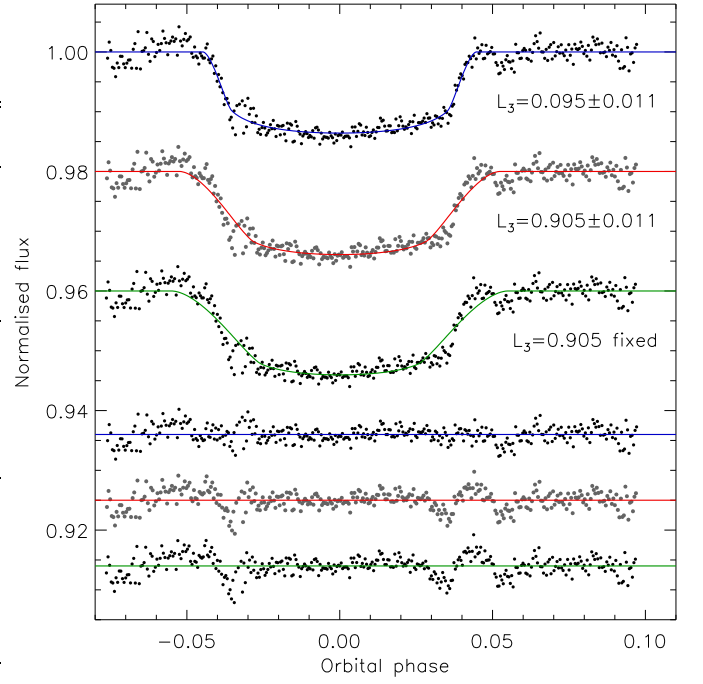
Fig. 6. Fit to the light curve of WASP-76 presented in the current work. The plotted quantities are otherwise the same as for Fig. 4.
