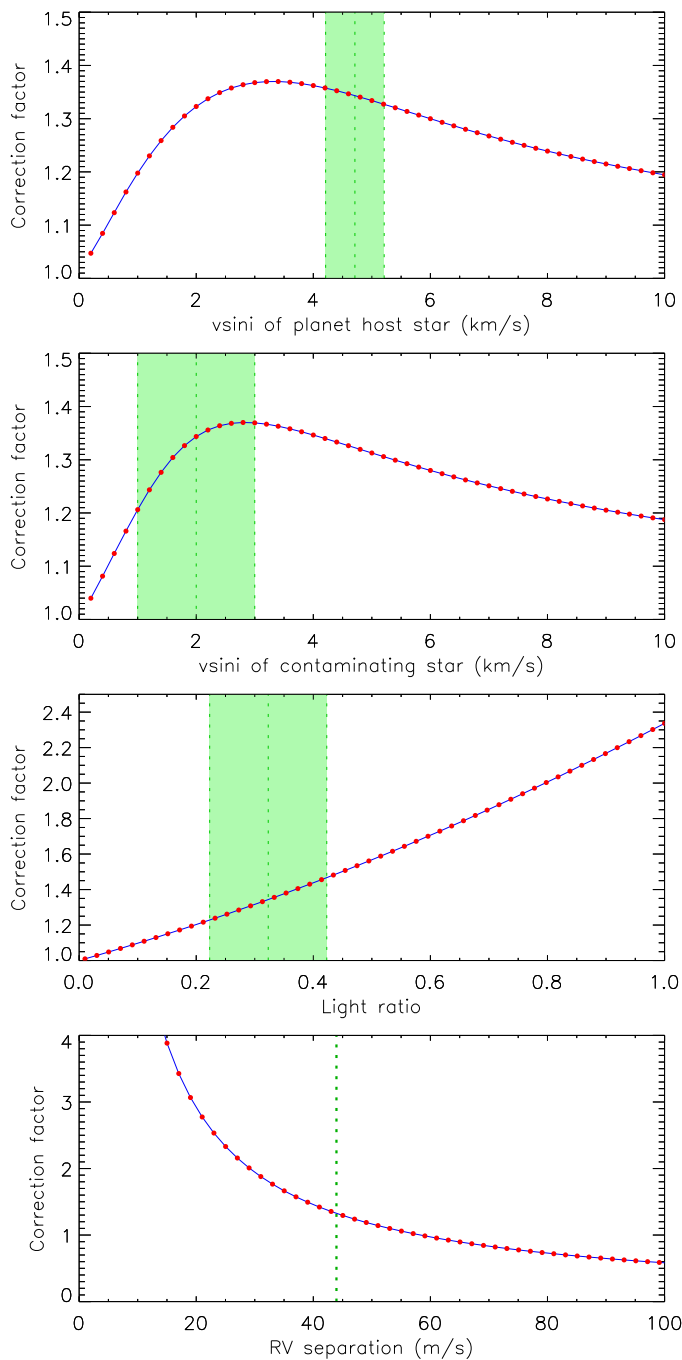
Fig. 2. Plots showing the behaviour of the correction factor for WASP-20 in the case that the planet transits the brighter star. The correction factor is shown as a function of the v \sin i values of the two stars, and of the light ratio. The bottom panel is included for reference and shows its variation as a function of the RV separation of the two stars. In each case the correction factor is shown using red points connected by blue lines, and the assumed system parameters are shown with their errorbars as green dotted lines, with the range of values allowed by the uncertainties indicated by light green shading.
