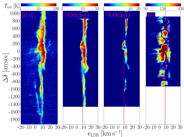
Fig. 8. PV diagrams along vertical position cut 1 indicated in Fig. 2 ( \Delta\alpha = 167'' - 242'' ) in [C II], ^{12}\text{CO}(2-1) , ^{13}\text{CO}(2-1) (Berné et al. 2014; Goicoechea et al. 2020), and H I (Van der Werf et al. 2013).
