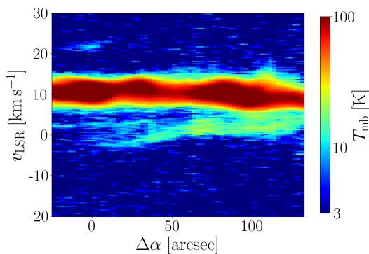
Fig. 22. PV diagram along position cut shown in Fig. 13 of Van der Werf et al. (2013), perpendicular to the Orion Bar through the Huygens Region.
