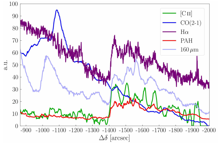
Fig. 4. Line cut through the southwest of the Veil shell, indicated in Fig. 2. The onset of the shell is marked by a steep increase in all tracers, except CO, at \Delta\delta \simeq -1400'' . With a line angle of 30^\circ with respect to the vertical axis, this is at a distance of 3.25 pc from the Trapezium stars.
