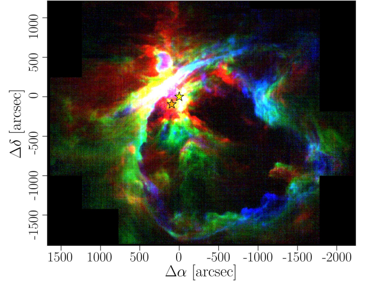
Fig. 7. Three-color image of velocity channels towards M42 and M43. Blue is the velocity channel v_{\text{LSR}} = 4\text{--}5 \text{ km s}^{-1} , green v_{\text{LSR}} = 6\text{--}7 \text{ km s}^{-1} , and red v_{\text{LSR}} = 9\text{--}10 \text{ km s}^{-1} . With increasing v_{\text{LSR}} , the limb-brightened Veil shell filament is displaced outward, away from the bubble center. The gas of M43 that is expanding towards us can be observed in the blue channel; the limb-brightened shell of M43 has higher v_{\text{LSR}} .
