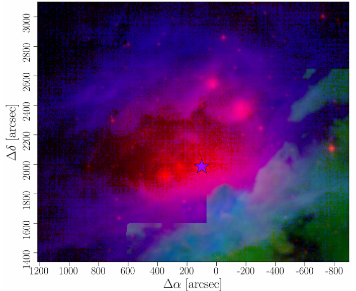
Fig. 14. Three-color image of NGC 1977. Red is H \alpha emission from the ionized gas, green is line-integrated CO(2-1) emission from molecular gas (coverage only in OMC3), and blue is the [C II] line-integrated intensity, tracing the neutral gas.
