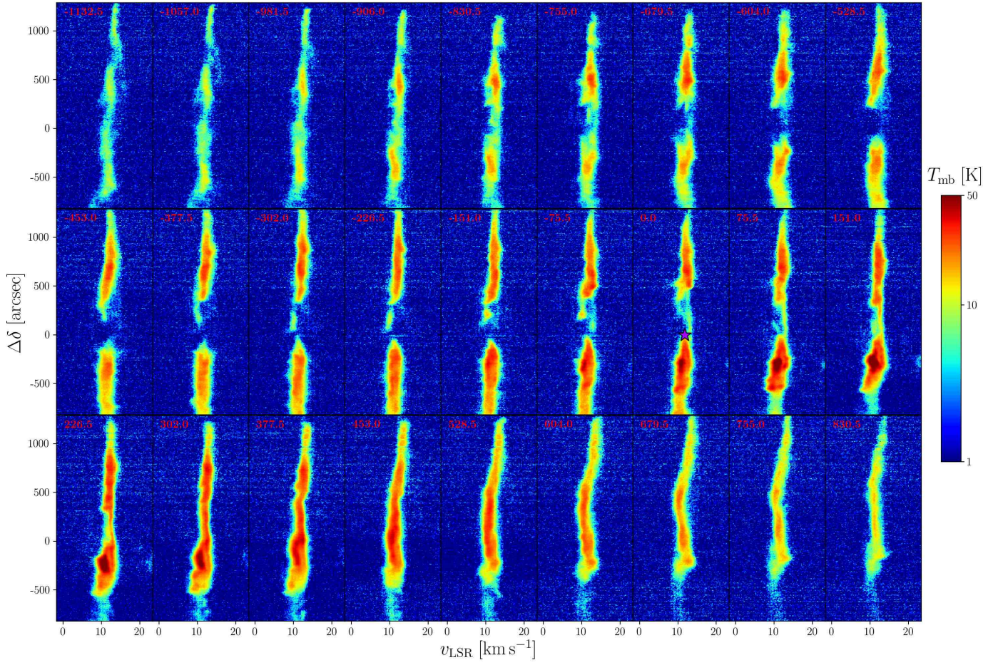
Fig. C.4. [C II] pv diagrams from NGC 1977, sliced along Dec. axis. Red numbers are the respective R.A. offsets in arc seconds. Coordinate offsets are given with respect to the position of 42 Orionis.
