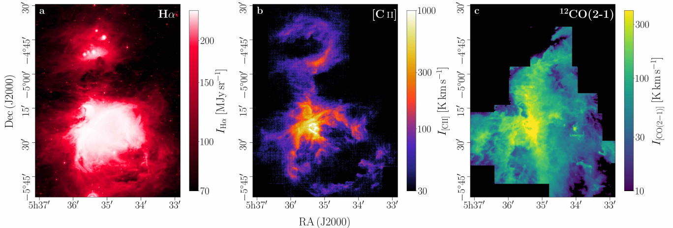
Fig. 1. Overview of the Orion Nebula (M42), M43, and NGC 1973, 1975, and 1977 in different wavelengths. Left: DSS2 H\alpha emission (ESO Archive). Center: [C\text{ II}] line-integrated emission (Pabst et al. 2019). Right: Line-integrated ^{12}\text{CO}(2-1) emission (Berné et al. 2014; Goicoechea et al. 2020). H\alpha emission stems from the ionized gas ( T \sim 10^4 K), the [C\text{ II}] line is emitted by mostly neutral gas ( T \sim 100 K), whereas CO traces the molecular gas ( T \sim 30 K). M42 and M43 have a substantial amount of molecular gas in the background, while NGC 1977 seems to be devoid of it (the coverage of the CO map is not sufficient, however, see discussion of the expansion characteristics below). All three regions comprise ionized gas within their neutral limb-brightened shells.
