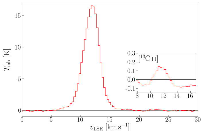
Fig. 15. Average [C II] spectrum towards [C II]-bright shell of NGC 1977 (without OMC3). The inlaid panel shows the (smoothed) residual of the spectrum, in the systemic velocity of the ^{13}\text{C II} F = 2-1 line, after subtracting the ^{12}\text{C II} fit. The ^{12}\text{C II} component can be approximated by a Gaussian with T_P \simeq 16.5 \pm 0.1 K, v_P \simeq 12.0 \pm 0.1 km s ^{-1} , \Delta v_{\text{FWHM}} \simeq 3.2 \pm 0.1 km s ^{-1} ; the ^{13}\text{C II} F = 2-1 component is fitted by a Gaussian with T_P \simeq 0.21 \pm 0.03 K, v_P \simeq 11.8 \pm 0.2 km s ^{-1} , \Delta v_{\text{FWHM}} \simeq 2.1 \pm 0.5 km s ^{-1} .
