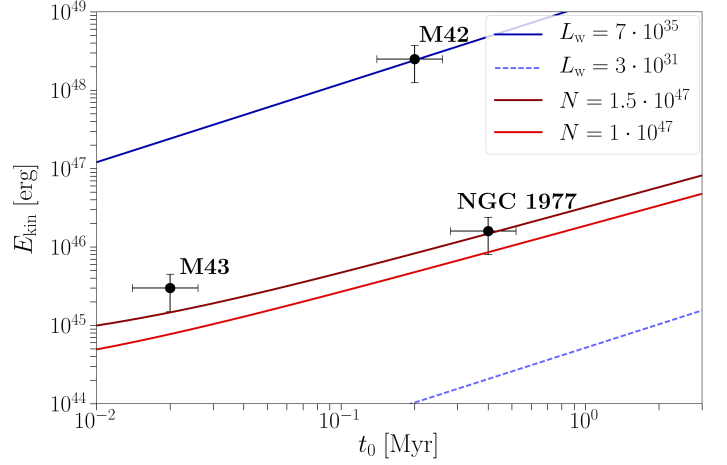
Fig. 23. Kinetic energy of expanding bubble shells versus expansion time. The lines are the predictions of wind models (blue) and models of pressure-driven expansion (red) with the parameters compiled in Tables 8 and 9.
