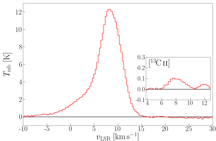
Fig. 3. Average [C II] spectrum towards the Veil shell without OMC1 and ISF. The inlaid panel shows the residual of the spectrum, in the systemic velocity of the ^{13}\text{C II} F = 2-1 line, after subtracting the ^{12}\text{C II} fit. The ^{12}\text{C II} line can be fitted by two Gaussians with T_P \simeq 11.2 \pm 0.3 K, v_P \simeq 8.8 \pm 0.1 km s ^{-1} , \Delta v_{\text{FWHM}} \simeq 5.0 \pm 0.1 km s ^{-1} and T_P \simeq 2.3 \pm 0.1 K, v_P \simeq 4.0 \pm 0.4 km s ^{-1} , \Delta v_{\text{FWHM}} \simeq 9.3 \pm 0.5 km s ^{-1} ; the ^{13}\text{C II} F = 2-1 component is fitted by a Gaussian with T_P \simeq 0.11 \pm 0.02 K, v_P \simeq 8.2 \pm 0.3 km s ^{-1} , \Delta v_{\text{FWHM}} \simeq 2.1 \pm 0.6 km s ^{-1} . The main line could also be fitted with three Gaussian components, but we compare the respective combined peak temperatures of the ^{12}\text{C II} and ^{13}\text{C II} line for a first-order estimate of the excitation conditions.
