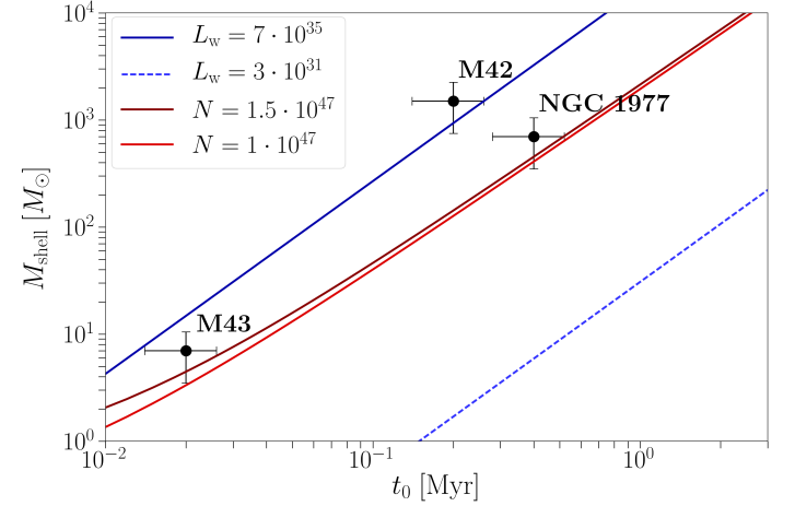
Fig. 24. Masses of expanding bubble shells versus expansion time. The lines are the predictions of wind models (blue) and models of pressure-driven expansion (red) with the parameters compiled in Tables 8 and 9.
