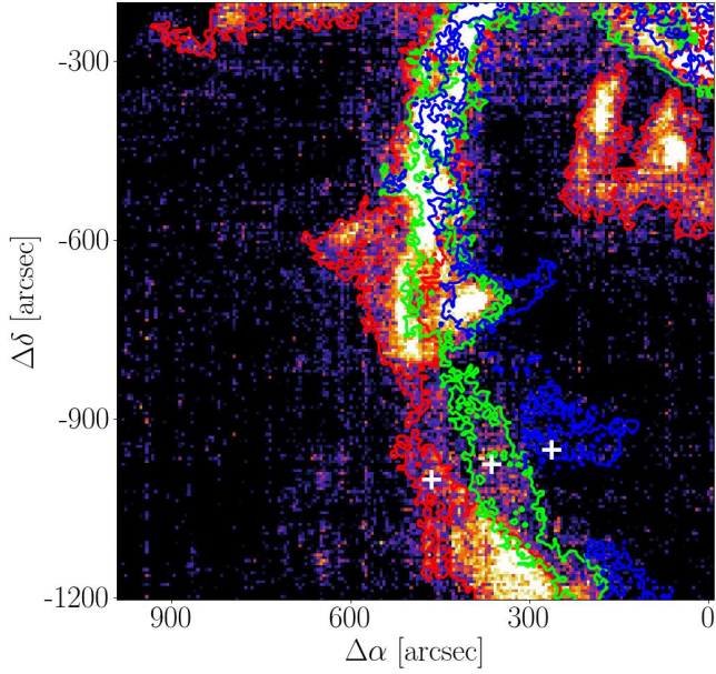
Fig. B.1. Color map of [C II] emission in velocity interval v_{\text{LSR}} = 0\text{--}5\text{ km s}^{-1} , with contours of the channel emission in v_{\text{LSR}} = 0\text{--}1\text{ km s}^{-1} , v_{\text{LSR}} = 2\text{--}3\text{ km s}^{-1} , and v_{\text{LSR}} = 4\text{--}5\text{ km s}^{-1} (blue, green, and red, respectively). From the displacement of the structure of brightest emission in these channels with respect to each other, points marked by the white crosses, we can estimate the expansion velocity to be v_{\text{exp}} \simeq 4.25\text{ km s}^{-1} . The projected distance between the crosses is 0.2\text{ pc} , and the projected distance from the Trapezium stars of the outermost filament, traced by blue contours, is 1.75\text{ pc} .
