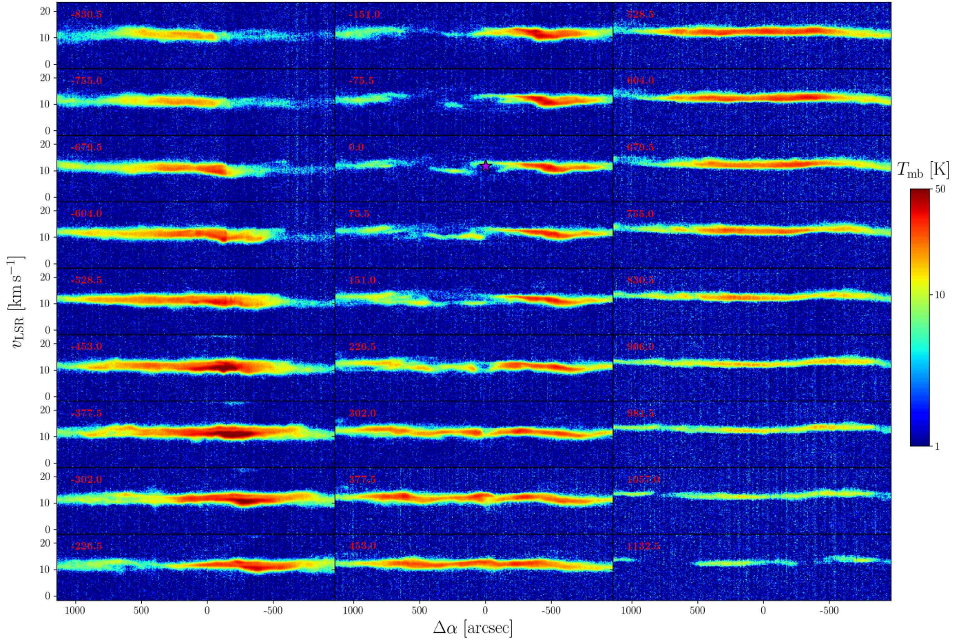
Fig. C.3. [C II] pv diagrams from NGC 1977, sliced along R.A. axis. Red numbers are the respective Dec. offsets in arc seconds. Coordinate offsets are given with respect to the position of 42 Orionis.
