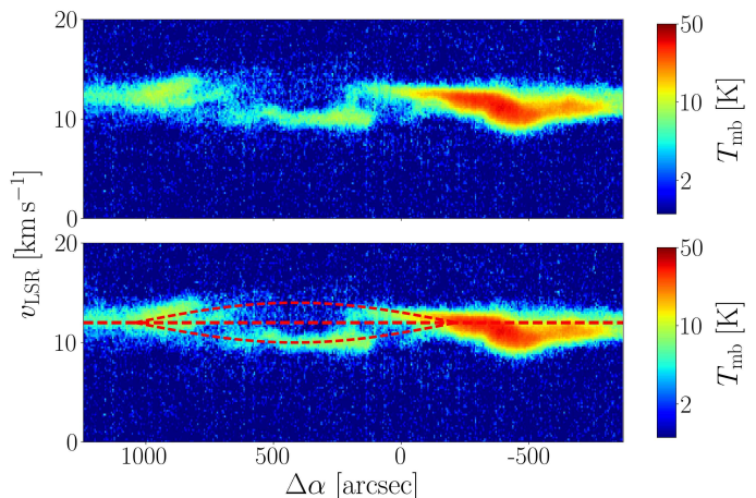
Fig. 17. [C II] pv diagram of NGC 1977 along position cut 3, indicated in Fig. 2 ( \Delta\delta = 2085''-2259'' ). The lower panel shows the same cut with the arc structure for an expansion velocity of \pm 1.5 km s ^{-1} (red dashed lines).
