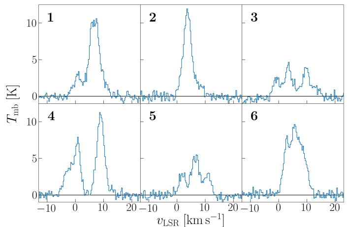
Fig. 20. [C II] spectra towards southern Veil shell. Each spectrum is averaged over a circle with a radius of 40'' as indicated in Fig. 19. We note that each spectrum consists of multiple line components, which is characteristic of thermodynamic instabilities.
