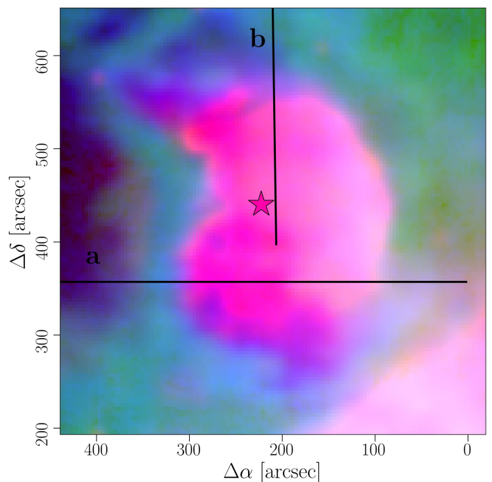
Fig. 9. Three-color image of M43. Red is H \alpha emission from the ionized gas, green is line-integrated CO(2-1) emission from molecular gas, and blue is the [C II] line-integrated intensity, tracing the neutral gas. The line cuts in Fig. 10 are taken along lines a and b.
