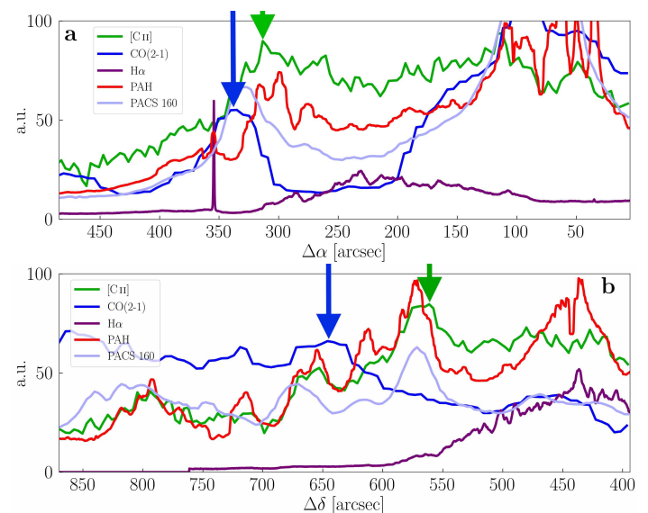
Fig. 10. Line cuts along lines a and b, indicated in Fig. 9. The arrows indicate the peaks in [C II] emission (green) and CO emission (blue) that correspond to the shell.
