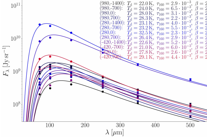
Fig. A.1. SED fits to individual points throughout the Orion Nebula complex. The flux in the PACS bands is plotted as circles; fluxes of the SPIRE bands are plotted as crosses. Numbers in brackets are the R.A. and Dec. offset, respectively, in arc seconds.
