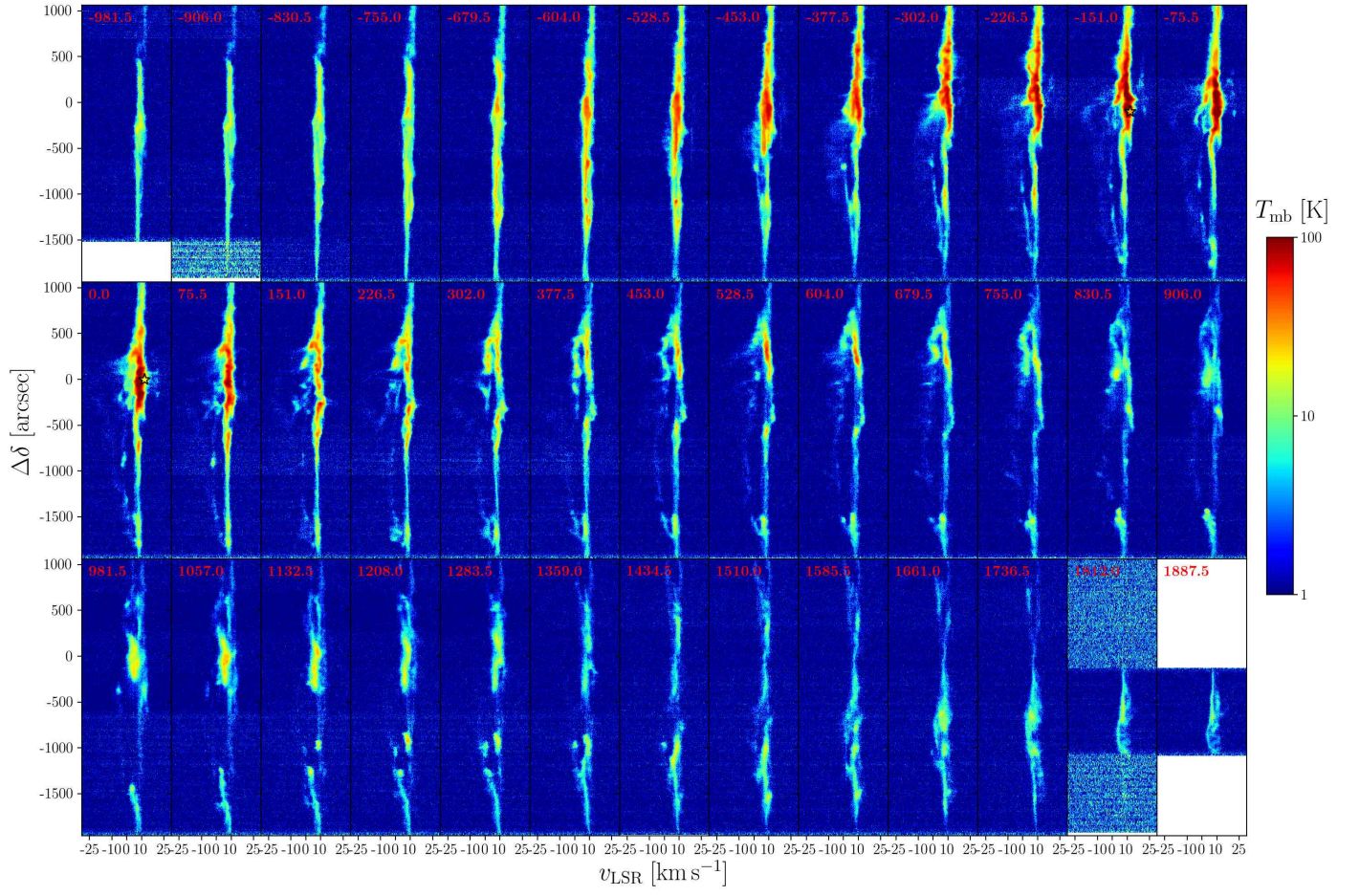
Fig. C.2. [C II] pv diagrams from the Veil shell, sliced along Dec. axis. Red numbers are the respective R.A. offsets in arc seconds.
