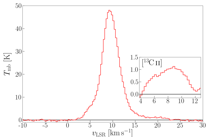
Fig. 11. Average [C II] spectrum towards the eastern shell of M43. The inlaid panel shows the residual of the spectrum, in the systemic velocity of the ^{13}\text{C II} F = 2-1 line, after subtracting the ^{12}\text{C II} fit. The ^{12}\text{C II} line can be fitted by a Gaussian with T_P \simeq 46.2 \pm 0.3 \text{ K} , v_P \simeq 9.6 \pm 0.1 \text{ km s}^{-1} , \Delta v_{\text{FWHM}} \simeq 4.6 \pm 0.1 \text{ km s}^{-1} ; the ^{13}\text{C II} F = 2-1 component is fitted by a Gaussian with T_P \simeq 1.1 \pm 0.2 \text{ K} , v_P \simeq 8.6 \pm 0.3 \text{ km s}^{-1} , \Delta v_{\text{FWHM}} \simeq 4.8 \pm 0.8 \text{ km s}^{-1} . We note that a better fit of the ^{12}\text{C II} line can be obtained by fitting two components with T_P \simeq 30.9 \pm 1.3 \text{ K} , v_P \simeq 9.6 \pm 0.1 \text{ km s}^{-1} , \Delta v_{\text{FWHM}} \simeq 3.3 \pm 0.1 \text{ km s}^{-1} and T_P \simeq 17.5 \pm 1.3 \text{ K} , v_P \simeq 9.8 \pm 0.1 \text{ km s}^{-1} , \Delta v_{\text{FWHM}} \simeq 6.8 \pm 0.2 \text{ km s}^{-1} , but both fits leave significant residuals.
