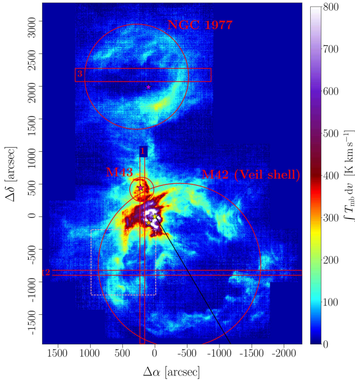
Fig. 2. [C II] line-integrated intensity from the Orion Nebula (M42), M43, and NGC 1977. The red rectangles 1 and 2 indicate the positions of the pv diagrams shown in Figs. 5 (horizontal) and 8 (vertical). Rectangle 3 indicates the position of the pv diagram shown in Fig. 17. The red circles delineate the approximate extent of the expanding bubbles of gas that are the Veil shell, M43, and NGC 1977, and within which the respective masses and luminosities are computed. The light-red dashed rectangle circumscribes the area of the eastern bright arm shown in Figs. B.1 and B.2. The black line indicates the position of the line cut in Fig. 4. The stars mark the position of \theta^1 Ori C (yellow), \theta^2 Ori A (orange), NU Ori (pink), and 42 Orionis (purple). Unless noted otherwise, all coordinate offsets are given with respect to the position of \theta^1 Ori C, (\alpha, \delta) = (5^{\text{h}}35^{\text{m}}16.46^{\text{s}}, -5^{\circ}23'22.85'') .
