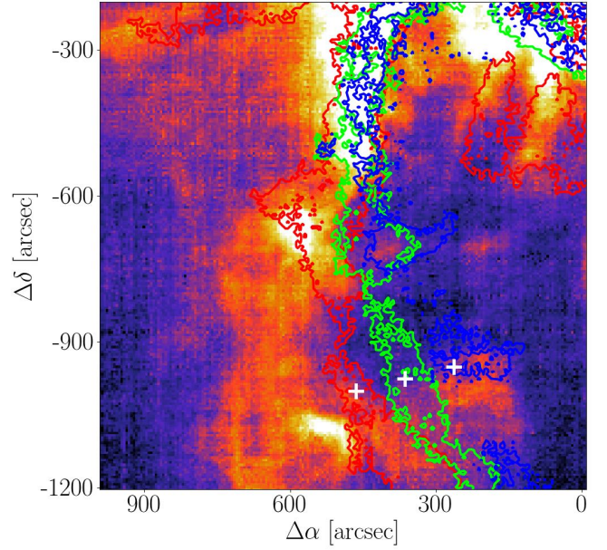
Fig. B.2. Color map of [C II] emission in velocity interval v_{\text{LSR}} = 0\text{--}15\text{ km s}^{-1} , with contours of the channel emission in v_{\text{LSR}} = 0\text{--}1\text{ km s}^{-1} , v_{\text{LSR}} = 2\text{--}3\text{ km s}^{-1} , and v_{\text{LSR}} = 4\text{--}5\text{ km s}^{-1} (blue, green, and red, respectively). The expanding filament grows brighter as it moves outward, probably mainly due to increasing limb-brightening, so the color map is dominated by the most outward filament.
