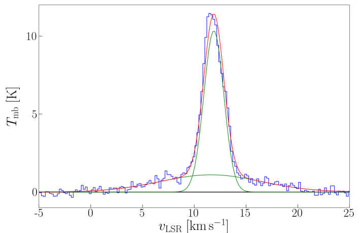
Fig. 16. [C II] spectrum towards NGC 1977, averaged over circular area with radius 125'' centered at 42 Orionis ( (\Delta\alpha, \Delta\delta) = (-100.4'', 1984.7'') ), with Gaussian fits. The fit parameters are given in Table 3.
