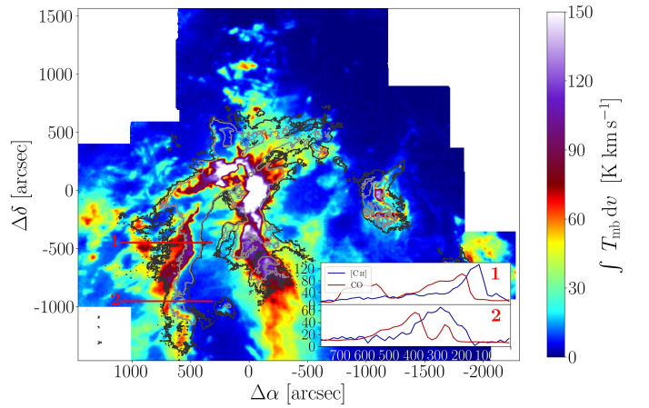
Fig. B.4. ^{12}\text{CO}(2\text{--}1) emission in velocity interval v_{\text{LSR}} = 5\text{--}8\text{ km s}^{-1} with [C II] emission in same velocity interval in contours (dark grey: 30\text{ K km s}^{-1} , light grey: 50\text{ K km s}^{-1} ). The in-laid panels show the line cuts along the two red lines indicated in the figure.
