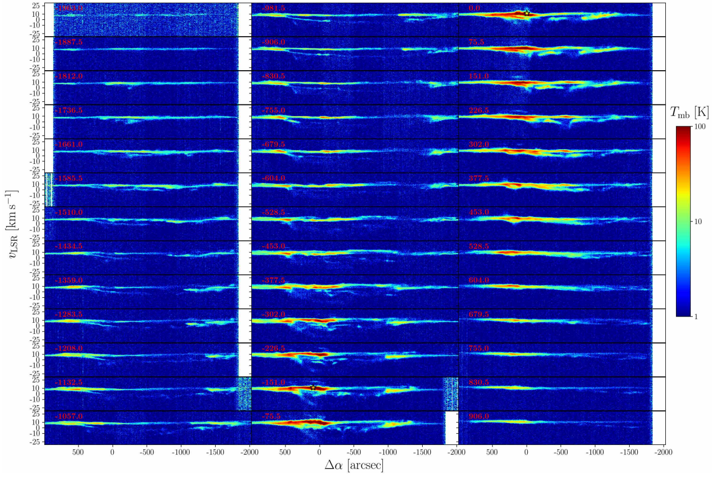
Fig. C.1. [C II] pv diagrams from the Veil shell, sliced along R.A. axis. Red numbers are the respective Dec. offsets in arc seconds.
