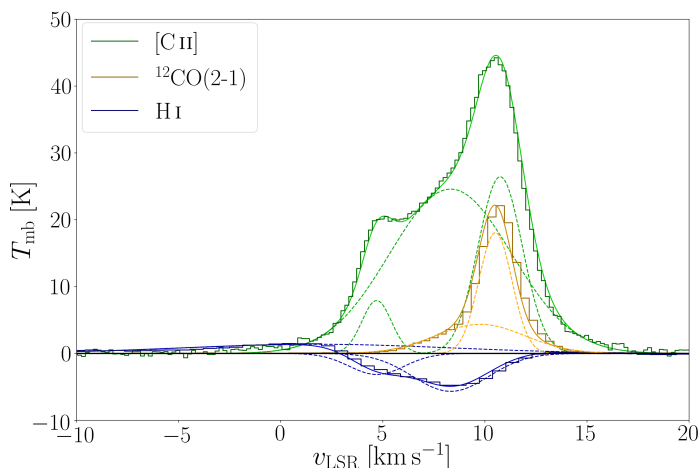
Fig. 21. [C II] (green), ^{12}\text{CO}(2-1) (yellow), and H I (blue) spectra towards the center of M43, averaged over a circle with radius r \simeq 40'' and center (\Delta\alpha, \Delta\delta) = (-226'', 440'') . Plotted are also the results of Gaussian fits (dashed lines). The fit parameters are given in Table 7. The H I spectrum is multiplied by 10^{-2} to fit the scale.
