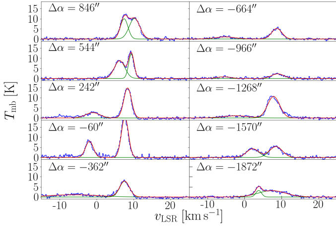
Fig. 6. [C II] spectra in the Veil shell taken from pv diagram in Fig. 5 with Gaussian fits. Spectra at \Delta\alpha = -362'' to \Delta\alpha = -1268'' are averaged over 151'' \times 75.5'' in order to improve the signal-to-noise ratio of the faint shell component to be fitted, others are averaged over 75.5'' \times 75.5'' . Coordinate offsets indicate the lower left-hand corner of the rectangle over which the spectra are averaged; \Delta\delta = -907'' . The fit parameters are given in Table 1.
