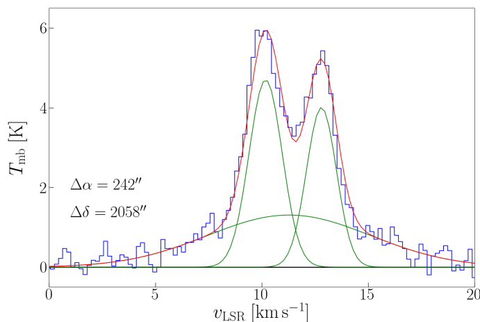
Fig. 18. [C II] spectrum along pv diagram in NGC 1977 (Fig. 17) with Gaussian fits, averaged over 201'' \times 201'' . Coordinate offsets indicate the lower left-hand corner of the square over which the spectrum is averaged. The two narrow components stem from the expanding shell, while the broad component originates in the ionized gas that is contained within the shell. Since the bubble expands in both directions, the peak-velocity difference is twice the expansion velocity, v_{\text{exp}} \simeq 1.3 \text{ km s}^{-1} . The fit parameters are given in Table 4.
