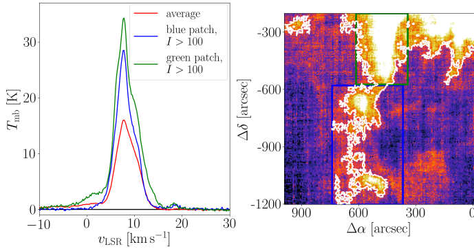
Fig. B.3. Right: [C II] line-integrated intensity in the bright eastern Rim. White contours indicate I_{[\text{C II}]} > 100\text{ K km s}^{-1} . Left: Averaged spectra from this region as indicated. Results of the analysis of the peak temperatures are given in Table B.1.
