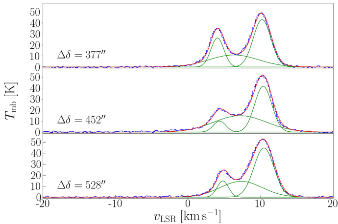
Fig. 13. [C II] spectra along position cut 1 (cf. Fig. 12) in M43 with Gaussian fits. Each spectrum is averaged over 75.5'' \times 25.2'' . The expanding shell has a distinguished emission peak. Additionally to the main component and the shell component, we fit a third, broad, component, that possibly stems from the ionized gas within the shell. Coordinate offsets indicate the lower left-hand corner of the rectangle over which the spectra are averaged; \Delta\alpha = 242'' . The fit parameters are given in Table 2.
