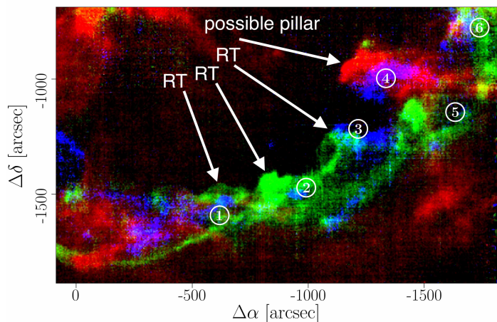
Fig. 19. Three-color image of [C II] velocity channels of the southern Veil shell. Blue is the velocity channel v_{\text{LSR}} = 0\text{--}2\text{ km s}^{-1} , green v_{\text{LSR}} = 4\text{--}6\text{ km s}^{-1} , and red v_{\text{LSR}} = 8\text{--}10\text{ km s}^{-1} . Arrows indicate structures that resemble fingers formed due to the Rayleigh-Taylor (RT) instability. One of these, labeled “possible pillar”, might also be formed by an overdensity encountered by the expanding shell and subsequently sculpted by the strong stellar radiation field, as it also is observed in CO (cf. Fig. 1c). The spectra shown in Fig. 20 were extracted towards the areas indicated by the numbered circles.
