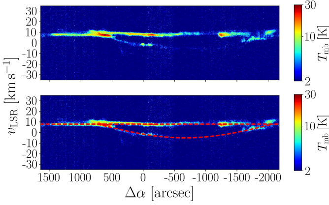
Fig. 5. [C II] pv diagram along horizontal position cut 2 indicated in Fig. 2 ( \Delta\delta = -907'' – 831'' ). The lower panel shows the same cut with the arc structure for an expansion velocity of 13 \text{ km s}^{-1} on a background velocity of 8 \text{ km s}^{-1} (red dashed lines).
