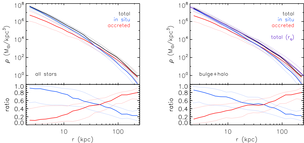
Figure 3. Left: The median stellar density profiles of the ARTEMIS systems for the total stellar component (black curve), in situ stellar component (light blue curve) and accreted stellar component (red curve). The dotted curves correspond to the scatter (16 th and 84 th percentiles). The bottom subpanel shows the median ratios of the in situ and accreted components both with respect to the total, as well as the 1-sigma halo-to-halo scatter in these profiles. Right: In analogy to the left panel but for the halo + bulge component only (i.e., omitting the disc). The purple curve corresponds to the total density profile of the halo + bulge, corrected for the flattening, \rho(r_q) .
