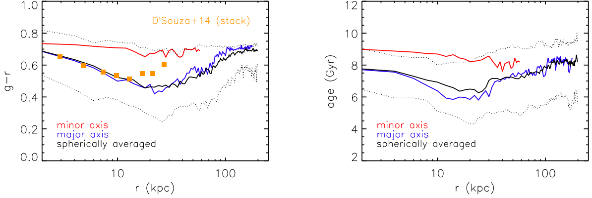
Figure 7. Left: A comparison between simulated g-r profiles and observations. The coloured curves represent the median colour along the major axis (blue), along the minor axes (red) and spherically-averaged (black). The black dotted curves show the corresponding galaxy-to-galaxy scatter (16 th and 84 th percentiles) for the spherically-averaged case. The filled orange squares show the azimuthally-averaged g-r colour of Milky Way-mass galaxies in SDSS DR9 from D’Souza et al. (2014). Right panel: The median age profile of the simulated galaxies. The coloured curves have the same meaning as in the left panel.
