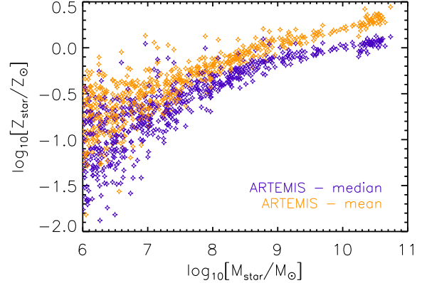
Figure A1. Comparison the stellar mass–metallicity relation of ARTEMIS using either the median star particle metallicity (empty purple stars) or the mass-weighted mean metallicity (empty orange stars), both for all stars within a 30 kpc (physical) aperture.
