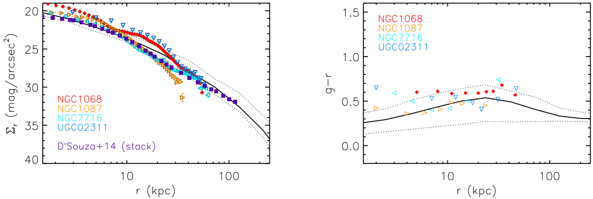
Figure 6. Left: The median r -band surface brightness profile, \Sigma_r(r) , of the simulated galaxies (solid black curve) and 1-sigma scatter (16 th and 84 th percentiles, dotted black curves). Various coloured data points are \Sigma_r measurements in 4 disc galaxies from the sample of Bakos & Trujillo (2012) that fall within our simulated mass range. All galaxies are face-on. Also plotted is the stacked SDSS r -band profile of D’Souza et al. (2014) for Milky Way-mass galaxies. Right: The median simulated g-r profile and its scatter (purple curves) versus g-r data from Bakos & Trujillo (2012) (symbols are as in the left panel).
