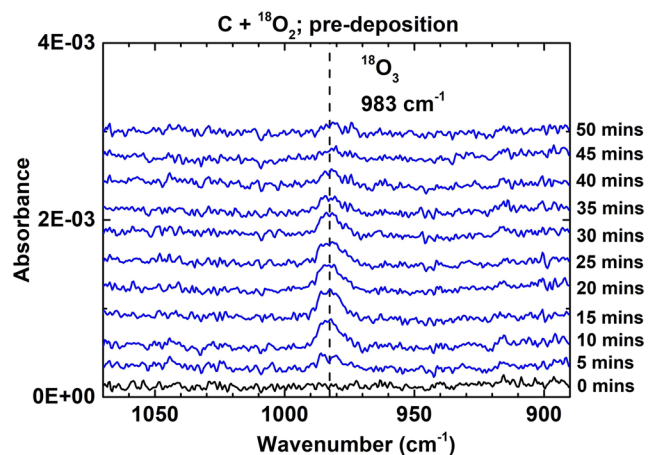
FIG. 6. RAIR spectra acquired after pre-deposition of atomic C and 18 O 2 on a 10 K surface (expt. 2). 10 L of 18 O 2 is first deposited, followed by carbonation for 50 min. The increase and subsequent decrease in the 18 O 3 band are highlighted. RAIR spectra are offset for clarity.
