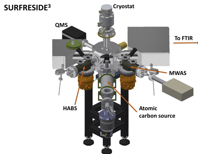
FIG. 1. A three atomic beam line system, including the new C-atom source introduced here. The three atomic beam lines are capable of generating H/D, N, O, and C-atoms, in addition to small radicals (e.g., OH, NH). It also contains two regular deposition lines. Both pre-deposition and co-deposition experiments can be performed. RAIRS and TPD-QMS are used as diagnostic tools.
