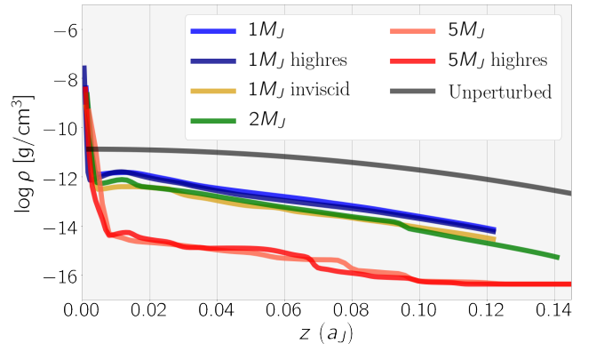
Figure 4. Vertical density above the planet for each simulation. Horizontal axis represents the height from the mid-plane in Jupiter semi-major axis ( a_J ); vertical axis shows density in logarithmic scale, in \text{g} \cdot \text{cm}^{-3} units.
