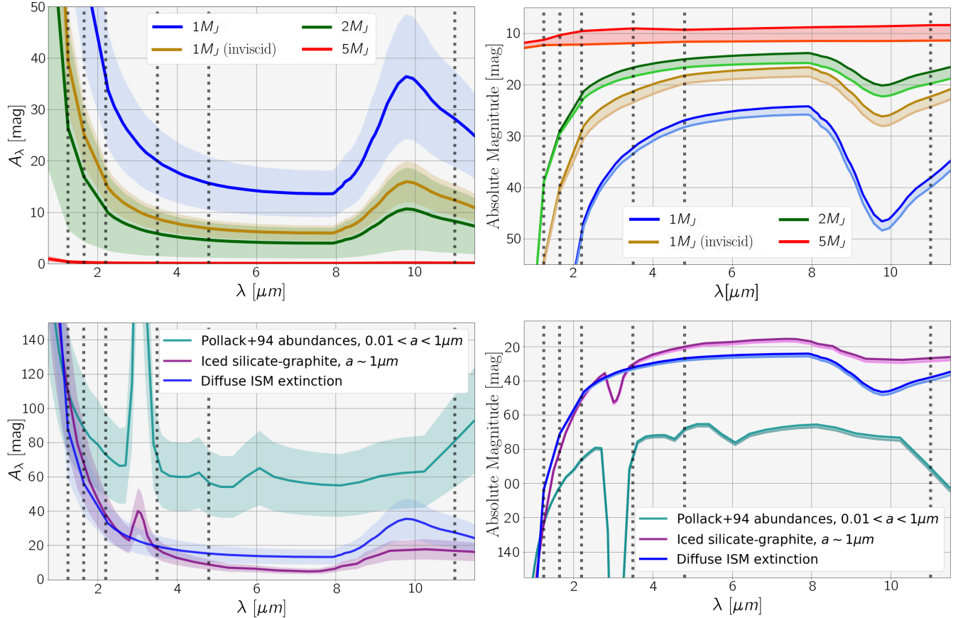
Figure 8. Top panels: extinction coefficients with uncertainties (left), and predicted magnitudes for the simulated systems (right), both as a function of wavelength. The predicted planet magnitudes are shown as an area delimited by the hot and cold planetary model. Bottom panels: extinction and predicted magnitudes of the 1 M_J viscous case using different dust grain models. The results for the various dust models are normalised at A_V . For every panel, the vertical dotted lines represent (from left to right) the central wavelength of J -, H -, K -, L -, M -, and N -bands.
