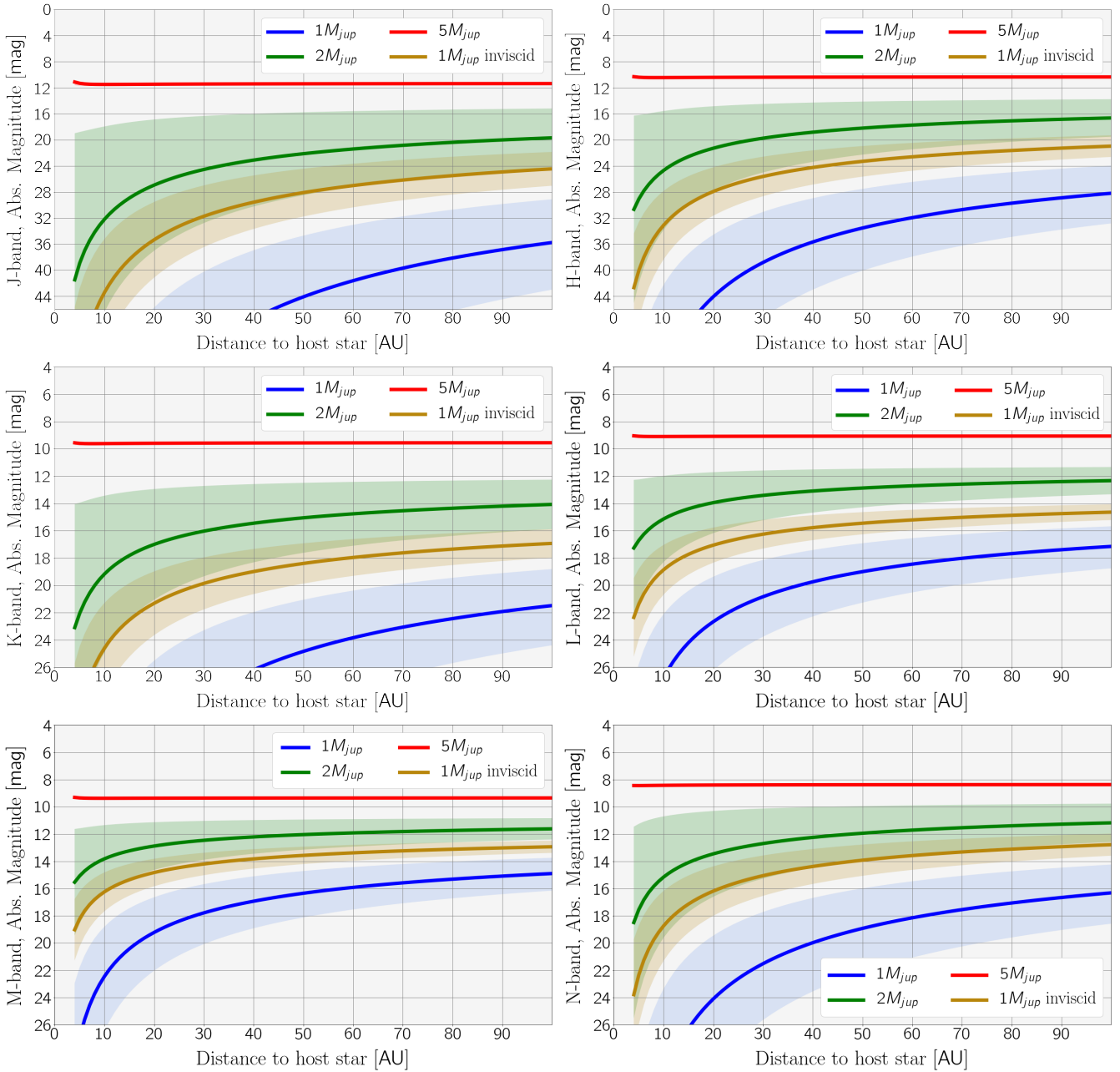
Figure 9. Absolute magnitudes at J -, H -, K -, L -, M - and N -bands for the simulated disc with an embedded planet ( 1 , 2 , 5 M_J , or a 1 M_J planet inviscid case) at different distances to the central star. The results are shown for a hot-start model of the formation scenario. The vertical axis for J and H -bands covers a wider range in order to include all the planets in the same panel.
