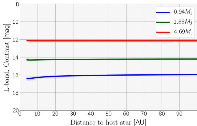
Figure 10. Application of our model to planets with 0.94, 1.88 and 4.69 M_J masses embedded in the CQ Tau disc. The coloured lines represent the contrast in L -band of each planet as a function of the distance to the central star placed at different distances along the disc.
