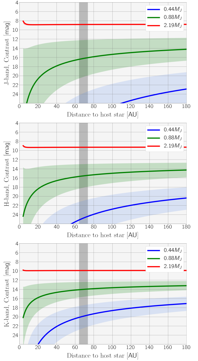
Figure B2. Application of our model to planets with 0.44 , 0.88 and 2.19 M_J masses embedded in the HL Tau disc. Contrast is shown for different distances to the host star in J -, H - and K -bands.
