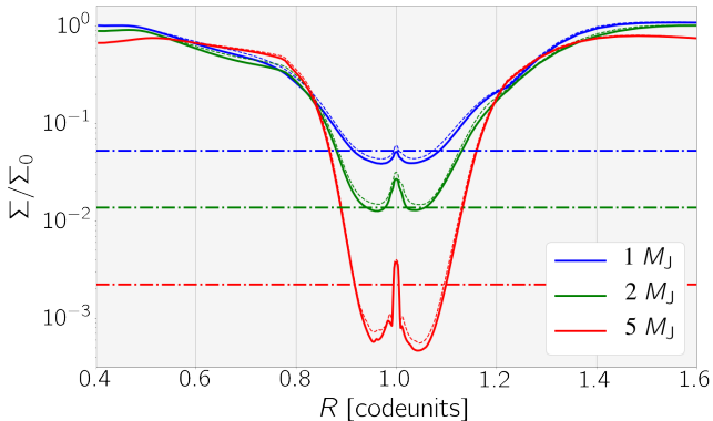
Figure 3. Surface density radial profile for 1, 2 and 5 M_J planets after the simulations reach a steady-state, shown as solid lines. The dash-dot lines are the respective predicted gap-depths, derived from an analytical model for gaps in protoplanetary discs (Duffell 2015). The dashed lines represent the surface density after 20 orbits. A value of 1 in radial code units is equivalent to 5.2 AU.
