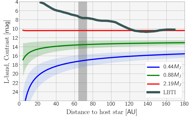
Figure 12. Contrast curves in L -band for planets embedded in HL Tau, including the 5\sigma detection limit of the observation from Testi et al. (2015). The observations were performed using LBTI/LMIRcam. The contrast curves are for planet masses of 0.44 , 0.88 and 2.19 M_J . The considered apparent magnitude of the central star was L = 6.23 mag (Testi et al. 2015). The coloured regions account for the uncertainty in the planet contrast. The grey vertical area is delimited by the D5 and D6 rings detected in dust continuum (ALMA Partnership et al. 2015).
