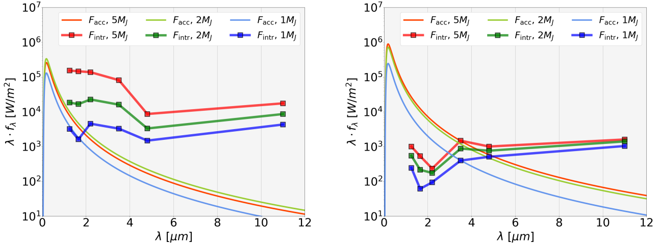
Figure 7. Intrinsic ( F_{\text{intr}} ) and accretion fluxes ( F_{\text{acc}} ) for 1, 2 and 5 M_J planets. The results for planets with a hot-start model are shown on the left panel, while cold-start models on the right. The intrinsic fluxes are plotted at the central wavelength of each band.
