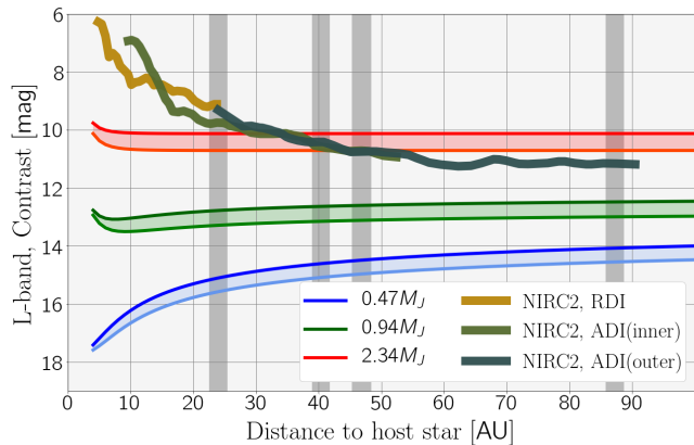
Figure 13. Contrast curves in L -band for planets embedded in TW Hya, including 95% significance detection limits of Keck/NIRC2 observations (Ruane et al. 2017). The contrast limits are shown for angular differential imaging (ADI) and reference star differential imaging (RDI). The contrast curves shown are for planet masses of 0.47 , 0.94 and 2.34 M_J . The apparent magnitude of the central star is L = 7.01 mag, taken from the W1 band in the WISE catalogue (Wright et al. 2010). The coloured regions for each planet model are delimited by the estimated ages (7-10 Myr, Ruane et al. 2017). The grey vertical lines account for the gaps observed in Andrews et al. (2016) and van Boekel et al. (2017).
