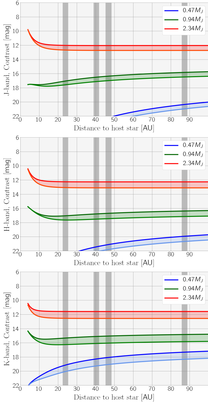
Figure B3. Application of our model to planets with 0.47 , 0.94 and 2.34 M_J masses embedded in the TW Hya disc. Contrast is shown for different distances to the host star in J -, H - and K -bands.
