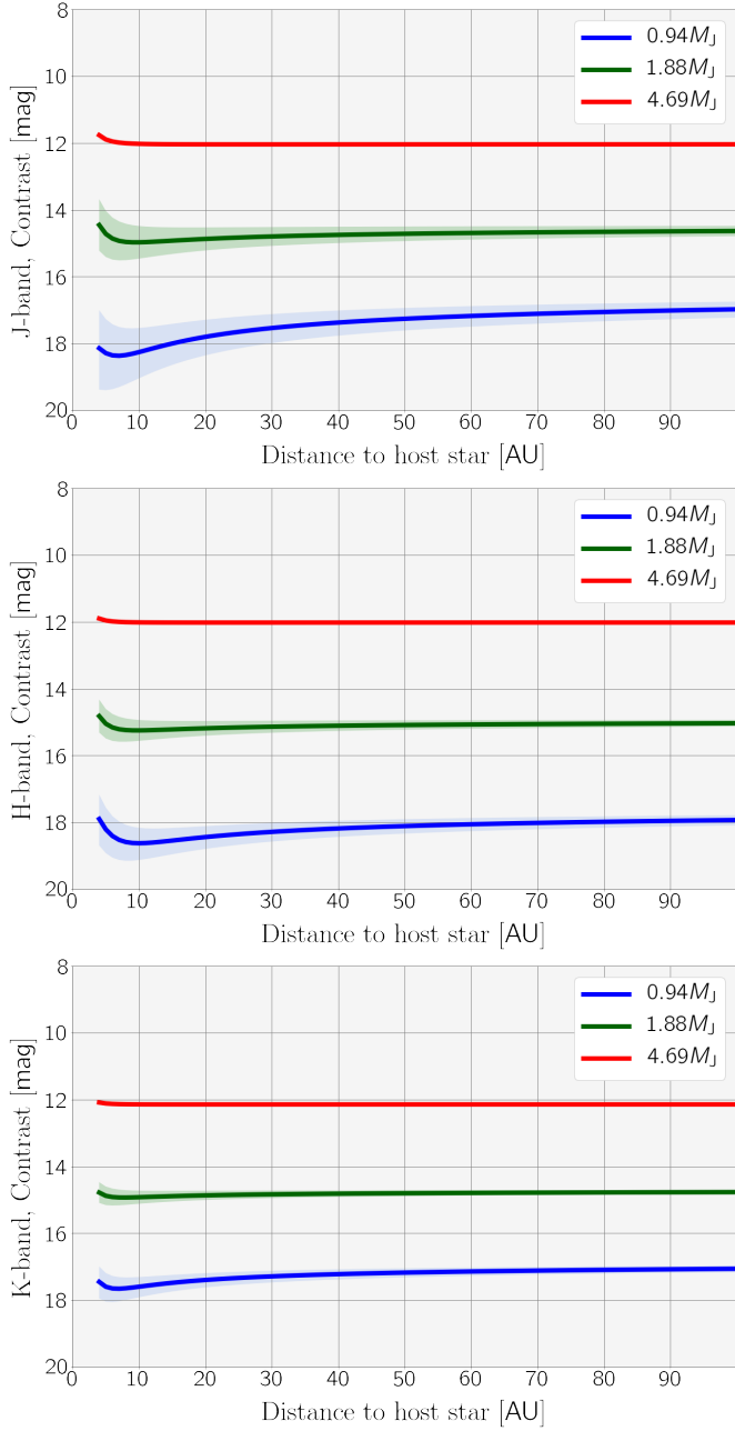
Figure B1. Contrast in J -, H - and K -bands of planets embedded in the CQ Tau disc as a function of distance to the central star. Results are for planets with 0.94 , 1.88 and 4.69 M_J .
