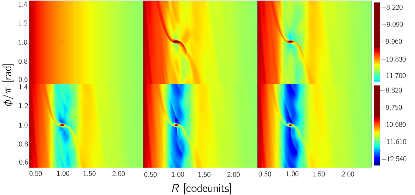
Figure 2. Evolution in time of the 2D density map at the mid-plane for the viscous disc with an embedded 1 M_J planet. A value of 1 in radial code units is equivalent to 5.2 AU (Jupiter semi-major axis). Density is represented in logarithmic scale, with values in \text{g} \cdot \text{cm}^{-3} . From top left to bottom right, each snapshot represents the density \rho of the disc after 1, 20, 50, 100, 150 and 200 orbits.
