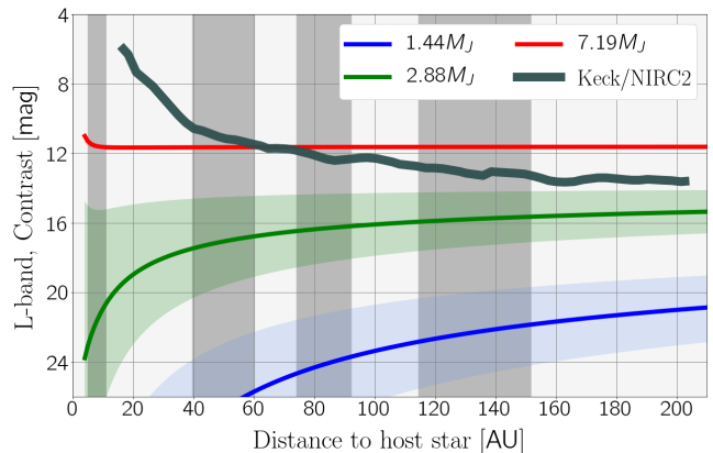
Figure 14. Contrast curves in L -band for planets embedded in HD 163296, including the 5\sigma detection limits of the observation from Guidi et al. (2018). The observations were performed using Keck/NIRC2. The contrast of planets with 1.44 , 2.88 and 7.19 M_J are shown. The apparent magnitude of the central star is L = 3.7 mag, inferred from the W1 band in the WISE catalogue (Wright et al. 2010). The grey vertical lines account for the gaps observed in Isella et al. (2016, 2018).
