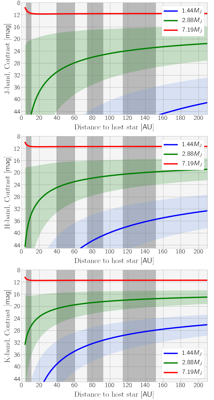
Figure B4. Application of our model to planets with 1.44 , 2.88 and 7.19 M_J masses embedded in the HD 163296 disc. Contrast is shown for different distances to the host star in J -, H - and K -bands.
