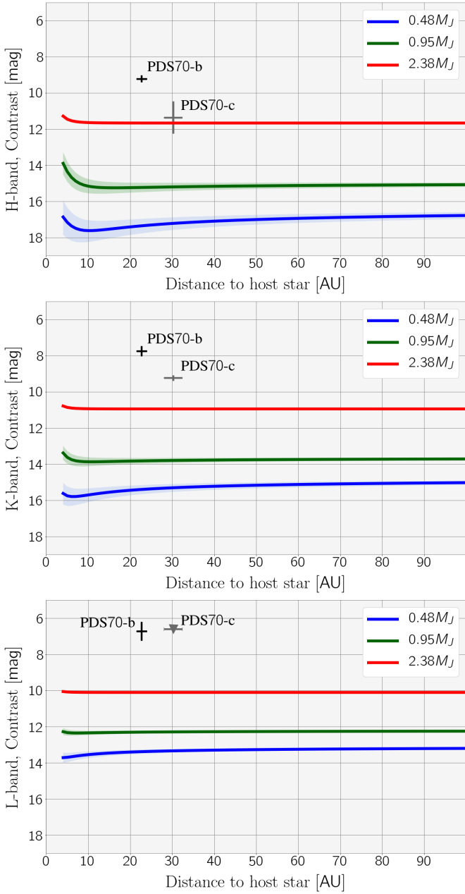
Figure 11. Application of our model to planets with 0.48 , 0.95 and 2.38 M_J embedded in the PDS 70 disc. The contrast curves shown for H -, K - and L -bands were obtained considering stellar magnitudes of H = 8.8 mag, K = 8.5 mag and L = 7.9 mag (Cutri et al. 2003; Cutri & et al. 2014). The two planetary companions (Keppler et al. 2018; Mesa et al. 2019; Haffert et al. 2019) are shown as black and grey crosses, with the corresponding uncertainties.
