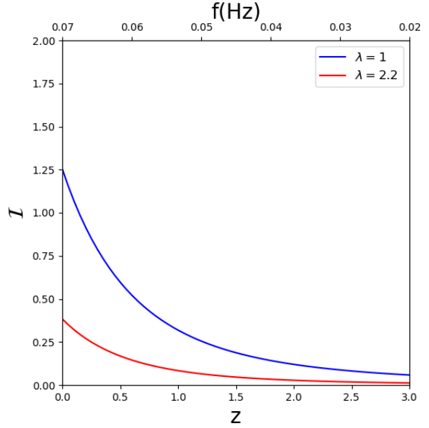
Figure 1. \mathcal{I}(z) , i.e. the function under integral (70) integrated only in \mathcal{M} , plotted with respect to z and f . We see that, independently from the value of \lambda , this function goes to zero for z_{\text{max}} \approx 3 , i.e. f \approx 0.02 \text{ Hz} .
