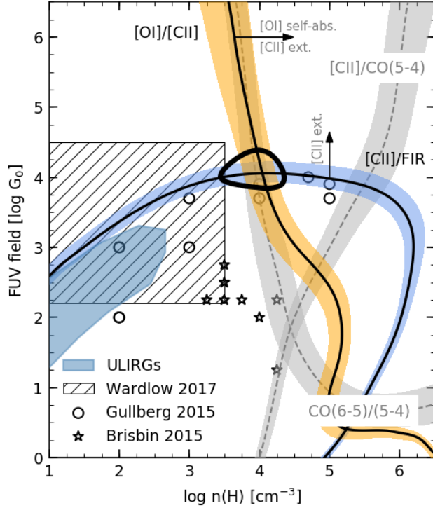
Figure 4. FUV field G and density ( n ) in G09.83808 inferred using the PDRTOOLBOX models (Kaufman et al. 2006; Pound & Wolfire 2008), compared to other unresolved studies of DSFGs at z = 1 - 5 (Brisbin et al. 2015; Gullberg et al. 2015; Wardlow et al. 2017), and z \sim 0 ULIRGs from Díaz-Santos et al. (2017). The thick black line indicates the 1\sigma confidence region. The [\text{C II}]/\text{CO}(5-4) and \text{CO}(6-5)/\text{CO}(5-4) line ratios are not used in the PDR modelling. The arrows indicate the direction (not magnitude) of the contours shifting if the [\text{C II}] emission is significantly more extended than FIR continuum, or if [\text{O I}]_{63} is self-absorbed.
