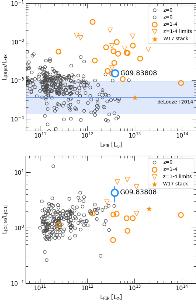
Figure 3. [O I]/FIR ( upper ) and [O I]/[C II] ( lower ) luminosity ratios in G09 83808, compared to other high-redshift detections and upper limits and z \sim 0 galaxies (GOALS sample from Díaz-Santos et al. 2017 and sources from the Graciá-Carpio et al. 2011 and Coppin et al. (2012) compilation), and the [O I] 63 -FIR correlation from De Looze et al. (2014). The line luminosities are given in units of L_{\odot} . FIR luminosities from the literature have been converted to the 8–1000 \mu\text{m} range. For strongly lensed sources, the luminosities are given as source-plane (de-lensed).
