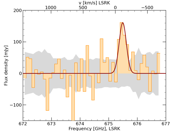
Figure 1. APEX SEPIA 660 spectrum of G09.83808, resampled into 100 MHz (45 km s -1 ) bins. The best-fitting Gaussian profile is indicated in red, the grey shading indicates the rms noise. The line is detected at \sim 4\sigma level over 100 MHz channels, and \sim 5\sigma over 225 MHz (100 km s -1 ) channels.
