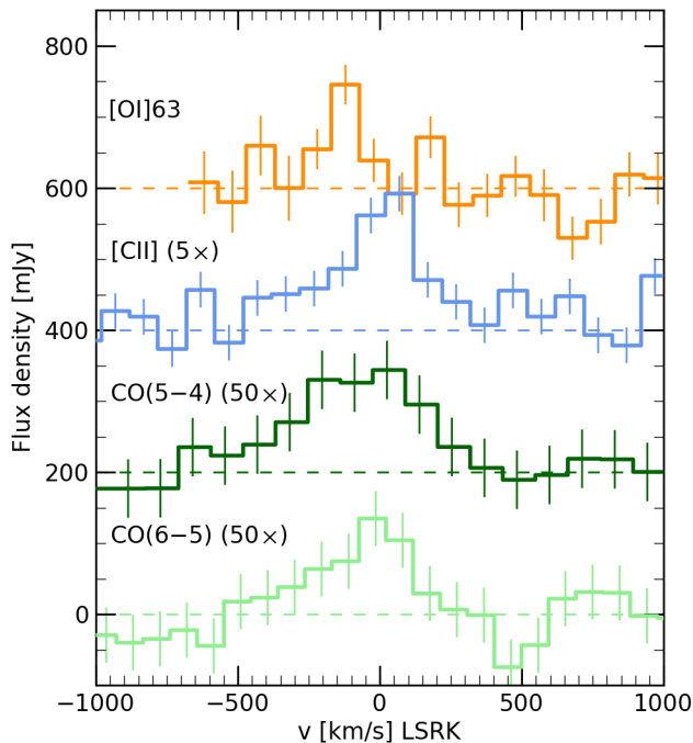
Figure 2. Comparison of the [\text{O I}]_{63} spectrum to the [\text{C II}] and \text{CO}(6-5) and (5-4) line profile from Zavala et al. (2018b). The [\text{O I}]_{63} line is noticeably narrower than the [\text{C II}] and \text{CO} emission, and tentatively offset from the [\text{C II}] line peak. All spectra have been re-sampled to 100 \text{ km s}^{-1} bins and are offset by 200 mJy for clarity. The velocities are given in the LSRK frame, using the optical definition.
