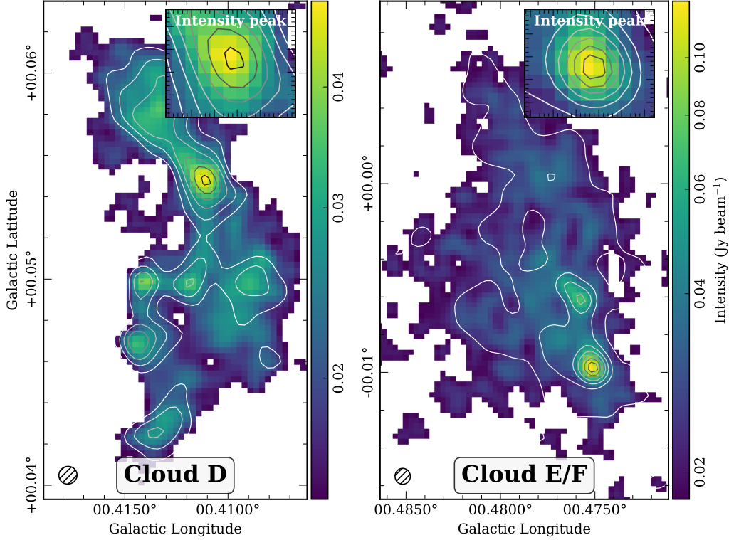
Figure 7. CMZoom observations compare favorably with more recent ALMA observations (Barnes et al. 2019). Shown in colorscale are the SMA observations towards the Dust Ridge Cloud D (left, also known as G0.412+0.052 ) and Cloud E (right, also known as G0.489+0.010 ) molecular clouds. These have been masked above a 3\sigma level, where \sigma = 5 \text{ mJy beam}^{-1} for Cloud D and \sigma = 6 \text{ mJy beam}^{-1} (upper limits from Walker et al. 2018). Overlaid are contours from similar frequency ALMA observations ( \sim 250 \text{ GHz} ) towards these sources, which have been smoothed to the approximate resolution of the SMA observations for comparison (see beam in lower left of each panel). The contours have been plotted in colors of white to black with increasing intensity. Also shown for clarity is a zoom-in of the flux peak in the upper right of each panel, with an identical color scale and contours to the full image.
