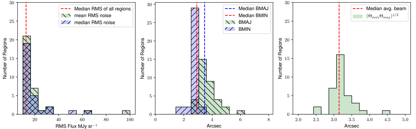
Figure 8. The overall angular resolution of the CMZoom survey is about 3''.2 (0.13 pc) and the RMS noise level is about 13 \text{ MJy Sr}^{-1} . There is variation across the survey, due to varying observing conditions and antenna configurations, as well as variations in the dynamic range based on the source emission in each field. Left: Histograms of the median and mean RMS noise value for each of the regions in the survey. Middle: Histograms of the variation of the beam major and minor axes over all surveyed regions. Right: A histogram of the geometrically averaged beam size (\theta_{\min} \cdot \theta_{\text{maj}})^{1/2} over all regions in the survey.
