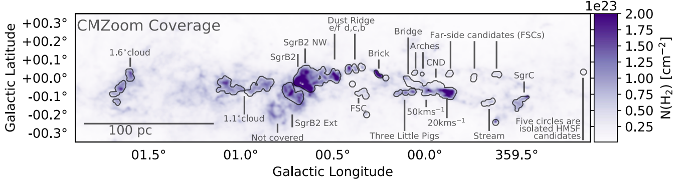
Figure 1. The Central Molecular Zone as seen in N(\text{H}_2) derived from the Herschel cold dust continuum (Molinari et al. 2010, Battersby et al., in prep.) in units of \text{cm}^{-2} in the colorscale with the CMZoom coverage is shown as gray contours. The figure shows colloquial names or notes on each observed region, as they are referenced to in Table 2 and throughout the text. Within the inner 5^\circ longitude \times 1^\circ latitude of the Galaxy, CMZoom is complete above a column density threshold of 10^{23} \text{ cm}^{-2} , with the exception of the cloud to the SE of Sgr B2 and isolated bright pixels, and with the addition of a few clouds as noted in Section 2.1. CMZoom covered 974 individual mosaic pointings over about 550 hours on the SMA.
