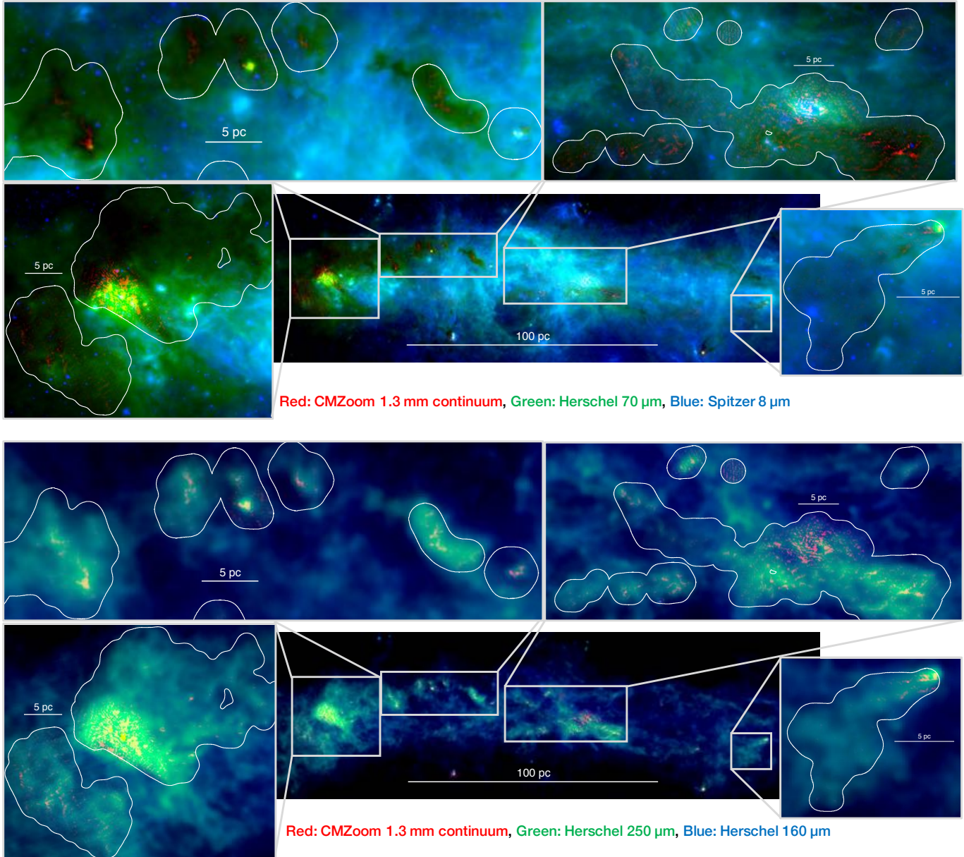
Figure 5. Three color images of the inner \sim 200 pc of the Galaxy, highlighting new CMZoom data in red, with various zoom-in views towards regions of interest. This figure shows only part of the full CMZoom coverage which extends in longitude in both directions (see Figures 1 and 4). All figures show CMZoom 1.3 mm dust continuum in red (not primary beam corrected) with survey coverage contours in white. The top figures show Herschel Hi-GAL 70 \mu\text{m} (Molinari et al. 2010) in green, and Spitzer GLIMPSE 8 \mu\text{m} (Benjamin et al. 2003) in blue. The bottom figures show Herschel Hi-GAL 250 and 160 \mu\text{m} (Molinari et al. 2010) in green and blue, respectively.
