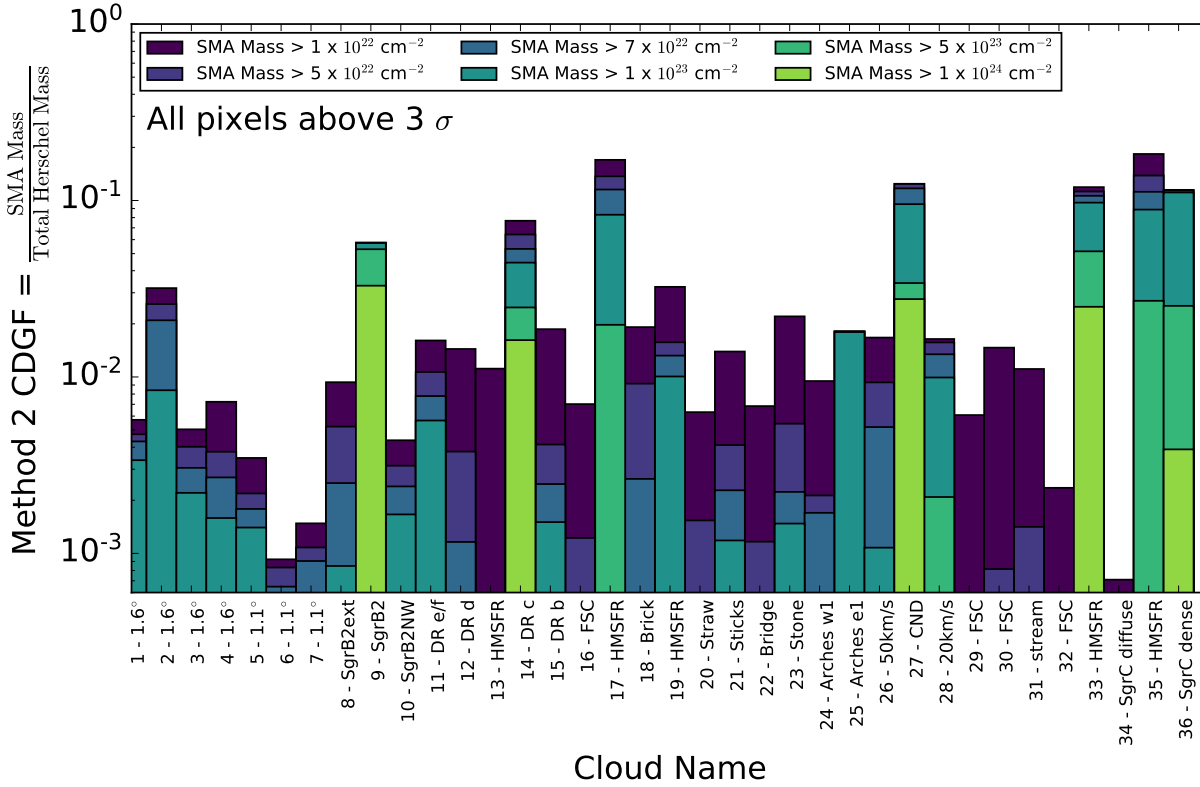
Figure 10. The method 2 compact dense gas fraction (CDGF), as measured in a comparison between the SMA and Herschel mass in each cloud. The names on the x-axis consist of a prefix, which is the mask number, and a shorthand name for each cloud, of which more details are provided in Table 2. They are ordered in decreasing central Galactic longitude from left to right. Each bar shows the mass above 3\sigma in the corresponding CMZoom SMA-mapped cloud, above various column density thresholds as shown in the legend, divided by the total mass of the cloud (at all column densities) as seen in Herschel. As also seen in Figure 9, the overall CDGF is less than 10% for most of the clouds, but this figure demonstrates the varying levels of substructure in each cloud. Note that the apparently high CDGF seen toward the CND located near \ell = 0^\circ , is likely due to contamination from the strong synchrotron source Sgr A* and resulting imaging artifacts (see Section 5.4 for more details). The CND is removed from the remaining CDGF plots.
