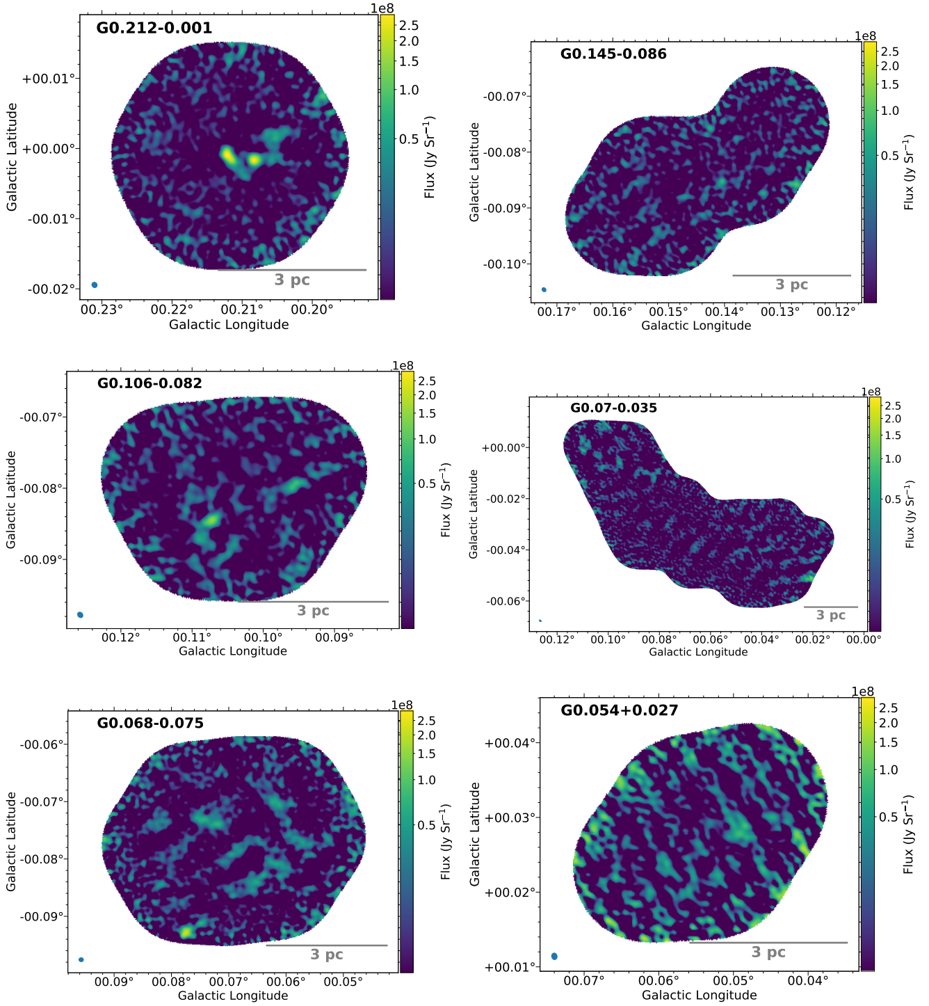
Figure 17. Images show the 1.3 mm dust continuum from the CMZoom Survey with a 3 pc scale-bar. The white contour shows the approximate 5- \sigma level while the black contour shows the approximate 10- \sigma level. All the images are displayed on same color scale from 2 - 290 MJy Sr -1 .
