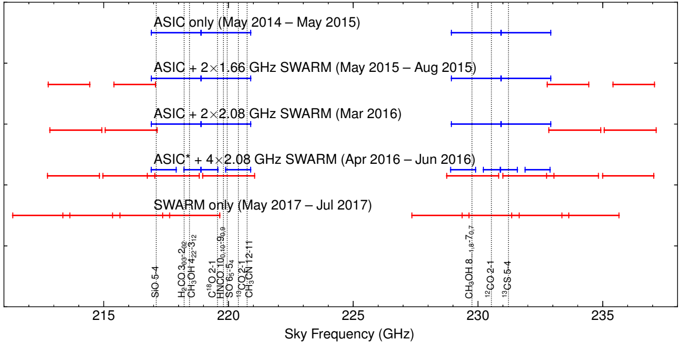
Figure 2. Spectral coverage of the CMZoom survey over time. Observations for the CMZoom survey took place over the period of May 2014 to July 2017. During this time, the SMA transitioned from the ASIC to the SWARM correlator, starting with ASIC only (spectral coverage shown in blue) and ending with SWARM (spectral coverage shown in red) only, with varying degrees of overlap in between. The ASIC* from April to June 2016 indicates a transitional period where ASIC was operating differently than its standard mode. Our key target spectral lines are shown as dashed lines in the plot. Coverage of these lines was maintained over the lifetime of the survey, except for a few tertiary lines in the three tracks observed in 2017 and a few other oddities that will be discussed in the spectral line data release paper.
