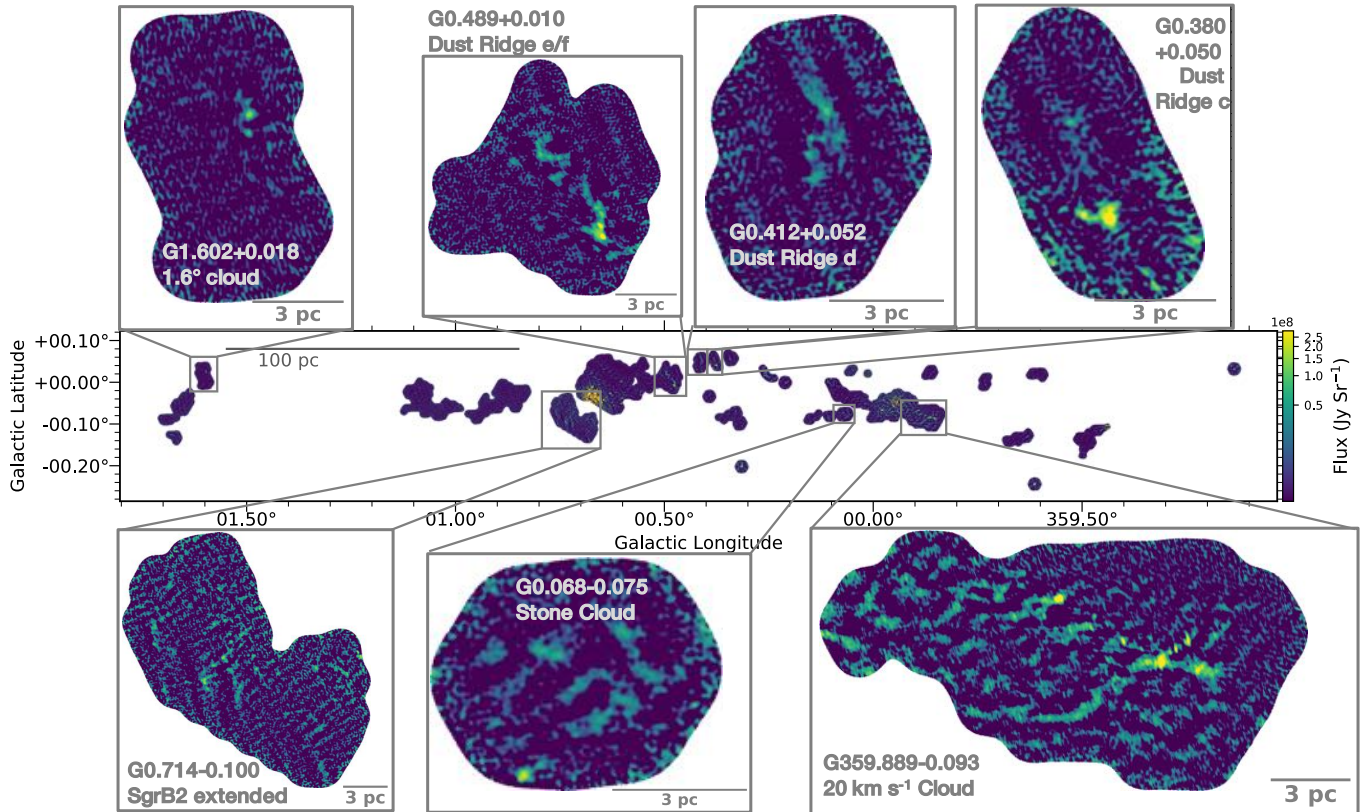
Figure 4. A mosaic of the full coverage of the CMZoom survey in 1.3 mm dust continuum, with zoom-ins toward various regions of interest. The images are all on the same color scale. The full image gallery is in Appendix C. Locally higher noise is seen in the vicinity of the strong continuum sources Sgr B2 ( l \sim 0^\circ.7 ) and Sgr A* ( l \sim 359^\circ.9 )
