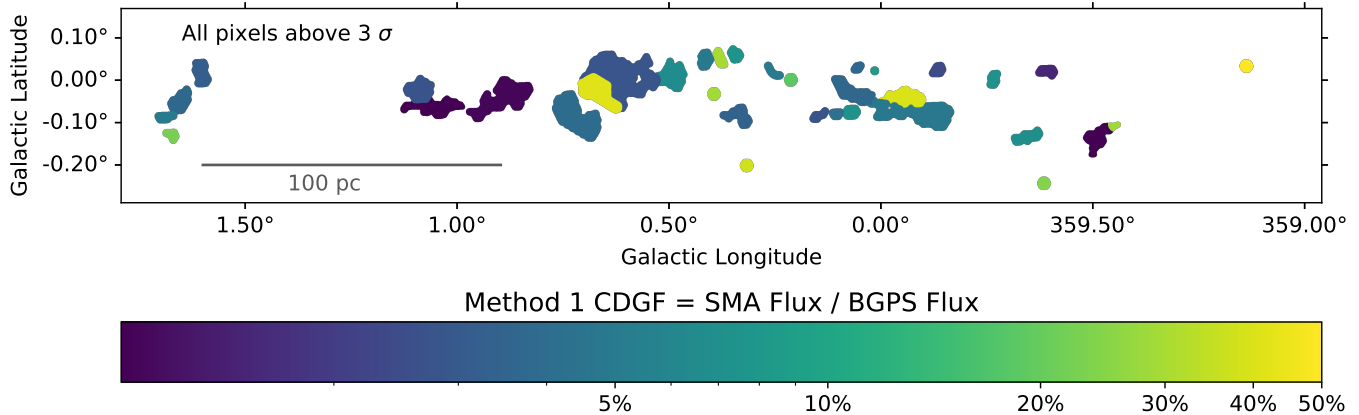
Figure 9. The method 1 compact dense gas fraction (CDGF), as measured by comparing the SMA-only (interferometer) and BGPS (single-dish) total flux in each cloud. This map shows the total SMA flux divided by the total BGPS flux in each cloud above 3\sigma . This figure highlights that the vast majority of gas in the CMZ (as measured by BGPS dust emission) is not in compact, dense cores of a few tens of parsecs in size (as measured by the SMA dust emission). Most clouds in the CMZ have CDGFs below 10%. Note that the apparently high CDGF seen toward the CND, located near \ell = 0^\circ , is likely due to contamination from the strong synchrotron source Sgr A* and resulting imaging artifacts (see Section 5.4 for more details). The CND is removed from the remaining CDGF plots.
