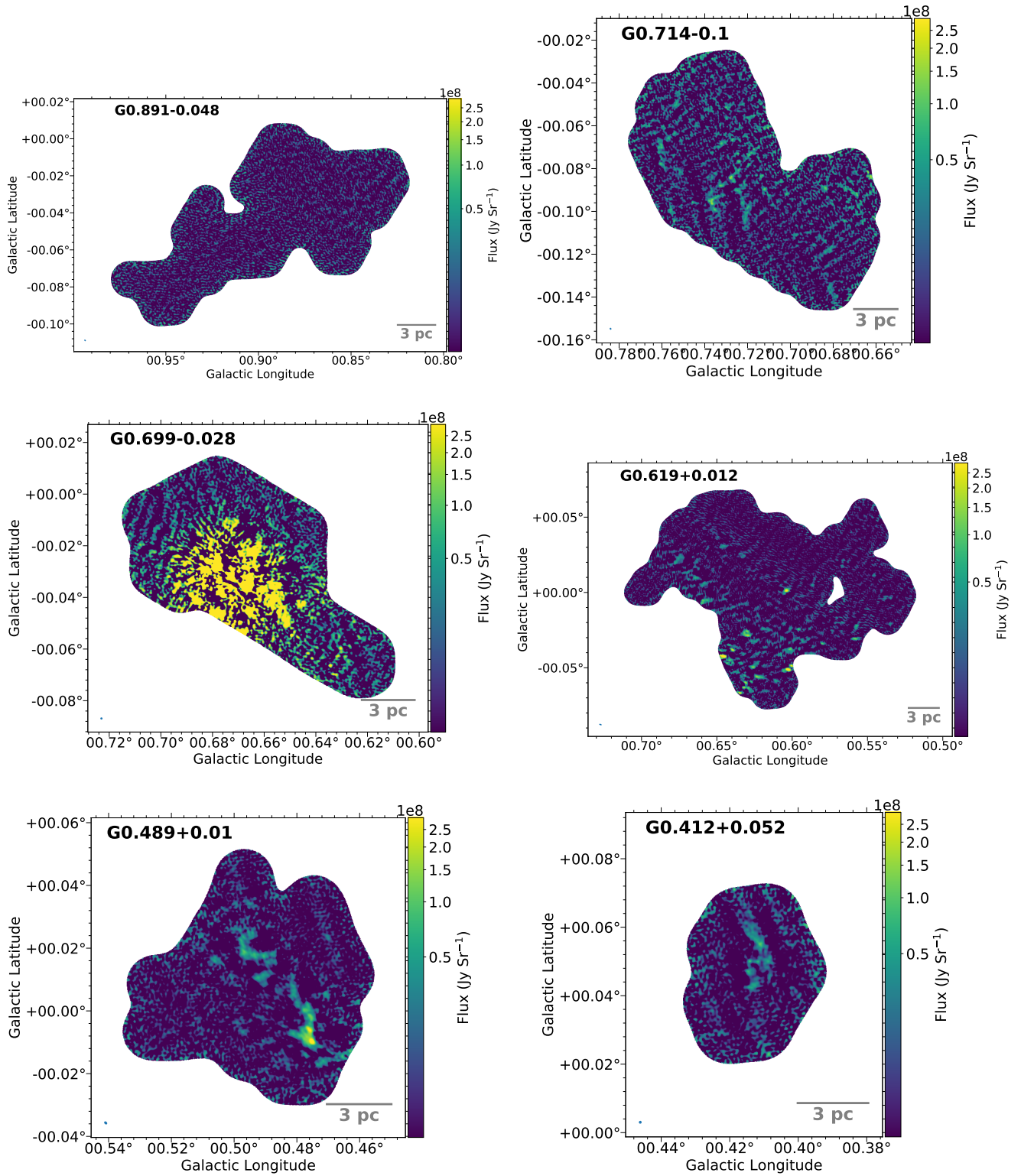
Figure 15. Images show the 1.3 mm dust continuum from the CMZoom Survey with a 3 pc scale-bar. The white contour shows the approximate 5\text{-}\sigma level while the black contour shows the approximate 10\text{-}\sigma level. All the images are displayed on same color scale from 2 - 290 \text{MJy Sr}^{-1} .
