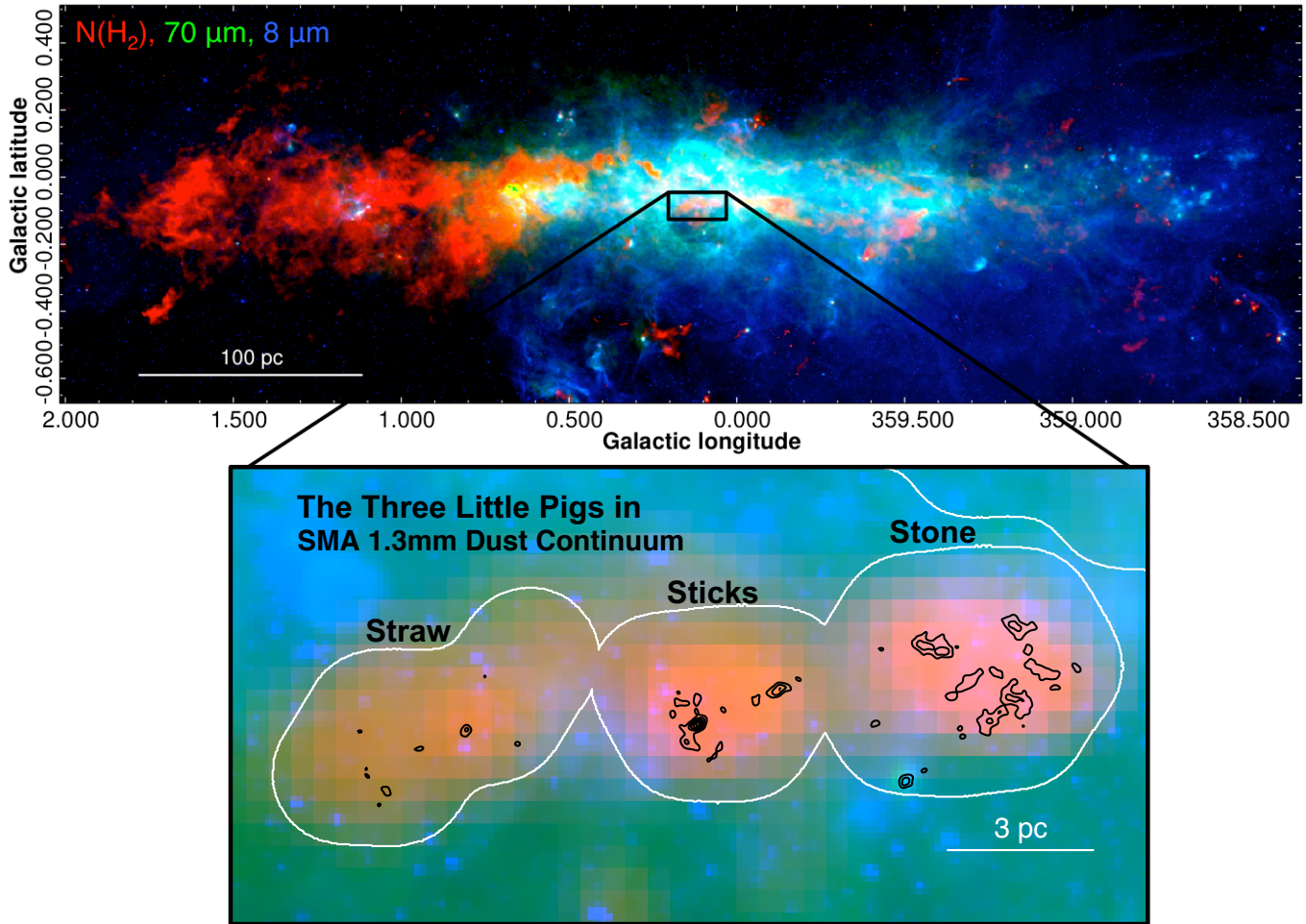
Figure 6. A three-color image of the CMZ, as seen with Herschel in N(H 2 ) (from Molinari et al. 2010, Battersby et al. in prep.) in red, 70 μm (Molinari et al. 2010) in green, and Spitzer GLIMPSE 8 μm (Benjamin et al. 2003) in blue. The lower-panel is a zoom-in toward three clouds dubbed the “Three Little Pigs.” In previous single-dish data, the clouds have similar column densities, masses, temperatures, and sizes, however, the detailed structure seen with the SMA dust continuum (shown as the four black contour levels at 2, 4, 6, and 8 σ) tells a different story. From left to right, the clouds increase in their levels of substructure, from the ‘Straw Cloud’ on the left, with very little substructure, to the ‘Sticks Cloud’ in the middle with moderate substructure, and finally to the ‘Stone Cloud’ on the right, with the most substructure.
