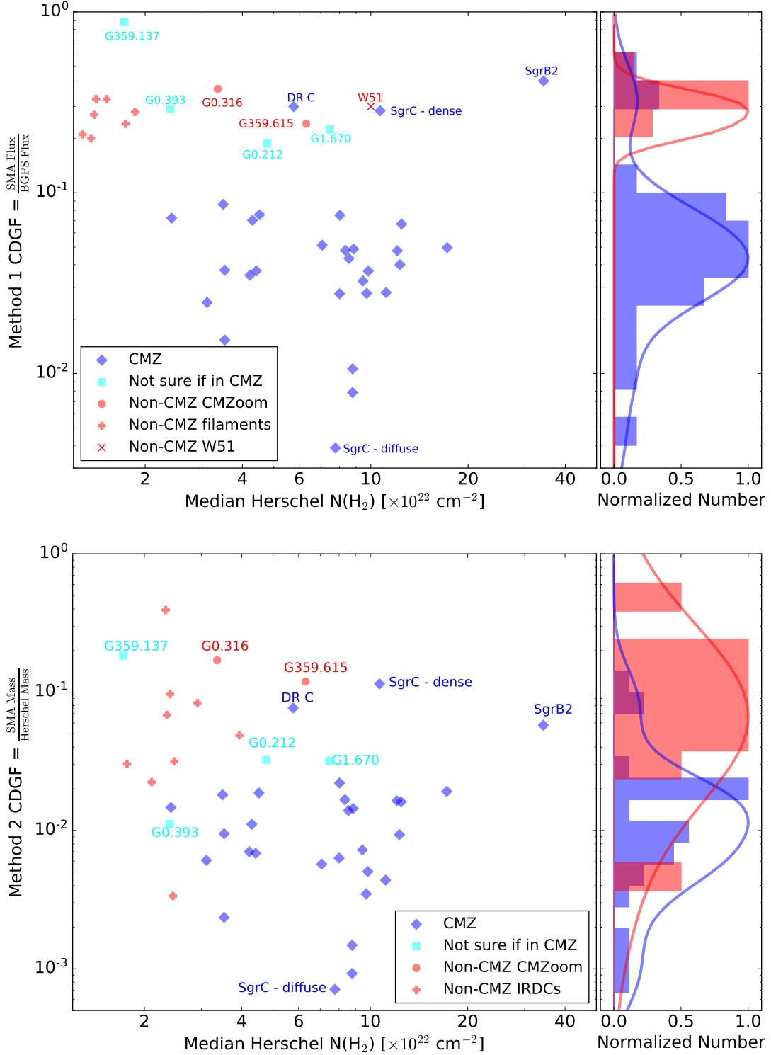
Figure 12. Clouds in the CMZ overall have a much lower compact dense gas fraction (CDGF), with the exception of highly star-forming Dust Ridge Cloud C, SgrC - dense, and SgrB2, than clouds in the Galactic disk, despite their high average column densities. This figure shows the method 1 CDGF (SMA flux divided by BGPS flux) vs. the median Herschel column density for each cloud on the top with the method 2 CDGF (SMA mass divided by Herschel mass) in the bottom panel. The right panel of each plot shows the histogram of CMZ (blue) and non-CMZ (red) data points with a Kernel Density Estimator fit. Clouds marked with a dark blue diamond are located within the CMZ, those marked with cyan squares are not definitively inside or outside of the CMZ (see Section 5.2), and those marked as red circles, plus signs, or an x are not in the CMZ. The Non-CMZ data points are discussed in 5.3. While we tried to measure the CDGF and median column density for the non-CMZoom points in the same way, we advise a factor of two uncertainty in the interpretation of the relative data points (see Section 5.3).
