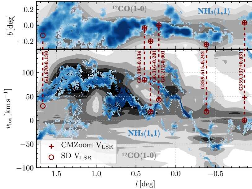
Figure 11. The location of the potential foreground sources, G1.670–0.130, G0.393–0.034, G0.316–0.201, G0.212–0.001, G359.615–0.243, and G359.137+0.031, on a longitude-latitude and longitude-velocity plot of the CMZ. The gray data are CO from Dame et al. (2001) and the color points are the 3-D locations of Gaussian fit centroids to \text{NH}_3(1,1) data from The \text{H}_2\text{O} Southern Galactic Plane Survey (HOPS; Walsh et al. 2011; Purcell et al. 2012; Longmore et al. 2017), fit using SCOUSE from Henshaw et al. (2016). The circles indicate the measured peak single-dish velocity of the region and the plus sign indicates the CMZoom preliminary peak velocity of the region as described in detail in Section 5.2 and summarized in Table 3.
