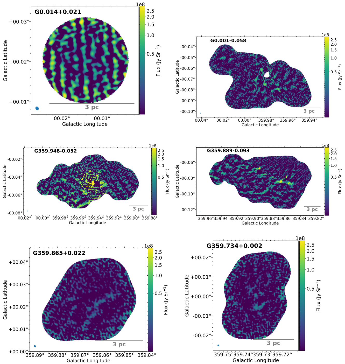
Figure 18. Images show the 1.3 mm dust continuum from the CMZoom Survey with a 3 pc scale-bar. The white contour shows the approximate 5\text{-}\sigma level while the black contour shows the approximate 10\text{-}\sigma level. All the images are displayed on same color scale from 2 - 290 \text{MJy Sr}^{-1} .
