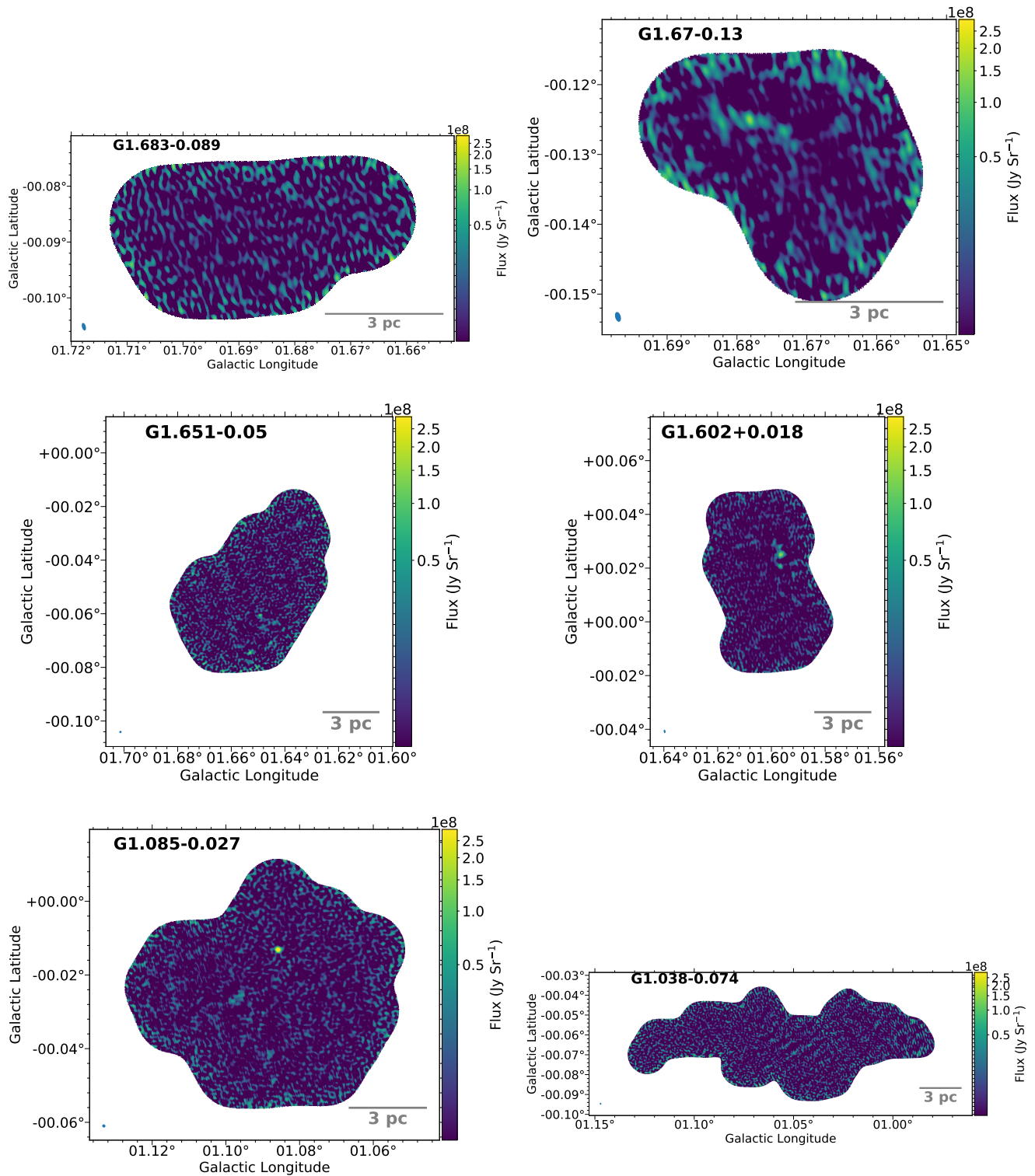
Figure 14. Images show the 1.3 mm dust continuum from the CMZoom Survey with a 3 pc scale-bar. The white contour shows the approximate 5- \sigma level while the black contour shows the approximate 10- \sigma level. All the images are displayed on same color scale from 2 - 290 MJy \text{Sr}^{-1} .
