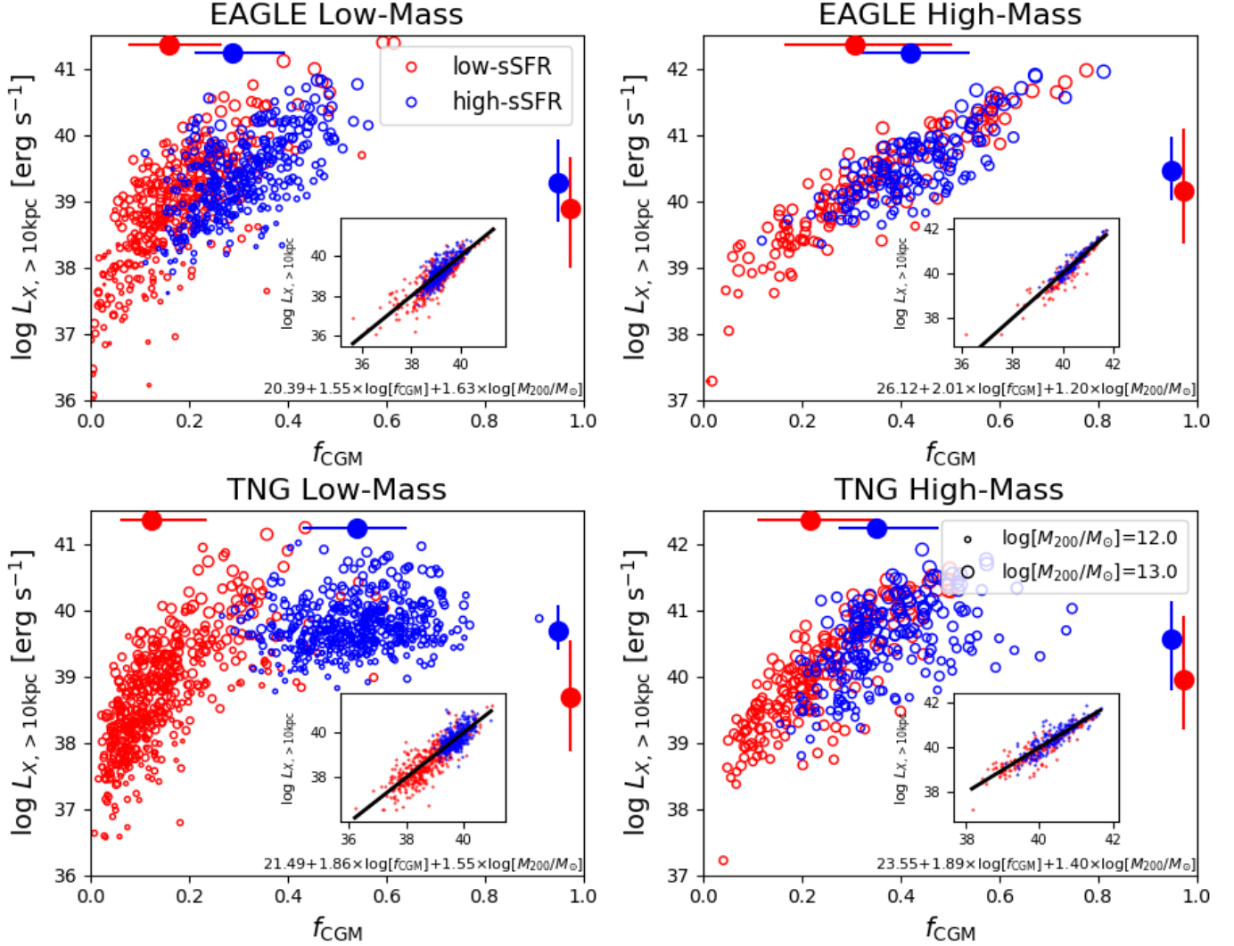
Figure 4. Extended ( r > 10 kpc) X-ray emission as a function of CGM mass fraction ( f_{\text{CGM}} ) divided into high and low-sSFR galaxies for low-mass (left panels) and high-mass (right panels) EAGLE (upper panels) and TNG (lower panels) halos. Median and 1\sigma spreads are indicated by large points with error bars. High-sSFR galaxies reside in halos with higher gas fractions than low-sSFR galaxies, with this trend being most pronounced for low-mass TNG galaxies. Extended X-ray luminosity is strongly correlated with f_{\text{CGM}} and is also dependent on M_{200} as indicated by symbol size. f_{\text{CGM}} equals unity for a halo that retains the cosmic proportion of baryons entirely in the CGM (see Eq. 1). Inset panels show two-parameter linear regressions indicating the combinations of \log[f_{\text{CGM}}] and \log[M_{200}/M_{\odot}] that best reproduce \log[L_{X, > 10\text{kpc}}] (equations below inset x-axes, black lines represent fits).
