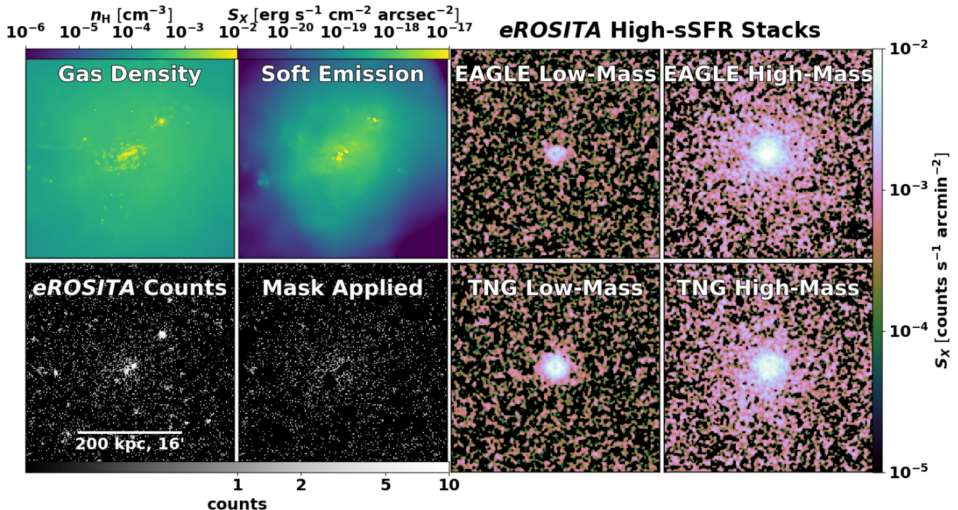
Figure 1. Left 4 panels: An EAGLE M_{200} = 10^{12.58} M_{\odot} halo hosting M_{*} = 10^{10.73} M_{\odot} star-forming, late-type galaxy. The density (upper left) and soft (0.5–2.0 keV) X-ray emissivity (upper right) are shown in 400 \times 400 kpc snapshot images. A mock z = 0.01 eROSITA count map is generated (lower left) and point source-like objects are masked, including CXB sources, the prominent satellite in the upper right, and emission on top of the galaxy, leaving behind an extended halo (lower right). This halo is brighter than typical, L_{X, > 10 \text{ kpc}} = 10^{41} \text{ erg s}^{-1} , and most halos do not show individually detectable emission. Right 4 panels: Mock eROSITA stacks of high-sSFR galaxies, including stacks of 100 low-mass galaxies (left panels) and 50 high-mass galaxies (right panels) for EAGLE (upper panels) and TNG (lower panels). These panels also span 400 \times 400 kpc.
