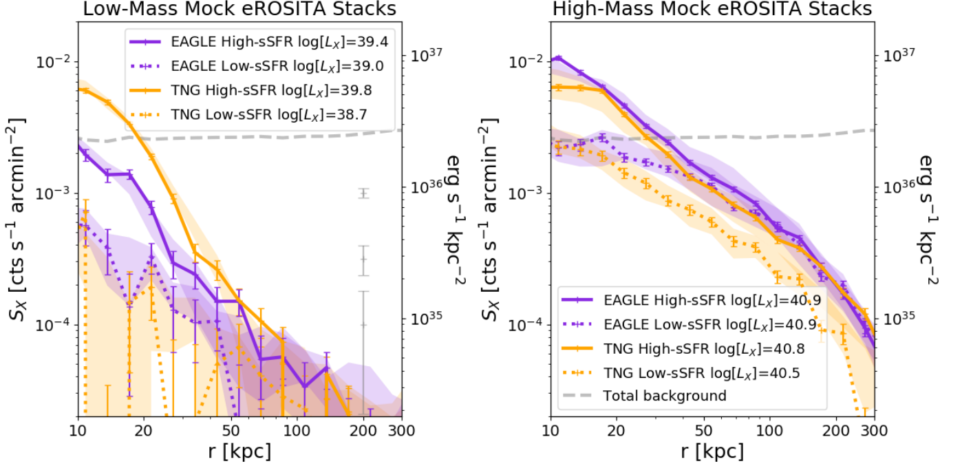
Figure 2. Simulated eROSITA 4-year of mean soft X-ray surface brightness profiles around low-mass (left) and high-mass (right) halos in EAGLE and TNG. Colored lines indicate one mock survey of 100 low-mass and 50 high-mass z = 0.01 galaxy stacks with Poisson error bars, which should be reproducible with half the all-sky survey. Shading indicates 1\sigma spreads from 20 mock surveys. Average L_{X,>10\text{kpc}}/\text{erg s}^{-1} values calculated from the stacks are listed in the legend. Both simulations predict brighter X-ray halos around higher sSFR galaxies. TNG predicts a greater dichotomy at low mass, and EAGLE predicts brighter halos overall at high mass. eROSITA should enable detection of star-forming galaxy halos out to 30 – 50 kpc around low-mass galaxies and of all halos out to 150 – 200 kpc around high-mass galaxies. The total astrophysical and instrumental background is indicated by the gray dashed lines. We plot example error bars in gray indicating 3% of the background level in the left panel to demonstrate the effect of possible systematic errors.
