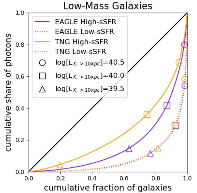
Figure 3. Low-mass z = 0.01 galaxy samples are rank-ordered by soft X-ray photon counts outside r = 10 kpc to demonstrate the relative share of extended emission arising from different galaxies within each stack. The black line demonstrates a completely equal distribution. High-sSFR X-ray halos are distributed more uniformly than low-sSFR halos. Symbols indicate the fraction of galaxies with extended luminosities fainter than the values listed in the legend. Deep eROSITA observations of individual halos will be able to complement stacking observations by constraining the upper portions of these curves.
