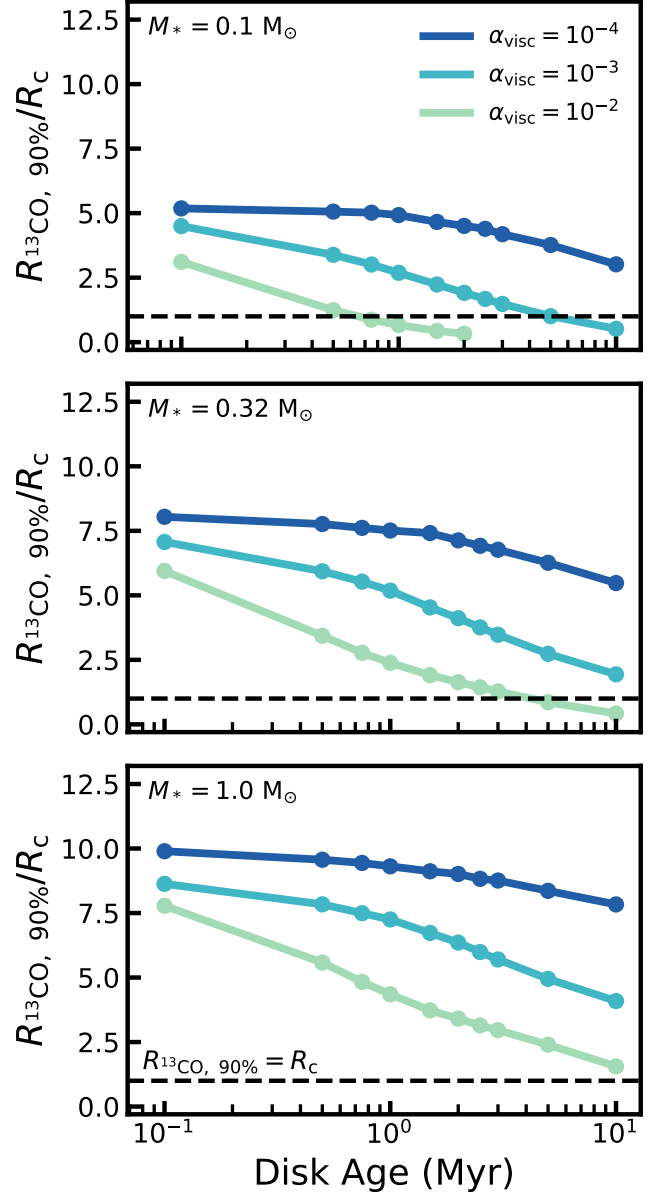
Fig. C.3: The ratio of gas outer radius ( R_{^{13}\text{CO}} ) over characteristic radius ( R_c ) vs. disk age. Gas outer radii are measured from ^{13}\text{CO} 2-1 emission of our models. The black dashed line indicates where R_{^{13}\text{CO}} = R_c . Top, middle and bottom panels show models with different stellar masses. Colors represent models with different \alpha_{\text{visc}} .
