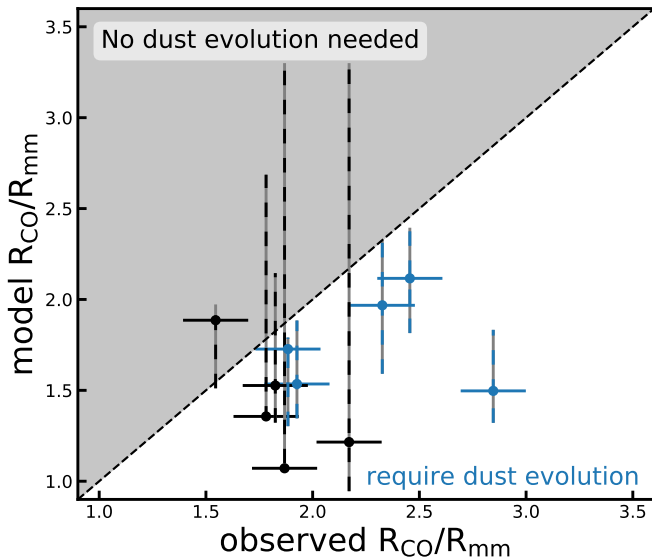
Fig. 5: Disk gas–dust size ratio comparison of the models with noise and the observations. Uncertainties of the model R_{\text{CO}, \text{mdl}}/R_{\text{mm}, \text{mdl}} were computed using the 16 th and 84 th quantile of the R_{\text{CO}} distribution. Sources where R_{\text{CO}, \text{mdl}}/R_{\text{mm}, \text{mdl}} < R_{\text{CO}, \text{obs}}/R_{\text{mm}, \text{obs}} are shown in blue. To reproduce the observed R_{\text{CO}, \text{obs}}/R_{\text{mm}, \text{obs}} these sources require a combination of dust evolution and optical depth.
