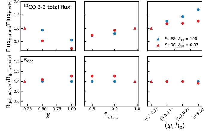
Fig. B.1: Effects of vertical structure and the large grains. Top panels: Integrated ^{13}\text{CO} flux as function of large grain settling ( \chi ), fraction of large grains ( f_{\text{large}} ) and disk vertical structure ( h = h_c(R/R_c)^\psi ). The models for Sz 98 and Sz 68 are shown in red and blue respectively. Triangle markers denote the value used in the rest of this work (cf. Sections 3.2.1 and 3.2.3). Bottom panels: As top panels, but showing the variations of the gas outer radius R_{\text{CO}} .
