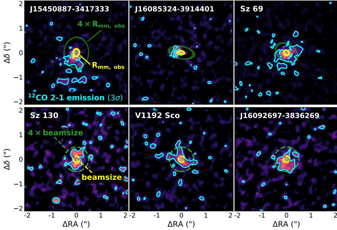
Fig. 6: ^{12}\text{CO} moment-zero maps of the six sources from the “low S/N sample” (see Section 5.1) where the \text{S/N} = 3 contour of their ^{12}\text{CO} emission, shown in cyan, reaches beyond 4 \times R_{\text{mm}} . Using this contour as a proxy for R_{\text{CO}} , these disks likely have R_{\text{CO}}/R_{\text{mm}} \geq 4 and are therefore clear candidates for having undergone dust evolution (cf. Trapman et al. 2019). The top three disks have resolved continuum emission and their R_{\text{mm, obs}} is shown by the yellow ellipse. For these sources, Keplerian masking was applied to the ^{12}\text{CO } J = 2 - 1 emission (see Appendix A). The bottom three disks have unresolved continuum emission. The dashed yellow circle shows the size of the beam ( 0''.25 ) as an upper limit to the dust disk size. Similarly, the dashed green circle shows four times the beam size.
