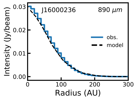
Fig. 2: Example comparison between model and observed 890\ \mu\text{m} continuum intensity profile for J16000236-4222115. Similar comparisons for the other disks can be found in Figure C.1.
