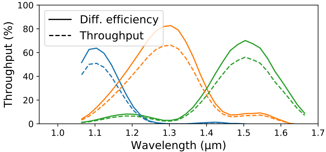
Fig 11 The measured diffraction efficiency and throughput of the spectrograph without the fiber link as measured by the Tunable Laser Source. The solid lines show the diffraction efficiency of the stacked VPHG system. The dashed lines include the throughput of the spectrograph optics.
