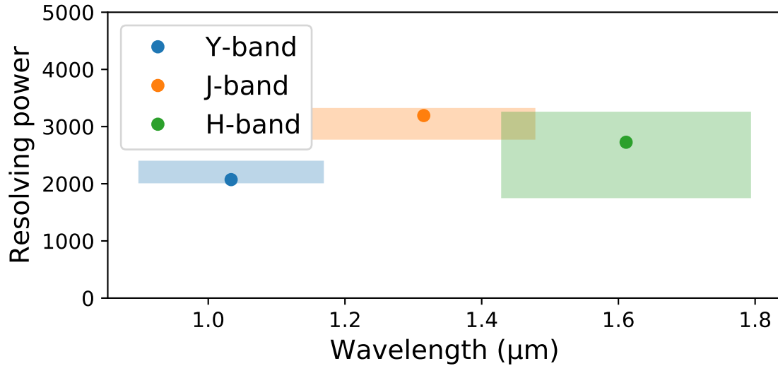
Fig 13 The measured resolving power of the MCIFU for the three different spectral orders. The shaded area shows the 1-\sigma resolving power estimates from several emission lines within each order. The points in each area show the median resolving power of that order. The H-band resolving power has a large spread due to line blending of many of the measured lines. The estimated resolving power is a factor 2 to 3 lower than the theoretical limit.
