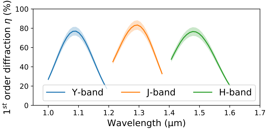
Fig 7 Simulation of the combined diffraction efficiency of the multiplexed VPHG for an incidence angle of 21.5^\circ for unpolarized light. The shaded area present the minimum and maximum diffraction efficiency prediction for the manufacturing process. Material absorption and reflection losses have been estimated and taken into account.
