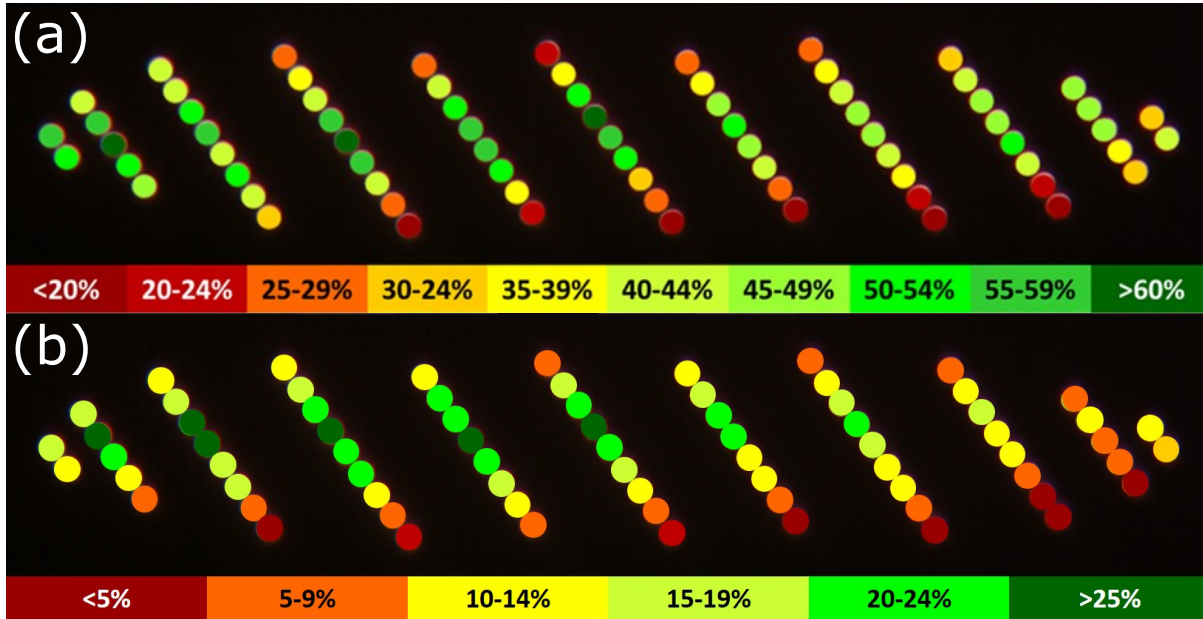
Fig 4 Illustration of the measured monochromatic (1310 nm) throughput results for the fiber link. (a) shows the throughput for the 73 individual cores through the fiber, the reformatter and the chromium mask. (b) as for (a) but for the full fiber link, including the microlenses. The colour bars represents the throughput ranges for each figure.
