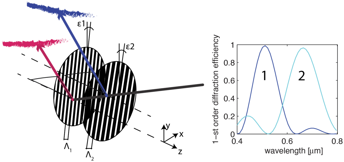
Fig 6 Scheme of the spectral-multiplexing concept. For simplicity a two-stacked VPHG is presented, each creating a separate spectrum which are shown in different colours. The inset shows the simulated diffraction efficiencies of the two layers for an example design.
