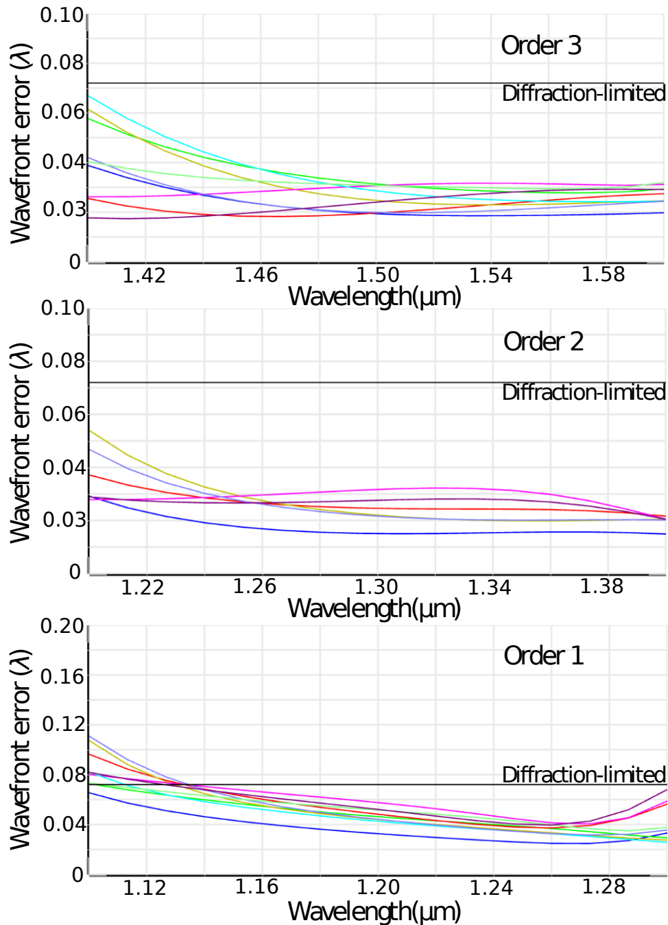
Fig 8 The wavefront quality of the spectrograph as function of wavelength for the three different orders that are made by the VPHG. The various colors represent a position along the pseudo-slit, and are the same pseudo-slit position for each order. Here we can see that the spectrograph design is diffraction-limited over almost the full spectral bandwidth. Only the blue part of the Y-band is slightly non diffraction-limited, which will lower the effective resolving power.
