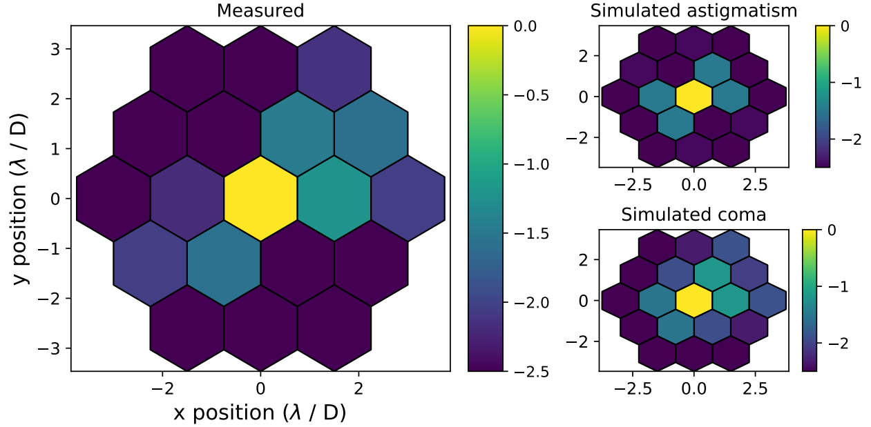
Fig 15 The monochromatic post-fiber contrast map on a logarithmic scale as measured with a 1550nm laser (left). A comparison of the asymmetry in the illumination with simulations (right) hints on the presence of 0.5 radians rms residual astigmatism and/or coma.
