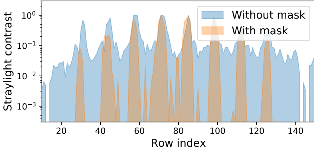
Fig 3 A slice along one of the rows of the reformatter showing the scattered light with and without the chromium mask. Here, the input microlens array is overfilled, specifically to simulate background light in astronomical observations. The blue shaded area, shows where the scattered light is still detectable between the waveguides, the red shaded area shows the stray light with the mask. The row index is the pixel index along the extracted slice.
