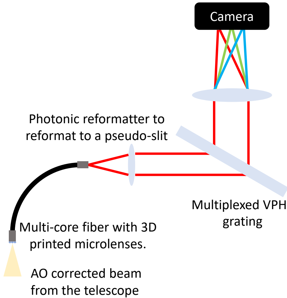
Fig 1 An overview of the multi-core integral field unit (MCIFU). The telescope beam is imaged onto a microlens array that is written on top of a multi-core fiber. The output of the multi-core fiber is rearranged into a pseudo-slit by the photonic reformatter to make it dispersable. And finally a triple multiplexed grating is used to disperse a broad wavelength range into three orders at a resolving power higher than R = 5000 . The spectrograph itself is used in a first-order manner, where a lens is used to collimate the light onto a grating and a second lens is used to image the spectrograph focal plane.
