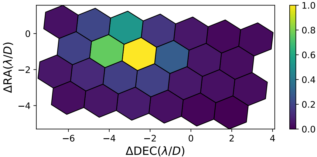
Fig 18 The on-sky reconstructed H-band image, using the MCIFU, of the bright star Alpha Herculis. The observations were taken at 10Hz. The image shown here are is the mean of 1000 successive images from the data stream. Each micro-lens samples roughly 1.3 \lambda/D . The asymmetry in the PSF comes from a slow drift in tip/tilt alignment during the observations.
