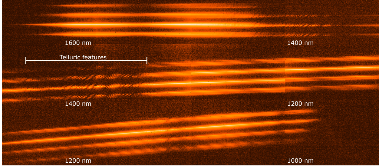
Fig 16 The full spectrograph output of Vega after stitching 12 detector positions together. The color of the image is logarithmically stretched to highlight the spectra from the fainter fiber cores. Each fiber captures a different part of the PSF at the input, therefore the brightness of the spectral trace corresponds with the brightness of the captured part of the PSF. The main features that are visible are the telluric lines imprinted into the spectrum of Vega. Abrupt changes in the continuum of the individual cores are visible because the full image was reconstructed from 12 observations that were taken one after another, with varying conditions. The beginning and end of each spectrum has been marked with the corresponding wavelength.
