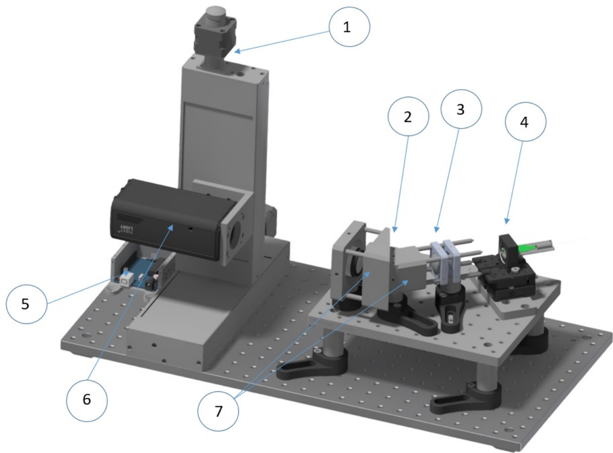
Fig 10 Mechanical design of the spectrograph from the reformatter to the camera: 1) Motorized stages, 2) Dispersing element, 3) Collimating Optical elements, 4) Reformatter holder, 5) Arduino control components, 6) C-RED 2 camera, 7) 3D printed elements.
