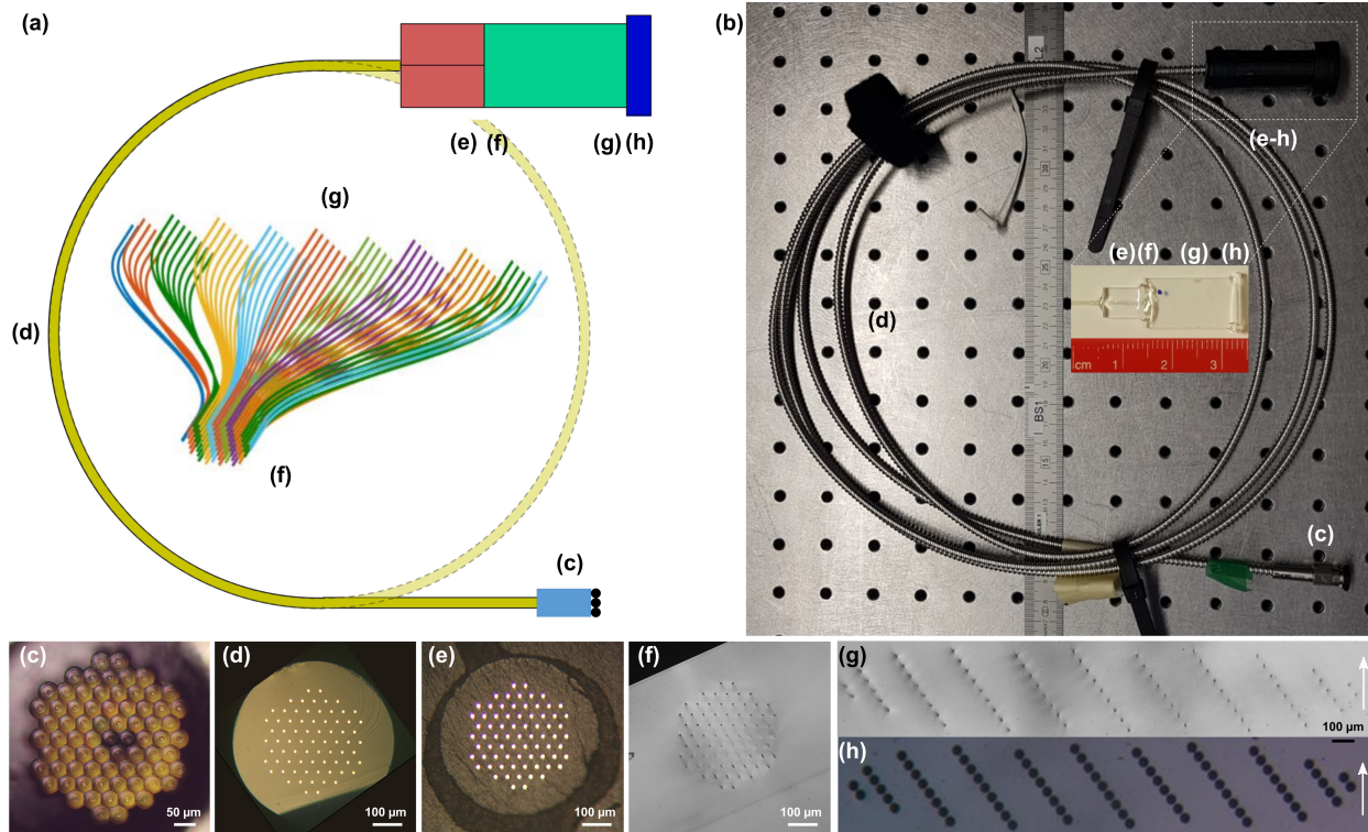
Fig 2 The MCIFU fiber link, with important sections shown. (a) A schematic representation of the fiber link, (b) photograph of the complete packaged fibre-link comprising all the elements from the microlens array, (c) the 3D printed microlenses, (d) the bare fiber, (e) the bare fiber in a v-groove, (f) the input of the chip reformatter. (g) The output of the reformatter (h) The output mask. The white arrow in (g/h) indicates the dispersion direction. Inset in (b): scale picture of the full reformatter.
