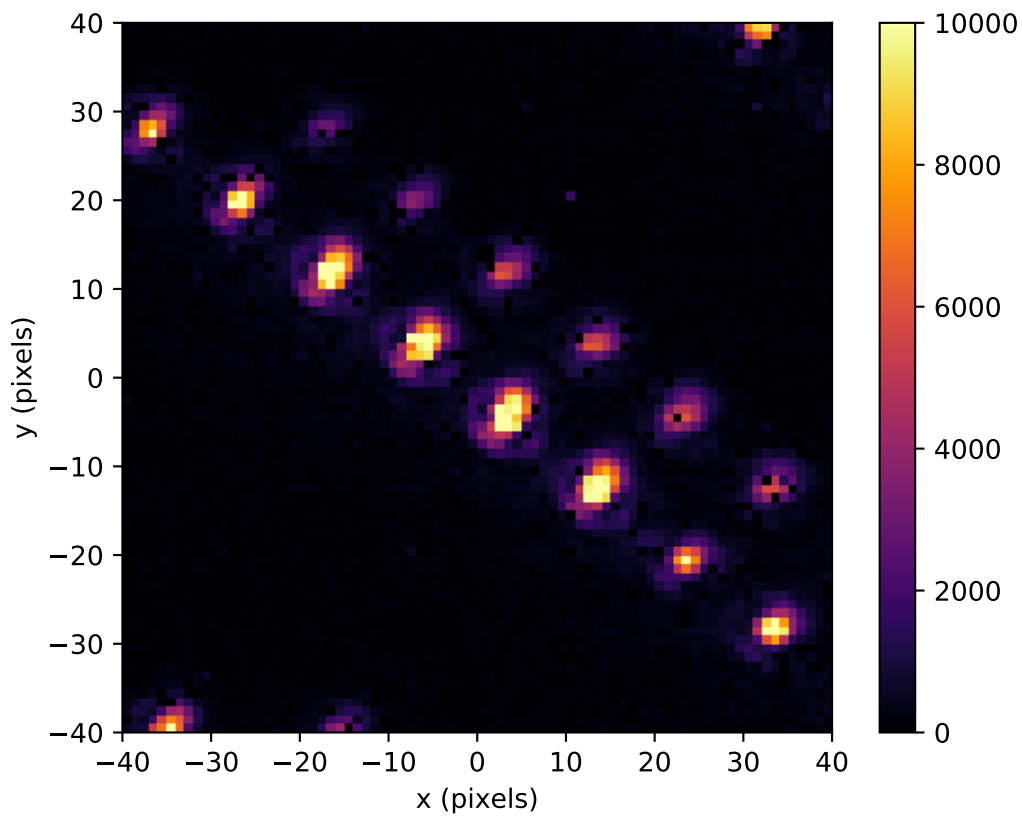
Fig 14 The PSFs of the spectrograph as measured with the Kr spectral calibration lamp. The horizontal axis is the dispersion axis. The diagonal array of PSFs is the output of a single emission line illuminating a single row of the reformatter. The PSFs are extended and asymmetric towards the north-east and show a clear Airy ring.
