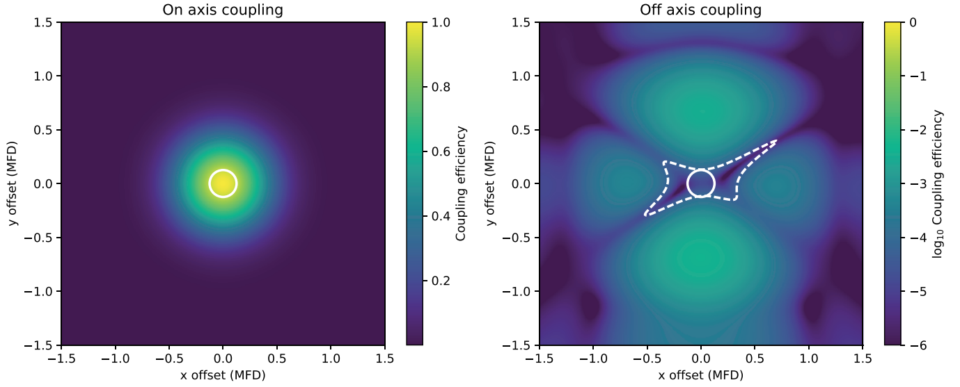
Fig. 9. Left panel: throughput of an on-axis source as function of fiber misalignment. Right panel: off-axis contrast as function of misalignment. The white contour encircles the area where the contrast is below 1 \times 10^{-4} . The white circle is the largest circle that fits within the contour with a radius of 1/8th of the mode field diameter.
