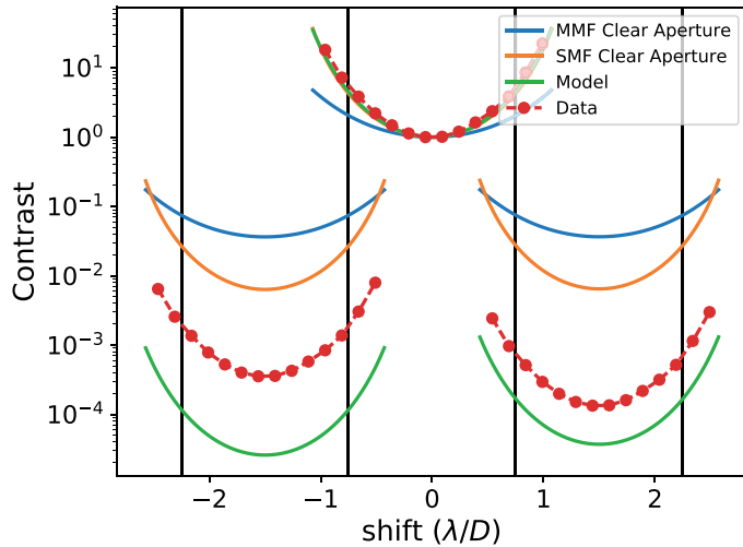
Fig. 5. Contrast as a function of position on the microlens array. The black lines show the borders of the microlenses. The blue lines show the contrast for a multi-mode fiber. The orange lines show the contrast for a single-mode fiber. A single-mode fiber already provides extra contrast compared to a multi-mode fiber. The green lines show the model of the SCAR coronagraph, and the red dots are the measurements.
