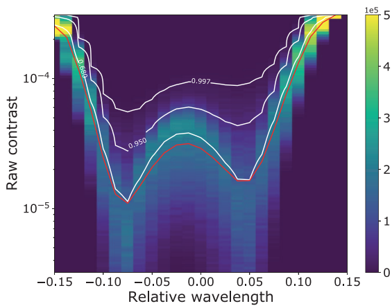
Fig. 11. Results of the Monte Carlo tolerance analysis as function of wavelength. The red curve shows the expectation value of the contrast. The white curves are the 0.68, 0.95 and 0.997 percentile confidence limits. The analysis indicates that within specified tolerances a contrast below 1 \times 10^{-4} can be reached over a 15 percent bandwidth. Within the full 20 percent bandwidth the contrast is below 2 \times 10^{-4} .
