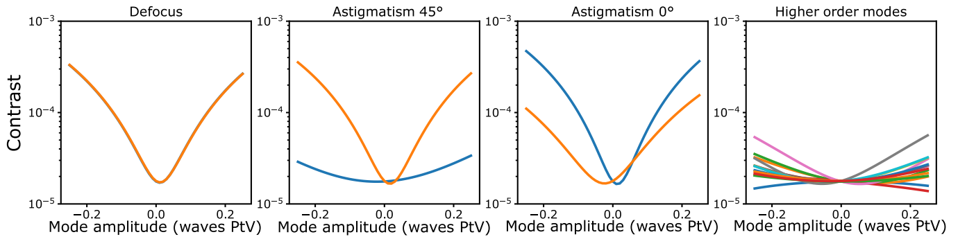
Fig. 10. Effect of wavefront errors in the microlenses on the contrast due to a certain Zernike mode. First three panels: effects on two different fibers. Due to symmetry the other four fibers behave in the same way as these two. The radial symmetry of the defocus mode causes the same effect in all fibers, therefore the curves of the two fibers overlap. Rightmost panel: effects of Zernike modes 6 to 10. Focus and astigmatism are the most dominant wavefront errors for lowering the contrast.
