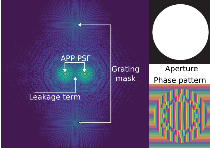
Fig. 3. Left: simulated focal plane of the phase pattern. Right: phase and aperture. On the focal plane several PSF's can be seen. The left and right PSFs are the PSFs that contain the phase pattern. The top and bottom correspond to the light that scatters away due to the grating mask. And in the center there is a 1 percent leakage term. The horizontal PSFs are at \pm 10\lambda/D and the aperture PSFs are at \pm 50\lambda/D
