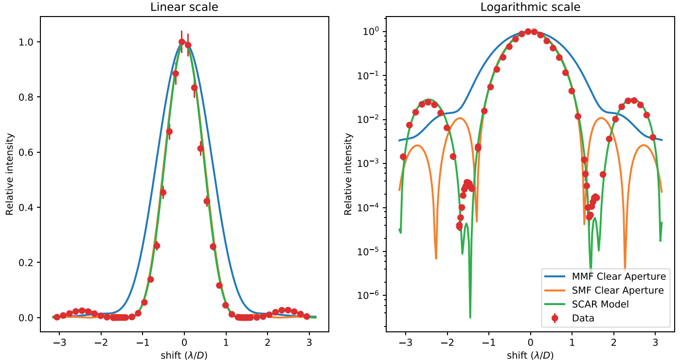
Fig. 4. Left panel: relative throughput on a linear scale as function of relative shift with respect to the microlens center. The red points are the measurements with errorbars due to random errors. The green line shows the model of this SCAR design. Right panel: throughput on a logarithmic scale. The null is uneven between left and right and not as deep as designed. This is suspected to be caused by 10 nm rms residual low-order aberrations. The blue line shows the amount of light that falls on the microlens with a clear aperture and without SCAR. This is comparable to the contrast curve for normal imaging or using a multi-mode fiber. The orange line shows the normalized throughput with a unobstructed aperture and a SMF. The SMF shows a gain compared to the MMF.
