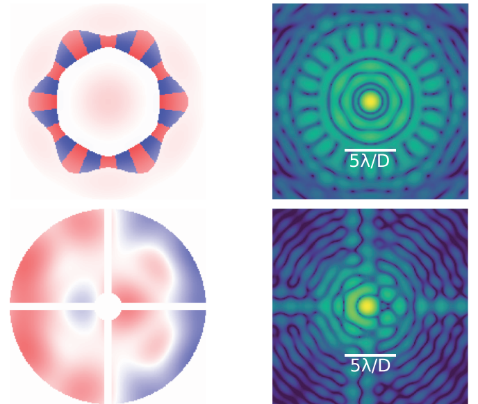
Fig. 2. Left column shows theoretical phase pattern. Here blue is \pi phase, white is zero phase and red is -\pi phase. The corresponding PSF is shown on the right with a 5 \lambda/D scale bar. Both images of the PSF are on log scale with the color scale shown on the right. The first phase pattern creates a 360 dark region for a clear aperture. The second pattern creates a one-sided dark region for a pupil that has a central obscuration and spiders.
