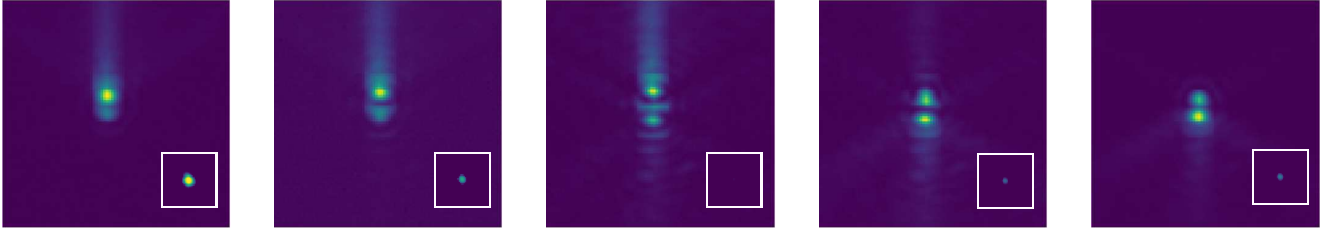
Fig. 6. Measured microlens spot structure for the 360 SCAR. The inset shows the throughput of the single mode fiber. The deepest null occurs with a triple spot structure, which is a second order null due to the two zero crossings. The white circle shows the position and MFD of the fiber.
