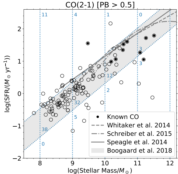
Figure 3. SFR- M_* relation of our CO(2-1) stacking sample. The gray filled band shows the main-sequence relation and its intrinsic scatter for MUSE-detected galaxies (at z = 1.43 , Boogaard et al. 2018). The gray solid, dashed and dashed dotted lines are the main-sequence relations from Speagle et al. (2014) (which is used for PHIBSS2 Tacconi et al. 2018, see also Appendix D), Whitaker et al. (2014) and Schreiber et al. (2015), respectively. The blue vertical and diagonal dotted lines show the divisions of the bins that we used for stacking. The numbers at the top left of each grid are the counts of galaxies in the bin. The filled circles indicate the galaxies which have CO(2-1) line detections in the ASPECS blind search (see §3.2).
