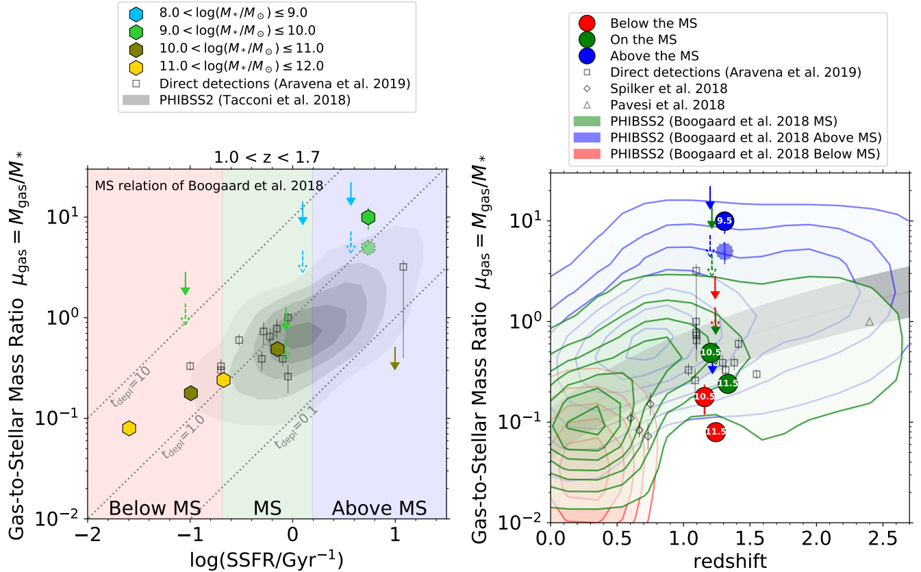
Figure 6. [Left] Gas-to-stellar mass ratios as a function of SSFR. The symbols are the same as in Figure 5, but now we show the entire sample, below, on, and above the main-sequence relation, color-coded with their stellar masses as indicated in the legend. The same as the other figures involving molecular gas mass estimates, we use \alpha_{\text{CO}} = 3.6 M_{\odot} (\text{K km s}^{-1} \text{pc}^2)^{-1} for galaxies in the \log(M_*/M_{\odot}) > 10 bins and 7.2 and 10.8 for the \log(M_*/M_{\odot}) \sim 9.5 and 8.5 bins, respectively (see §5.1). We also show the estimates based on a constant \alpha_{\text{CO}} = 3.6 M_{\odot} (\text{K km s}^{-1} \text{pc}^2)^{-1} in the lower mass bins with the dashed symbols for reference. The data points are centered on the mean values of the parameters on the x-axis. The three diagonal gray dotted lines represent constant depletion time scales of 0.1, 1.0, and 10 Gyr from the bottom to the top. The background pink, green, and blue filled colors indicate the below, on, and above the main-sequence relation of Boogaard et al. (2018) for a galaxy at \log(M_*/M_{\odot}) = 10.0 . A version using the main-sequence relation of Speagle et al. (2014) is shown in Appendix D. [Right] The evolution of gas-to-stellar mass ratios. The symbols are the same as Figure 5 but now we include galaxies above and below the main-sequence relation: above (blue), below (red), and on the MS relation (green). The values inside each symbol indicate the corresponding stellar mass bins in log scale. The PHIBSS2 galaxies classified as above, below, and on the MS by the main-sequence relation of Boogaard et al. (2018) are also depicted as red, green, and blue contours, respectively. The gray curve in the background and its shaded region show the evolutionary track of main-sequence galaxies from Tacconi et al. (2018).
