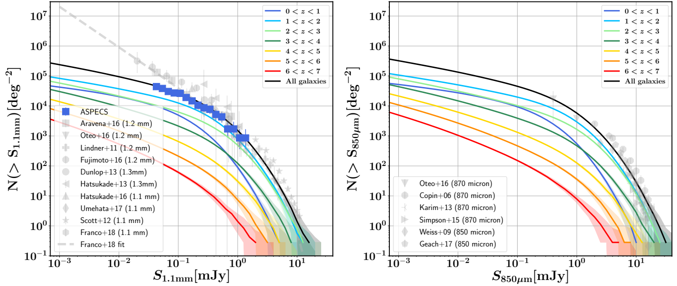
Figure 3. The 1.1 millimeter (left) and 850 \mu\text{m} (right) galaxy number counts. The black solid lines mark our predictions for the number counts when accounting for all the galaxies in the lightcone (as shown in Fig. 1). The coloured lines mark the number counts when selecting galaxies based on their redshift. The color shading corresponds to the two-sigma scatter when sampling over the intrinsic scatter of the empirical scaling relations. The model predictions are compared to a literature compilation of number counts as in Fig. 1. The 1.1 mm number counts are dominated by galaxies at z=1-2 , with additional contributions from galaxies up to z=3 at the brightest fluxes and galaxies in the range z=0-1 at the faintest fluxes.
