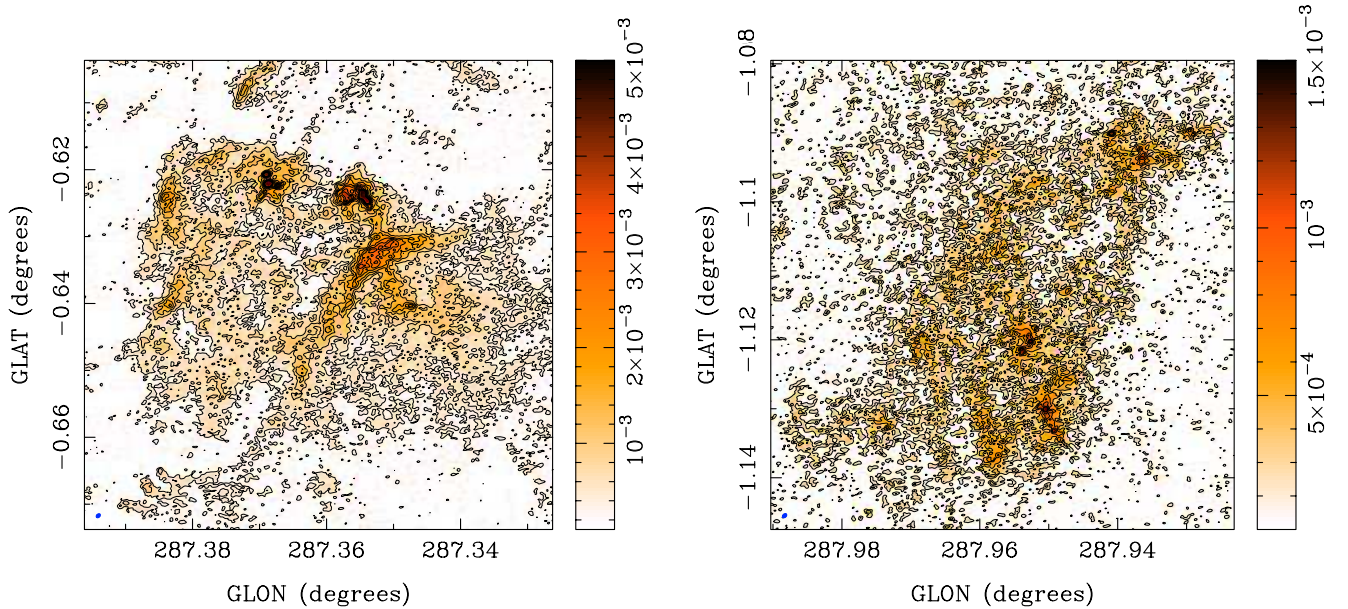
FIG. 16.— Continuum images resulting from the combination of ALMA and APEX data from ATLASGAL survey. The left panel shows the NC while the right panel shows the SP region. The color bar is in Jy/beam. The contours are given by 2 \times k \times \sigma_{\text{rms}} , where k = 1, 2, 3, 4, 5, 6 . We clearly see a recovery of the more diffuse emission which was filtered out by ALMA interferometric observations. Our sensitivity limit defined as 2 \times \sigma_{\text{rms}} is closed in our maps.
