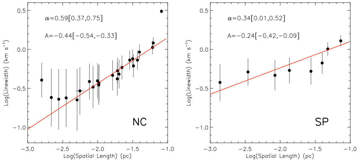
FIG. 14.— The Linewidth vs. Spatial Length relationship derived from \text{HCO}^+ data for the NC (Left) and SP (Right) using the PCA technique implemented in the TURBUSTAT python package. The red lines show the fitted power law generated by the Bayesian regression fit method for each region. The red lines are constructed by using the peak values of the parameter distributions shown in Figure 15. In the case of the NC, the outliers are removed from the fit. For each parameter, the peak value is shown, with the 90% HDI range in brackets.
