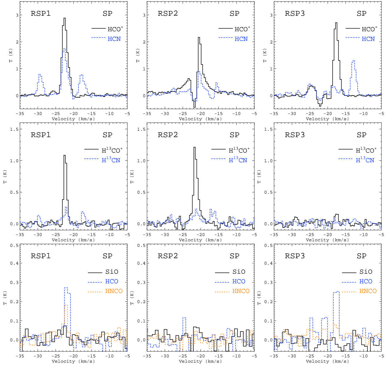
FIG. 8.— Average spectra of the detected lines towards three representative regions in the SP. The regions, RSP1, RSP2 and RSP3 are shown in Figure 4. As in NC, the brightest lines are the HCN and \text{HCO}^+ . In addition, HCN hyperfine structure are detected in all the regions. RSP2 and RSP3 present self-absorption features at -22 \text{ km s}^{-1} in both HCN and \text{HCO}^+ . In RSP3, we observe a total suppression of the main line of HCN but the hyperfine lines are still detected. On the other hand, \text{H}^{13}\text{CN} and \text{H}^{13}\text{CO}^+ are not detected in RSP3, but weak emission of HCO is observed.
