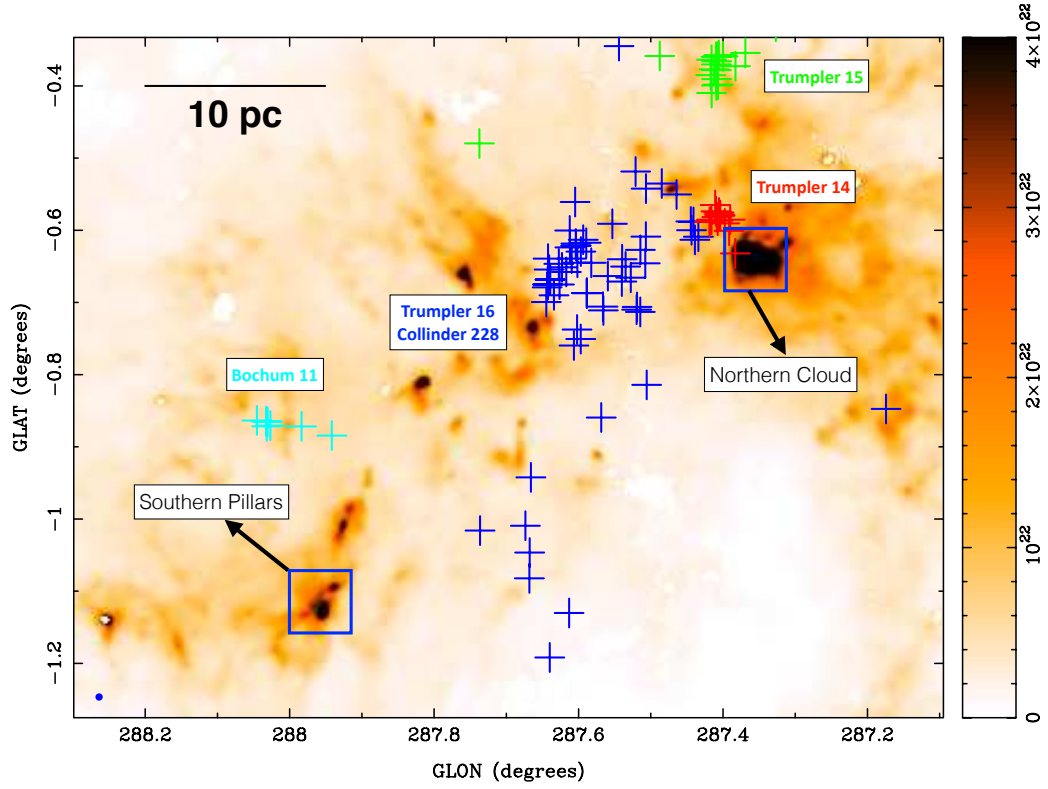
FIG. 1.— Total column density of the CNC derived from Herschel infrared maps (Rebolledo et al. 2016). The colour bar is in units of \text{cm}^{-2} . The blue boxes show the location of the regions observed with ALMA, one in the Northern Cloud and another in the Southern Pillars. Each box is \sim 4 \times 4 arcmin 2 . The horizontal black line shows the scale of 10 pc. The blue crosses show the Trumpler 16 and Collinder 228 stellar clusters, red crosses show Trumpler 14, green show Trumpler 15, and cyan crosses show Bochum 11 cluster, all of them listed in Smith (2006).
