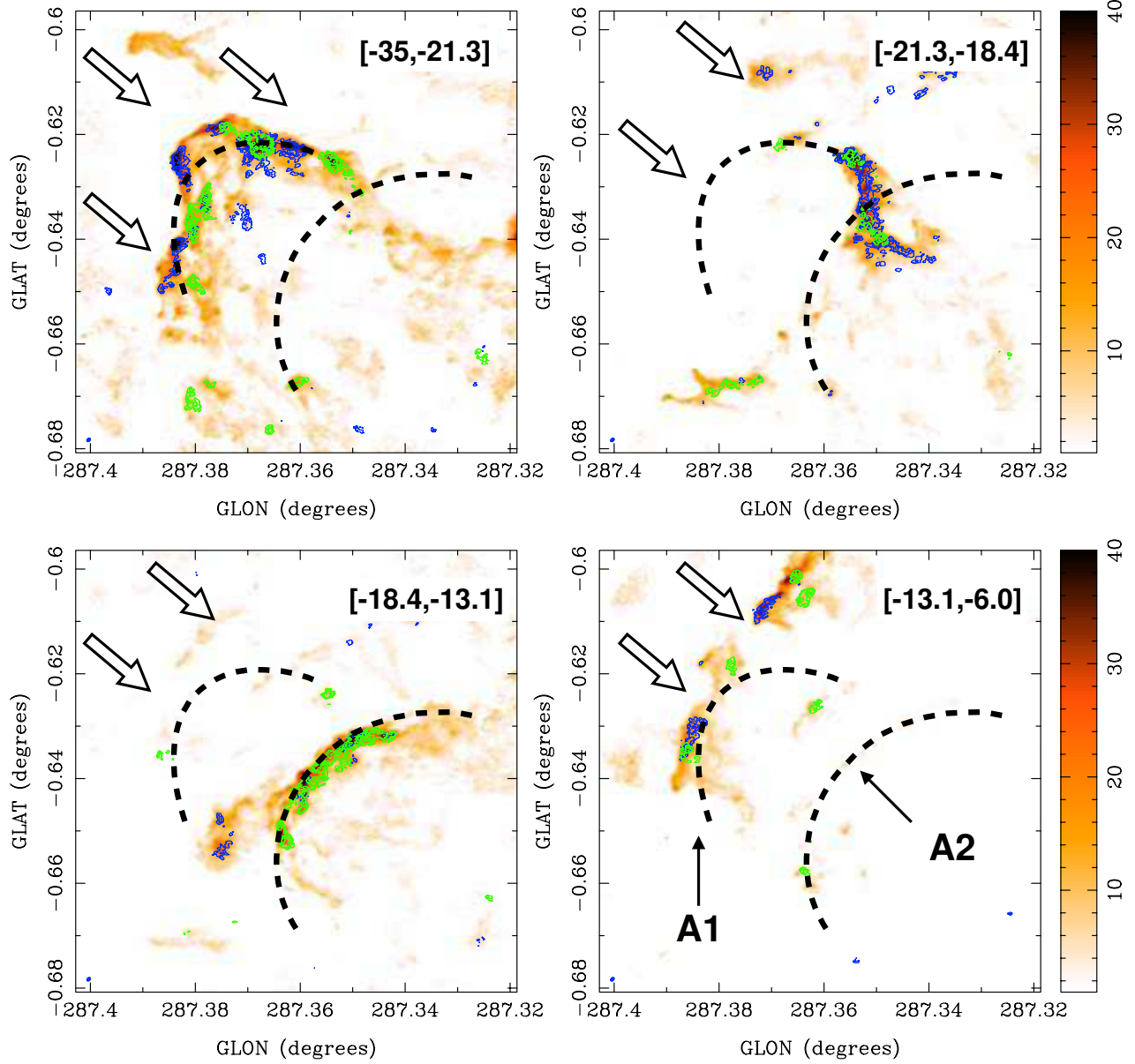
FIG. 7.— Velocity decomposition of the line emission in the NC. Each panel shows integrated intensity maps over the velocity range shown in the top-right in \text{km s}^{-1} . The velocity ranges are selected in order to show different gas shock fronts. The colour images are the integrated intensity of the \text{HCO}^+ in \text{K km s}^{-1} . The blue contours show the \text{H}^{13}\text{CO}^+ levels at 1, 2, 4, 8, 16, 32 and 64 \text{ K km s}^{-1} . The green contours show SiO integrated intensity levels at 0.5, 1, 2, 4, 8, 16, 32 and 64 \text{ K km s}^{-1} . The white arrows shows the approximate direction of the radiation front coming from the Trumpler 16 and 14 clusters shown in Figure 1.
