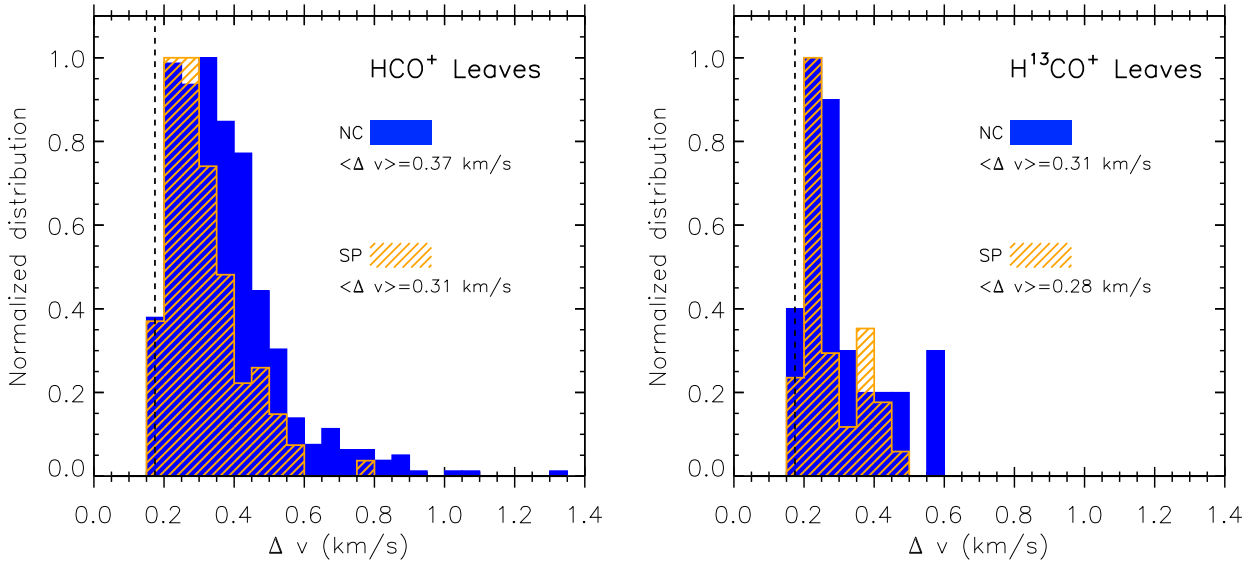
FIG. 13.— Normalised distributions of the velocity dispersion of the leaves identified by dendrograms in the \text{HCO}^+ (Left) and \text{H}^{13}\text{CO}^+ (Right). 584 leaves were identified in the NC and 184 in the SP. The filled blue histogram shows the leaves in the NC, while the line-filled orange histogram shows the leaves in the SP. The vertical dashed black line shows the channel width. The distribution of the velocity dispersion of the leaves identified in the NC has a larger mean and is broader than the distribution obtain from the leaves in the SP. Thus, at the scale probed by the size of the leaves, the level of turbulence is larger in the NC than the SP. However, the denser gas traced by \text{H}^{13}\text{CO}^+ shows no difference in the velocity dispersion between the two regions.
