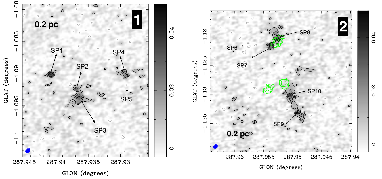
FIG. 5.— Zoomed view of the squares 1 and 2 shown in continuum map in Figure 4. Black and white map is the continuum, with colour bar in K. The blue ellipse in the left-bottom corner shows the ALMA synthesized beam. Grey (negative) and black (positive) contours show -3 , 3 , 5 , 7 and 9 sigma levels in the continuum map, with sigma equals to 3 mK. Green contours show the SiO integrated intensity levels 0.12 , 0.24 , 0.48 , 0.96 and 1.92 in units of \text{K km s}^{-1} . Ten cores are detected in the continuum emission map. SiO is detected nearby some compact sources, probably associated with outflows. Different from the NC, continuum or SiO diffuse emission are not detected.
