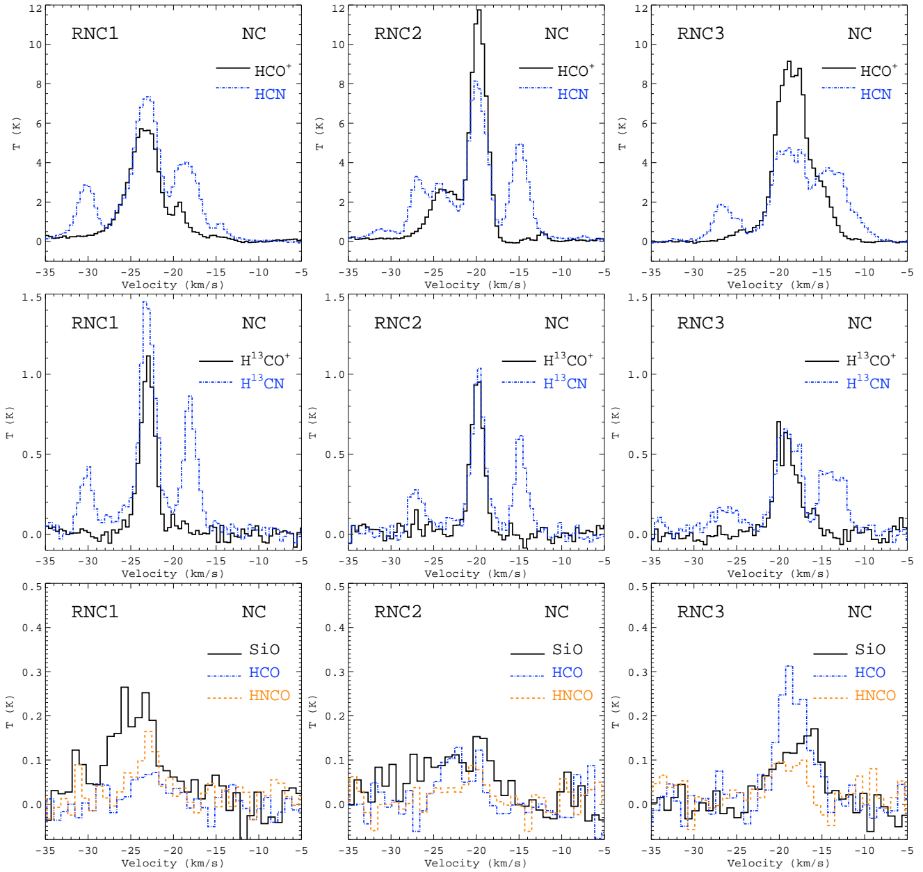
FIG. 6.— Average spectra of the detected lines towards three representative regions in the NC. The regions, RNC1, RNC2 and RNC3 are shown in Figure 2. HCN and \text{HCO}^+ are the brightest lines among the sample, and they show a complex velocity field in the NC. Hyperfine structure of HCN and \text{H}^{13}\text{CN} are clearly detected.
