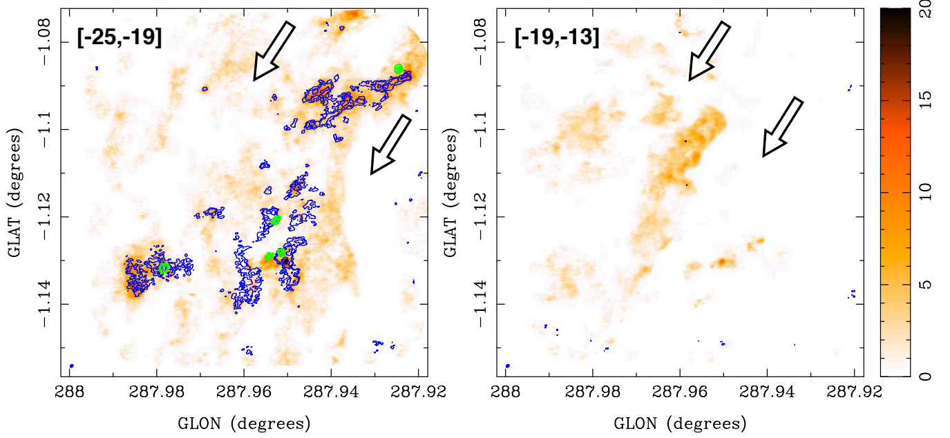
FIG. 9.— Velocity decomposition of the line emission in the SP. Each panel shows integrated intensity maps over the velocity range shown in the top-left in \text{km s}^{-1} . The velocity ranges are selected in order to show different gas shock fronts. The colour images are the integrated intensity of the \text{HCO}^+ in K. The blue contours show the \text{H}^{13}\text{CO}^+ levels at 1, 2, 4, 8 \text{K km s}^{-1} . The green contours show \text{SiO} integrated intensity levels at 0.12, 0.24, 0.48, 0.96, 1.92 \text{K km s}^{-1} . The white arrows shows the approximate direction of the radiation front coming from nearby massive star clusters shown in Figure 1.
