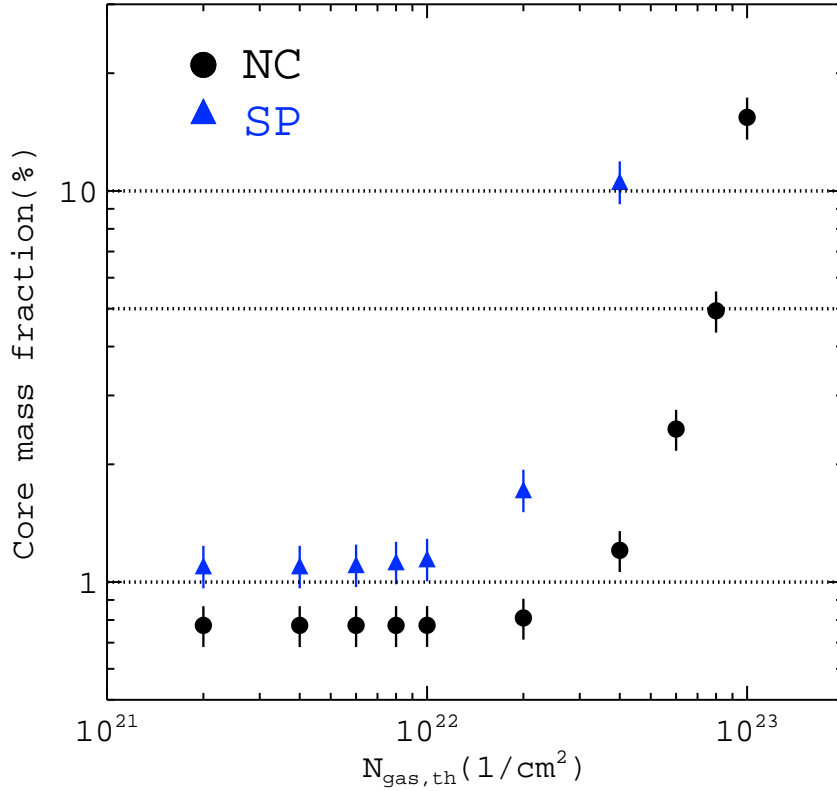
FIG. 10.— Fraction of the mass in cores with respect to the total mass calculated above a given column density threshold. Black circles shows the core mass fraction in the NC, while the blue triangles show the core mass fraction in the SP. The horizontal dotted lines show the 1%, 5% and 10% levels. When we estimate the total mass above N_{\text{gas,th}} = 2 \times 10^{21} \text{ cm}^{-2} , the core mass fraction is \sim 1\% for both SP and NC. As we increase the column density threshold to only consider the denser gas, the core mass fraction increases until it reaches a maximum of 10% at N_{\text{gas,th}} = 4 \times 10^{22} \text{ cm}^{-2} for the SP, and 16% at N_{\text{gas,th}} = 10^{23} \text{ cm}^{-2} for the NC.
