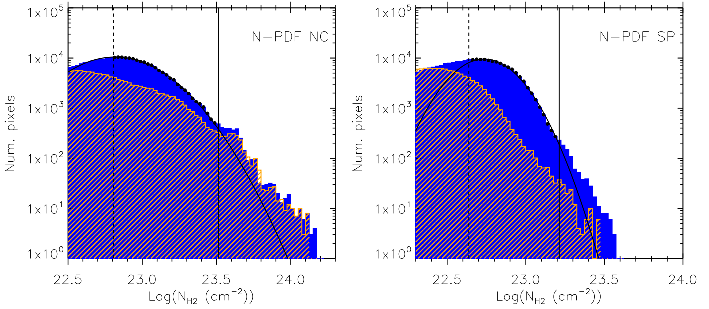
FIG. 17.— Probability distribution of the gas column density (N-PDF) in the NC (Left) and the SP (Right). The filled blue histogram shows the N-PDF obtained from the ALMA+APEX combined image, while the line-filled orange histogram shows the N-PDF from the ALMA only data. The black dashed line shows the 2\sigma_{\text{rms}} sensitivity limit of the continuum maps, and the vertical black solid line illustrates the values of N_{\text{H}_2, \text{log}} that mark the transition from gaussian to a power law regime. The black curved line shows the gaussian fit to the data, considering only the bins above the sensitivity limit and below the transition column density, which are shown with black dots.
