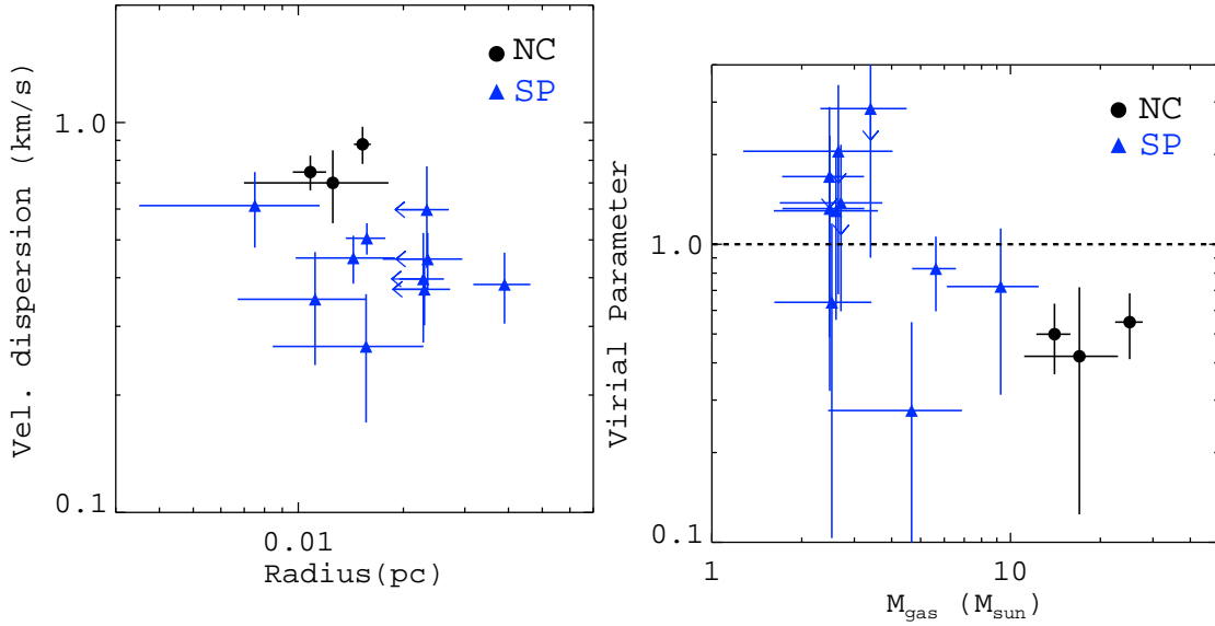
FIG. 11.— Left: Size vs. velocity dispersion relation for the cores identified in the continuum map. Velocity dispersion is calculated from the spectral profile derived from \text{H}^{13}\text{CO}^+ line. Solid black circles show the cores in the NC, while the blue triangles show the cores in the SP. The left pointing arrows show the un-resolved cores, so the sizes are upper limits. The cores in the NC have similar sizes compared to the cores at SP, but show slightly higher velocity dispersions. Right: Virial parameter vs. gas mass relation for the cores. Again, the down pointing arrows shows the un-resolved cores. In general, the resolved cores shows virial parameters below unity, giving some evidence of collapsing structures.
