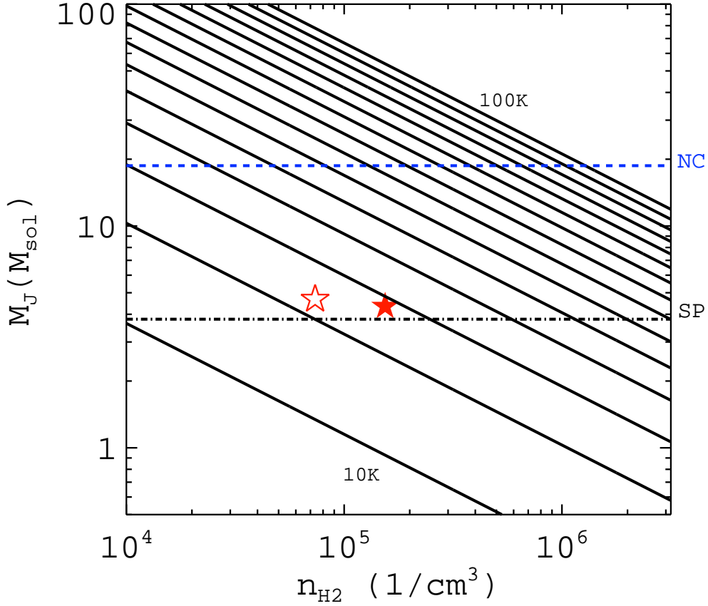
FIG. 12.— Relation between the Jeans mass ( M_J ) and the number volume density ( n_{\text{H}_2} ). Each diagonal line shows a relation for a different gas temperature, from 10 K (bottom) to 100 K (up) in steps of 10 K. Horizontal dashed lines shows the average core mass for the NC (blue dashed) and the SP (black dot-dashed). The red open star shows the M_J derived for average values of the volume density and temperature for the SP, while the red filled shows the value for the NC.
