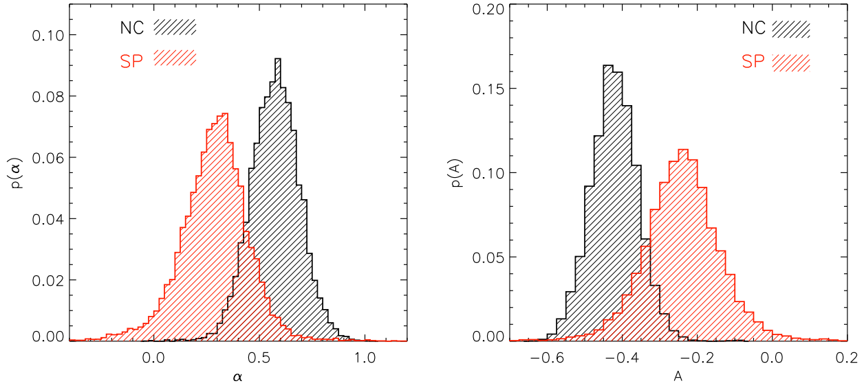
FIG. 15.— Probability distribution of the slope \alpha (Left) and the intercept coefficient A (Right) of the linear relation shown in Equation 6. The red line filled histograms show the parameter distributions obtained with SP data, and the black line filled histograms show the distributions for the NC. The \alpha parameter distribution peaks at a larger value in the NC (0.59) than in the SP (0.34), but a significant overlap exists between both distributions. This implies that there is a no negligible probability that both relations have the same slope. If the difference exists, then it might be related to the stellar feedback activity in the NC region, which is higher than in the SP. The turbulent motion detected in the \text{HCO}^+ line are tracing the effect of the stellar feedback on the low density gas in the NC region.
