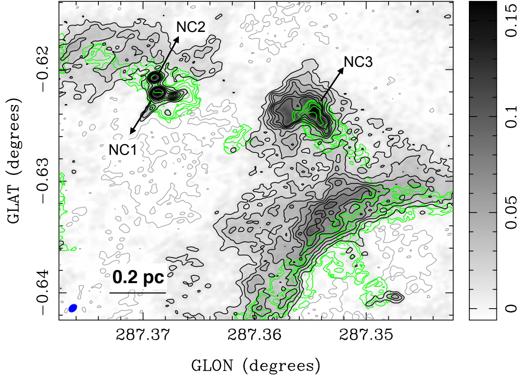
FIG. 3.— Zoomed view of the region shown in Figure 2. Black and white map is the continuum, with colour bar in K. The blue ellipse in the left-bottom corner shows the ALMA synthesized beam. Grey (negative) and black (positive) contours show -6 , -3 , 3 , 6 , 9 , 12 , 15 , 18 , and 21 sigma levels in the continuum map, with sigma equals to 4 mK. Green contours show the SiO integrated intensity levels 0.5 , 1 , 2 , 4 , 8 and 16 in units of \text{K km s}^{-1} . Three cores are detected in the continuum emission map. SiO is detected nearby the compact sources, probably associated with outflows. The diffuse SiO follows the arc-like structure A2 traced by the continuum emission, but it is spatially shifted. The continuum emission seen in A2 might be dominated by the ionized gas rather than hot dust emission. Thus, while the continuum emission traces the ionization front produced by the nearby massive stars, the SiO traces the PDR/shock front region.
