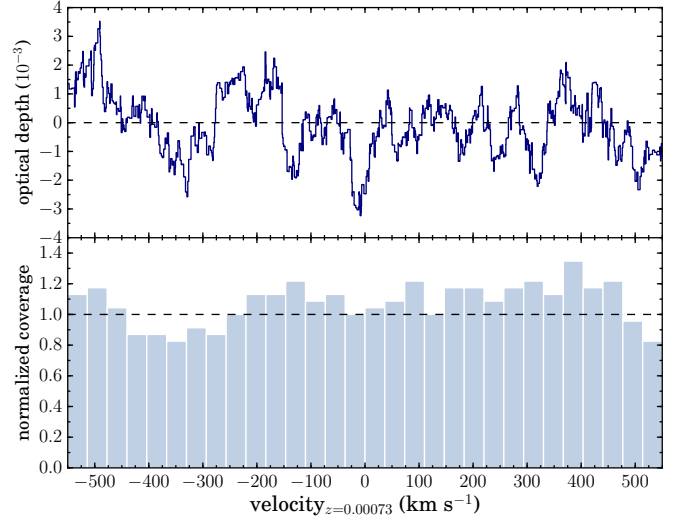
Figure B.4: Optical depth as a function of velocity, same as in Figure B.3, except we have extended the coverage to larger velocities by including subbands of M 82 flanking those which contain a line. The standard deviation in the line-free channels after correcting for non-uniform coverage is 1.3 \times 10^{-3} .
