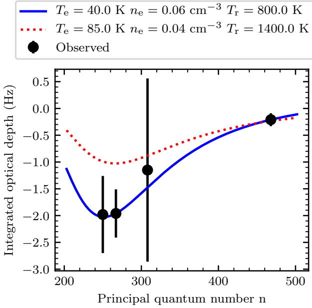
Figure 12: The integrated optical depth as a function of principal quantum number, n , for the Hydrogen RRLs detections associated with the -47 \text{ km s}^{-1} velocity component towards Cas A. The figure shows the values from Table 2 using 3\sigma error bars. The blue, solid line shows the best fit model. The red, dotted line shows the best fit model (O17) to Carbon RRL detections spanning quantum numbers 225 – 550 (e.g. see Figure 10).
