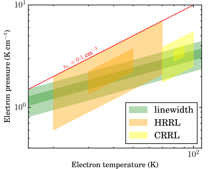
Figure 13: The electron pressure as a function of electron temperature of the -47 \text{ km s}^{-1} velocity component towards Cas A. The red solid line shows the upper limit of a Pressure broadened line-width. Shaded regions represent 1\sigma and 3\sigma uncertainty. The green shaded regions show the line-width constraints from the combined Doppler, pressure and radiation broadening terms for T_{r,100} = 1400 \text{ K} (S17). The orange shaded regions show the physical properties of the HRRLs constrained from modeling the integrated optical depth. The yellow shaded regions show the physical properties of the CRRLs constrained from modeling the integrated optical depth (O17). This plot shows the distinction between the HRRLs and CRRLs, where HRRLs arise from slightly colder, denser regions in the cloud.
