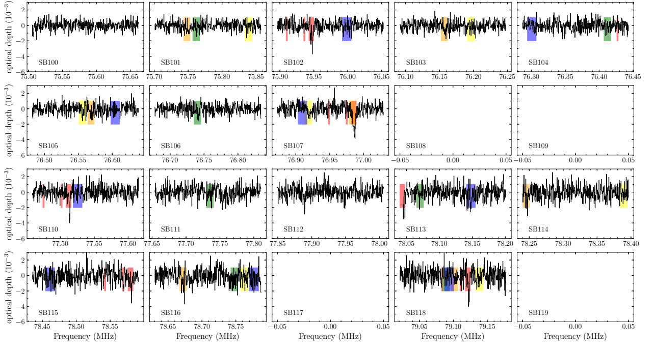
Figure A.1: The subband spectra of Cas A, shown after continuum removal, as the optical depth as a function of frequency. The red shaded regions cover the location of \alpha -transitions, orange regions cover \beta -transitions, yellow regions cover \gamma -transitions, green regions cover \delta -transitions, and blue regions cover \epsilon -transitions. We note that the widest shaded regions in red cover the spectral lines of the -47 km/s and -38 km/s C\alpha components; two recurring thin shaded regions in red represent the weak, narrow spectral lines of the 0 km s^{-1} C\alpha component and H\alpha at -47 km s^{-1} .
