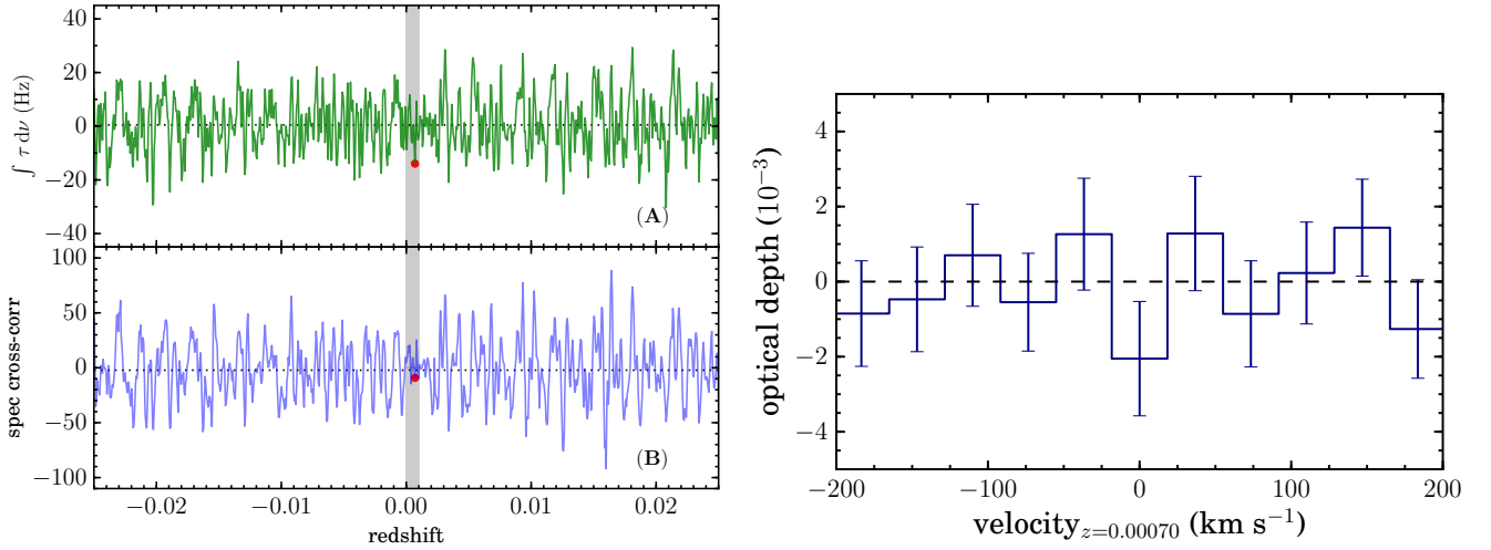
Figure 14: Our results for M 82. Left : Same as in Figure 8, except applied to the C\alpha -transitions of M 82. We did not proceed with the stack cross-correlation because no significant outlier was identified in (B). The shaded region in gray shows the redshift range probed by M14. The red data point shows marks z_{M82} = 0.00070 , the redshift corresponding to the peak of RRL emission, as reported by M14. Right : The stacked spectrum of M 82, in velocity units, with respect to z_{M82} = 0.00070 . The error bars reflect the standard deviation of a weighted mean (see Sec. 3.1)
