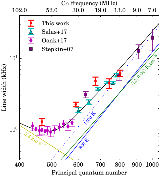
Figure 9: Line-width for the -47 \text{ km s}^{-1} velocity component (or the sum of blended -47 and -38 \text{ km s}^{-1} components) as a function of principal quantum number. The red points show the measured line-widths from this work (Table 1); the C\alpha(467) and C\beta(590) are derived only from the -47 \text{ km s}^{-1} velocity component, while the higher order transitions represent a single fit to the blended -47 and -38 \text{ km s}^{-1} components. The cyan triangles show the line-widths of the C\alpha and C\beta transitions of the -47 \text{ km s}^{-1} velocity component from S17. The purple diamonds show the line-widths of the -47 \text{ km s}^{-1} component from O17. The purple squares show the C\alpha , C\beta , C\gamma and C\delta data, for which the -47 and -38 \text{ km s}^{-1} components are blended, from Stepkin et al. (2007). The colored lines show the contribution from Doppler broadening (yellow line), pressure broadening (green line) and radiation broadening (blue lines). The solid black line shows the model which best fit the line-widths from S17: a Doppler line-width of 3.4 \text{ km s}^{-1} , T_e = 85 \text{ K} , n_e = 0.04 \text{ cm}^{-3} and a radiation field which is a combination of a power law with T_{r,100} = 800 \text{ K} and \alpha = -2.6 plus a contribution to the radiation field from Cas A.
