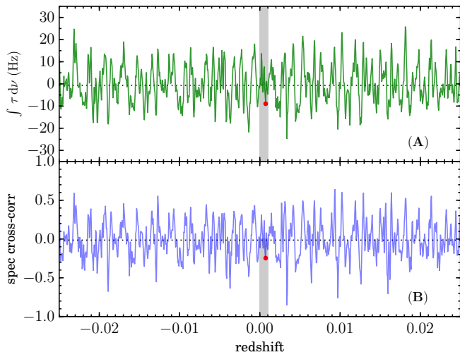
Figure B.5: Same as in Figure 14 where we have implemented a stacking and spectral cross-correlation across a range of redshifts, except in this case the spectra have been combined and smoothed via a Savitzky-Golay filter. We mimicked the procedure M14 used to flag, process, and smooth the data of M 82 as best as possible.
