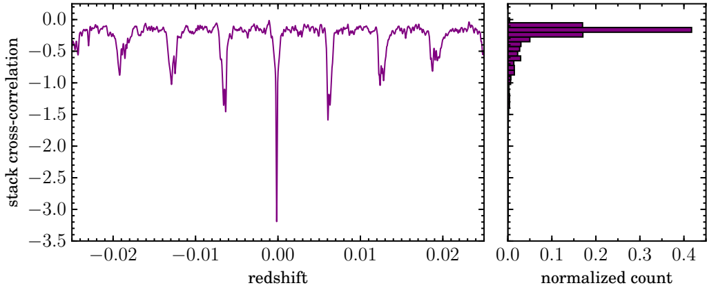
Figure 6: The integrated optical depth of the observed Cas A spectra is cross-correlated with the expected template spectrum. Here we clearly see an outlying peak at the redshift ( z = -0.000158 ) of the -47 \text{ km s}^{-1} component. The histogram on the right shows the binned distribution of integrated optical depth. Cas A \alpha -transition stacking demonstrates our method in a high signal-to-noise regime.
