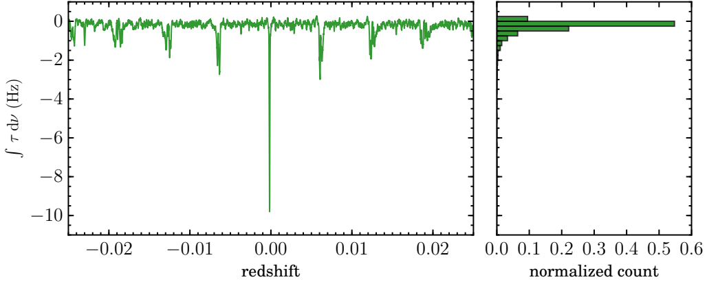
Figure 3: Cas A spectra has been stacked for C\alpha RRLs across a range of redshifts. The plot on the left shows the optical depth integrated at the central velocities ( -7.7 \text{ km s}^{-1} to +19.8 \text{ km s}^{-1} , which encompasses the -47 and -38 \text{ km s}^{-1} components) at each redshift. Here we clearly see an outlying peak at the redshift ( z = -0.000158 ) of the -47 \text{ km s}^{-1} component. The histogram on the right shows the binned distribution of integrated optical depth. Cas A \alpha -transition stacking demonstrates our method in a high signal-to-noise regime.
