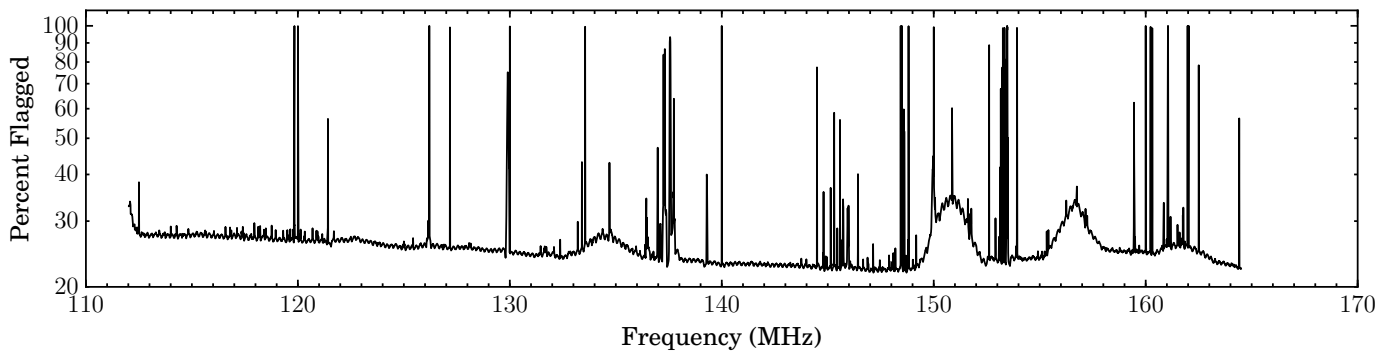
Figure 2: Percentage of flagged visibilities per channel in the calibrated target data. The total percentage here includes 10 remote stations and 4 core stations that have been flagged. Broad bumps centered at frequencies of about 135, 151, 157, and 162 MHz show broad-band RFI that results from intermodulation products of DAB amplifiers.
