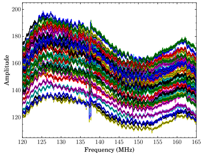
Figure 1: Bandpass solutions of the XX polarization towards the primary calibrator 3C196, in which stations are represented with different colors. These solutions demonstrate the global shape of the bandpass, as well a \sim 1 MHz ripple which results from a standing wave. Unflagged RFI is still present between 137–138 MHz. All core-stations have the same cable length and thus standing wave of the same periodicity. The fit to the solutions of each station, which is transferred to the target, is shown in black.
