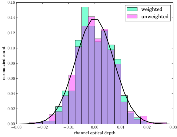
Figure B.2: Histogram of the optical depth of line-free channels, shown before (pink) and after (green) weighting with their overlap in purple. The black solid line shows the Gaussian fit to the weighted subbands. Unweighted, the fit to the distribution has a mean of \mu_{uw} = -1.4 \times 10^{-3} and a standard deviation of \sigma_{uw} = 7.2 \times 10^{-3} . Weighted, the best fit Gaussian has properties of \mu_w = -1.3 \times 10^{-3} and \sigma_w = 7.3 \times 10^{-3} . These subbands of M 82 were flagged and processed following the criteria of M14.
