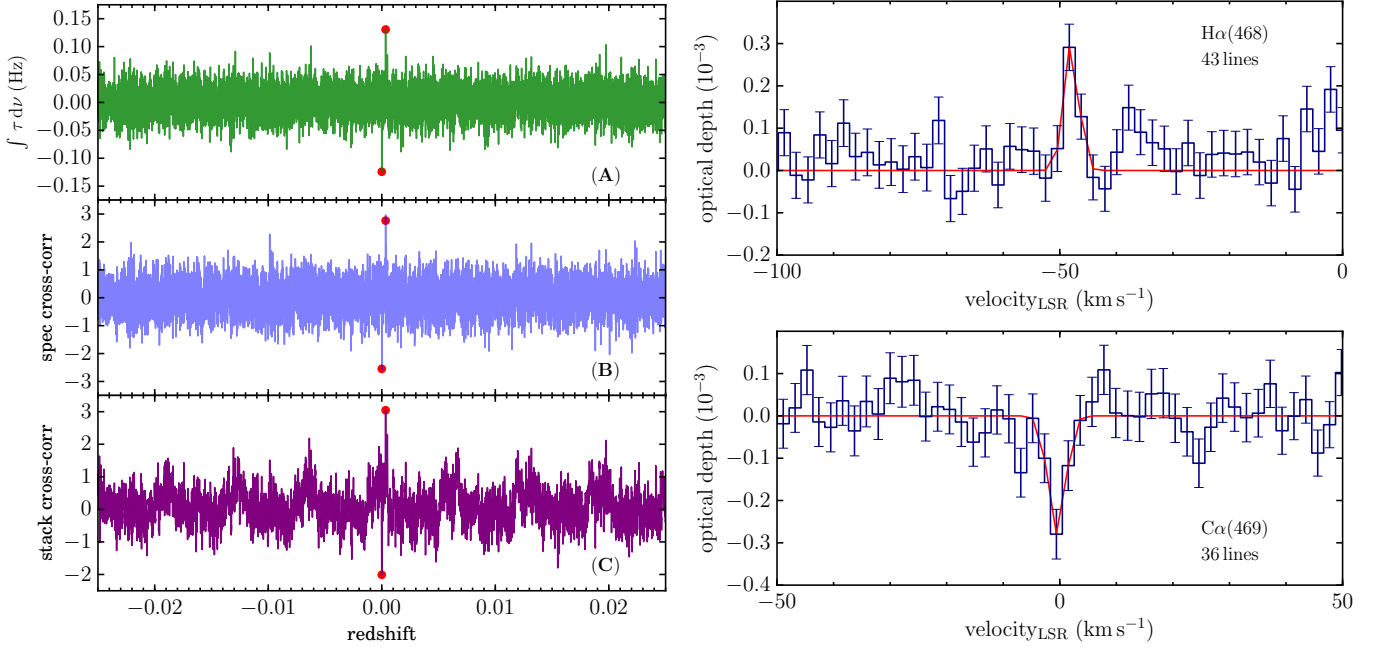
Figure 11: Left : Same as in Figure 8, except applied to \text{Ca}\alpha -transitions in Cas A spectra. Fits to the -47 \text{ km s}^{-1} and -38 \text{ km s}^{-1} components (and all higher order transitions) have been subtracted in the spectrum of Cas A. Residuals remaining from imperfect subtraction of the brightest \alpha transitions from -47 \text{ km s}^{-1} and -38 \text{ km s}^{-1} components can be seen in (C). These results demonstrate the behavior of the method in the presence of narrow, low signal-to-noise spectral lines. The redshifts ( z_H = 0.000337 and z_C = -0.000002 , with respect to stacking for \text{Ca}\alpha ) of the two detections are shown in red. Right : The stacked spectrum of \text{H}\alpha (top) associated with the -47 \text{ km s}^{-1} component, one of the lowest frequency detections of Hydrogen RRLs. \text{Ca}\alpha (bottom) associated with the Orion Arm, detected at this frequency for the first time.
