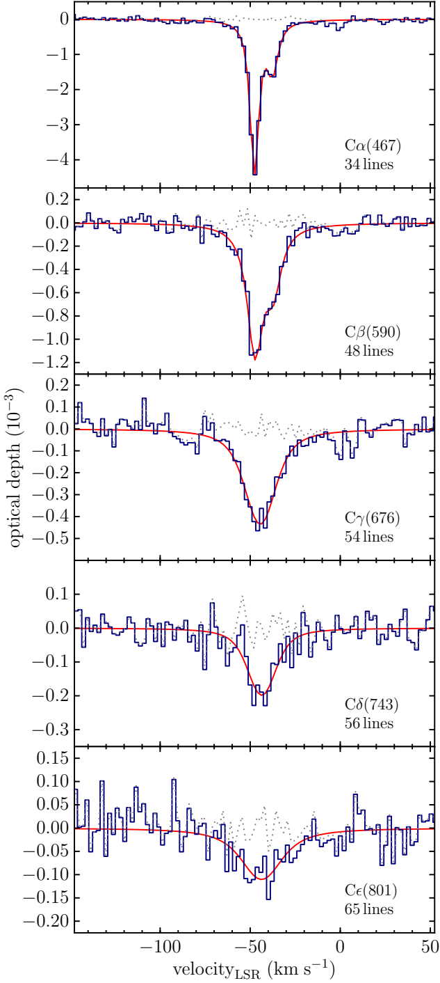
Figure 7: The stack averaged profiles for the carbon transitions associated with the v_{\text{LSR}} = -47 \text{ km s}^{-1} and v_{\text{LSR}} = -38 \text{ km s}^{-1} components in 55 MHz – 78 MHz observations of Cas A. These have all been significantly identified by our method.
