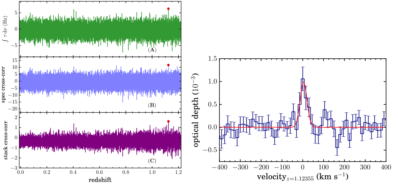
Figure 15: Our results for 3C 190. Left : Same as in Figure 8 except applied to the \text{Ca}\alpha -transitions of 3C 190. The red data point marks the significantly identified redshift of z = 1.12355 . Right : The spectrum resulting from stacking \text{Ca}\alpha -transitions at z = 1.12355 in 3C 190, using a line-blanking region of \pm 25 \text{ km s}^{-1} .
