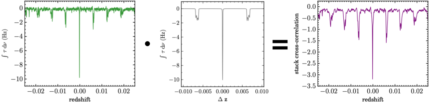
Figure 5: Here we demonstrate the stack cross-correlation. Cas A spectra have been stacked for C\alpha RRLs across a range of redshifts. The plot on the left shows the optical depth integrated at the central velocities at each redshift. The middle plot shows the integrated optical depth resulting from stacking the template spectrum. It has been done for a redshift of z = 0.000158 . We cross-correlate the left plot with the middle plot to obtain the stack cross-correlation on the right .
