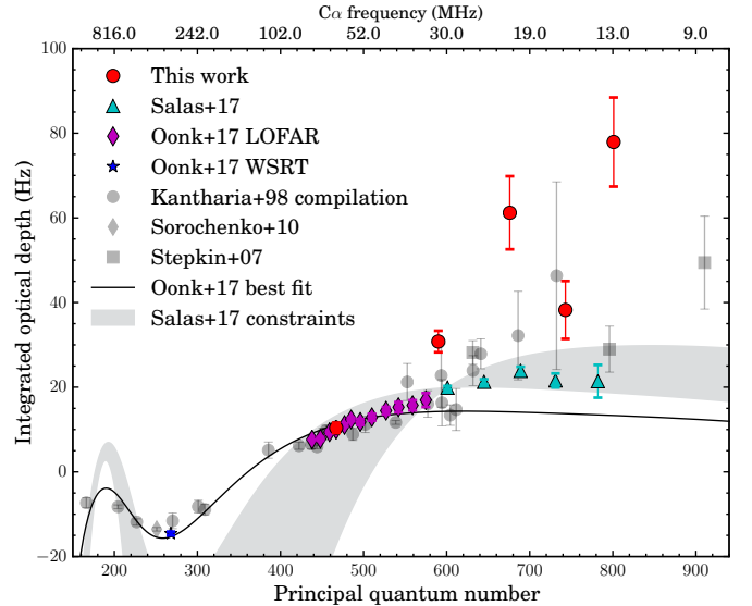
Figure 10: Integrated optical depth as a function of principal quantum number for the sum of the Perseus arm components at -47 and -38 \text{ km s}^{-1} adapted from S17. The cyan triangles show the 10–33 MHz LOFAR observations of S17. The purple diamonds represent the 33–78 MHz LOFAR detections and the blue star shows the WSRT detection (O17). Pre-LOFAR literature data are shown in gray data points (Kantharia et al. 1998; Stepkin et al. 2007; Sorochenko & Smirnov 2010). The black solid line is the best-fitting model from O17. The gray shaded region covers the models which correspond to the physical constraints from S17.
