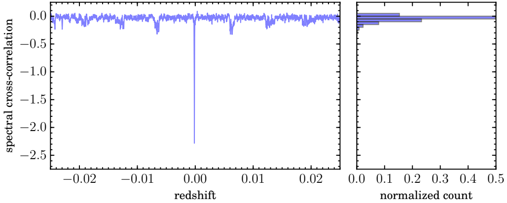
Figure 4: Cas A spectra have been cross-correlated for C\alpha RRLs with a template spectrum across a range of redshifts. The plot on the left shows the spectral cross-correlation value at each redshift. Again we clearly see an outlying peak at the redshift ( z = -0.000158 ) of the -47 \text{ km s}^{-1} component. The histogram on the right shows the binned distribution of cross-correlation values. Cas A \alpha -transition stacking demonstrates our method in a high signal-to-noise regime.
