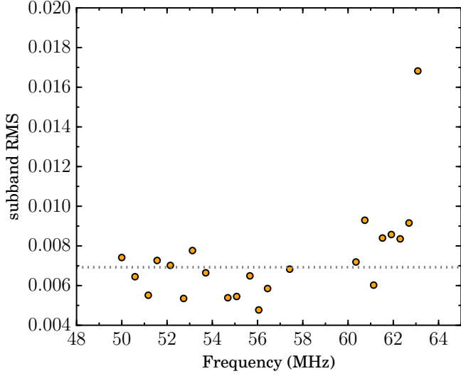
Figure B.1: The RMS of each M 82 subband plotted against the average frequency of the subband. The gray dotted lines represents the median value of 6.9 \times 10^{-3} . These subbands were flagged and processed following the criteria of M14. The RMS was determined from line-free channels only.
