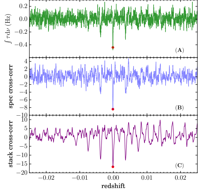
Figure 8: The three steps of our method applied to \epsilon -transition stacking in the spectrum of Cas A: (A) the integrated optical depth at each redshift (see Section 3.1) where “mirrors” are seen at e.g. z_m = \pm 0.004 , (B) the spectral cross-correlation (see Section 3.2), and (C) the stack cross-correlation (see Section 3.3). This example demonstrates the behavior of the method in the presence of broad RRLs.
