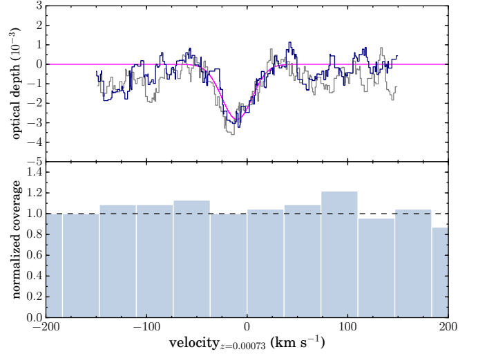
Figure B.3: The top plot shows the optical depth as a function of velocity for the RRL spectrum of M 82 stacked at z_{M82} = 0.00073 and smoothed with a Savitzky-Golay filter. In navy blue is the spectrum we reproduced following the criteria of M14; the magenta line shows the best fit Gaussian. The standard deviation in the line-free channels is 6.5 \times 10^{-4} . In gray is the final M14 spectrum (courtesy L. Morabito). The bottom plot shows the coverage, or number of subband data points, within velocity bins of 36.7 \text{ km s}^{-1} . The coverage count has been normalized by 23, the number of data points in the bin where the line peak falls.
