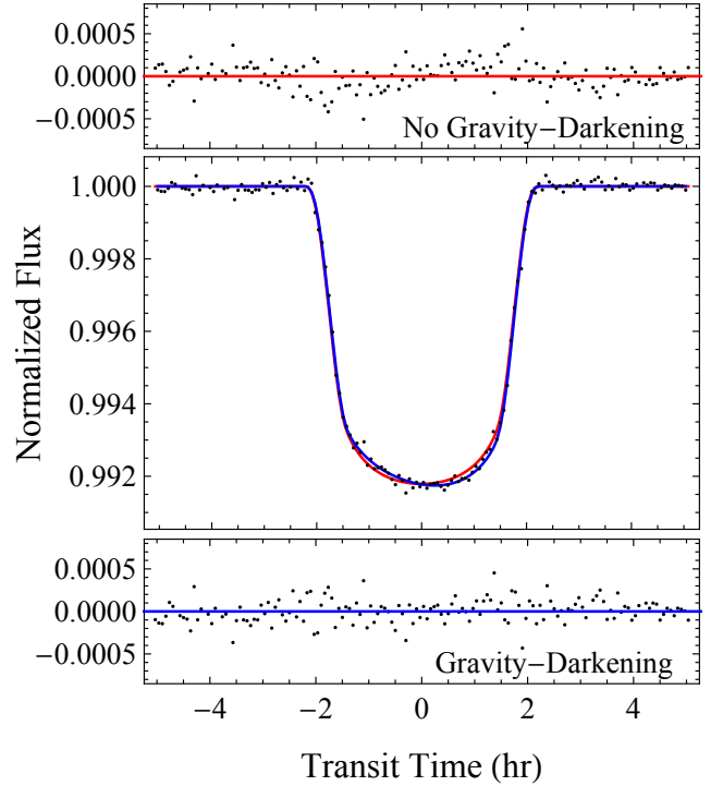
Figure 5. MASCARA-4 b’s TESS light curve shows a clear left/right asymmetry due to its host star’s gravity-darkened surface. The planet begins its transit near the star’s dim equator and moves toward the star’s bright pole, thus yielding a greater transit depth during egress. The above figure shows our best-fit model with and without gravity-darkening (blue and red, respectively). The gravity-darkening signal is evident in the top residual, in which a traditional best-fit model cannot resolve the star’s asymmetry.
