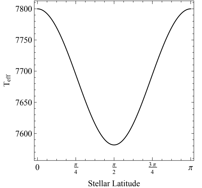
Figure 3. The MASCARA-4 b host star varies roughly 220 K between its poles and equator due to its rapid rotation. Its \sim 3\% change in local effective temperature corresponds to a \sim 12\% change in local brightness, resulting in a pole-to-equator luminosity gradient that influences MASCARA-4 b’s transit light curve and irradiation.
