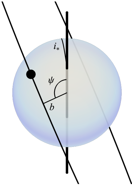
Figure 2. The gravity-darkening technique measures three point-of-view orbit geometry parameters that together yield the true spin-orbit angle. The stellar inclination ( i_* ) is the star’s rotation axis tilt toward/away the viewer. The projected obliquity ( \psi ) is the projected tilt of the planet’s orbit in the plane of the sky, and is the same angle measured by Doppler tomography. The orbital inclination ( i ) is the planet’s orbital tilt toward/away the viewer, and is defined by \cos(i) = bR_*/r , where b is the impact parameter and r is the planet’s distance from the star. The star’s color gradient represents its gravity-darkened surface.
