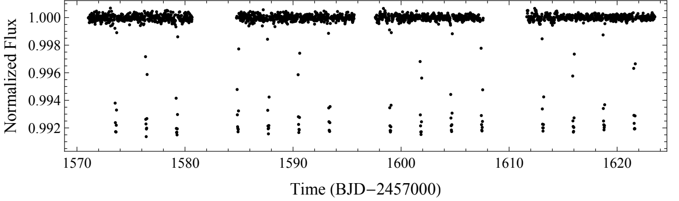
Figure 1. TESS observed 16 transit events of MASCARA-4 b during its sectors 10 and 11 observing campaigns at 30-minute cadence. We remove the first transit of Sector 10 from our dataset – which was contaminated by excess scattered light – leaving 15 transits for our analysis. We show the detrended MASCARA-4 b TESS light curve here.
