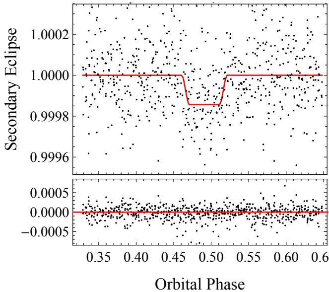
Figure 6. MASCARA-4 b’s secondary eclipse occurs at 0.491 \pm 0.007 orbital phase, indicating a slightly eccentric orbit. We measure an eclipse depth of 130 \pm 20 ppm. We list measured eclipse parameters in Table 2 and discuss the eclipse depth in §3.1.
