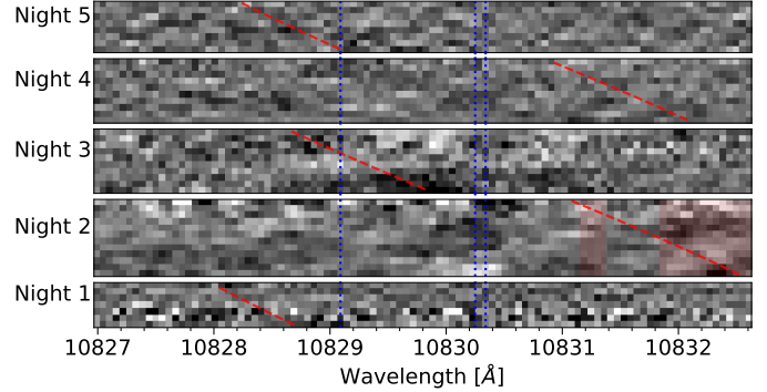
Fig. 4. Residual spectral series from night 1 to 5. The y-axis represents the time or orbital phase. The residuals are binned to 0.006 in phase for clarity. The slanted dashed lines in red trace the expected planetary helium line. The dotted lines in blue denote the positions of the stellar He I triplet. The shaded region in night 2 contains the telluric H 2 O absorption and OH emission line, overlapping with the expected planetary helium line.
