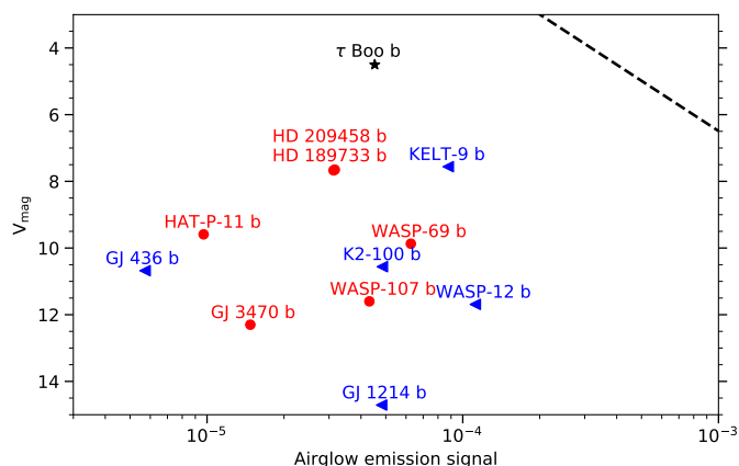
Fig. 9. The V magnitude of host stars plotted against the airglow emission signal estimated using Equation 3 for exoplanets with He I absorption detections (in red dots) or upper limits (in blue triangles). The black star represents the estimated signal of \tau Boo b assuming a typical absorption level of 1%. The black dashed line shows the detection limit of our analysis.
