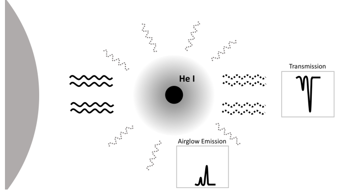
Fig. 1. Illustration of He I emission from an exosphere of a close-in planet. The gray disk represents the extended atmosphere around such planet. He I absorption is observed during transit, while airglow emission can be probed at other orbital phases.
