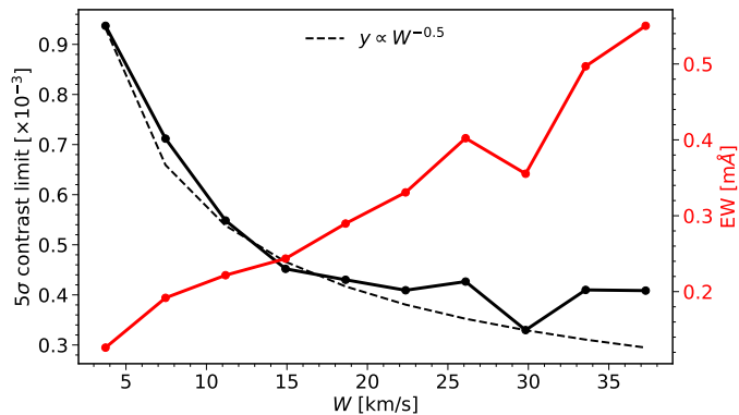
Fig. 7. The 5\sigma detection limit of the He I airglow emission as a function of the line width of the potential signal using 3 nights of observations of \tau Boo b (solid black line), and corresponding equivalent widths of the detection limit (solid red curve). The dashed line represents a scaled relation of W^{-1/2} , expected for pure Gaussian white noise.
