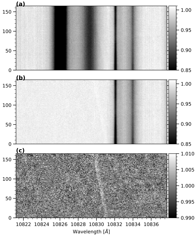
Fig. 3. Illustration of our data reduction steps applied to the spectral series taken on Night 4. Each row in the matrix represents one spectrum, with the y-axis corresponding to time. As detailed in Section 4.1, the steps include: (a) normalization of the continuum; (b) correction for stellar lines in each spectrum using an empirical model; (c) removal of telluric contamination by correcting the temporal variation of the flux in telluric lines using a column-by-column linear regression. The trail of an artificially injected planetary helium line (with a magnitude of 0.3% and a width of 11 km s -1 ) can be seen as a slanted white band near 10830 Å, shifting in time due to the change in the radial component of the orbital velocity of the planet.
