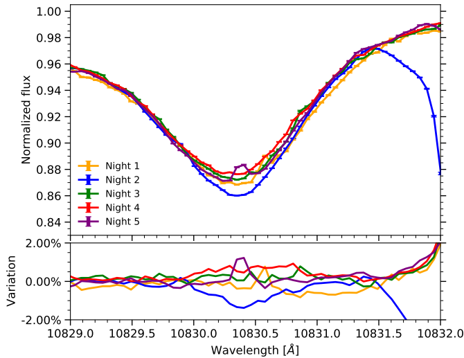
Fig. 5. Upper panel: the average profile of the stellar helium line in each night. Lower panel: the difference of each profile with respect to the mean. The deep absorption line at 10832.2 Å in night 2 (blue curve) is a telluric H 2 O line. The small peaks on top of the helium line in night 1 and 5 are caused by sky OH emission.
