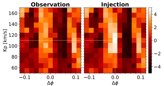
Fig. 8. The S/N map for a grid of planetary orbits with different semi-amplitude K_p and phase offset \Delta\phi . There is no salient signal in the observations (left panel). An injected signal at K_p = 110 \text{ km s}^{-1} and \Delta\phi = 0 is clearly recovered (right panel).
