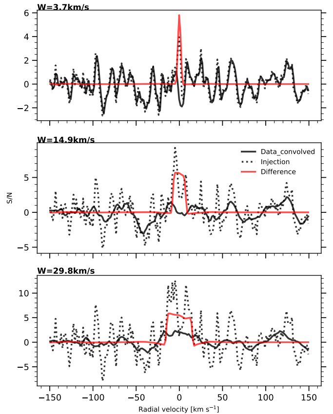
Fig. 6. Combined (3 nights) residual spectra in the planetary rest frame centered at the 10830 Å He I line. In the three panels, the solid black line indicates the residual spectra, boxcar-smoothed by 3.7 km s -1 (top), 14.9 km s -1 (middle), and 29.8 km s -1 (bottom). The dotted curves show an artificially injected signal at a S/N of 5, with the solid red curve the difference between the injected and original data. The values are scaled by the standard deviation of the observed residuals so that the y-axis represents the S/N.
