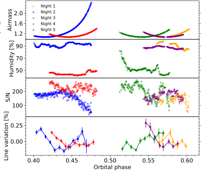
Fig. 2. Variation in airmass (upper panel), relative humidity (mid panel), S/N (lower panel) and variation around the mean of the stellar He I line (bottom panel) during observations in the different nights. The S/N of each spectrum is defined as the average signal-to-noise ratio of the continuum near the He I 10830 Å line.
