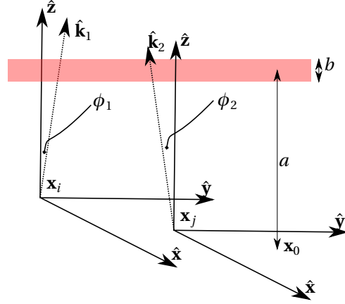
Fig. 1: The geometry of the toy model. The ionosphere is a layer of thickness b at height a above a reference location \mathbf{x}_0 . In general, \Delta\text{TEC} is the TEC along one geodesic minus the TEC along another parallel geodesic. Usually, these geodesics are originating at antennae i and j (locations \mathbf{x}_i and \mathbf{x}_j ), and pointing in directions \hat{\mathbf{k}}_1 and \hat{\mathbf{k}}_2 , respectively. One common choice is to have a fixed reference antenna for all \Delta\text{TEC} measurements. The corresponding zenith angles are \phi_1 and \phi_2 .
