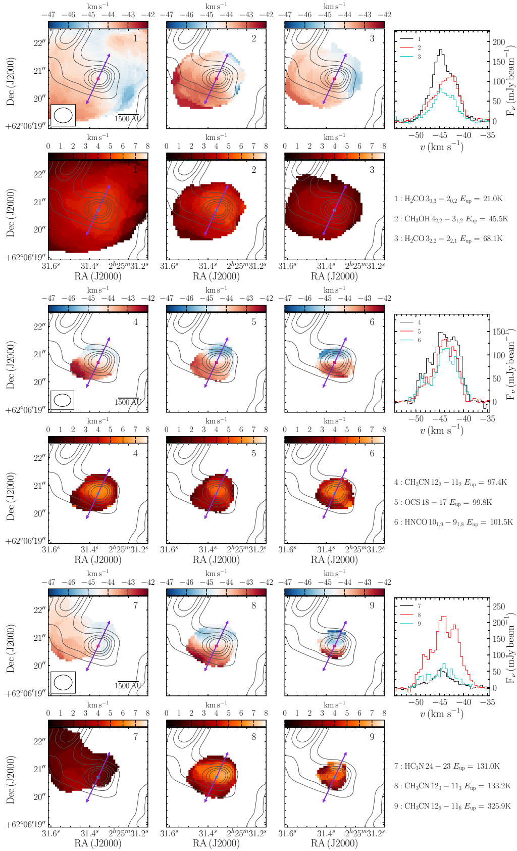
Fig. 11. Intensity-weighted velocity (moment 1, top, third, and fifth rows) and intensity-weighted FWHM (moment 2, second, fourth, and sixth rows) maps of key species in the high velocity-resolution data, along with their spectra at the continuum peak, as indicated with a red box on the moment 1 maps and a cyan box on the moment 2 maps. The lines are shown from left to right and top to bottom in order of increasing transition upper energy level ( E_{\text{up}} ). The NOEMA continuum emission with similar beam-size to the data are shown as grey contours from 5 to 45\sigma in 10\sigma intervals ( \sigma = 0.43 \text{ mJy beam}^{-1} ) in the maps, which are clipped at 5\sigma of the corresponding integrated intensity map. The purple arrows indicate the suggested direction of the outflow as in Fig. 9.
