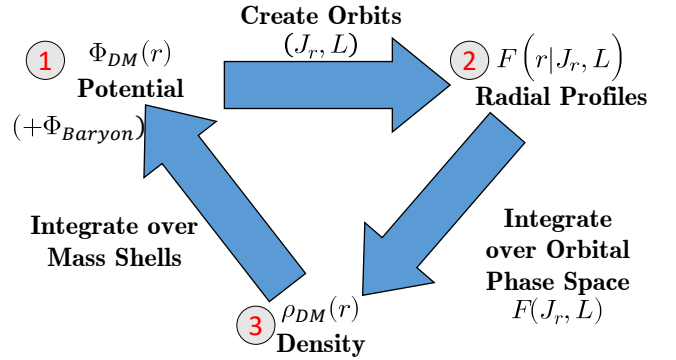
Figure 7. Flowchart of an iterative scheme to calculate a halo density profile starting from its action distribution, F(J_r, L) . The method proceeds as follows: 1) using a trial gravitational potential for the DM, \Phi_{DM}^0(r) , calculate the radial range, F(r|J_r, L) , of each orbit, (J_r, L) ; 2) integrate over all orbits to calculate the DM density profile, \rho_{DM}(r) ; 3) use the inferred DM density to update the DM potential, \Phi_{DM} ; and repeat from step 1) until convergence is achieved. If required, an additional baryon potential \Phi_{Baryon} can be added in step 1) to find a contracted halo.
