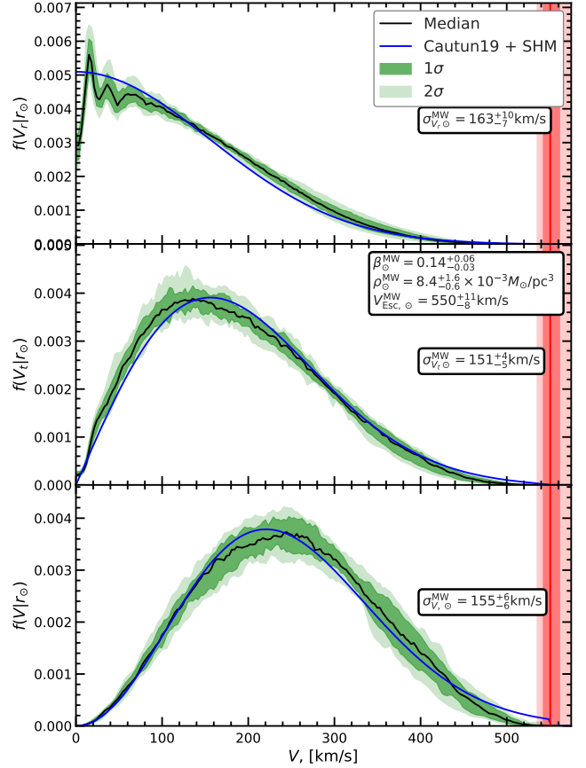
Figure 11. The DM velocity distribution at the Solar radius, r_{\odot} = 8\text{kpc} , as predicted by our halo contraction model. The radial, tangential, and total velocity distributions are shown in the top, middle and bottom panels, respectively. The median is indicated with a solid black line and the 68 and 95 percentiles are shown in shaded green. The blue curve illustrates the velocity distributions given by the Standard Halo Model (SHM) using the Cautun19 MW mass model. We also give several DM properties at the Solar radius (see text inserts in the panels) as predicted from our model: the local DM density, \rho_{\odot} ; the components of the velocity dispersion, \sigma_{\odot} ; the velocity anisotropy, \beta_{\odot} ; and the escape velocity, V_{\text{Esc},\odot}^{\text{MW}} (whose value is also shown as the red shaded region).
