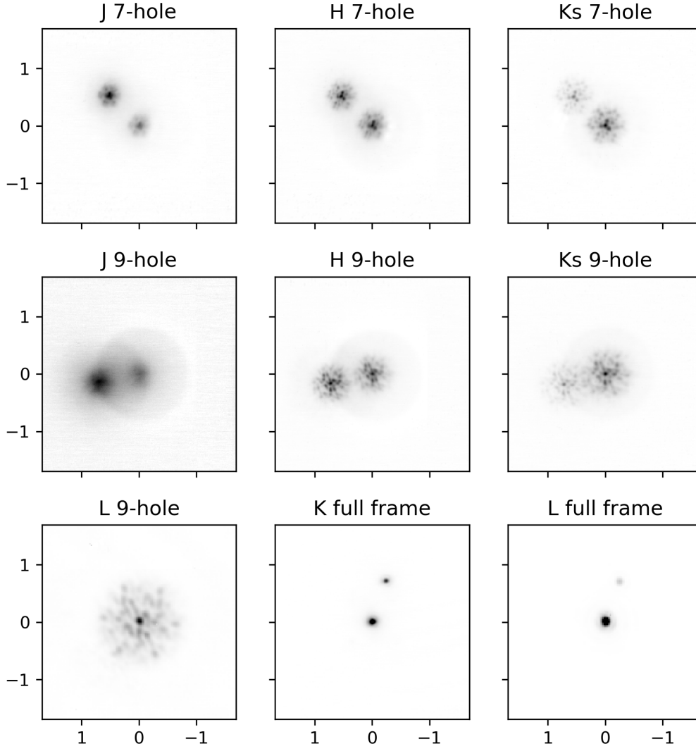
Figure A1. Example cleaned data frames of Apep from each band and mask (stacked over all frames in each sample cube). Images have been scaled to a common plate scale (axes are in units of mas), however the position angle which varies with epoch and time-of-observation has not, causing the orientation of the binary to appear to change.
