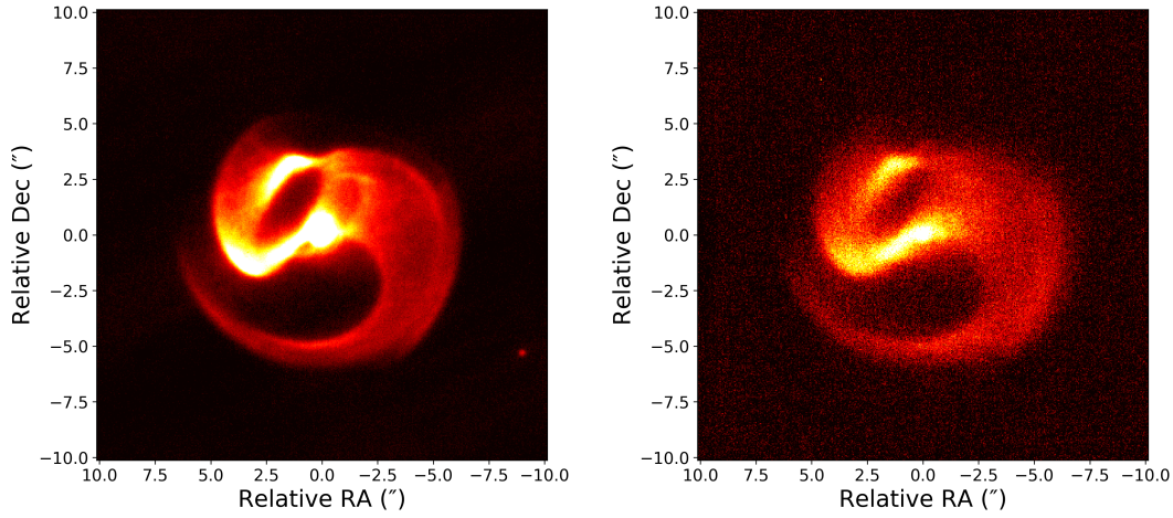
Figure 1. Reduced 2018 epoch images taken with the J8.9 filter (left) and Q3 filter (right). The normalised pixel values were stretched from 0 to 0.03 in J8.9 and to 0.5 in Q3 on a linear scale. The faint background star used for plate scale calibration, 2MASS J16004953-5142506, is just visible to the south-west of the plume near the edge of the field in the J8.9 data.
