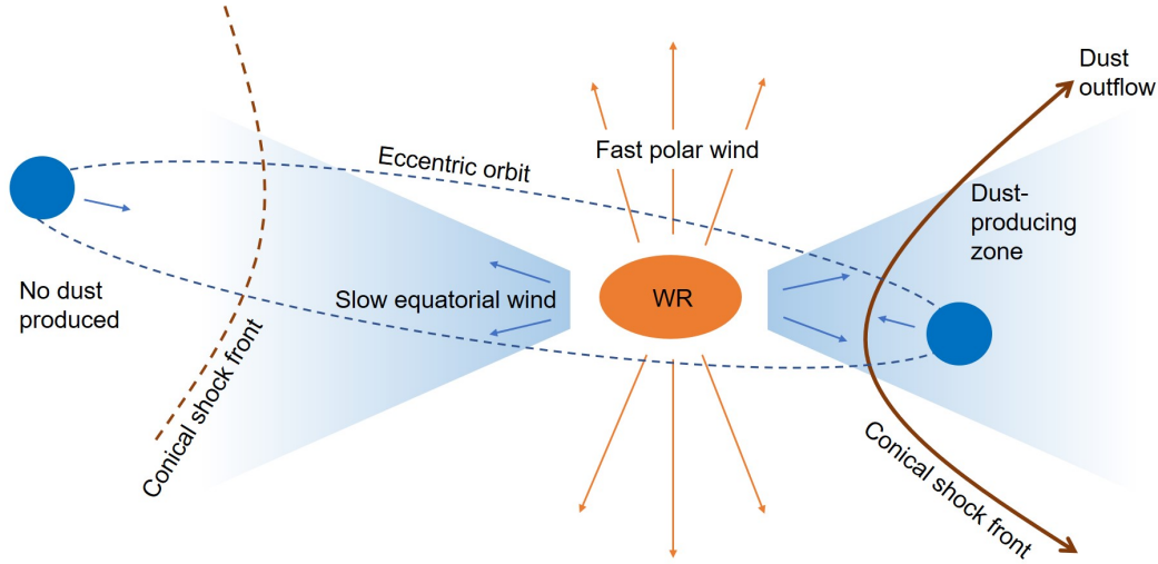
Figure 5. Schematic diagram of the anisotropic wind model which postulates a fast polar wind, evident in spectroscopic data, with a slow equatorial wind responsible for the more stately expansion of the dust plume. Only sectors of the orbit around periastron result in conditions suitable for dust production.
