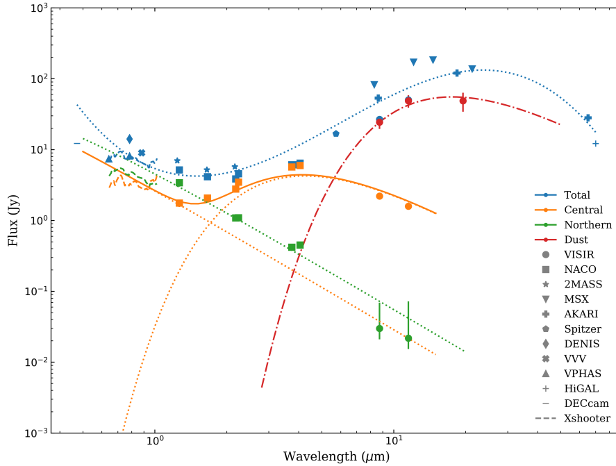
Figure 3. The optical and infrared SED of Apep’s components (central binary, northern companion and dust plume) dereddened with A_V = 11.4 (Callingham et al. 2019; Mathis 1990). The SEDs of the Apep system and calibrator stars listed in Table 1 are quoted from the DECcam (g) (Abbott et al. 2018), VPHAS+ (r, i) (Drew et al. 2014), DENIS (i) (Epchtein et al. 1999), VVV (Z) (Minniti et al. 2010), 2MASS (J, H, Ks) (Skrutskie et al. 2006), IRAC (5.8-micron) (Werner et al. 2004), MSX (A, C, D, E) (Price et al. 2001), AKARI (S9W, L18W, N60) (Doi et al. 2015) and Hi-GAL (70-micron) (Molinari et al. 2016) surveys and the calibrated XSHOOTER spectrum (moving average with 0.02-micron window) from Callingham et al. (2020). The total flux of Apep was decomposed based on aperture photometry extracted from NACO and VISIR imagery. The northern companion is joined by a black-body spectrum at 34 000 K (dotted green line), the dust plume at 290 K (dash-dotted red line), while the central binary (solid yellow line) can be modelled as the sum of two black bodies at 70 000 K and 1200 K respectively (dotted orange lines).
