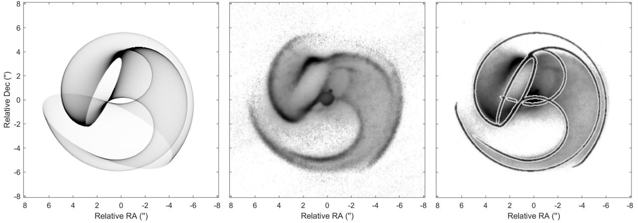
Figure 4. Left: a geometric model of the dust plume of Apep. Middle: edge-enhanced image of Apep at 8.72\mu\text{m} . Right: the outline of the geometric model overlaid on the data.
