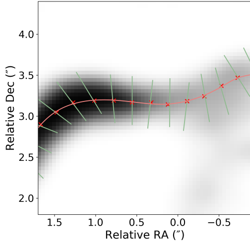
Figure B2. A zoomed in example of ridge-crawler in action showing sample points, search slices and a fitted spline.
