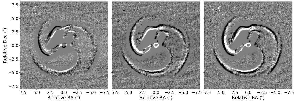
Figure B1. High-pass filtered difference images in which newer epochs have been subtracted from older. Data from 2016 and 2017 (left), 2017 and 2018 (middle), and 2016 and 2018 (right). Negative images (black) always lie exterior to positive ones (white) implying the expansion of the dust plume is clearly visible across all combinations.
