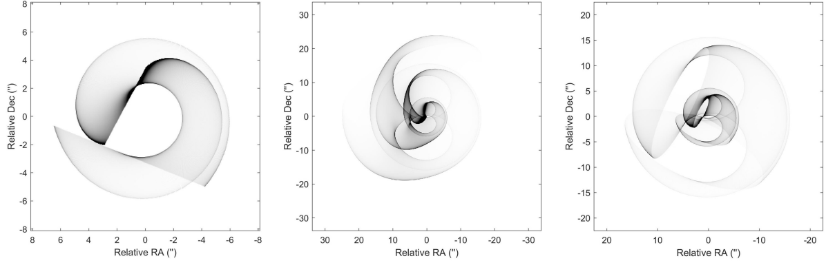
Figure C1. Left: pole-on view of the dust plume (inclination = 0^\circ ). Middle: the geometry of the dust plume assuming constant dust production over 2.5 periods (without the threshold effect) Right: the location and geometry of the dust plume produced from a prior cycle predicted by the threshold effect are presented, overlaid on the model of the dust plume visible in the mid-infrared.
