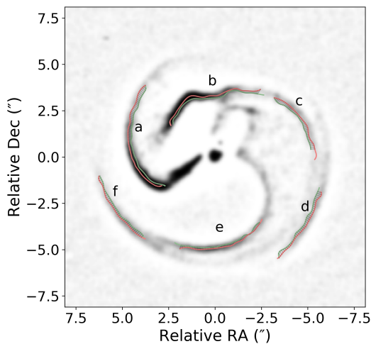
Figure 2. High-pass filtered 8.72\ \mu\text{m} image of Apep labelled with the location of prominent edges detected by ridge-crawler at the 2016 (green) and 2018 (orange) epochs.
