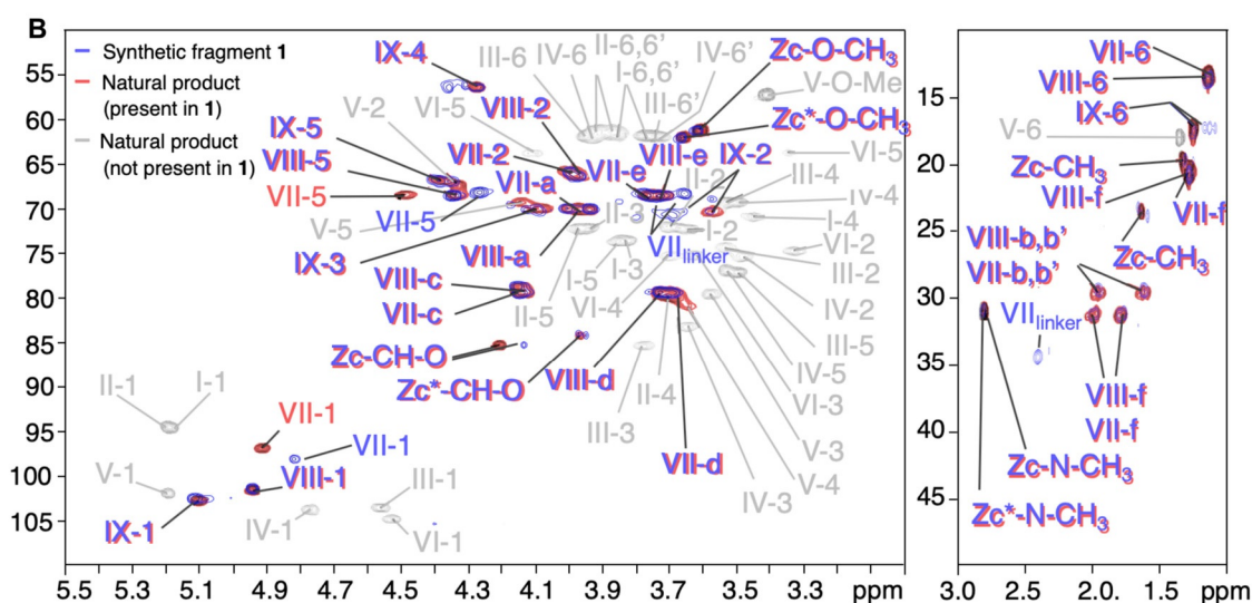
Figure 3. A) Assembly of LOS-IV fragment 1. Reagents and conditions: (1) \text{Ph}_2\text{SO} , TTBP, N-ethyl maleimide, then \text{Tf}_2\text{O} , then TBAI, TPPO, then 3-buten-1-ol, -80^\circ\text{C} to 40^\circ\text{C} (60%); (2) \text{HCl}/\text{HFIP} , TES, DCM (61%); (3) \text{Ph}_2\text{SO} , TTBP, DCM, then \text{Tf}_2\text{O} , then 31, -80^\circ\text{C} to -60^\circ\text{C} (50%); (4) \text{HCl}/\text{HFIP} , TES, DCM (60%); (5) \text{Ph}_2\text{SO} , TTBP, DCM, then \text{Tf}_2\text{O} , then 33, -80^\circ\text{C} to -60^\circ\text{C} (43%); (6) i. trimethylphosphine, THF ii. TEA, HATU, \text{CH}_3\text{CN} (15% over 2 steps); (7) i. \text{LiOH} , \text{H}_2\text{O} , THF ii. \text{Na} , \text{NH}_3 , t\text{-BuOH} , THF (40% over 2 steps). \text{Tf}_2\text{O} = trifluoromethanesulfonic anhydride, TTBP = 2,4,6-tri- t -butylpyrimidine, TBAI = t -butylammonium iodide, TPPO = triphenylphosphine oxide, HFIP = hexafluoroisopropanol, TES = triethylsilane, HATU = 1-[bis(dimethylamino)methylene]-1 H -1,2,3-triazolo[4,5- b ]pyridinium 3-oxide hexafluorophosphate, TEA = triethylamine. B) ^1\text{H} - ^{13}\text{C} HSQC NMR overlay of the acidic OS-IV fraction isolated by Rombouts et al. [12] (red = residues of the natural product present in the synthesized fragment 1, and grey = residues absent of the natural product in the synthesized fragment 1, and blue = synthesized compound 1). I to IX correspond to the nine monosaccharides of the OS-IV. In the overlay most signals overlap. Only signals close to the linker on VII are slightly off, because this area is different from the natural compound, which is linked to a xylose.
