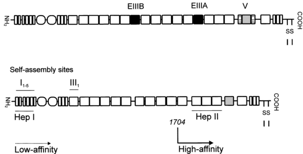
Figure 3. Schematic drawing of the total FN protein sequence (top) and the pFN protein sequence (bottom), with the proposed locations of the FN fragments involved in the accumulation of FN in glomerulosclerotic lesions. Indicated are the EIIIA, EIIIB and V regions, which can be included in or excluded from the protein by alternative splicing of the FN pre-mRNA. Rectangles represent homologous type I repeats, circles represent homologous type II repeats, and squares represent homologous type III repeats. The protein sequence of the high-affinity fraction starts at residue 1704 (homology repeat III 11 ), just before the high-affinity heparin-binding domain (Hep II). The N-terminus of the low-affinity fraction is suggested to be located near the low-affinity heparin-binding domain (Hep I, homology repeat I 1-5 ).
