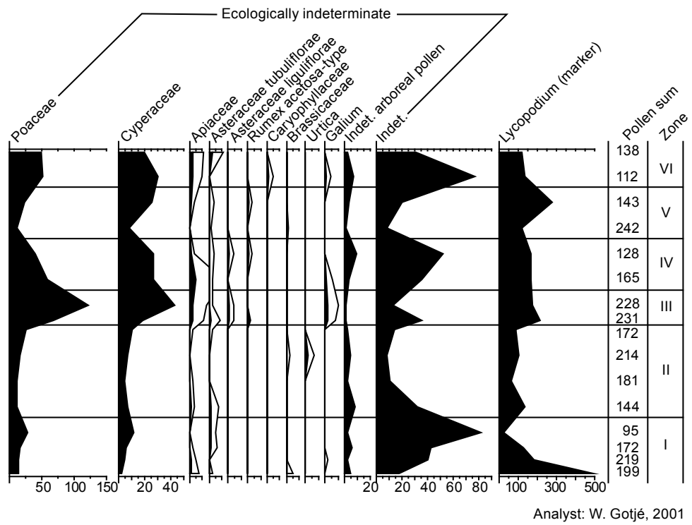
Figure 5.2 Hoge Vaart, prototype core, pollen diagram based on an upland pollen sum, exaggeration 5 x (after Gotjé 2001), part 2.
