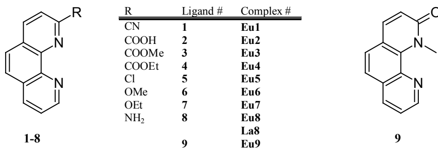
Figure 2.1: An overview of the compounds described in this work. The complexes have the general formula [\text{Ln}(\text{L})_2(\text{NO}_3)_3] , Ln = Eu, La, except for Eu2 (see text). The complex synthesized with ligand 9 analyzes as [\text{Eu}(\text{L})_3(\text{NO}_3)_3] .
