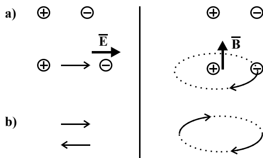
Figure 1.7: a) A schematic representation of the effect of an ED (left) and MD (right) operator on an electron. The ED operator (thick arrow, \vec{E} ) results in a shift of the electron (thin arrow). The MD operator (thick arrow, \vec{B} ) results in shifting the electron over a circular trajectory. b) the effect of the inversion operation on the effect of the ED (left) and MD (right) operators. It can be seen that the effect of the ED operator changes sign, as the direction of the arrow is inversed. Thus, it has odd parity. For the MD operator, inversion does not invert the sense of rotation and so the MD operator has even parity.
