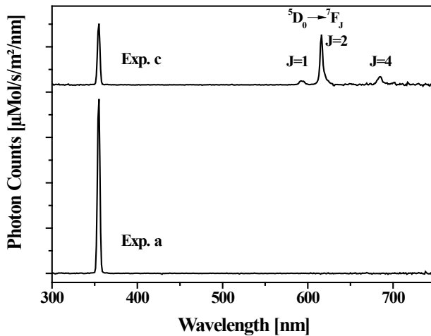
Figure A2: Spectra obtained with \text{BaSO}_4 (exp. a, bottom) and [\text{Eu}(\text{phen})_2(\text{NO}_3)_3] (exp. c, top) placed in the sample holder of the integrating sphere.
