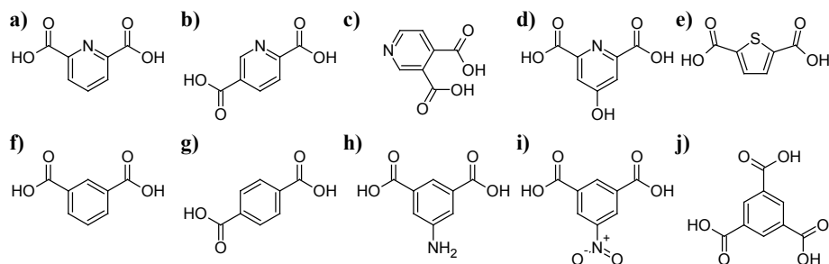
Figure 1.14: Overview of ligands that have been used for preparing MOFs with Ln(III) ions. (a) 2,6-dipicolinic acid, 2,6- H_2dpa , (b) 2,5- H_2dpa , (c) 3,4- H_2dpa , (d) 4-hydroxypyridine-2,6-dicarboxylic acid, H_3pdc , (e) thiophene-2,5-dicarboxylic acid, H_2tbc , (f) 1,3-isophthalic acid, 1,3- H_2ipa , (g) 1,4-benzenedicarboxylic acid, H_2bdc , (h) 5- NH_2 -1,3 H_2ipa , (i) 5- NO_2 -1,3 H_2ipa , (j) 1,3,5-benzenetricarboxylic acid, H_3btc [149-152, 154-162].
