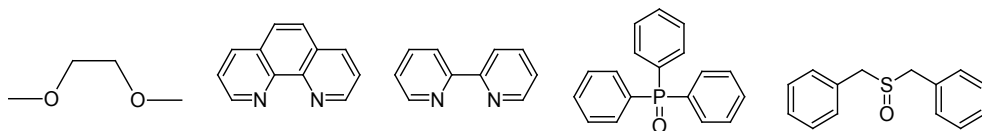
Figure 1.11: Examples of frequently used secondary ligands in lanthanoid(III) tris(dbm) complexes. From left to right: 1,2-dimethoxyethane (monoglyme), 1,10-phenanthroline (phen), 2,2'-bipyridine (bpy), triphenylphosphineoxide (tppo), dibenzylsulfoxide (dbso).
