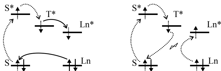
Figure 1.9: Schematic representation of Dexter (left) and Förster energy transfer mechanisms between the ligand and the lanthanoid ion. Transfer of electrons between the ligand and lanthanoid ion are indicated by solid arrows, dotted arrows indicate electronic processes within the ligand or lanthanoid ion.
