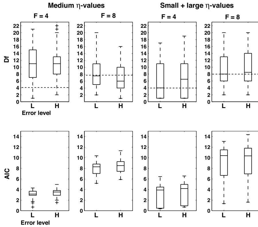
Figure 4.8: Boxplots showing the distributions of 50 simulation samples on 12 objects using a large random sample of the complete set of Gray codes combined with a filter. The experimental conditions are medium (left panels) and small + large (right panels) \eta values, two error conditions, low (L) and high (H), and two levels of true number of features (4 and 8) corresponding to two levels of n/T ratio equal to 16 and 8. The top panels show the effective number of features selected for each sample ( = Df ) with the true number of features represented as a dashed line. The lower panels show the associated AIC_L values.
