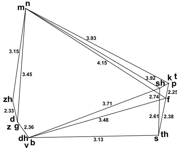
Figure 4.5: Feature Network representation for the consonant data based on the feature matrix selected by the Positive Lasso displayed in Table 4.6. ( dh = \text{ð} ; zh = \text{ʒ} ; th = \text{θ} ; sh = \text{ʃ} ).
