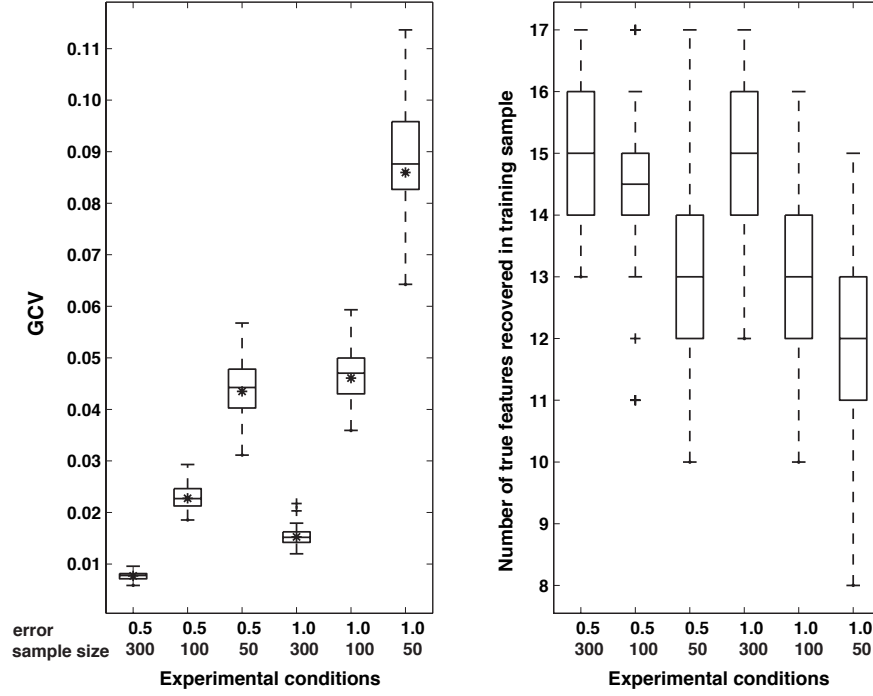
Figure 3.11: Left panel: Distribution of the GCV_{FNM} statistic estimated on the test samples based on the tree topology inferred for the training samples under all experimental conditions for 100 simulation samples. The asterisk in each box represents the mean of the true GCV_{FNM} values. Right panel: Distribution of the number of cluster features equal to the true cluster features ( T_C = 17 ) present in the tree topologies obtained for the training samples of the same 100 simulation samples in each experimental condition.
