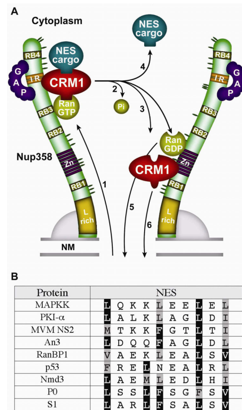
Figure 7. (A). Model of CRM1 export complex disassembly at the cytoplasmic face of the NPC. Nup358 is depicted as a filamentous protein (8) with the different domains indicated. The orientation is suggested by immuno EM studies (51) and the localisation of the ALK-Nup358 oncoprotein (30). 1. NES/CRM1/RanGTP complexes are translocated through the core NPC and bind to a cargo-dependent CRM1-binding site on Nup358. This binding may be cooperative with RanGTP/Ran Binding Domain (RBD, RB1-4) interaction. 2. RanGTP hydrolysis stimulated by Nup358-bound RanGAP (31, 32) and the RBDs of Nup358 (49, 53, 55). 3. CRM1 can be released into the cytoplasm, as is the NES cargo protein (4) or bind to the LMB insensitive CRM1 binding site on Nup358 that is located in the zinc finger region (3, 42); likewise RanGDP may bind to the zinc finger Ran Binding Domain (54); 5. RanGDP and (6) CRM1 recycle to the nucleus. NM, nuclear membranes; Zn, zinc finger domains; L-rich, leucine rich domain (See full-colour figure in cover). (B). Natural NESs deviate at hydrophobic residues from highest affinity NES sequence. Alignment of the sequence of previously identified natural NESs from MAPKK (17), PKI (52), MVM NS2, Xenopus An3 (2) RanBP1 (37) p53 (45) and Nmd3 (47) and the artificial P0 and S1 NESs. Consensus hydrophobic residues are shaded, hydrophobic residues identical to the S1 NES are boxed.
