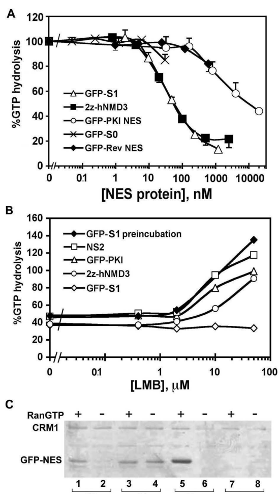
Figure 3. S1 NES binds to CRM1 with high affinity and independent of RanGTP. (A). CRM1 affinities of S0 and S1 peptides in recombinant GFP 3 fusion proteins were measured using the CRM1 RanGAP assay, which measures their ability in the presence of CRM1 to protect RanGTP from RanGAP-stimulated hydrolysis as a function of NES concentration. Regular strength NESs of PKI and HIV-1 Rev, and the high-affinity interaction of 2z-Nmd3 served as references. Error bars denote standard errors of three independent experiments. (B). Differences in LMB sensitivity of export complexes. Different concentrations of LMB were added to RanGTP/CRM1 complexes containing GFP 3 -S1, GFP-PKI, the MVM NS2 peptide or 2z-Nmd3, and stability was measured using the CRM1 RanGAP assay as above. (C). RanGTP independent binding to CRM1 of S1 NES. IgG sepharose columns containing 1.5 μM z-tagged CRM1 were incubated in the absence (-) or presence (+) of 4.5 μM RanGTP as indicated, and in the absence (-) or presence of 1 μM GFP 3 -S1 (S1), GFP 3 -S0 or GFP 3 -Rev (Rev). Bound fractions are visualised using SDS PAGE and Coomassie staining. A fraction of z-tagged CRM1 is co-eluted and indicated on the left.
