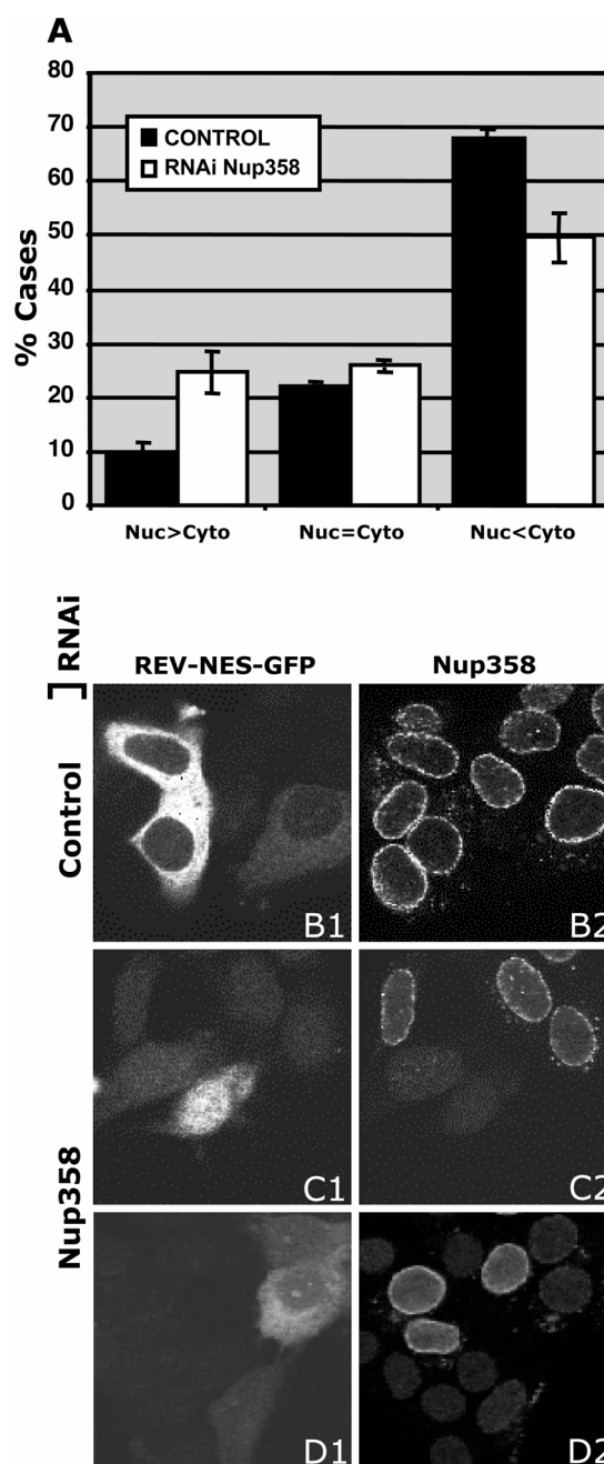
Figure 6: Nup358/RanBP2 knocked down cells are less efficient in CRM1-mediated export of Rev-GFP. (A) Rev-GFP transfected MCF-7 cells were scored for predominant accumulation of GFP in the cytoplasm (nuc < cyto), the nucleus (nuc > cyto), or equal distribution (nuc = cyto) between the two compartments under control (black bars) or Nup358 RNAi (white bars) conditions. The mean distribution in three independent experiments is shown; error bars represent standard errors. Illustrative images of Nup358 (C1 and C2) and empty pSUPER control (B1 and B2) are shown.
