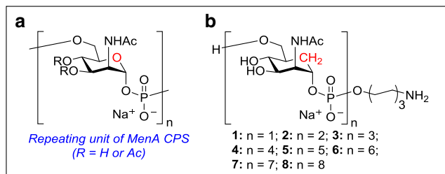
Fig. 1 Structure of MenA CPS and carbaMenA. a Native CPS repeating unit and b target MenA carba analogs.
