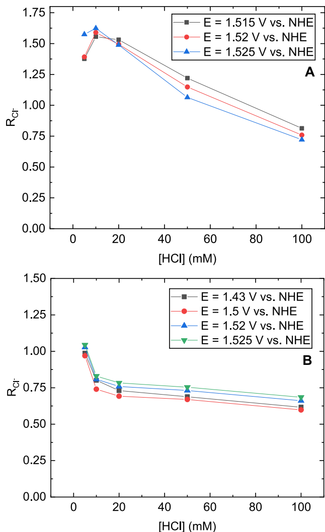
Fig. 7. Chloride reaction orders R_{Cl^-} for the CER, in presence (A) and absence (B) of 10 mM HBr, based on data from Fig. 5. Potentials were chosen to span the range where significant CER occurs, which is much narrower for the CER in presence of Br^- . Data in B are only shown for [Cl^-] values where the ring collection method is reliable [36].
