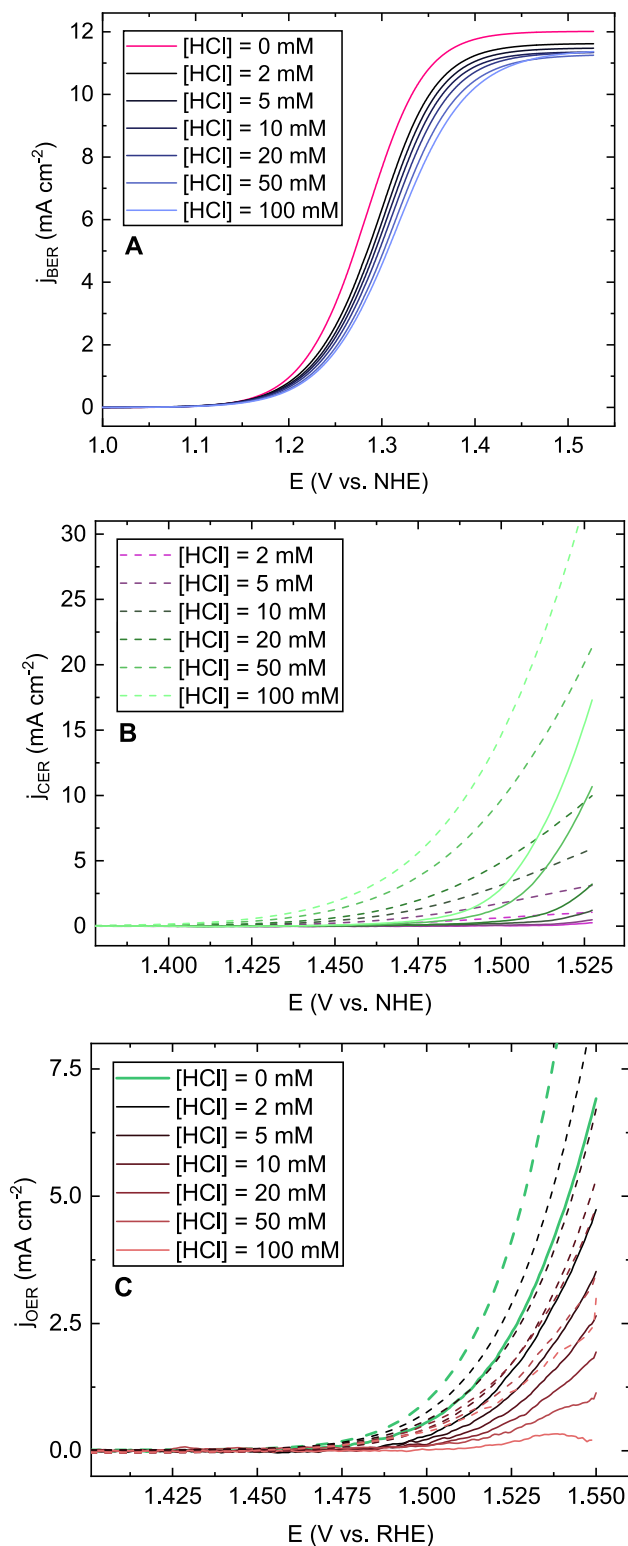
Fig. 5. Individual BER, CER and OER current densities during parallel \text{Br}^- , \text{Cl}^- and \text{H}_2\text{O} oxidation as function of [\text{HCl}] , on an \text{IrO}_x/\text{GC} electrode in 0.5 M \text{HClO}_4 and 10 mM HBr. A: BER current densities derived from generalized logistic fits of the foot and top of BER waves in Fig. 1A. Pink trace shows chloride-free conditions. B and C: CER and OER current densities derived from BER logistic fits and the ring response. Solid traces show CER (B) and OER (C) in presence of 10 mM HBr. Dashed traces are similar experiments in solutions free of \text{Br}^- . Green, solid trace in C shows OER measured in 0.5 M \text{HClO}_4 and 10 mM HBr only (no \text{Cl}^- ). Green, dashed trace in C shows 'pure OER', measured in 0.5 M \text{HClO}_4 (no \text{Cl}^- and \text{Br}^- ).
