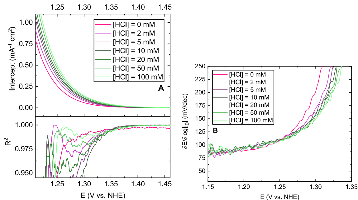
Fig. 2. Kinetic data measured in the potential region of bromide oxidation, in 0.5 M \text{HClO}_4 + 10 mM \text{HBr} , for varying concentrations of \text{HCl} . Data are shown on the NHE potential scale to account for minor ( \pm 4 mV) pH shifts. A: Values of the intercept as function of potential, derived from Koutecký-Levich plots as in Fig. S6. Pink trace shows data when [\text{HCl}] = 0 mM. Top panel shows values of the intercept; lower panel shows corresponding values of the linear correlation coefficient R^2 . B: Tafel slopes obtained from semi-logarithmic data of Fig. 1 (see Fig. S11).
