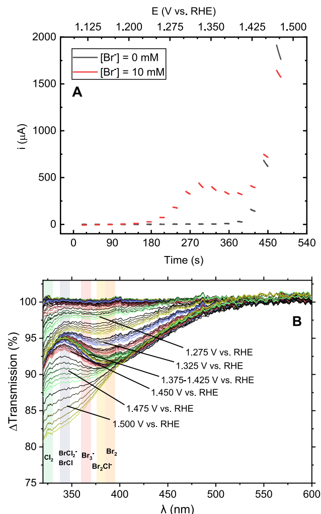
Fig. 4. UV-Vis measurements of a stationary \text{IrO}_x/\text{FTO} electrode in a solution of 0.1 M \text{HClO}_4 + 0.1 M \text{HCl} + 10 mM \text{HBr} . A: Currents measured during the experiment, where only the final 10 s of each potential step are shown for clarity (see Fig. S18 for full data). Currents in \text{Br}^- -free conditions are shown for comparison, upper axis shows the potentials applied at each moment in time. B: Corresponding differences in transmission data of the region where the halogen species adsorb. Varying colors among traces correspond to different potential steps, of which some are indicated; color gradients from dark to light indicate time evolution of the spectra during each potential step. All spectra are difference spectra relative to 1.100 V vs. RHE, the contribution from the \text{IrO}_x layer was subtracted (see main text).
